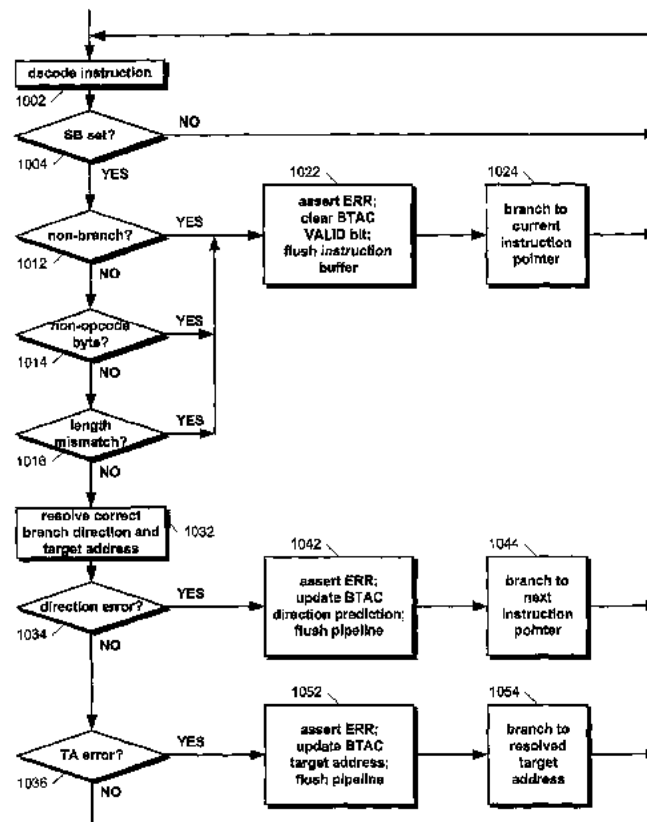
Detection and Correction of Speculative Branch Misprediction
