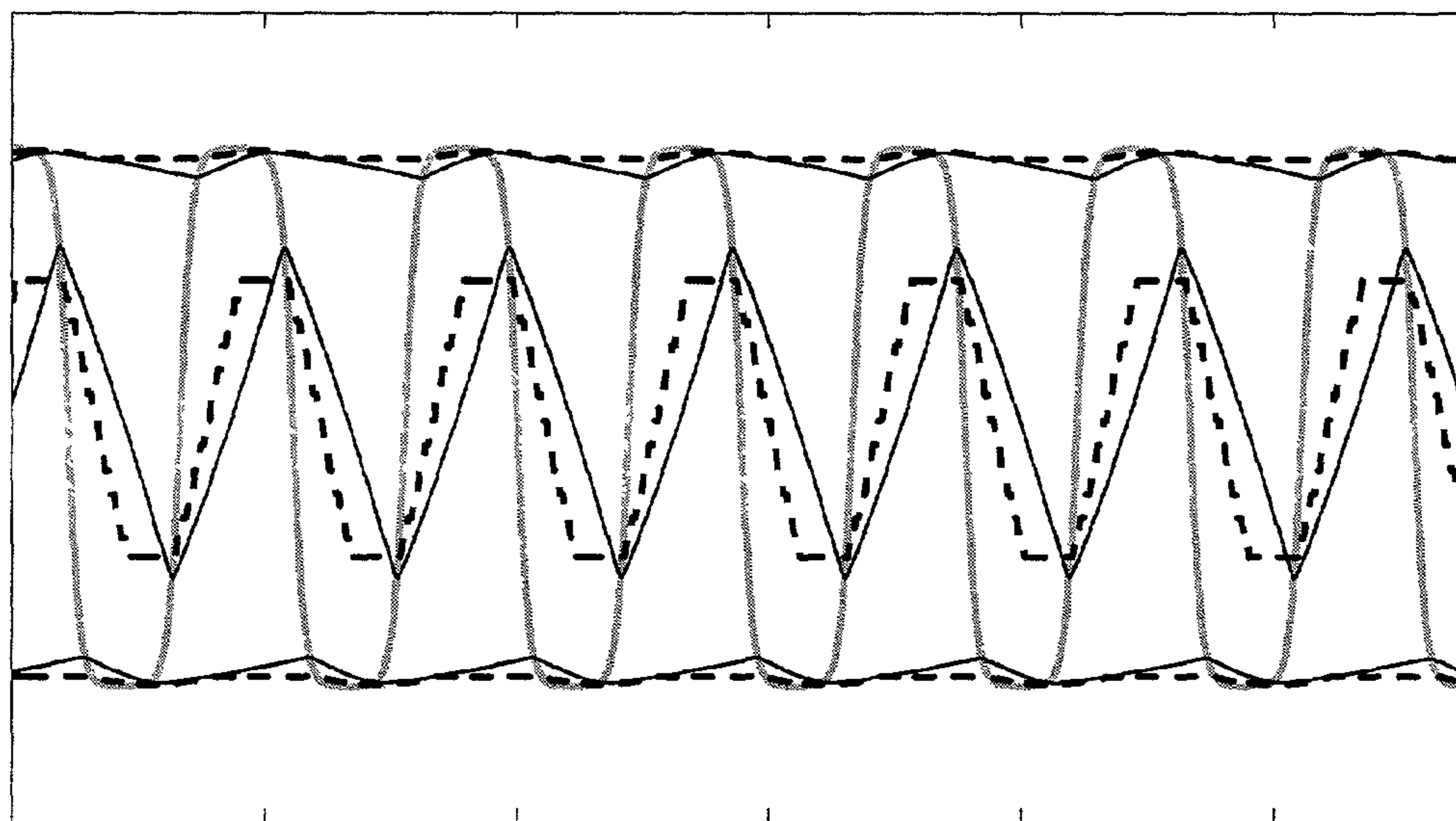
QUARTILE OUTPUTS OF DIGITAL RANK ORDER FILTER AND RC_{10} AARF
