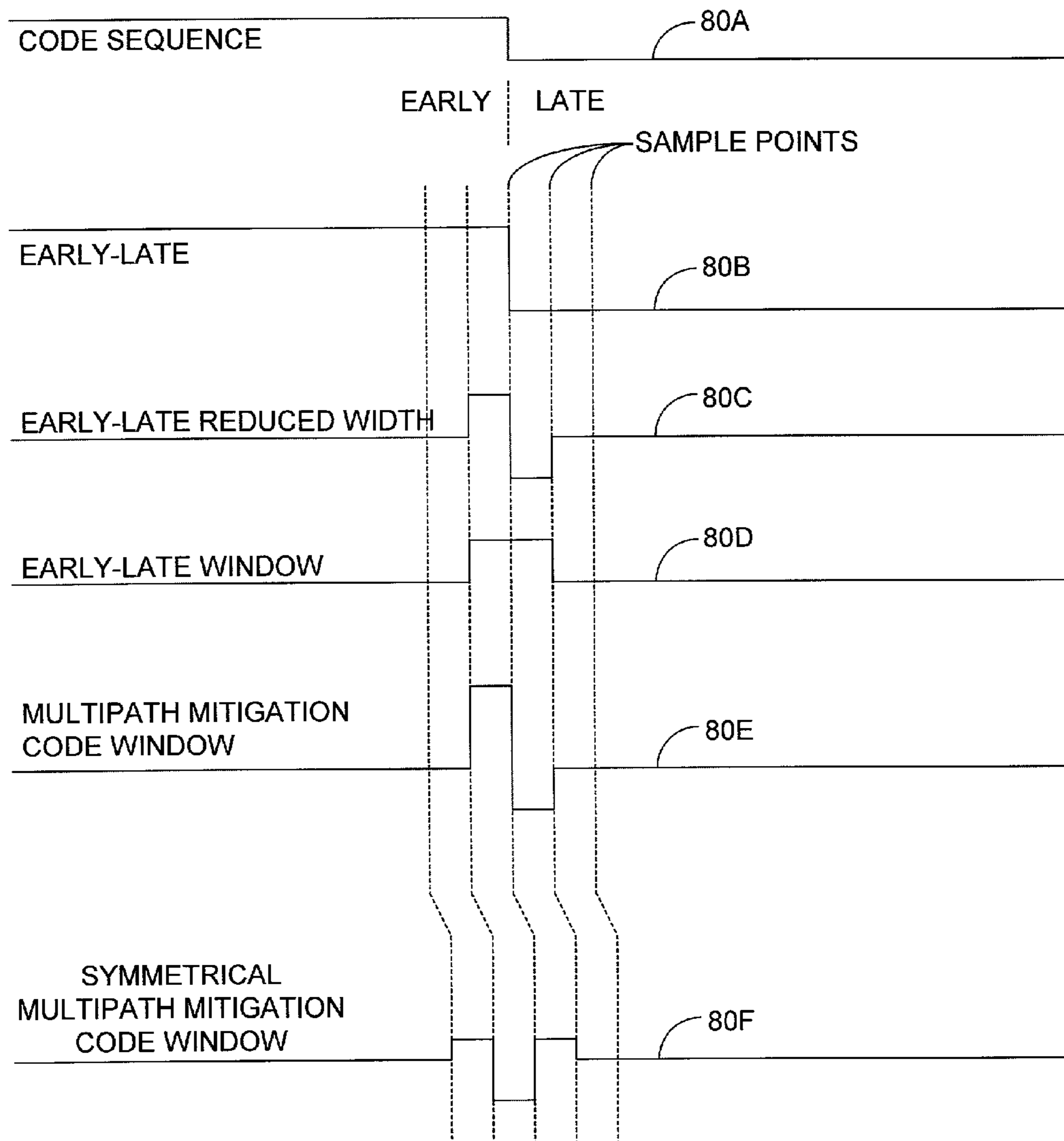
Figure 10 (prior art)
