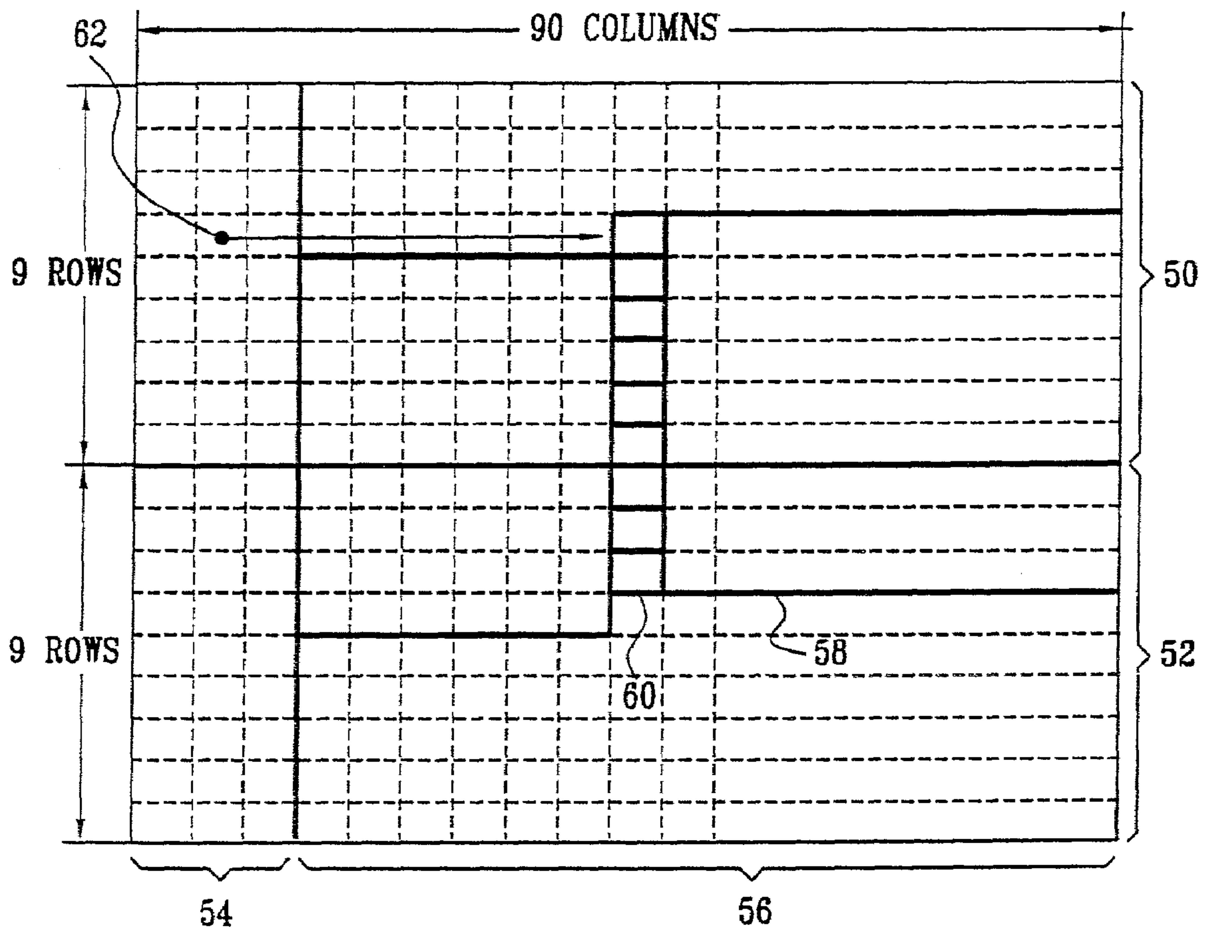
FIG. 3 PRIOR ART
