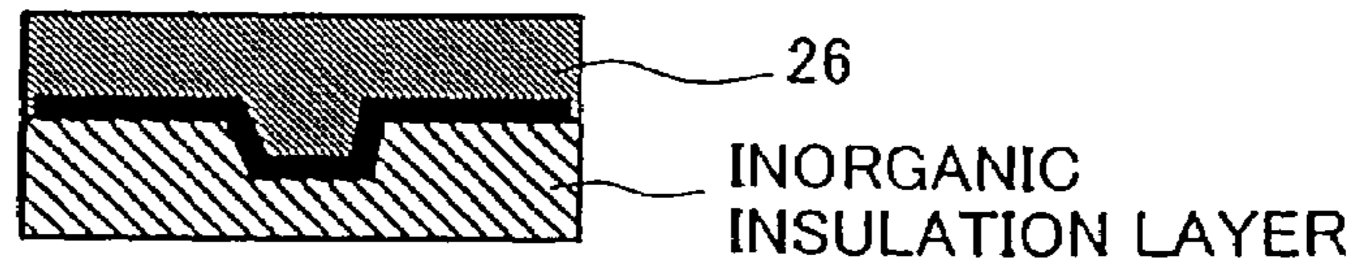
FIG. 12E STEP OF FORMING MAGNETIC LAYER
