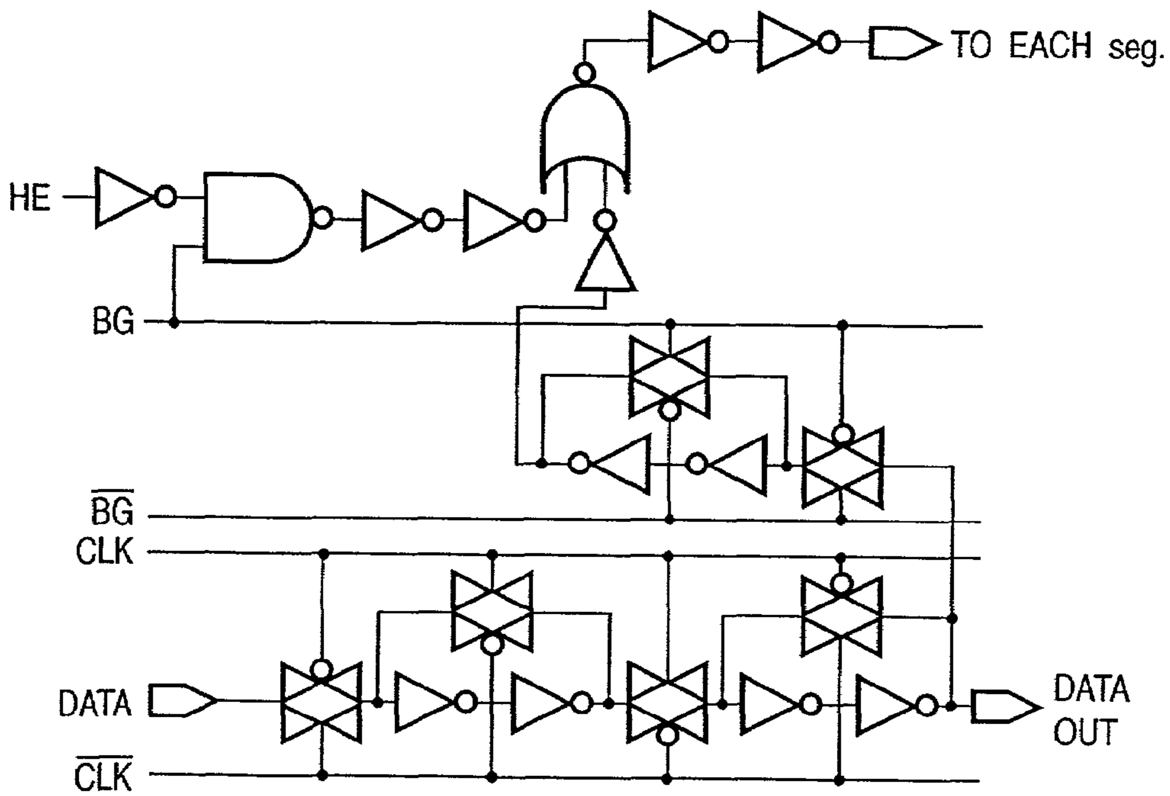
1 bit OF SHIFT REGISTER SECTION
