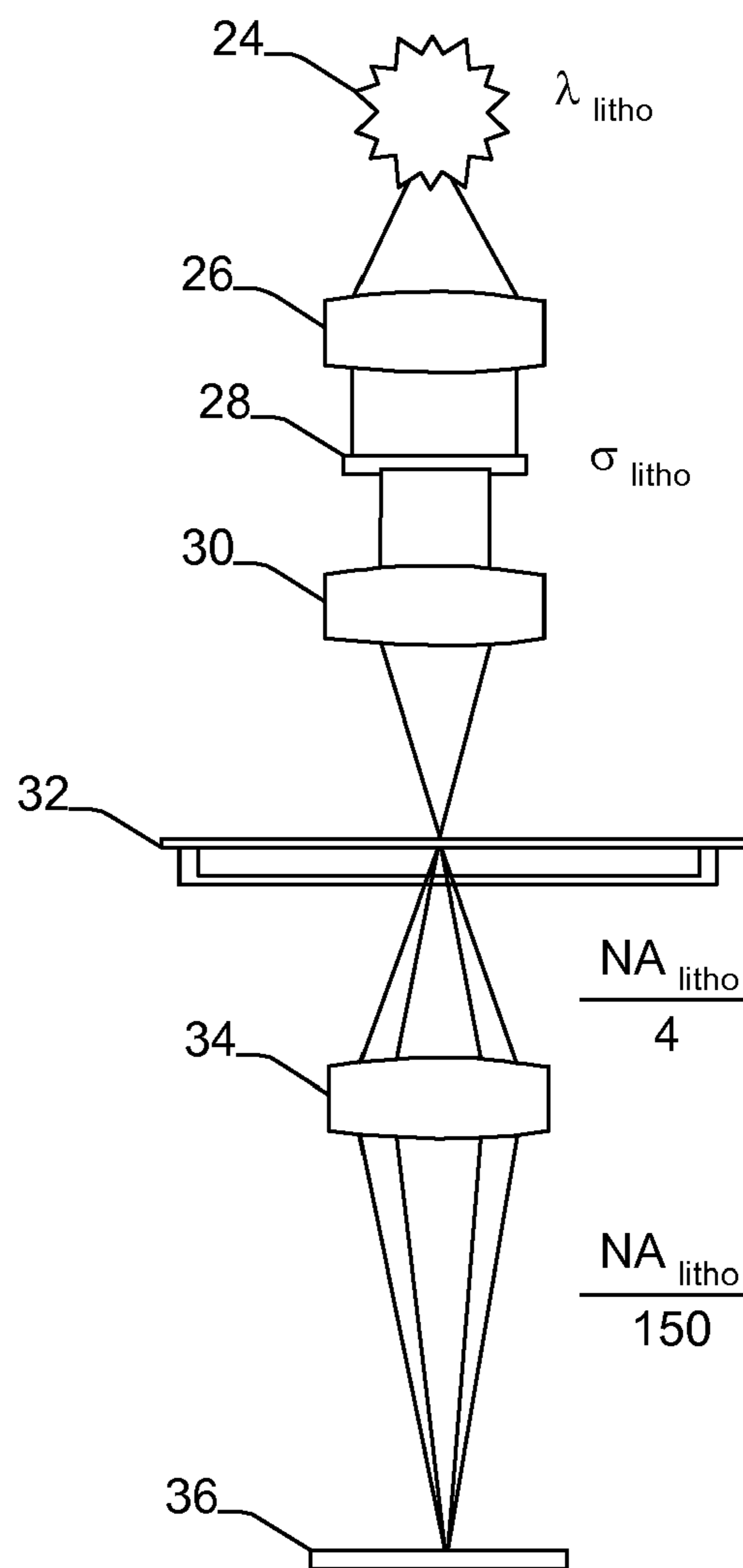
Fig. 2 (Related Art)
