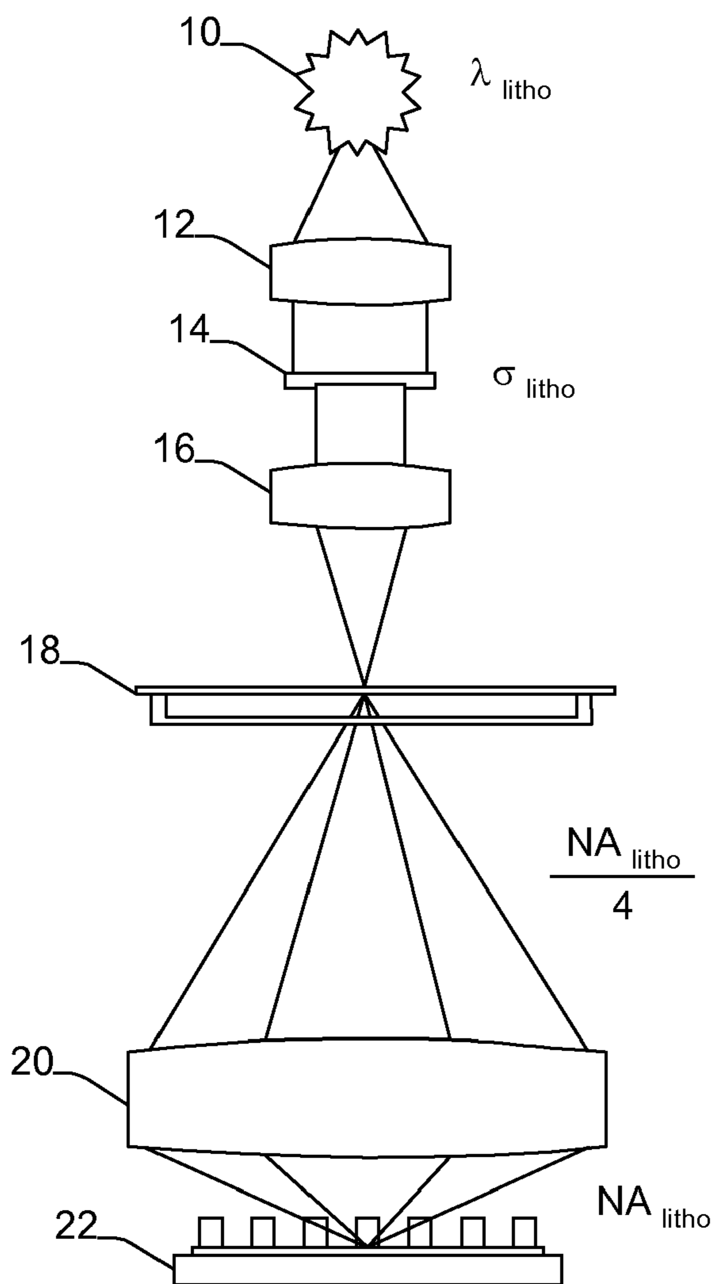
Fig. 1 (Related Art)
