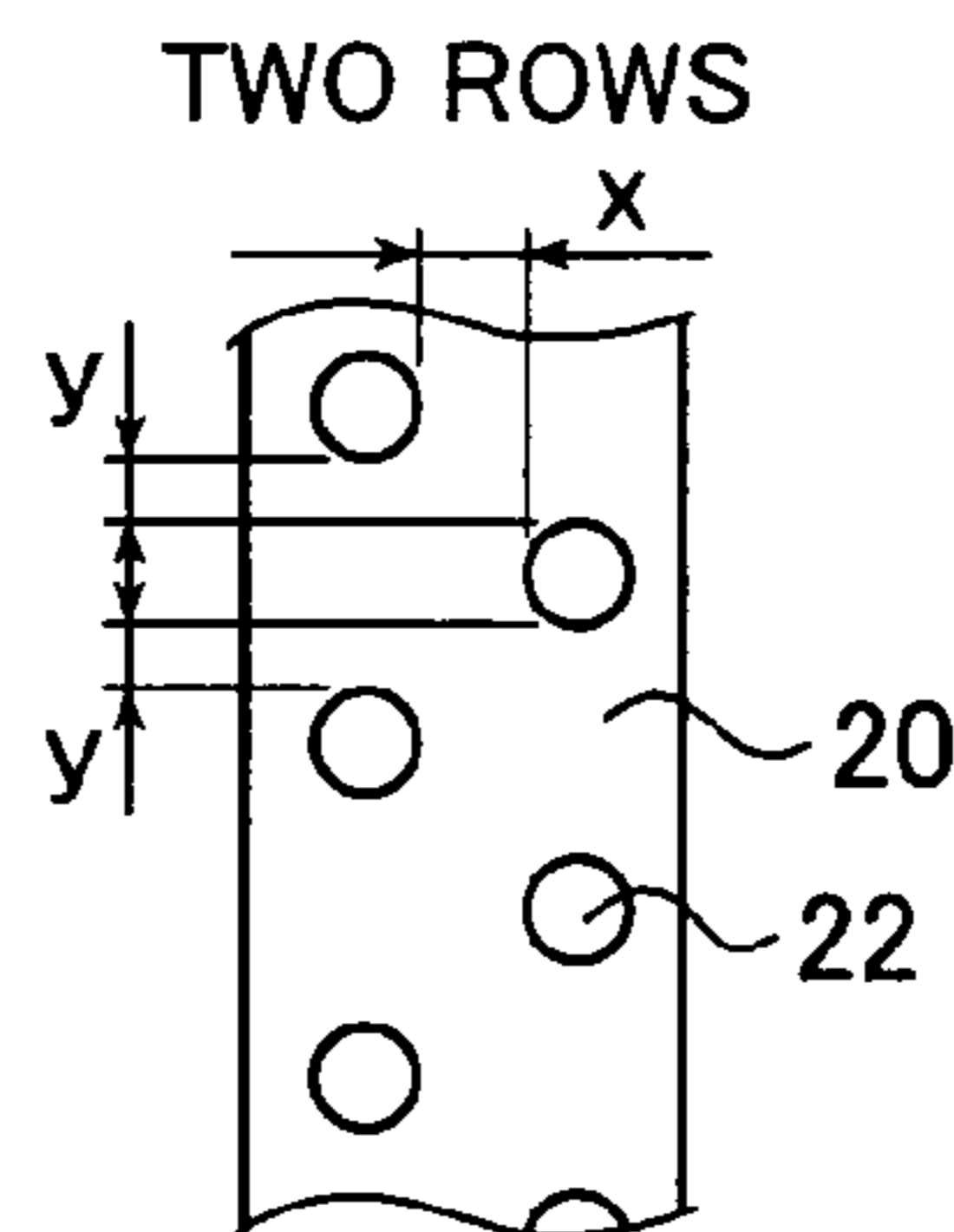
FIG. 11D
