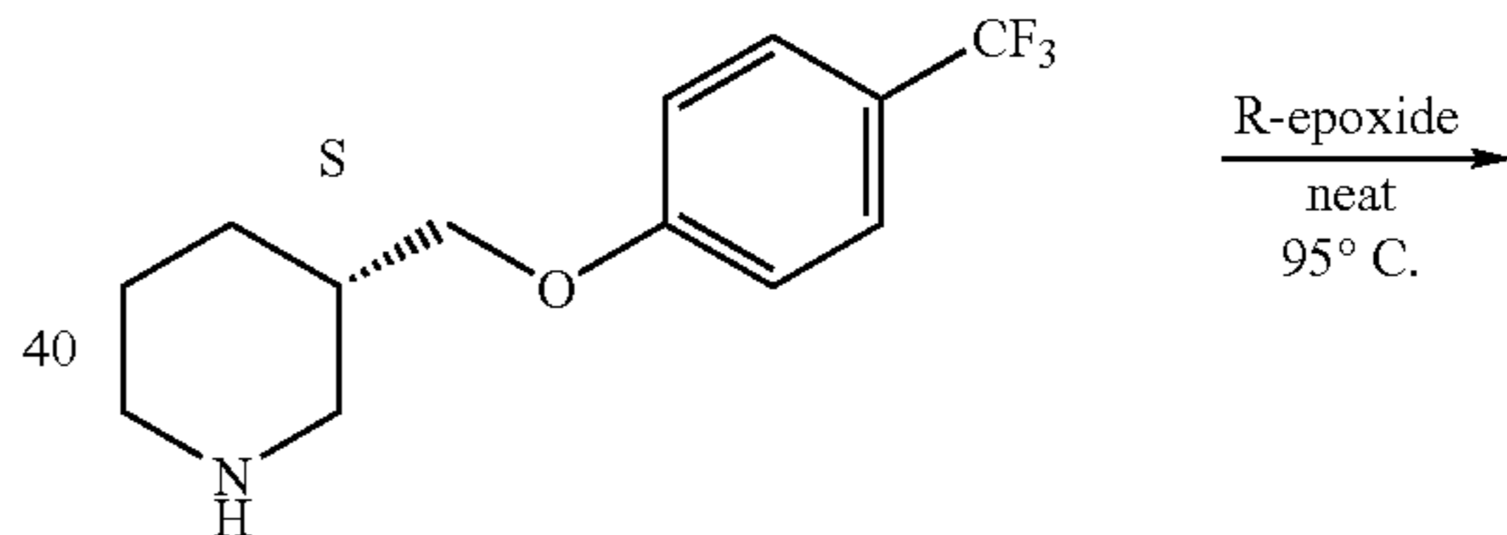
Scheme 3
