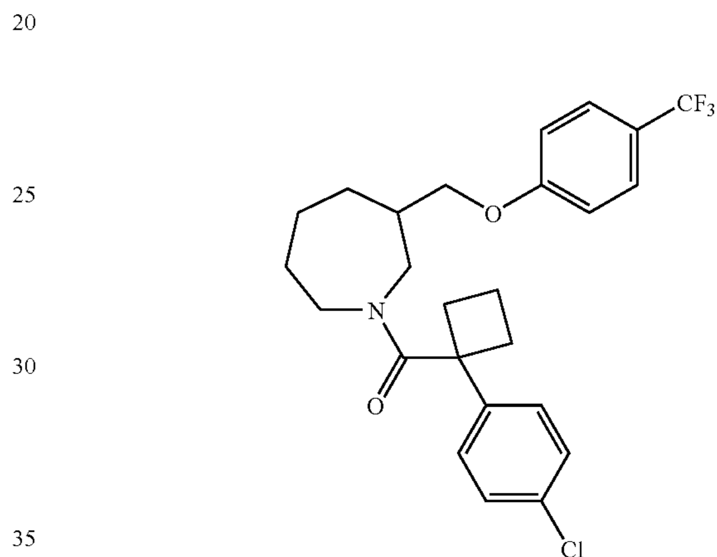
[1-(4-Chloro-phenyl)- cyclobutyl]-(3-(4-trifluoromethyl-phenoxy)methyl-azepan-1-yl)- methanone
