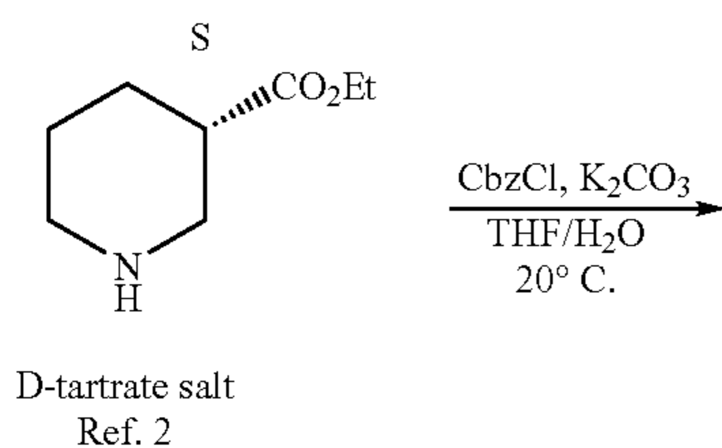
Scheme 2 Synthesis of 124
