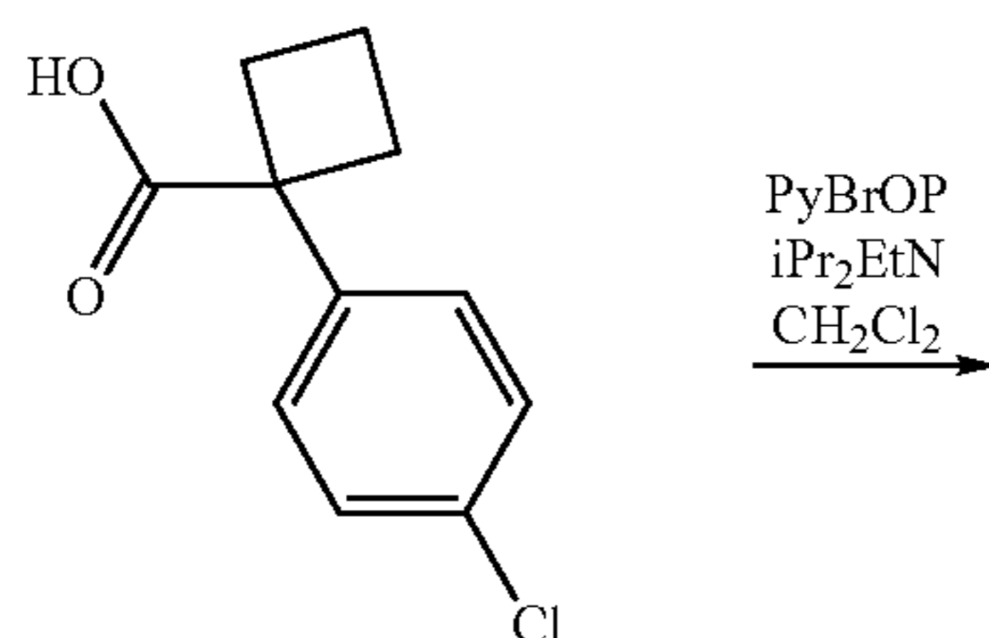
1-(4-Chloro-phenyl)- cyclobutanecarboxylic acid
