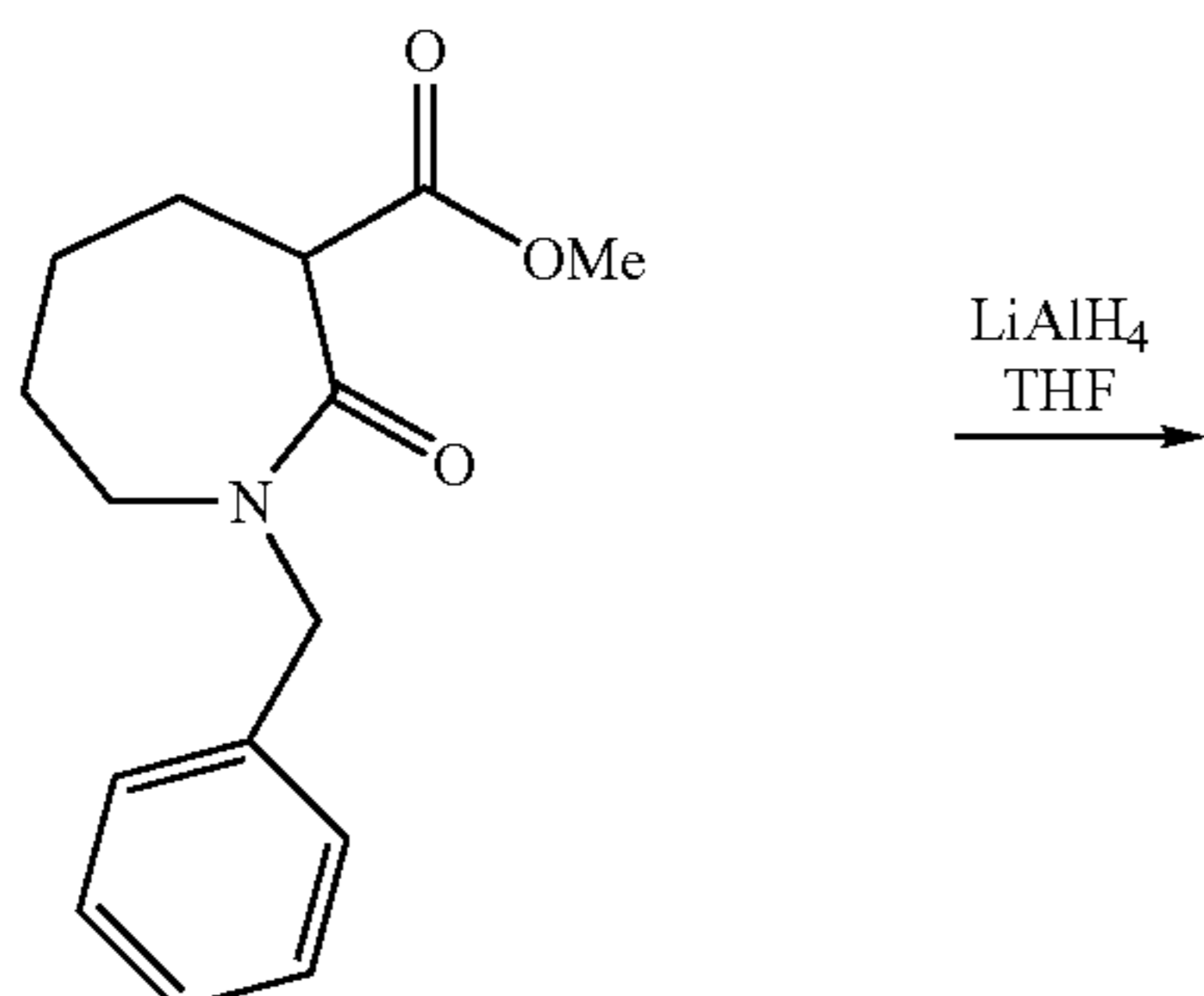
1-Benzyl-2-oxo-azepane-3-carboxylic acid methyl ester
