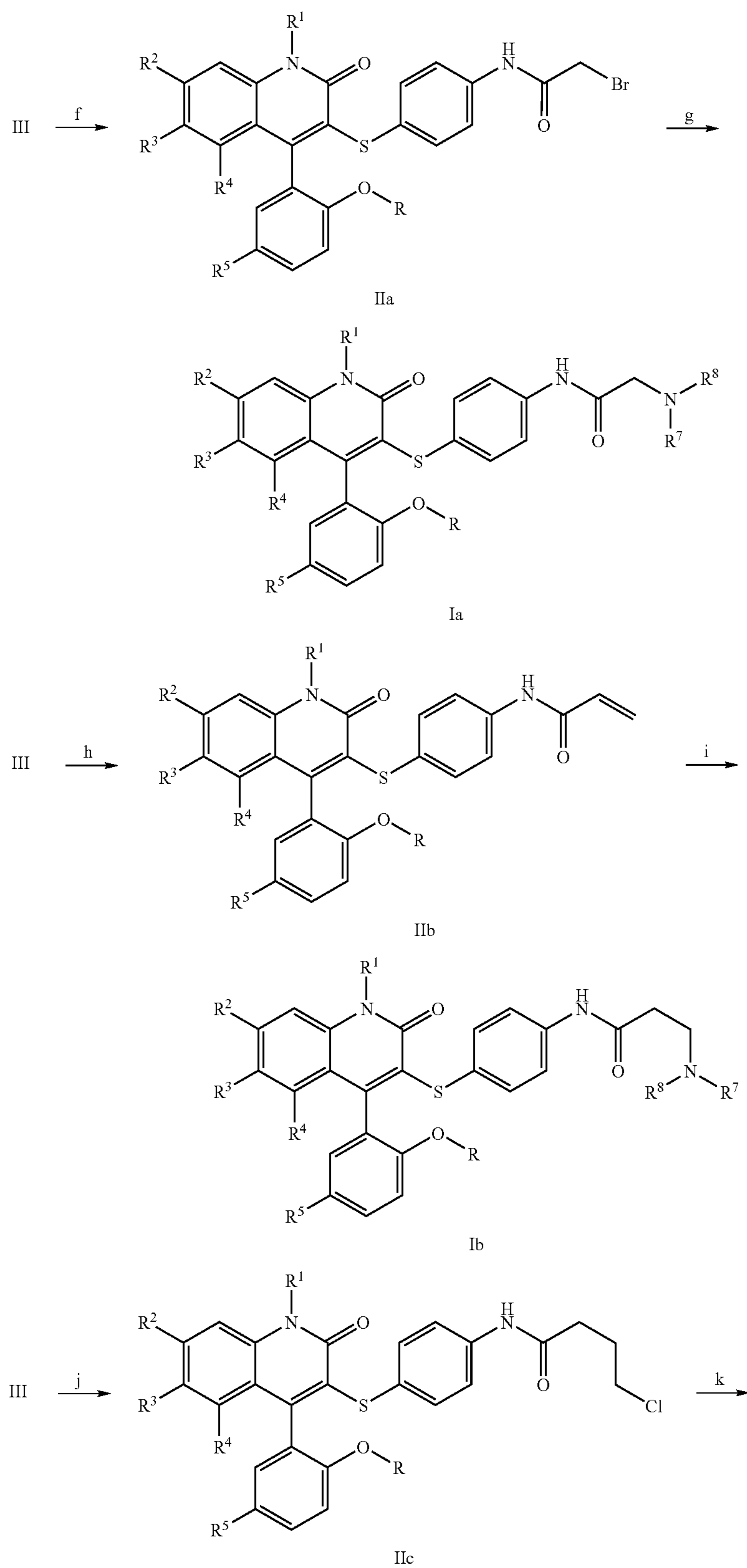
Scheme 2
