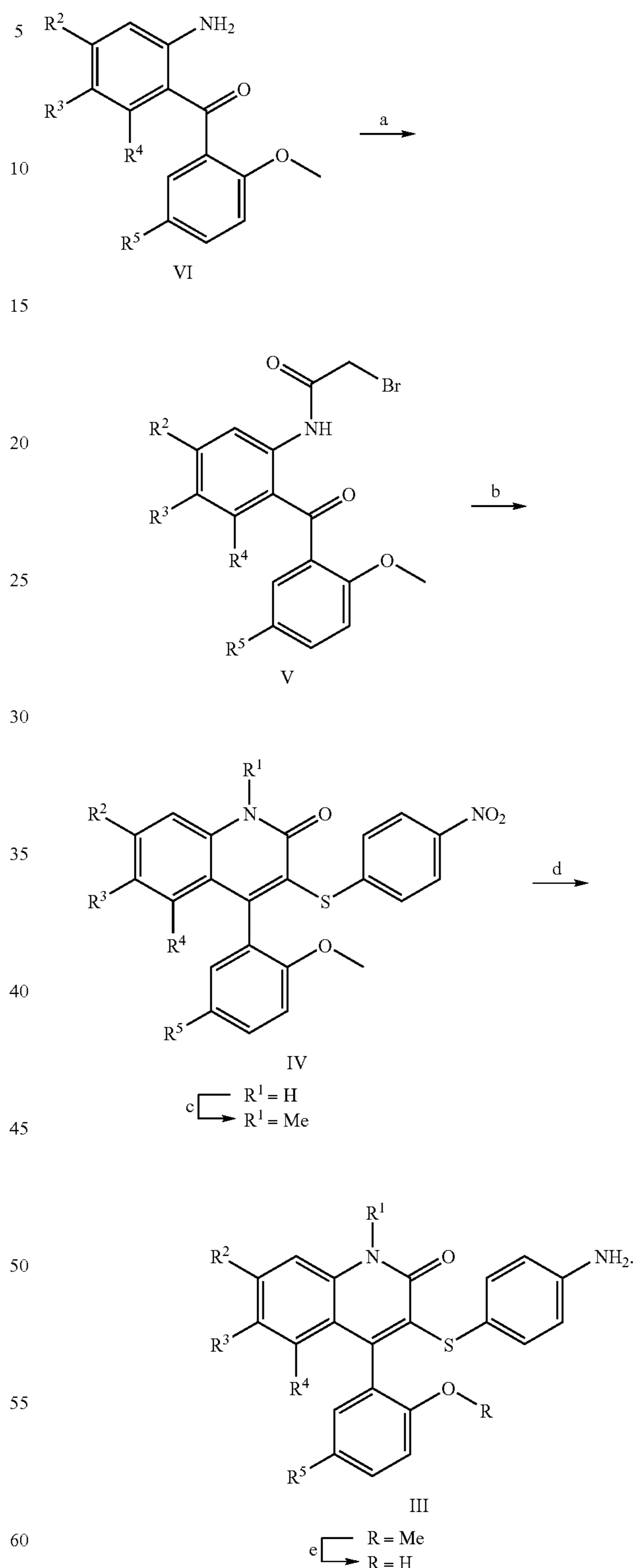
Scheme 1
