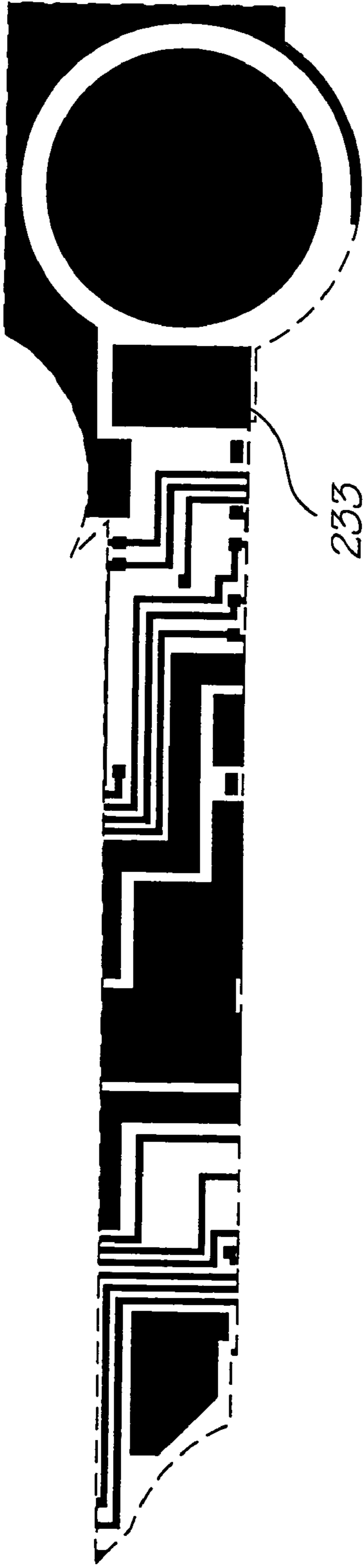
Metal 2 mask
