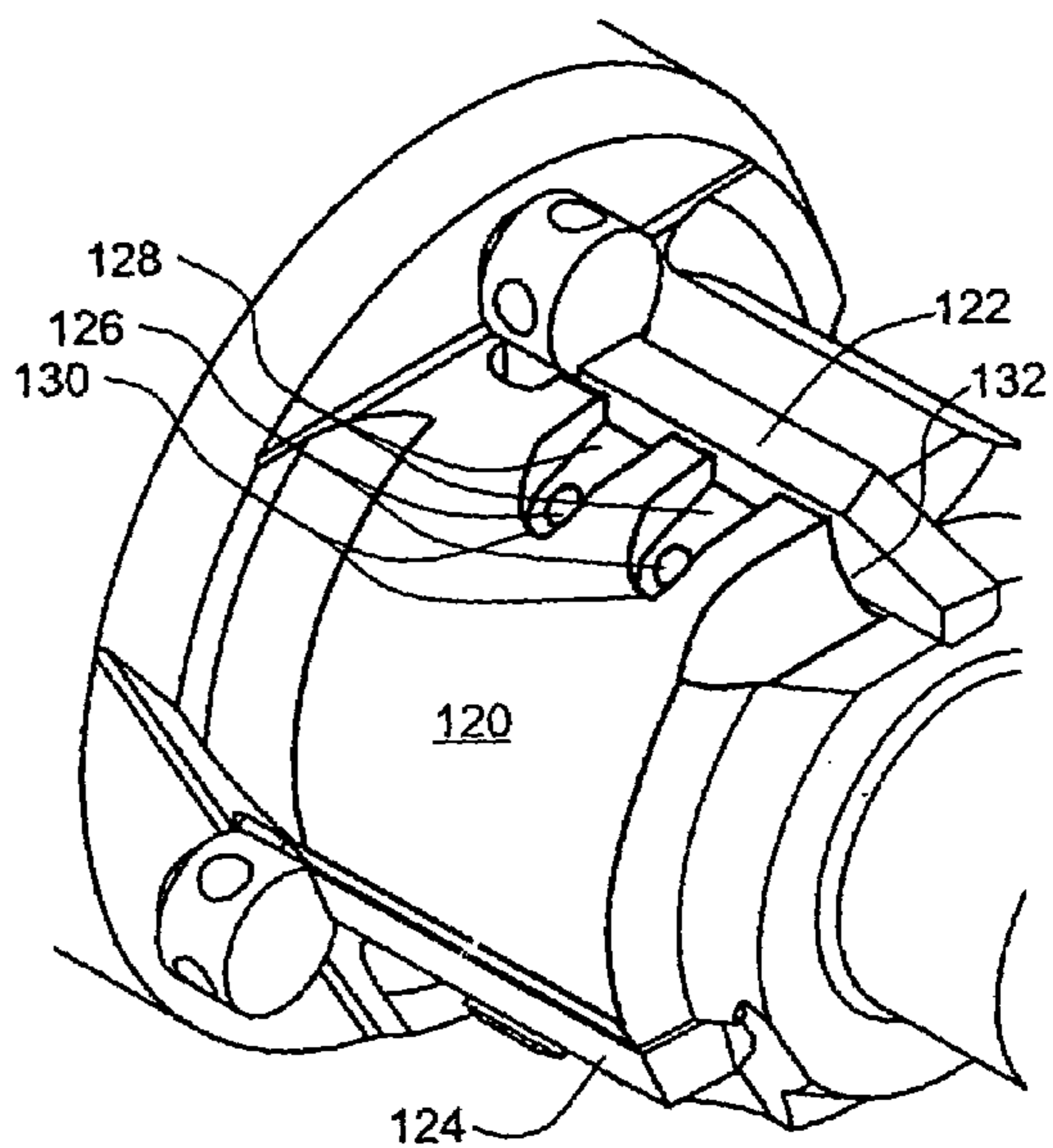
Fig. 1c Prior Art
