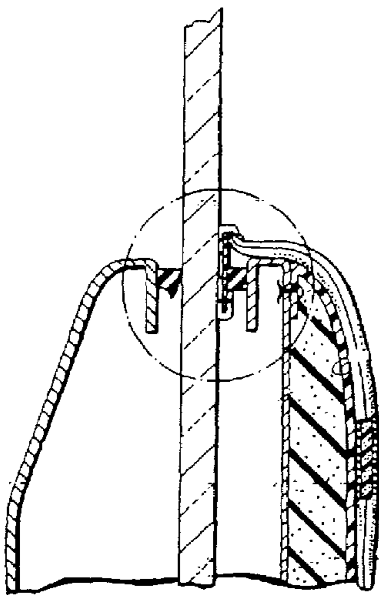
FIG. 3 PRIOR ART
