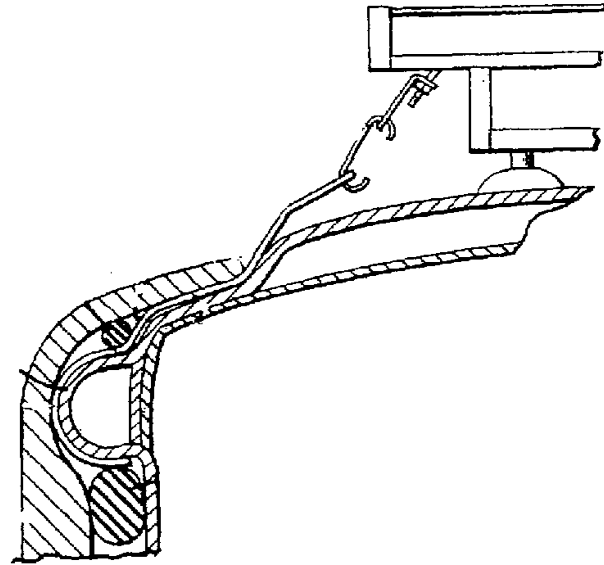
FIG. 2 PRIOR ART
