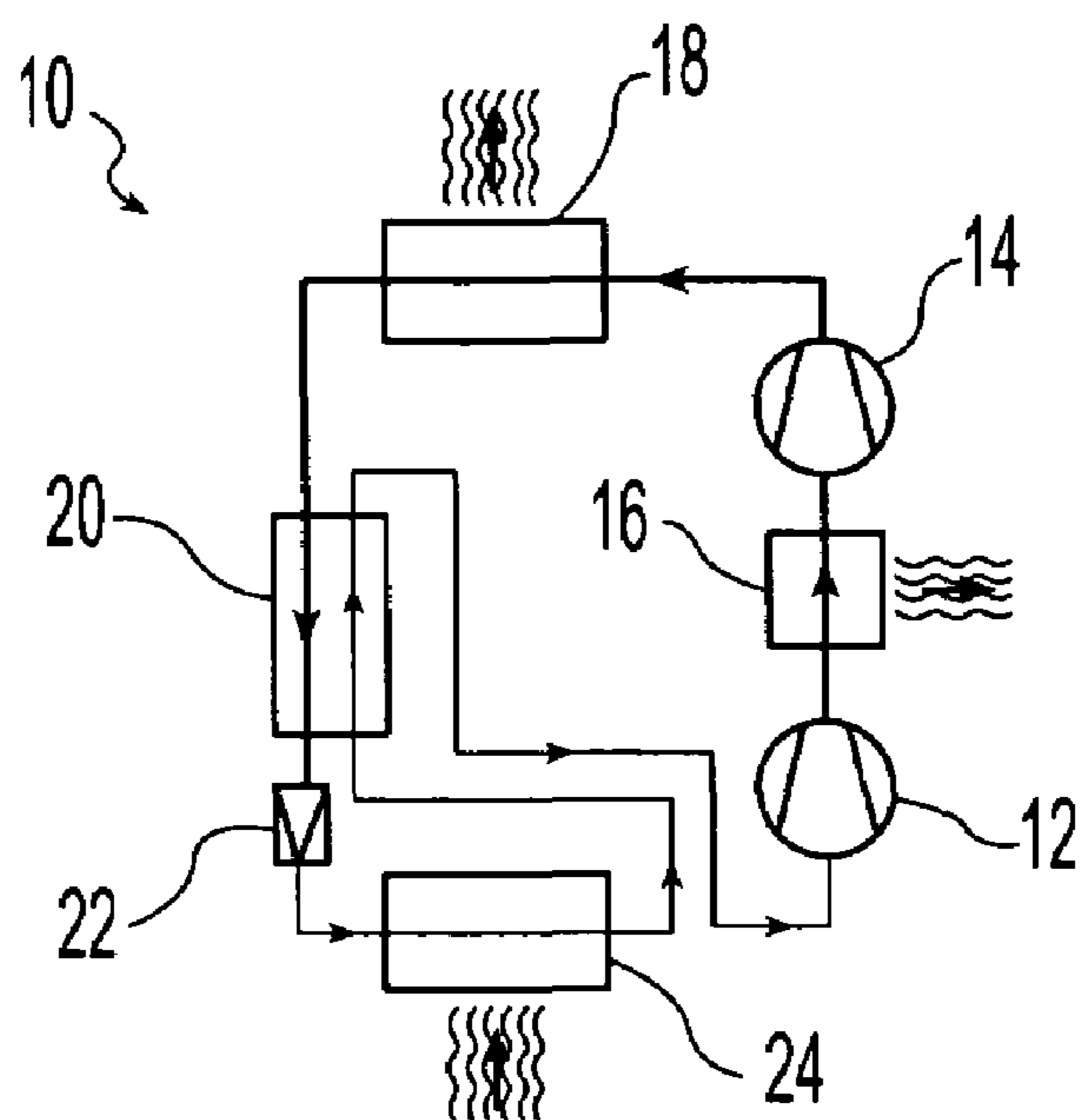
Fig. 1 (Prior Art)
