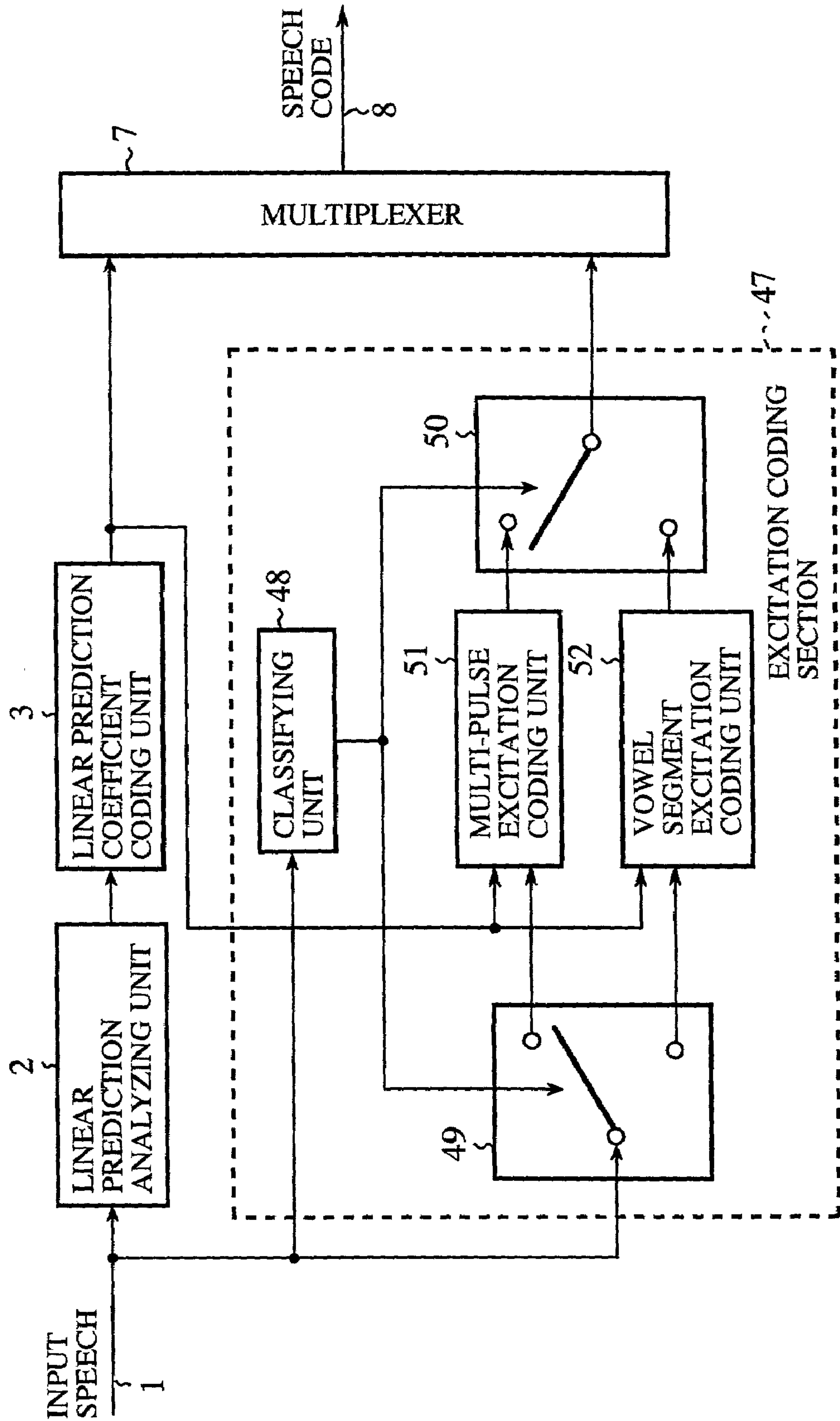
FIG.8 (PRIOR ART)
