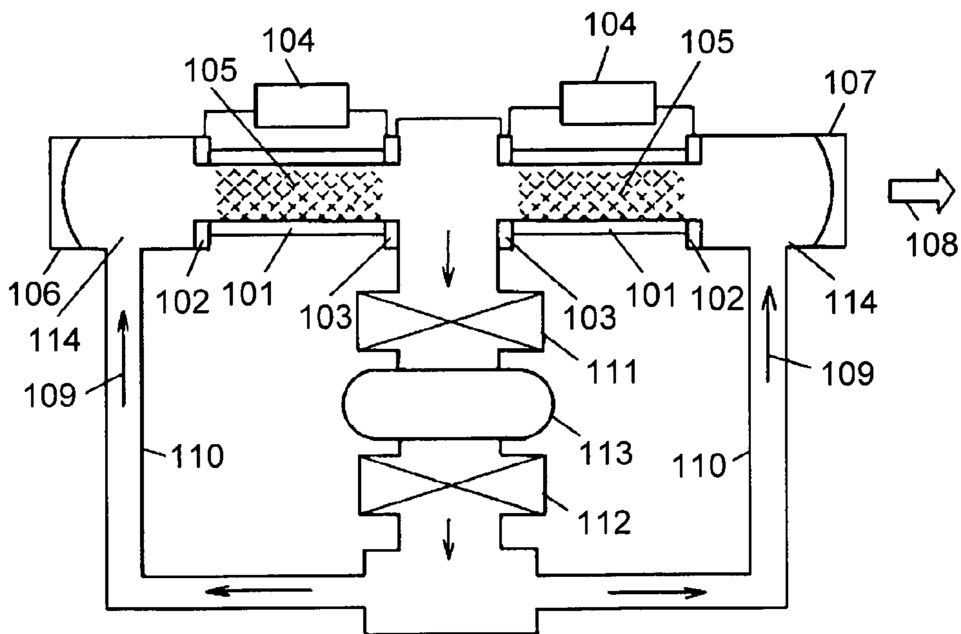
FIG. 12 – PRIOR ART
