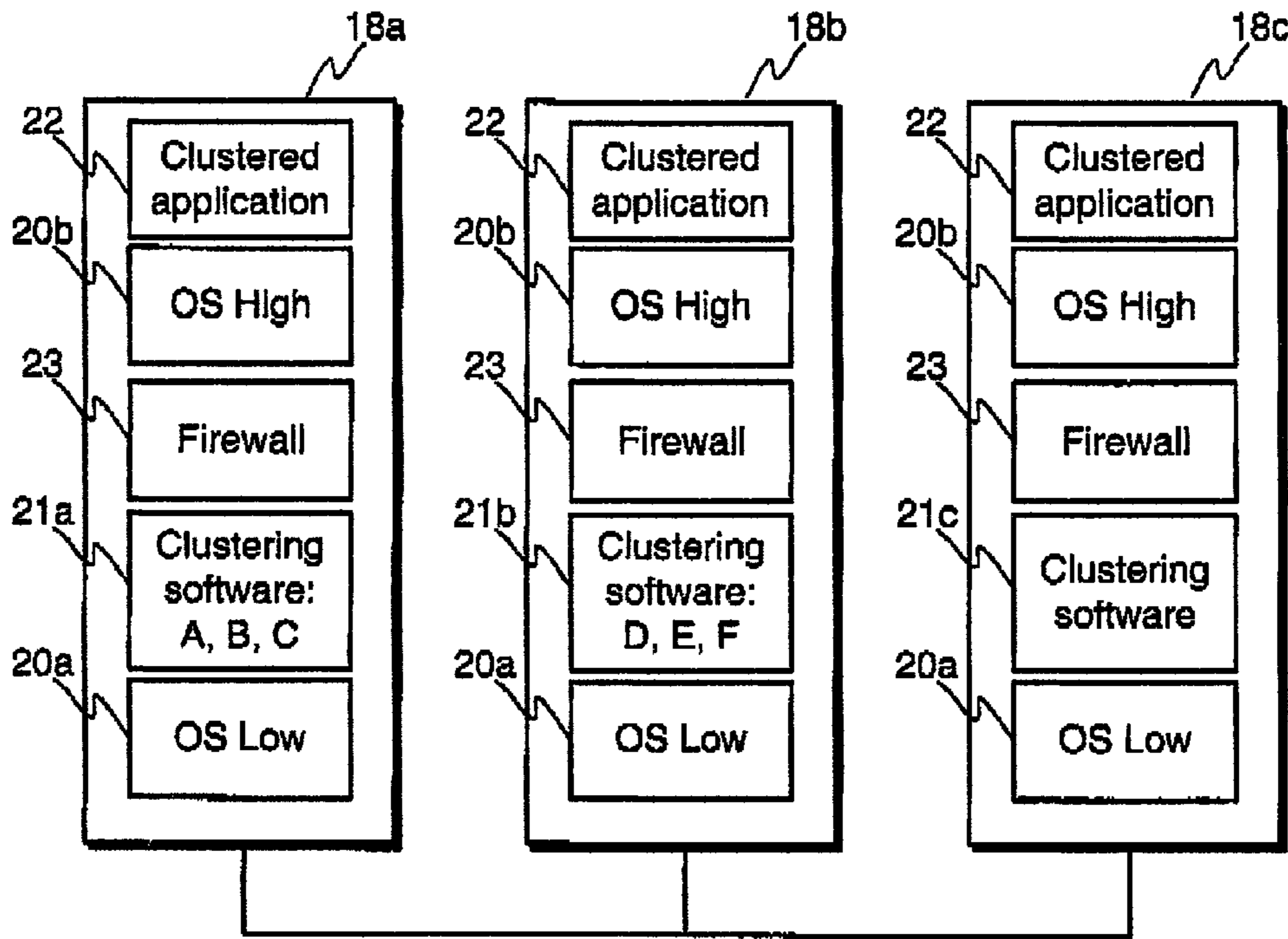
Fig. 2 Prior art
