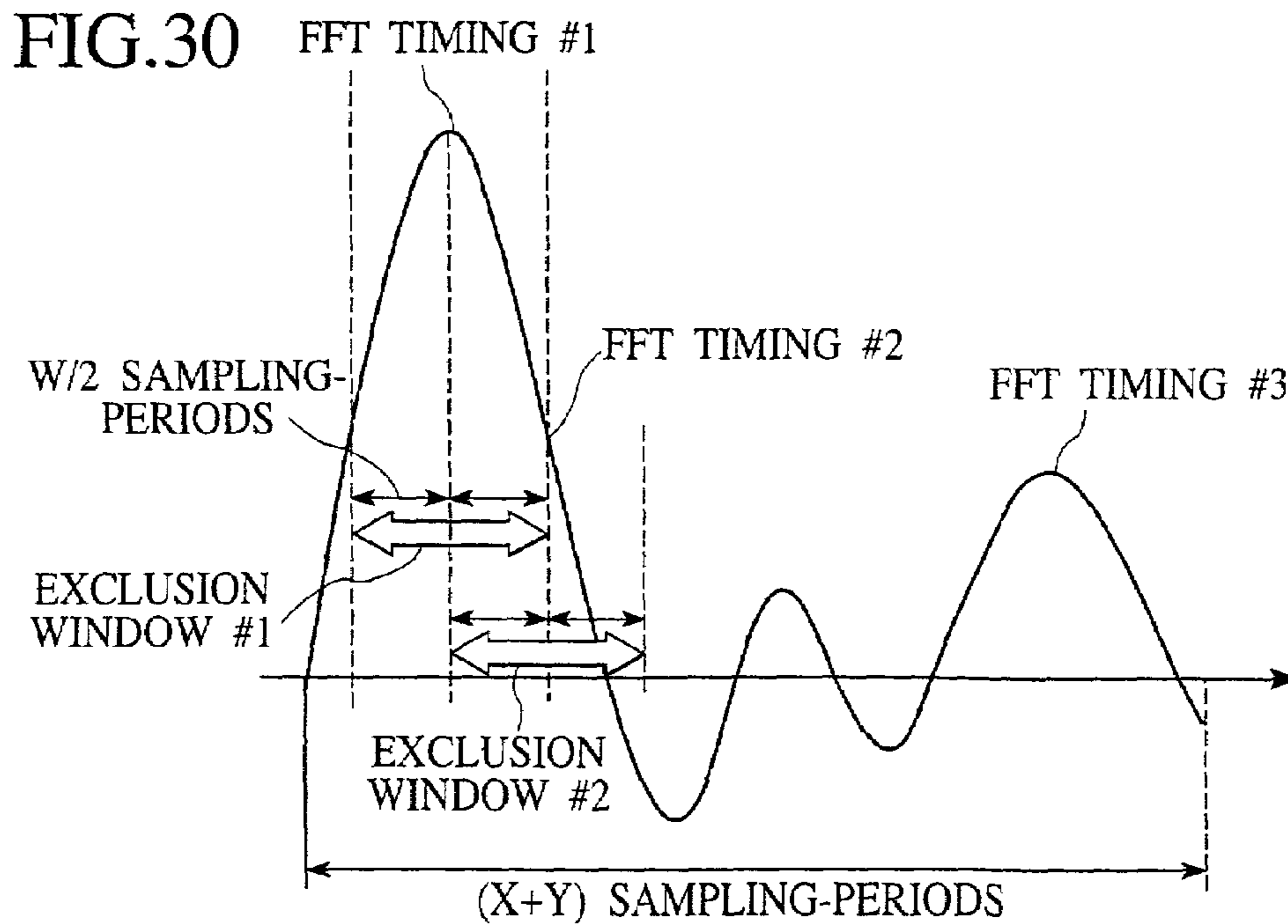
AN EXCLUSION WINDOW IS SET BEFORE AND AFTER A DETECTED FFT TIMING BY W/2 SAMPLING PERIODS (EXCLUSION WINDOWS #1 AND #2 ARE OVERLAPPING)
