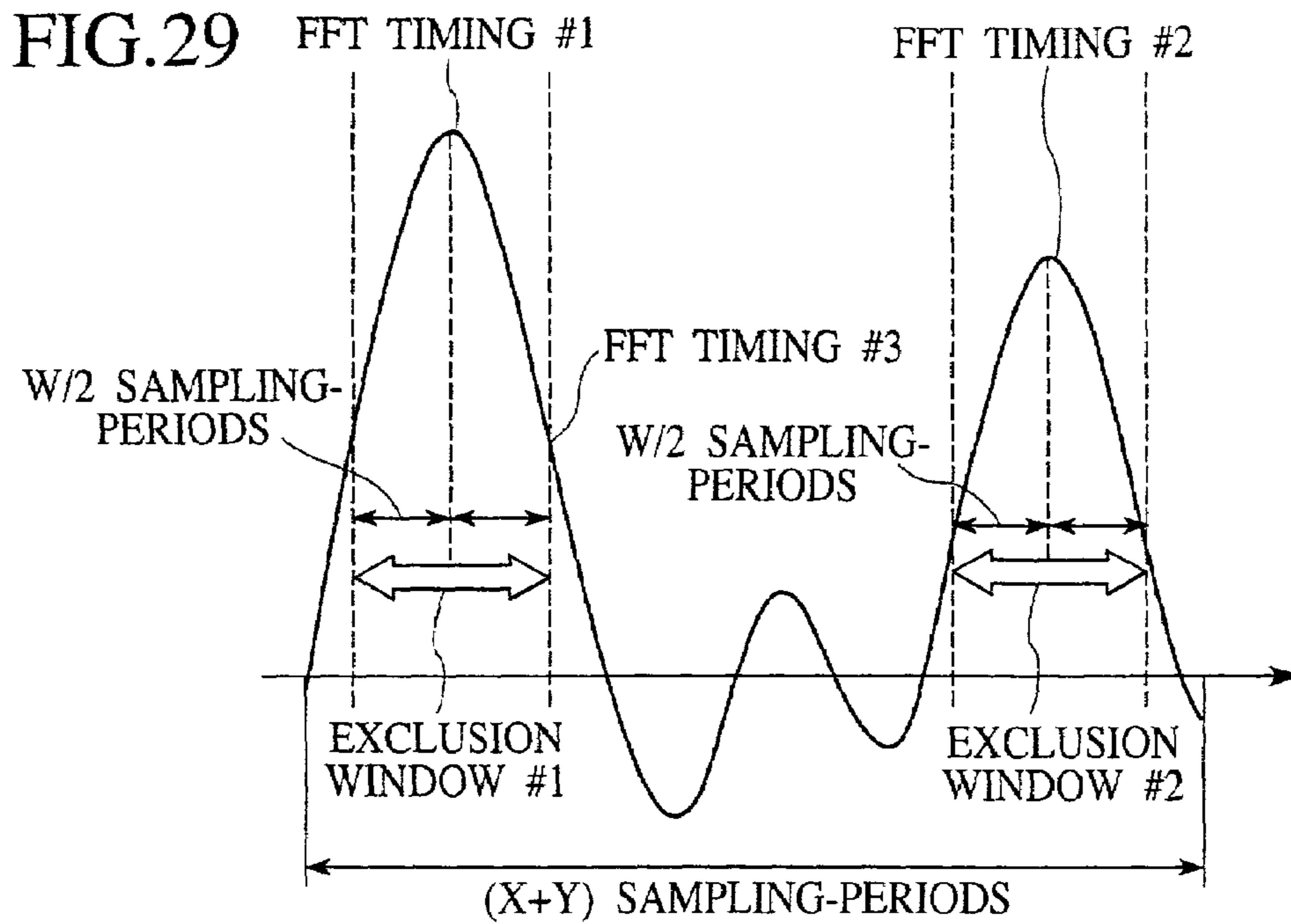
AN EXCLUSION WINDOW IS SET BEFORE AND AFTER A DETECTED FFT TIMING BY W/2 SAMPLING PERIODS (EXCLUSION WINDOWS #1 AND #2 ARE NOT OVERLAPPING)
