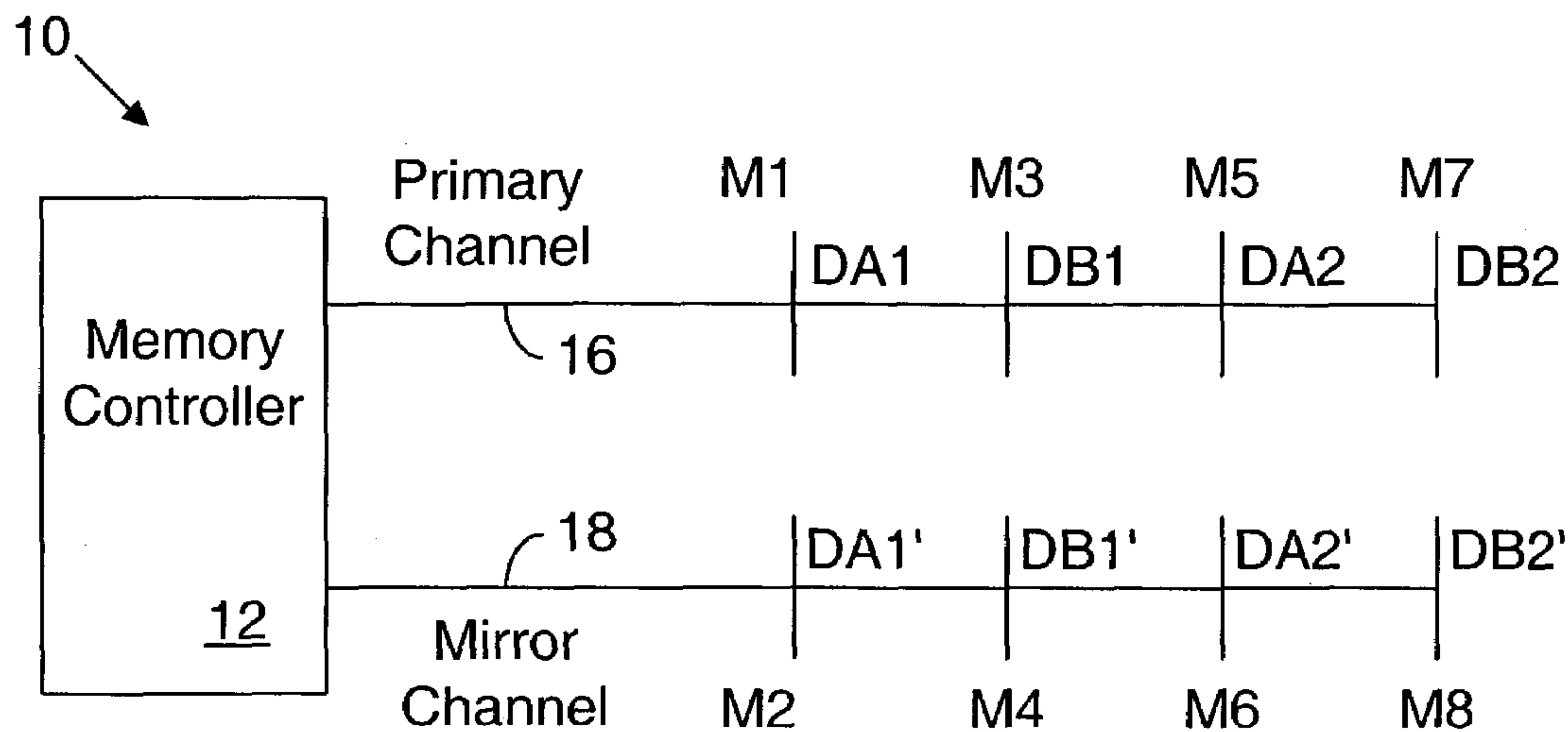
FIG. 1 (Prior Art)
