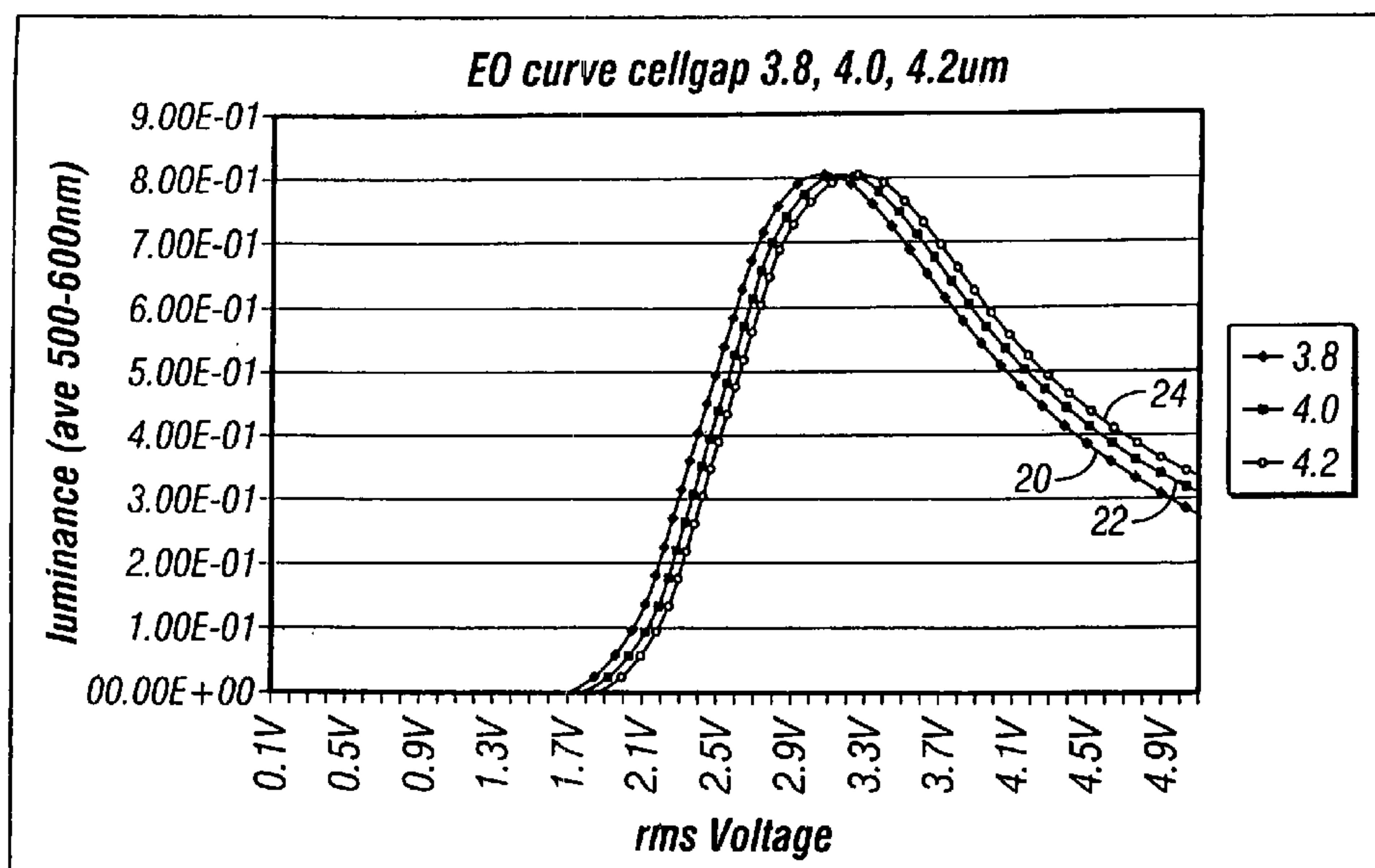
EO curves with 3.8, 4.0, 4.2um cellgaps
