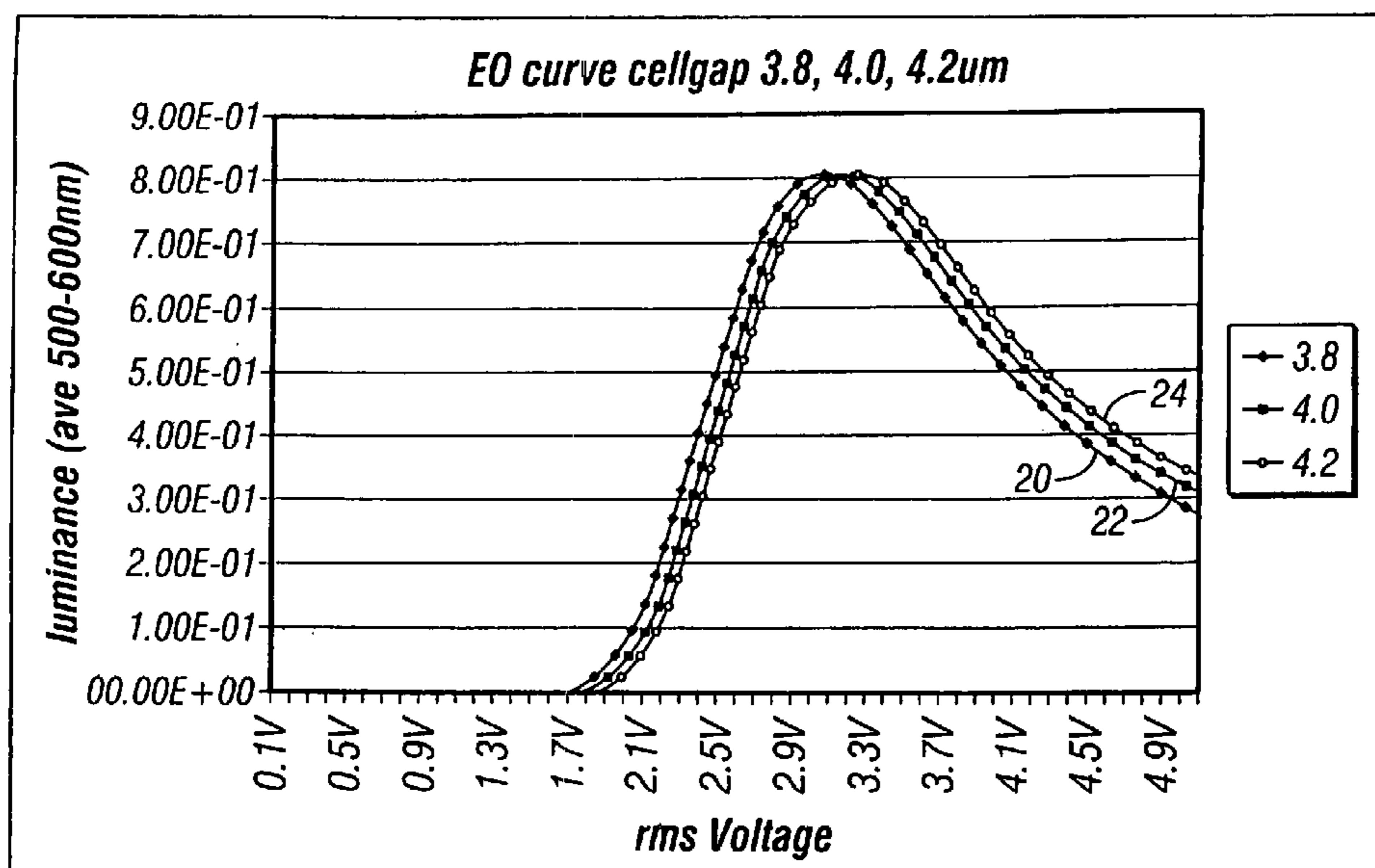
EO curves with 3.8, 4.0, 4.2um cellgaps
