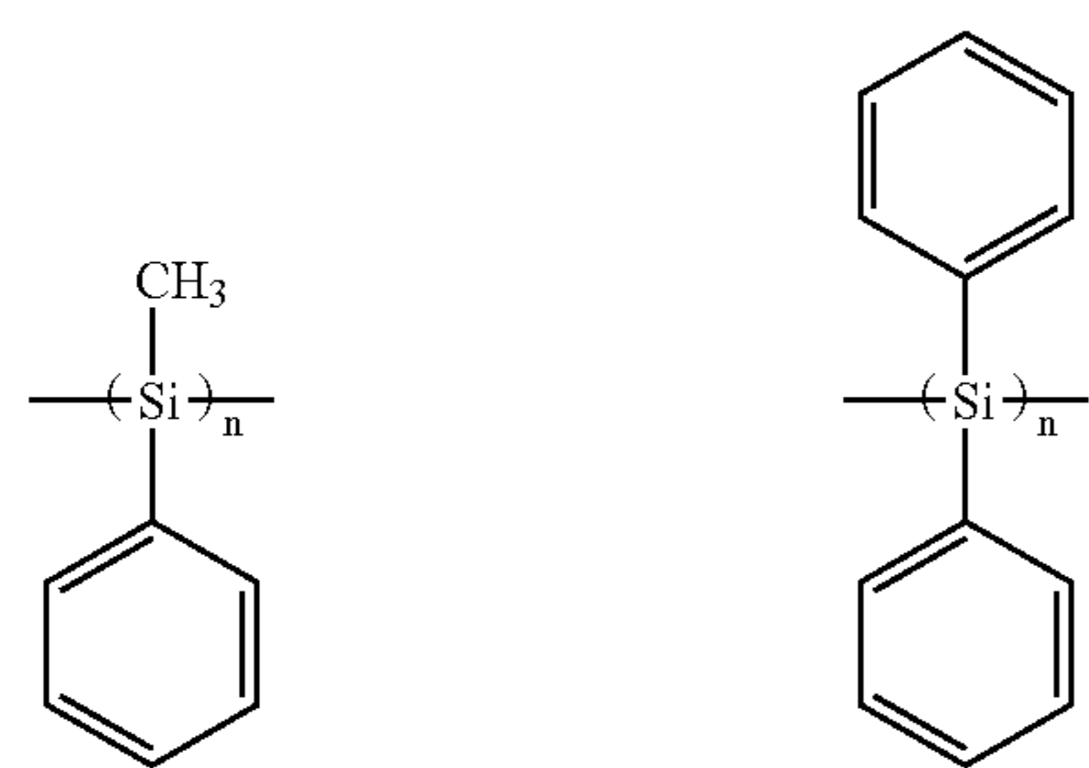
Polysilane
