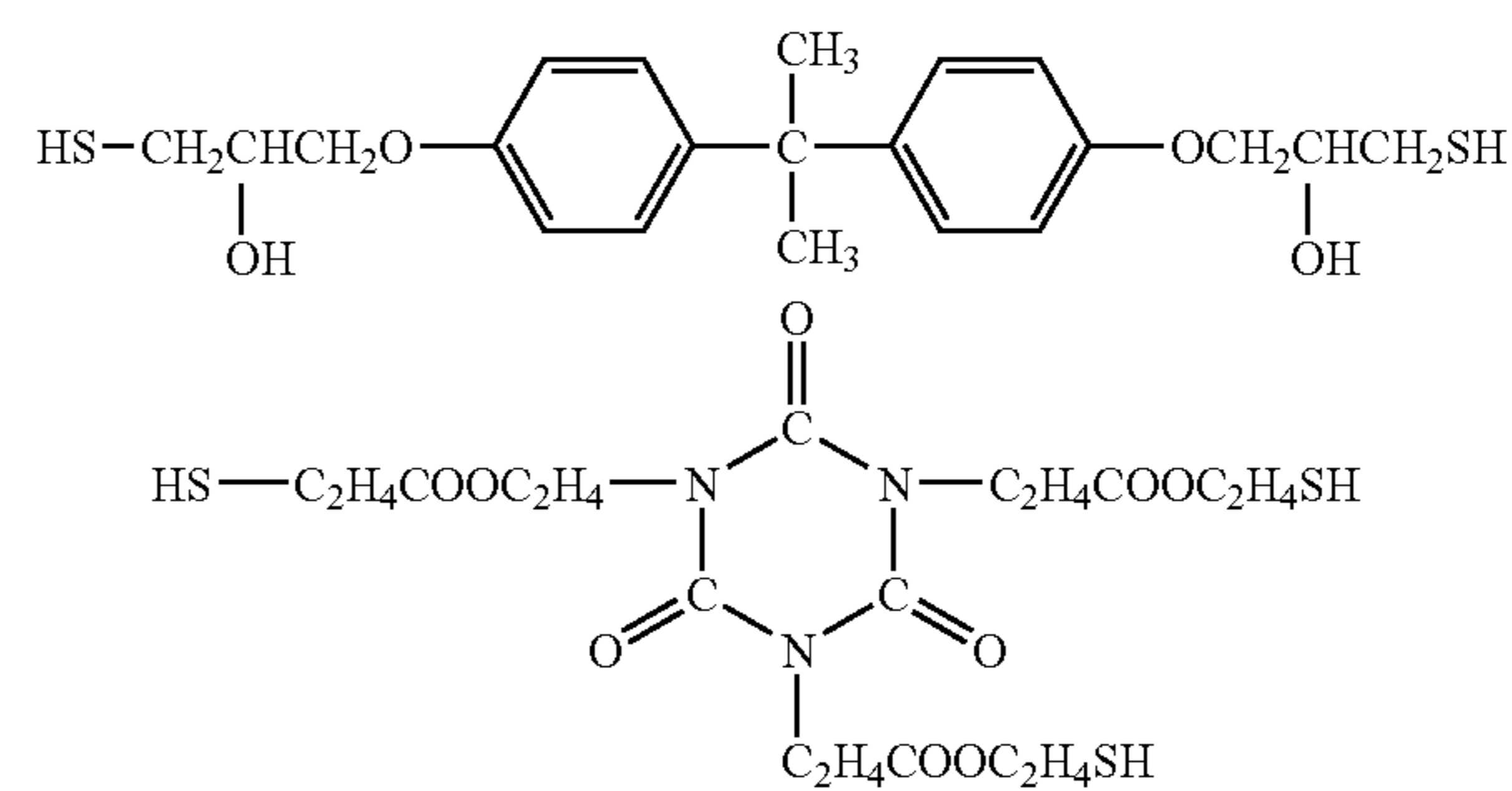
( \text{HSCH}_2\text{CH}_2\text{COOCH}_2 ) 3 CC 2 H 5 (TTMP)
