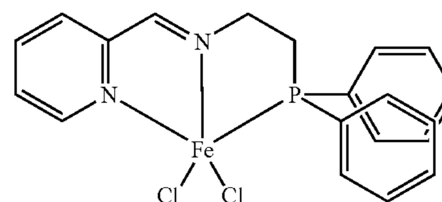
Structure XX
