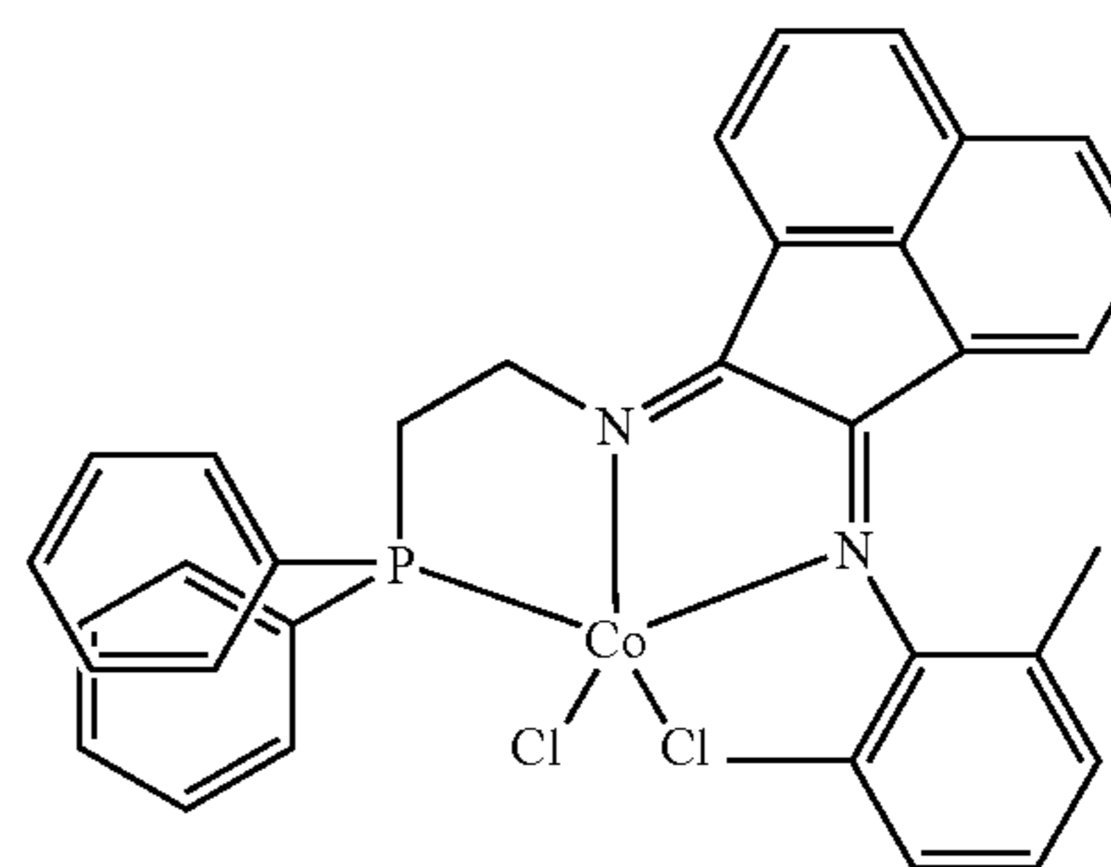
Structure XXI
