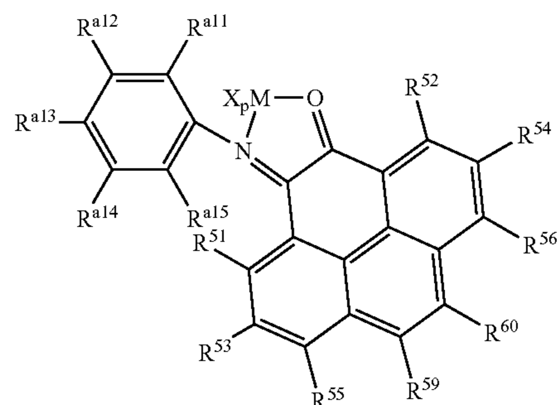
Structure 39d
