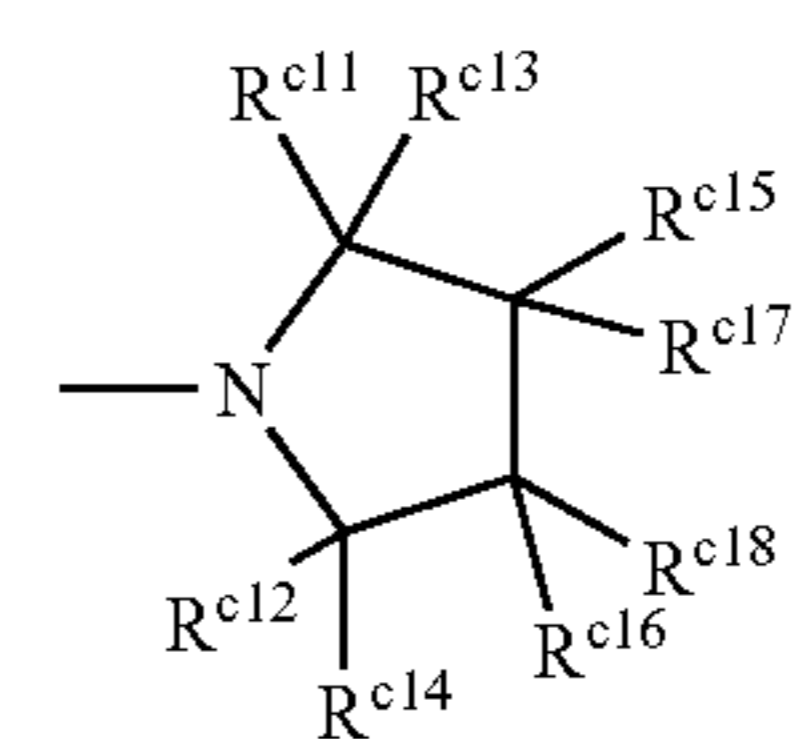
Structure 5c
