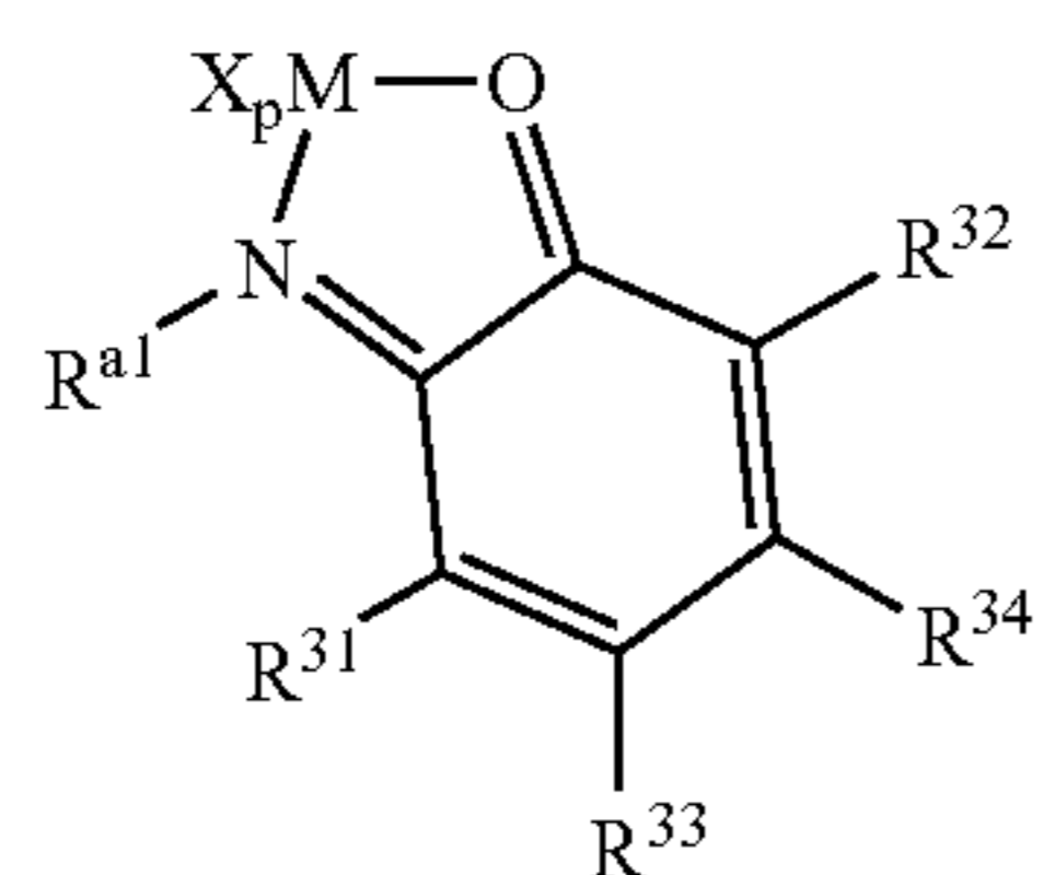
Structure 7d
