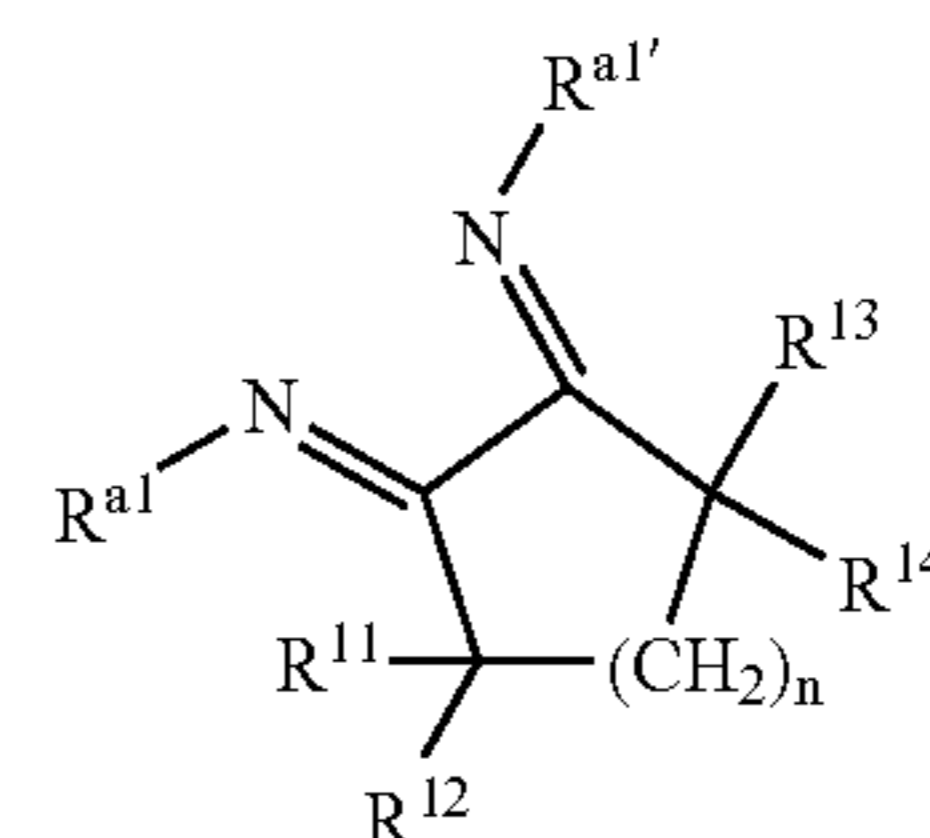
Structure 2f
