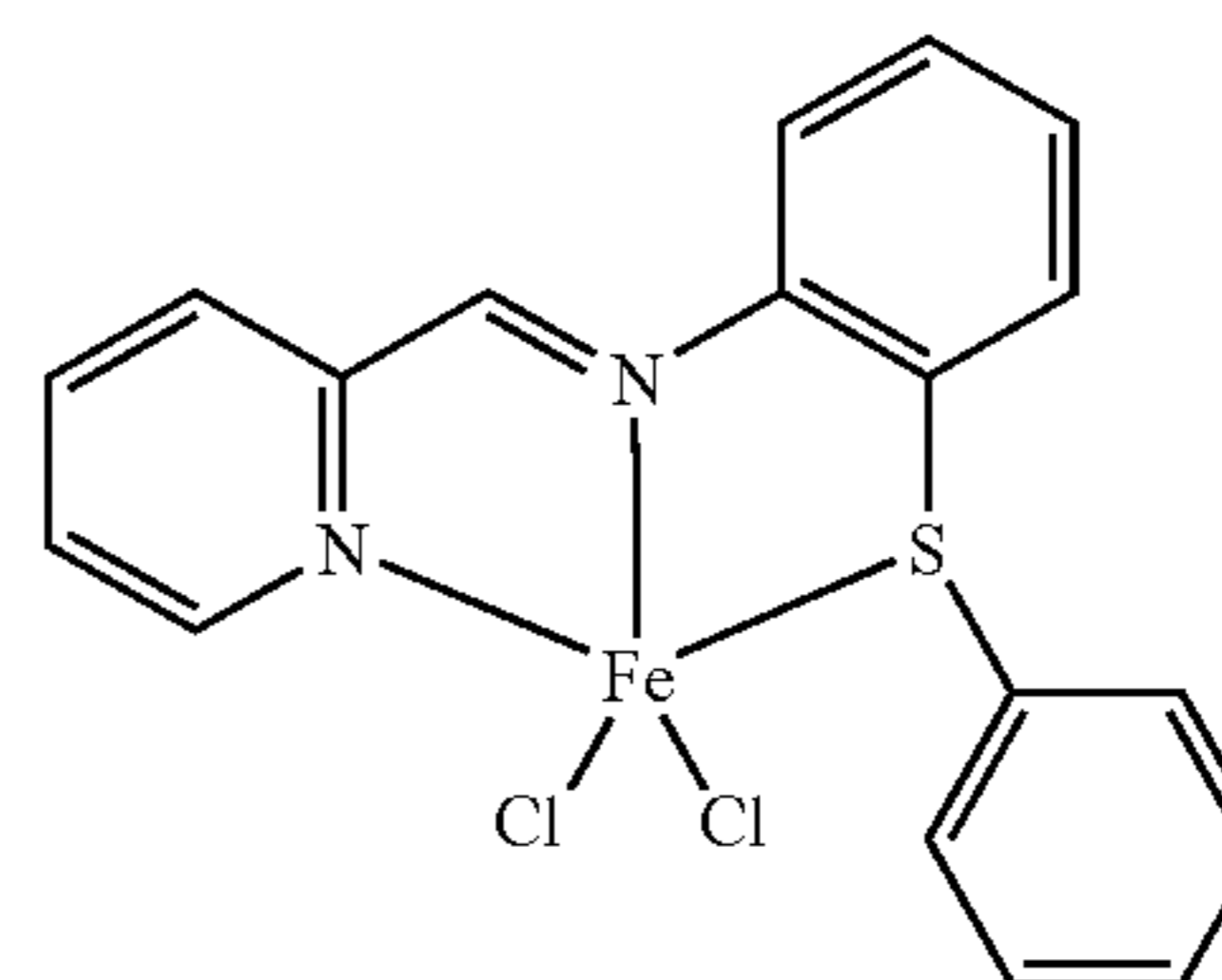
Structure XVIII
