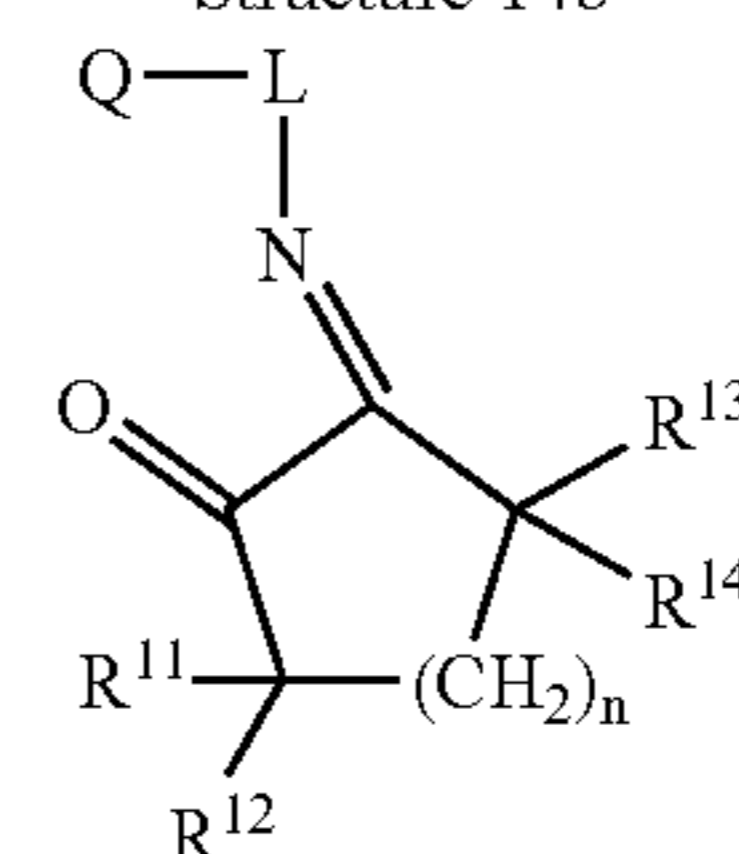
Structure 15b
