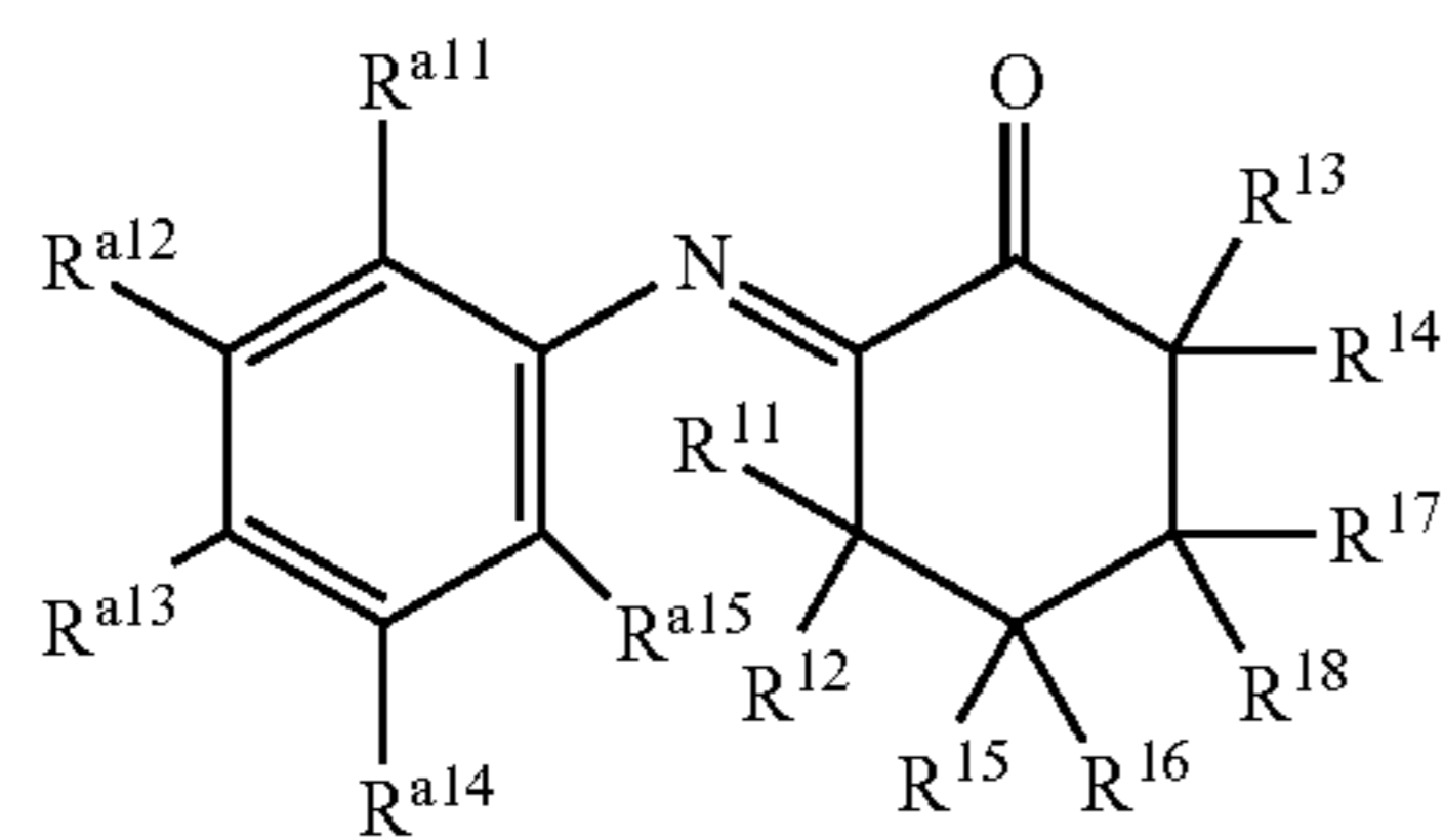
Structure 31b
