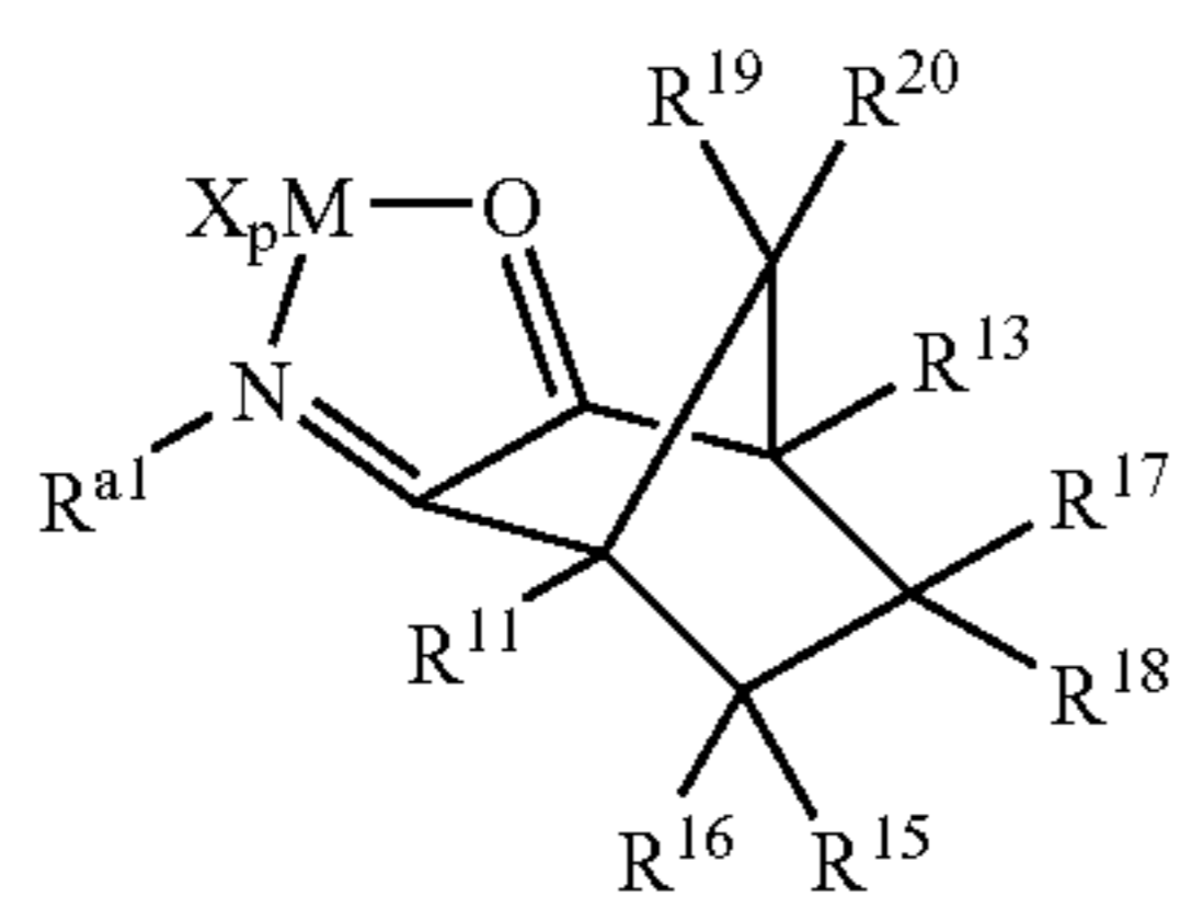
Structure 6d
