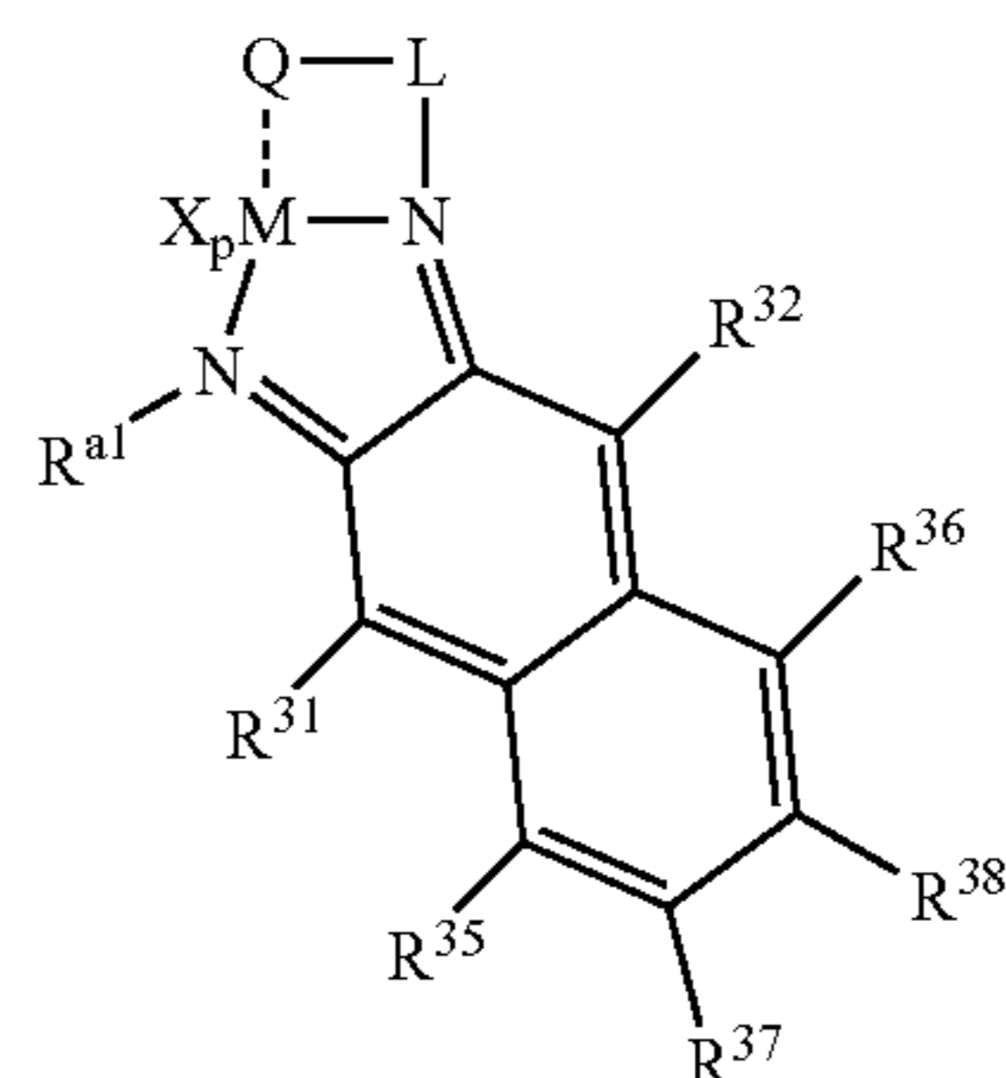
Structure 21e
