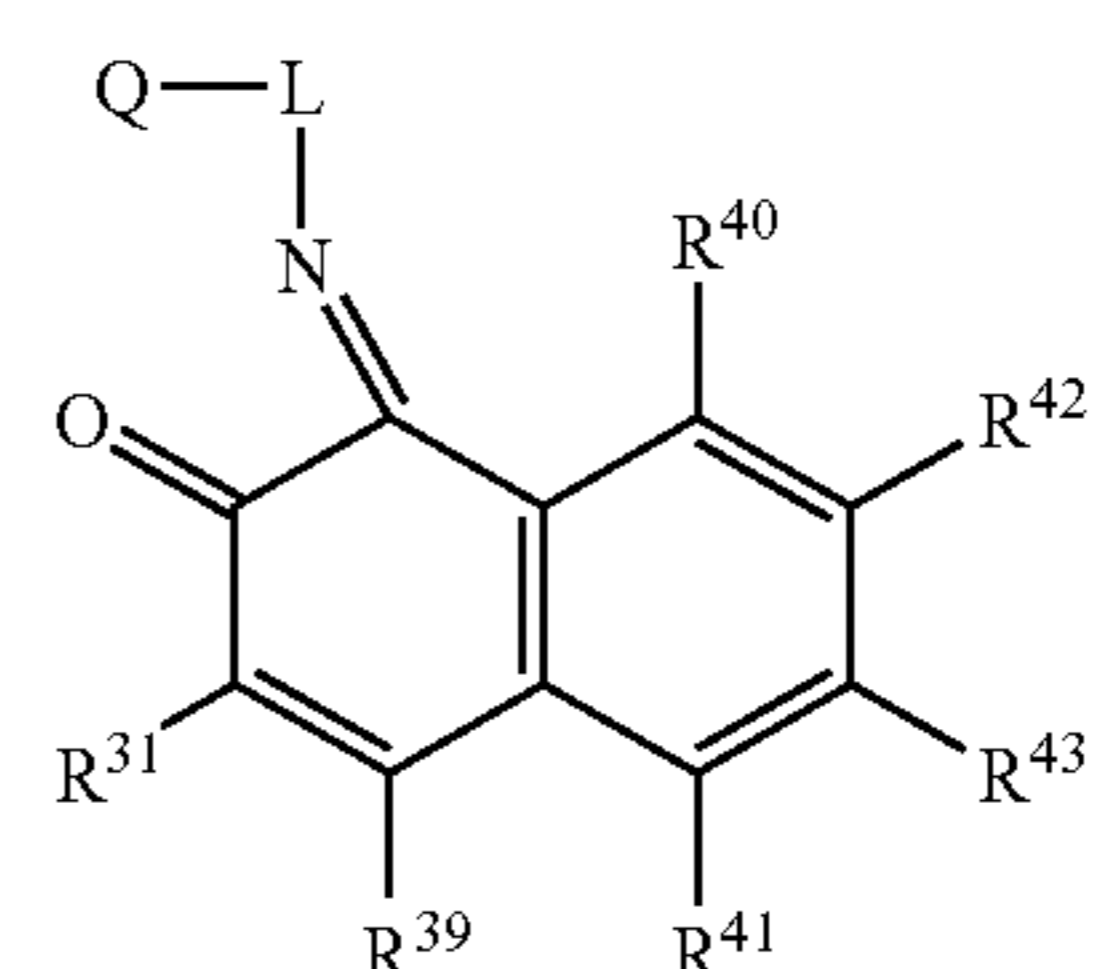
Structure 22b
