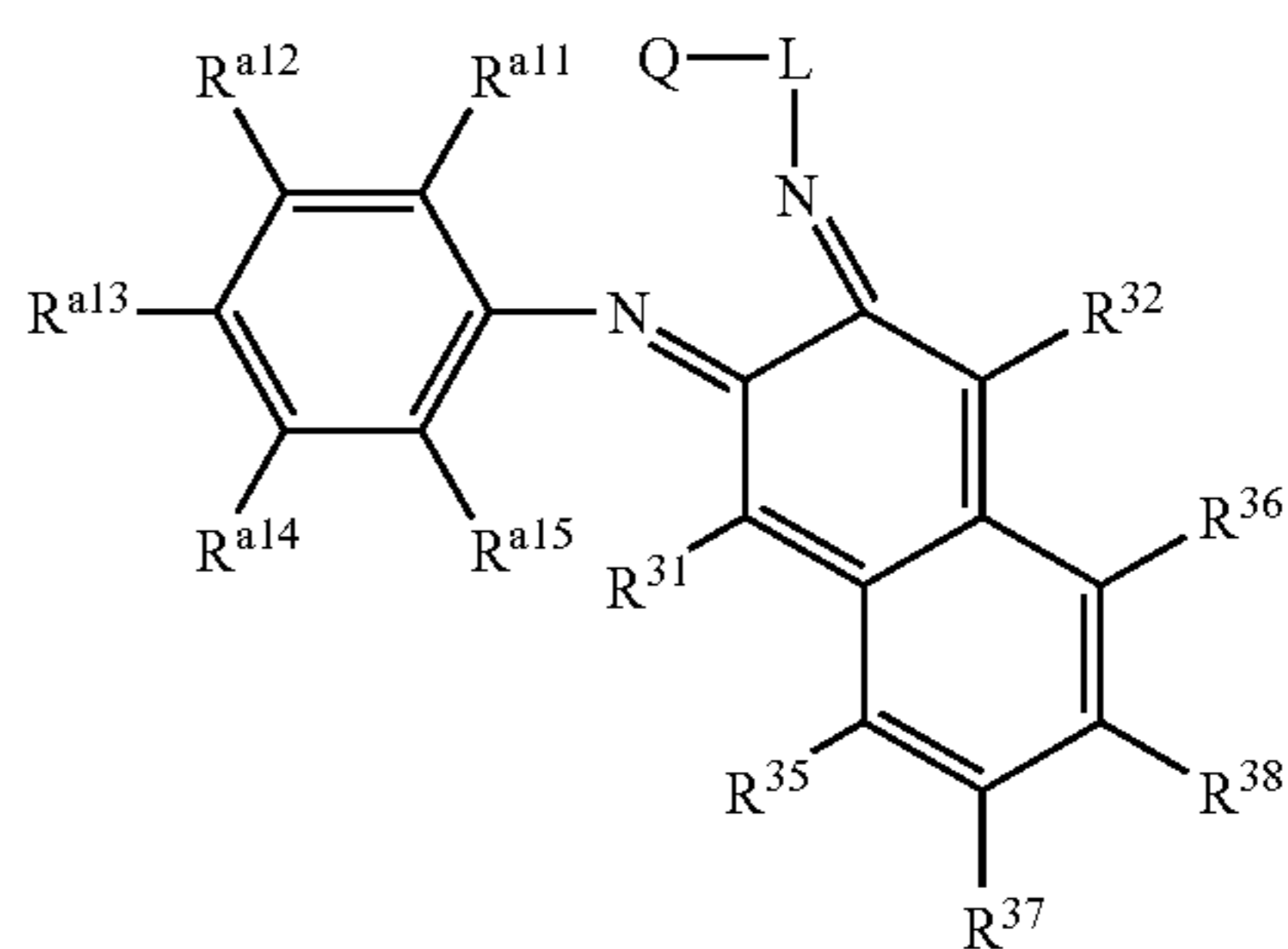
Structure 34f
