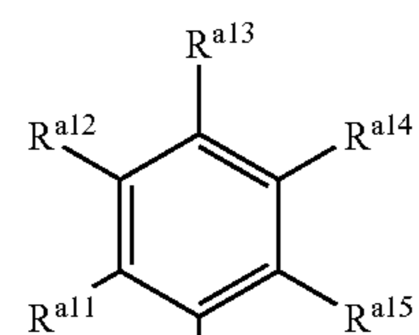
Structure 35b
