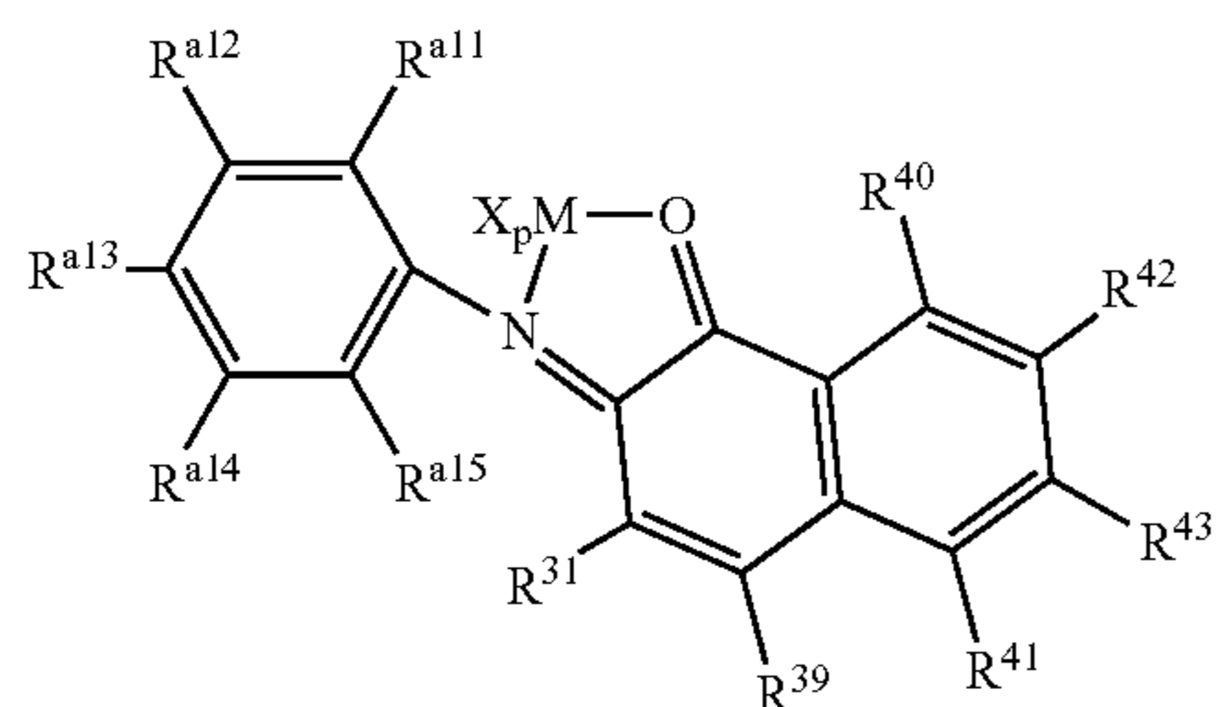
Structure 35d
