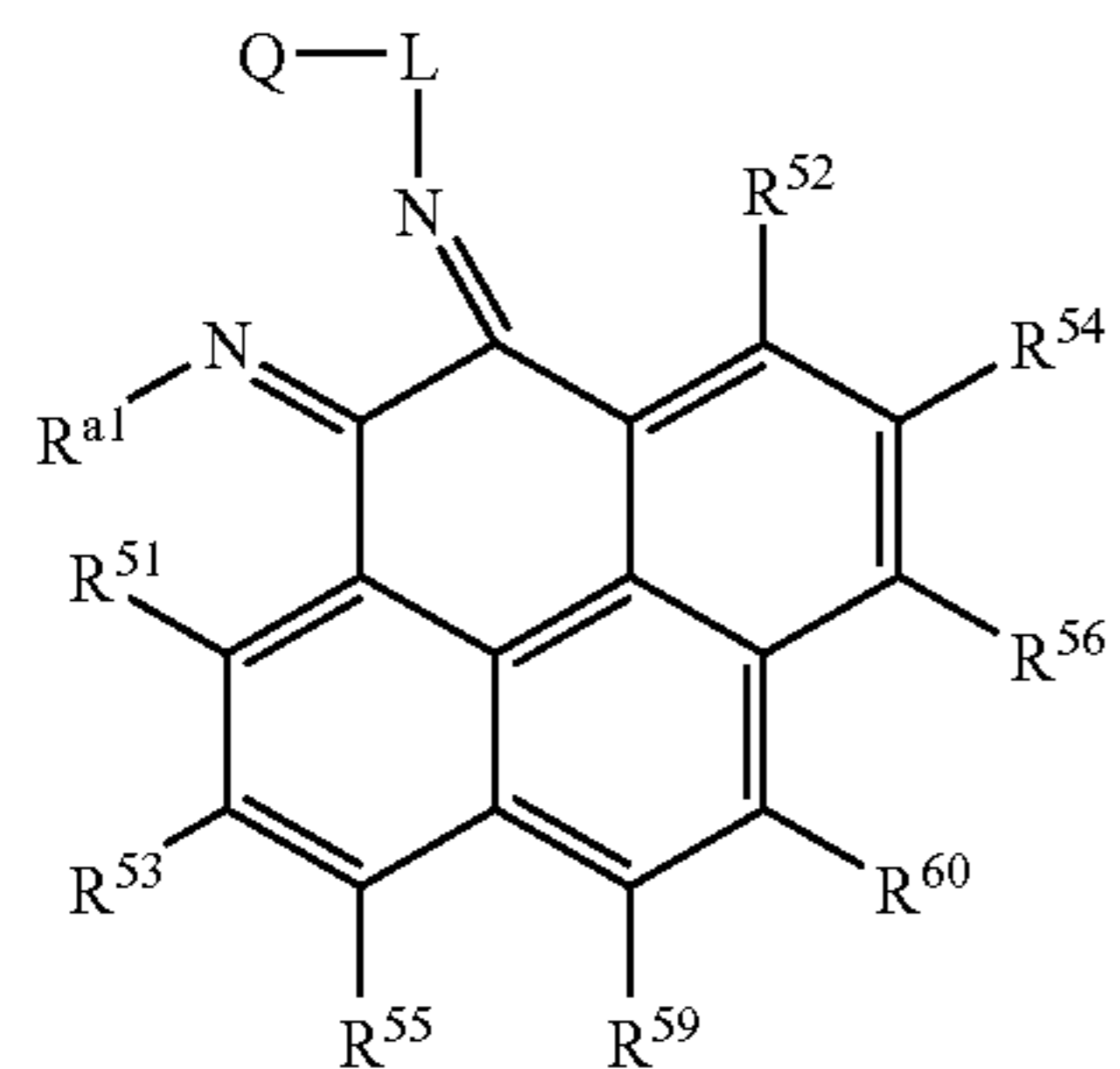
Structure 26f
