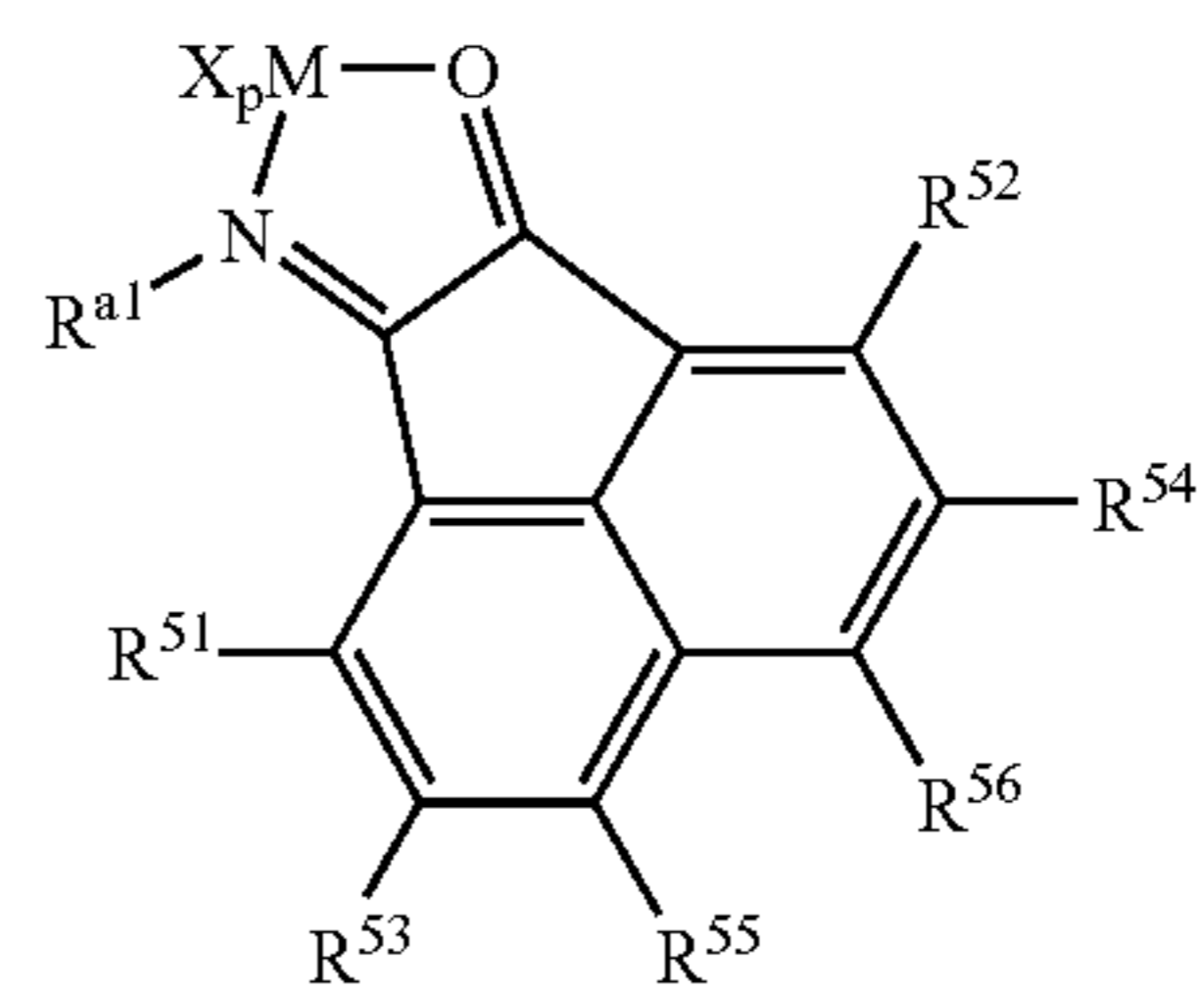
Structure 11d
