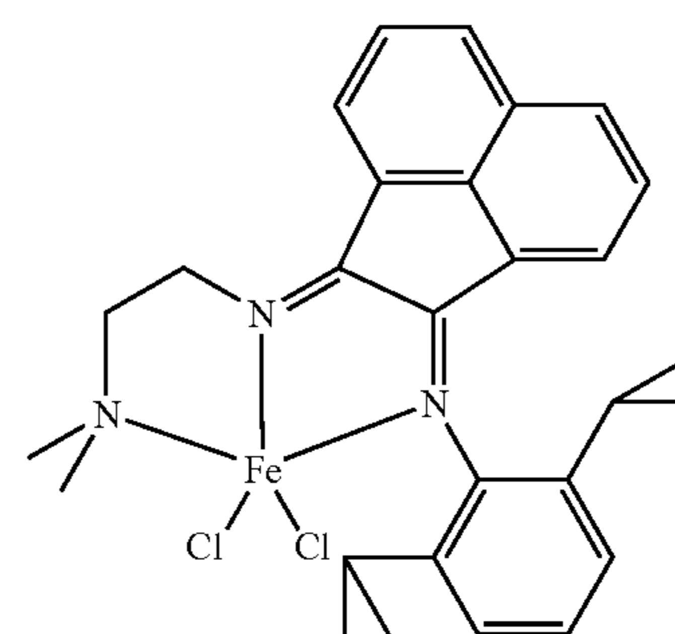
Structure XI
