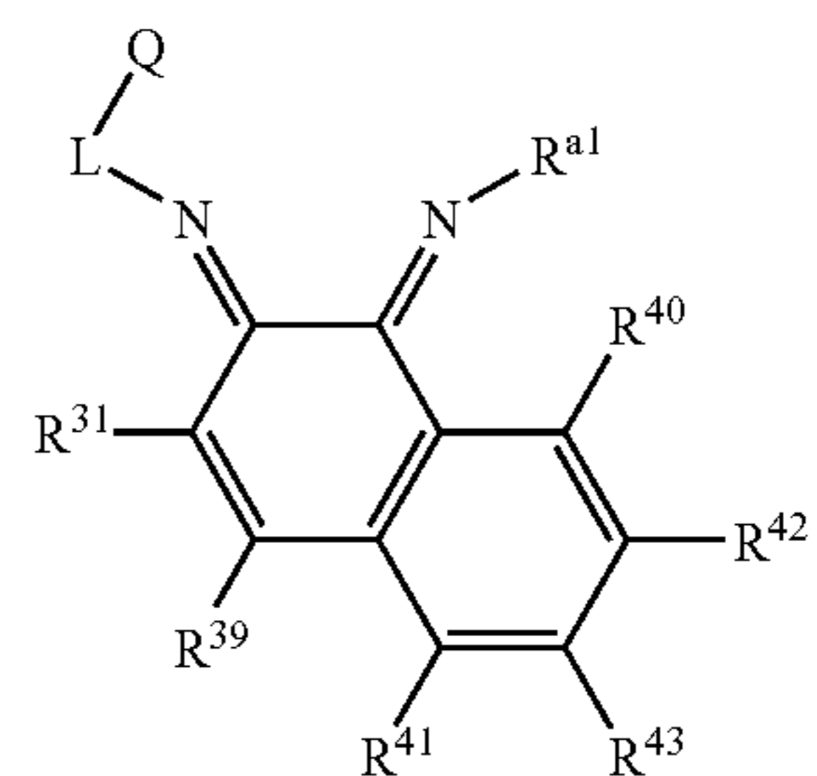
Structure 23f
