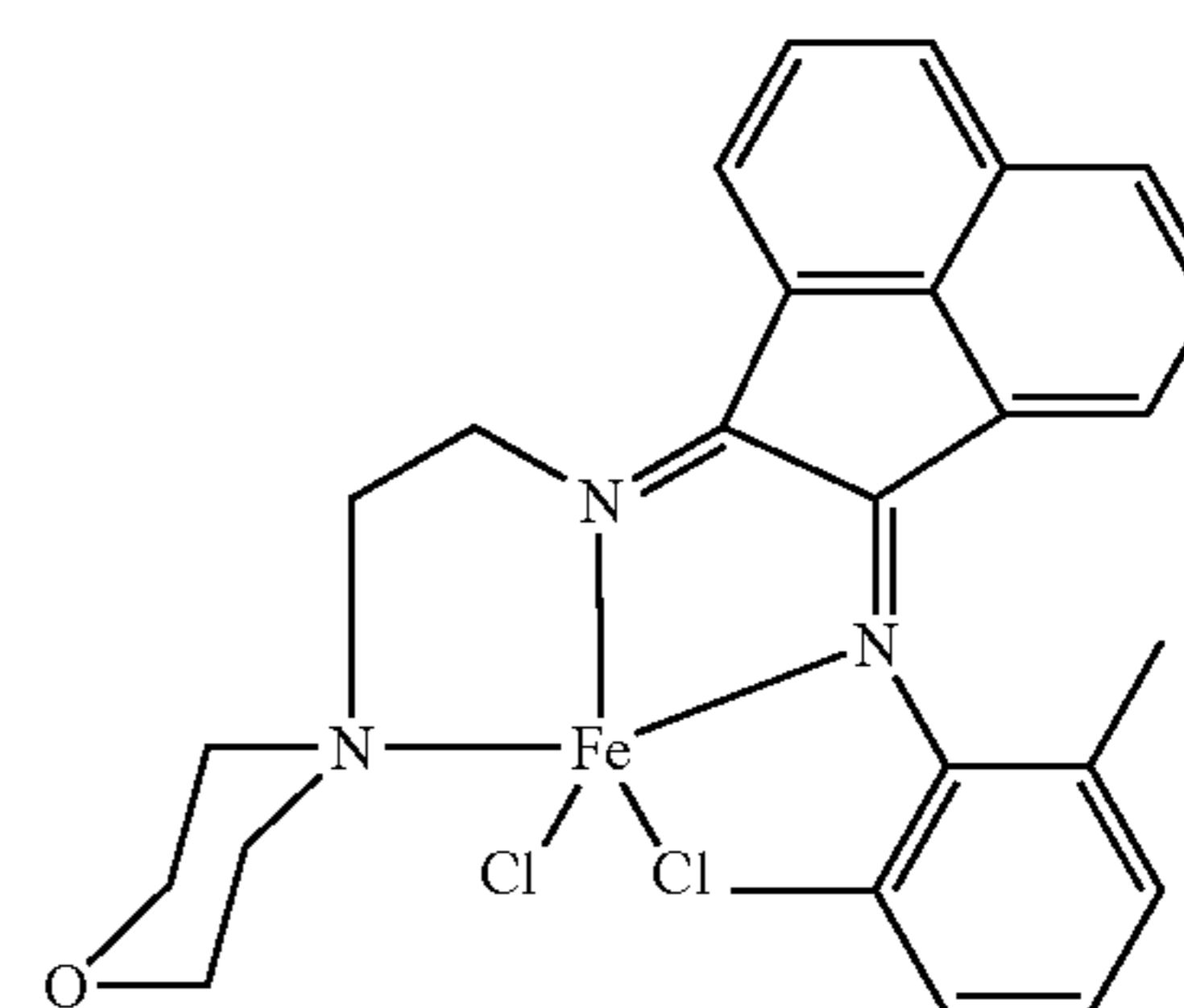
Structure IX
