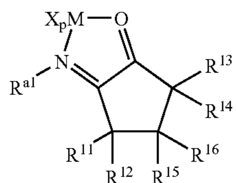
Structure 4d
