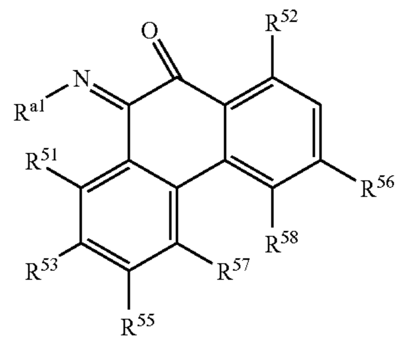
Structure 12b
