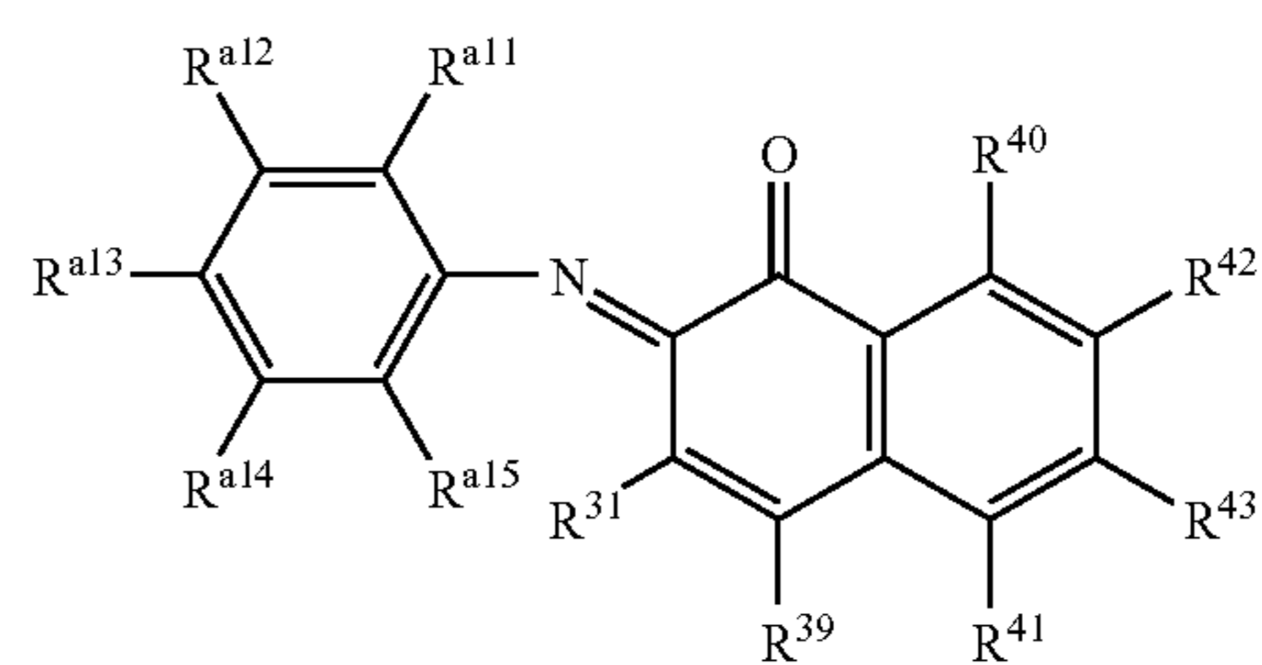
Structure 35b
