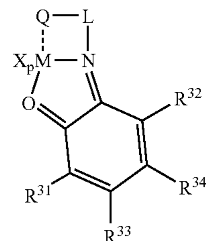
Structure 20d
