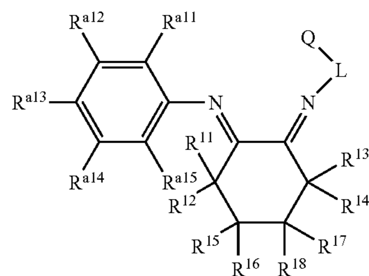
Structure 31f
