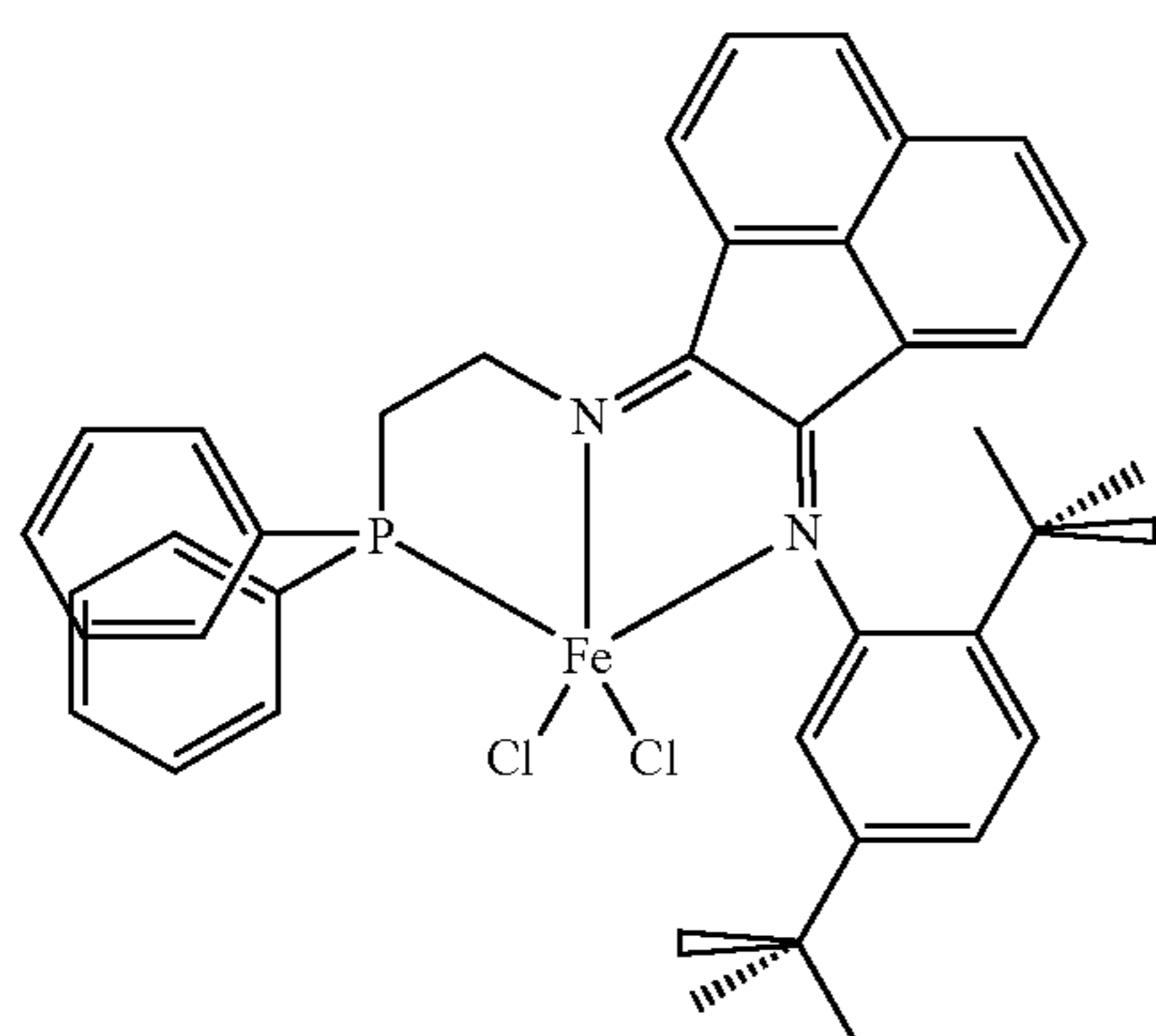
Structure VI
