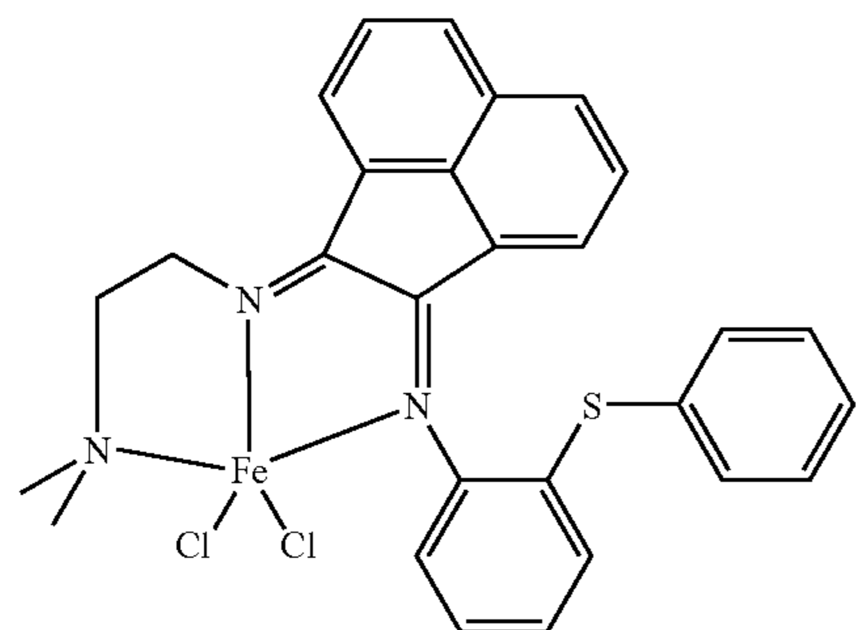
Structure XVI
