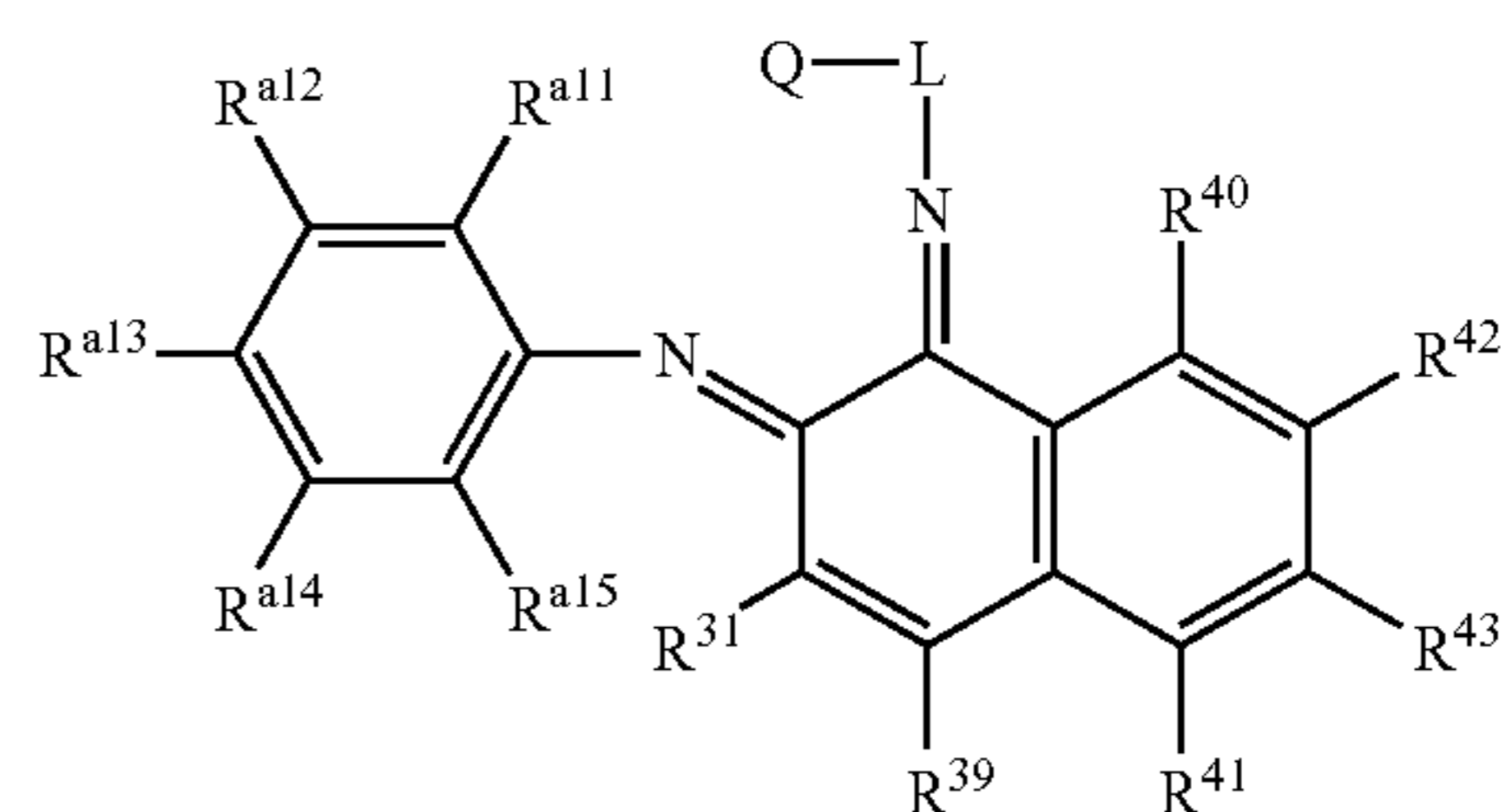
Structure 35f
