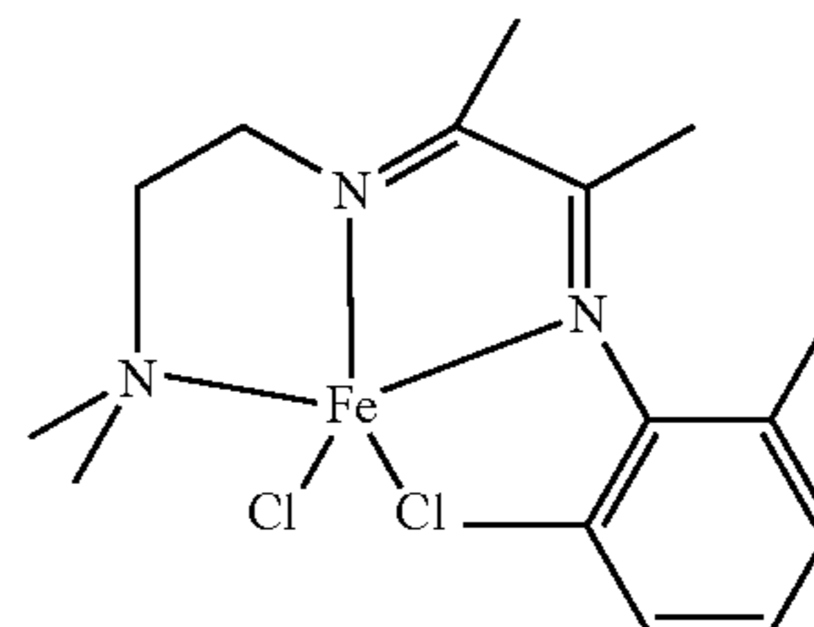
Structure XVII
