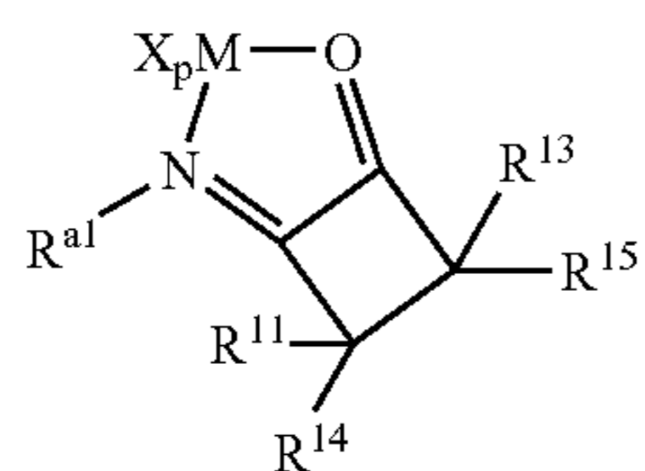
Structure 3d
