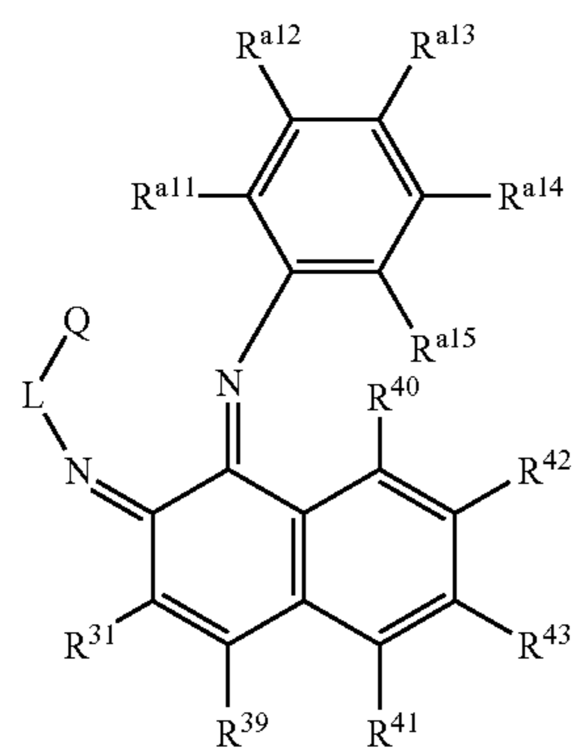
Structure 36f
