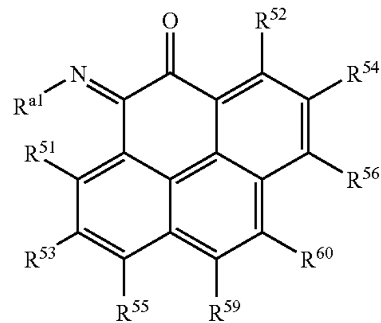
Structure 13b
