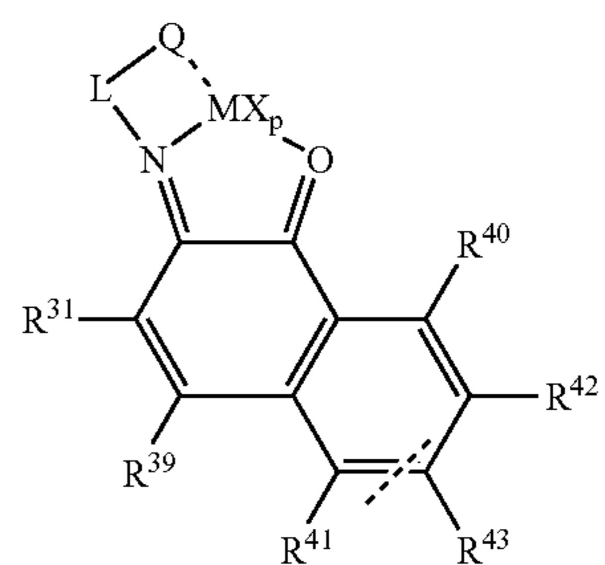
Structure 23d
