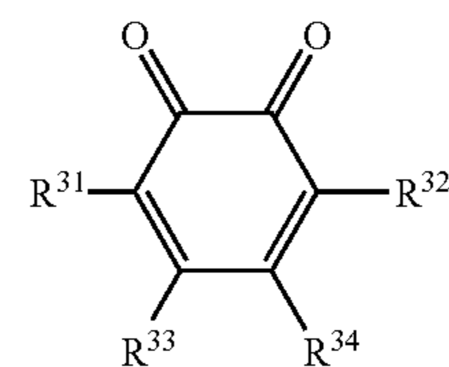
Structure 7
