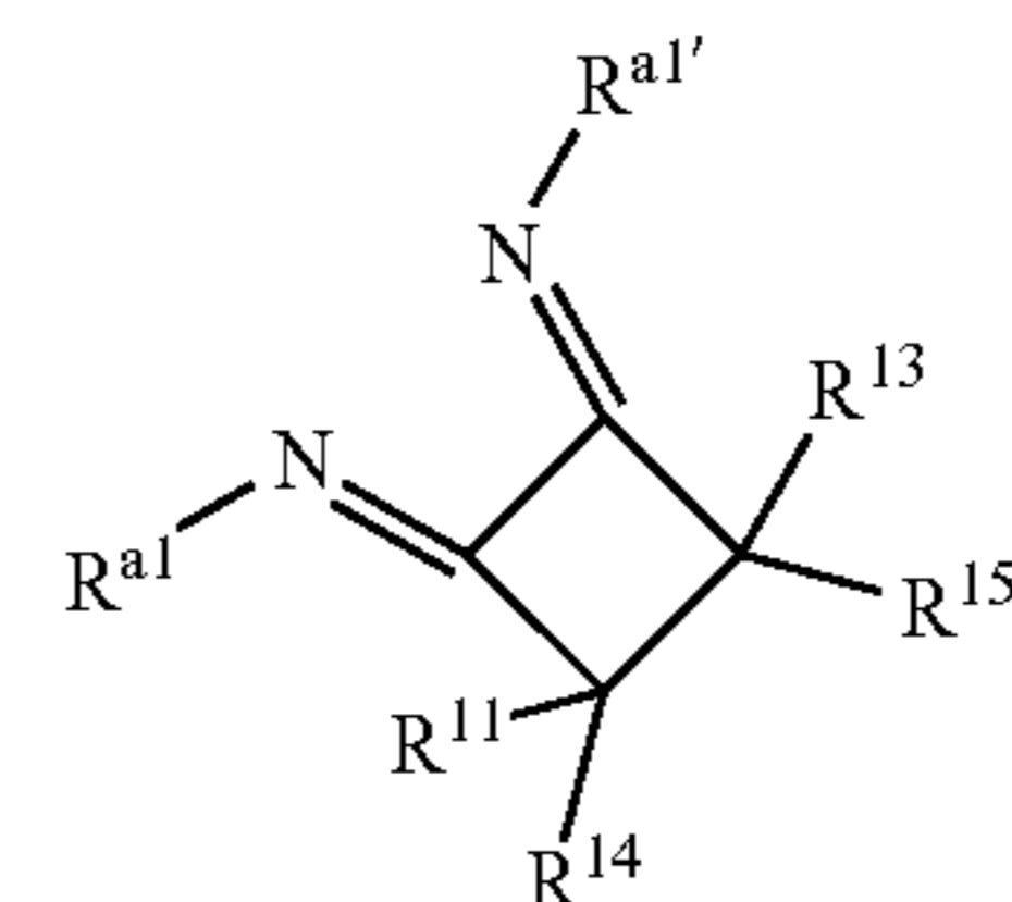
Structure 3f
