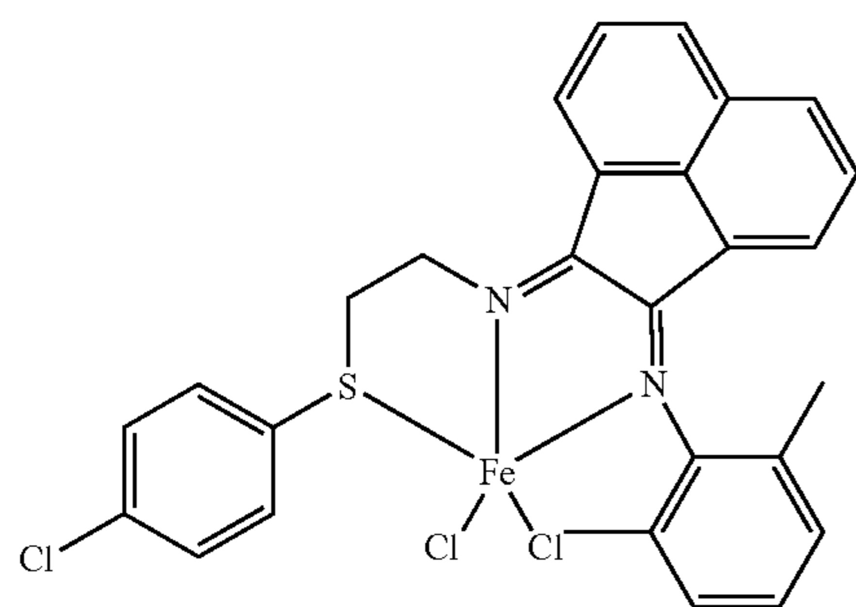
Structure V
