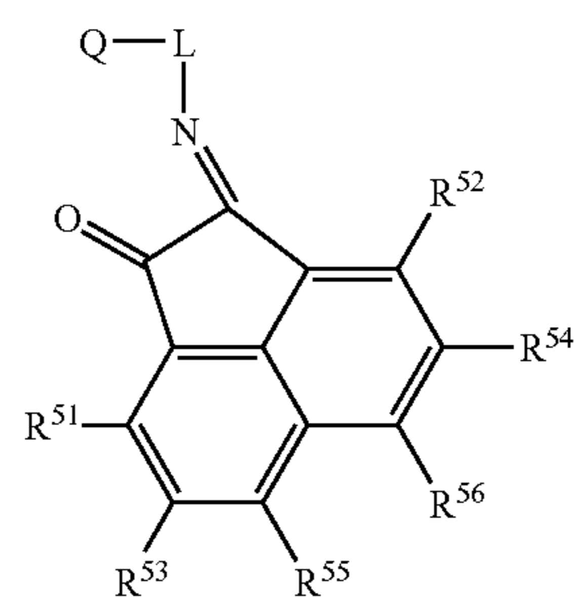
Structure 24b
