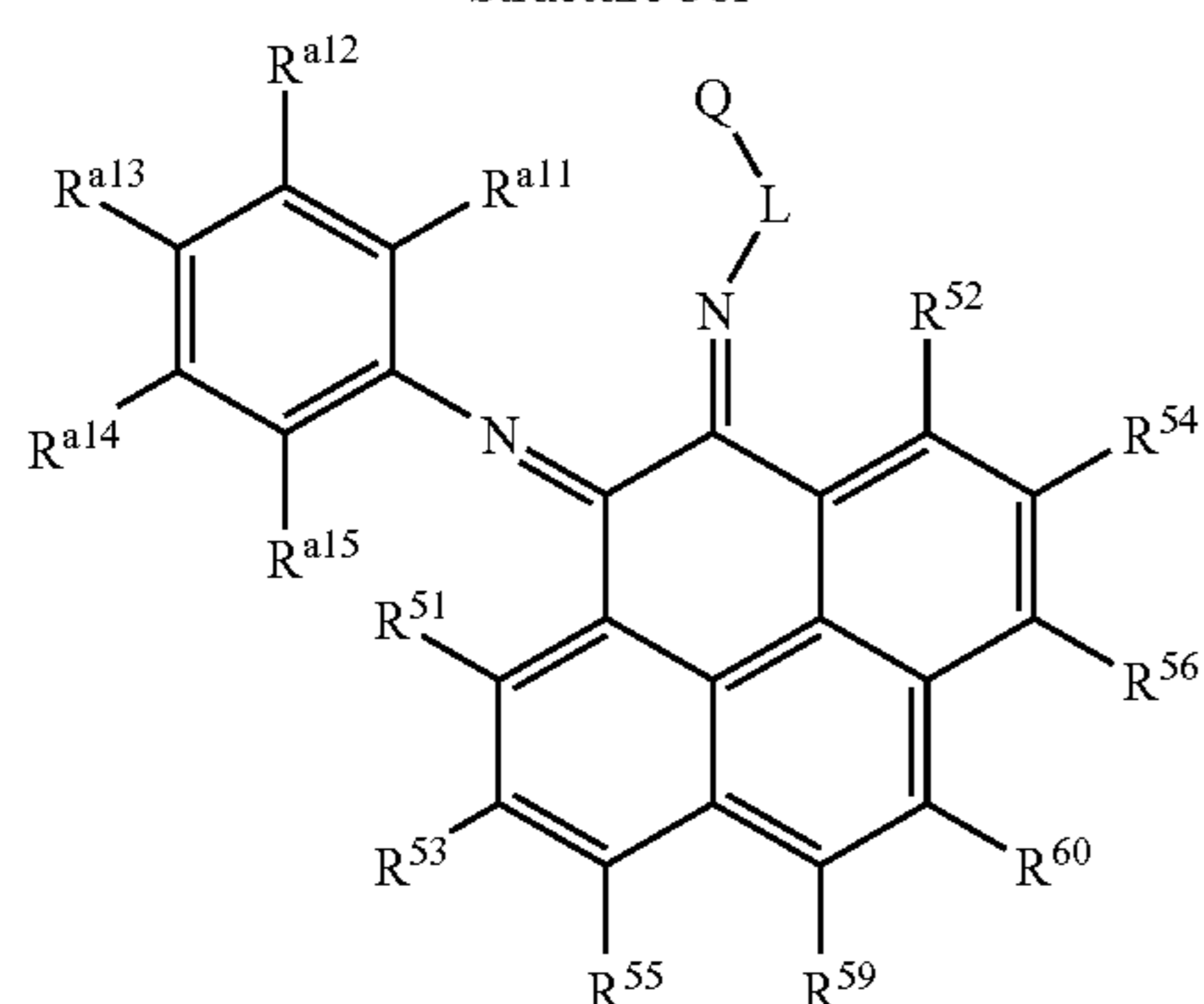
Structure 39f
