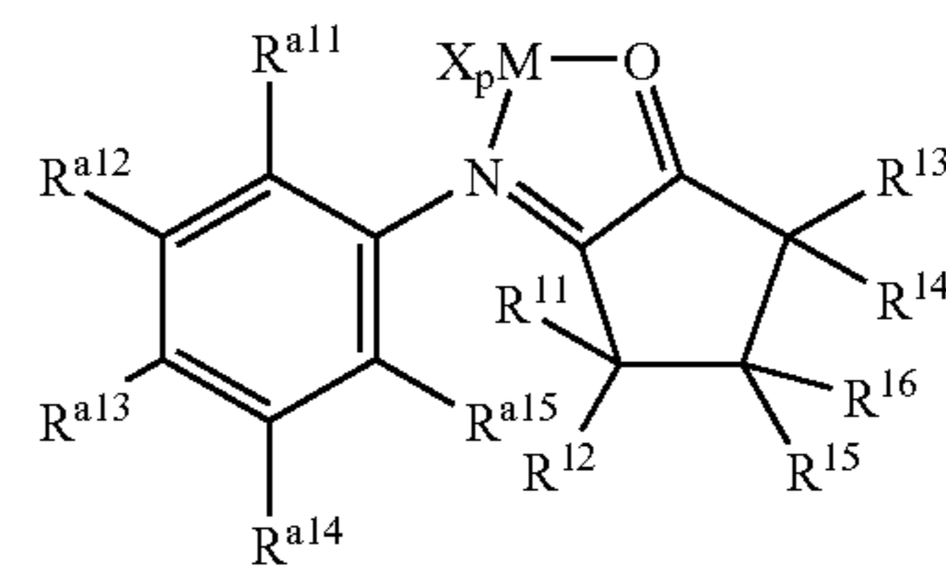
Structure 30d
