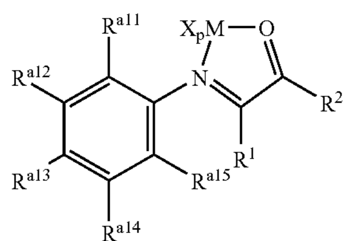
Structure 27d
