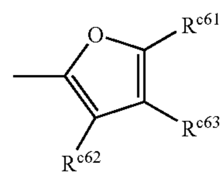
Structure 19c
