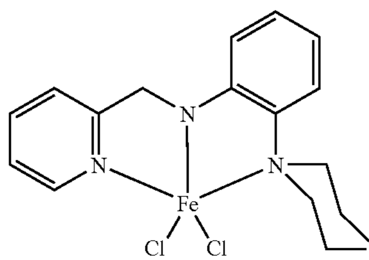
Structure XIX
