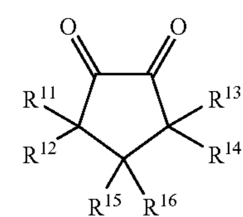
Structure 4
