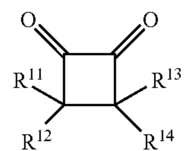
Structure 3
