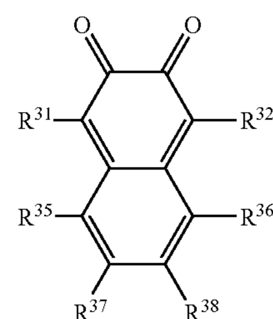
Structure 8
