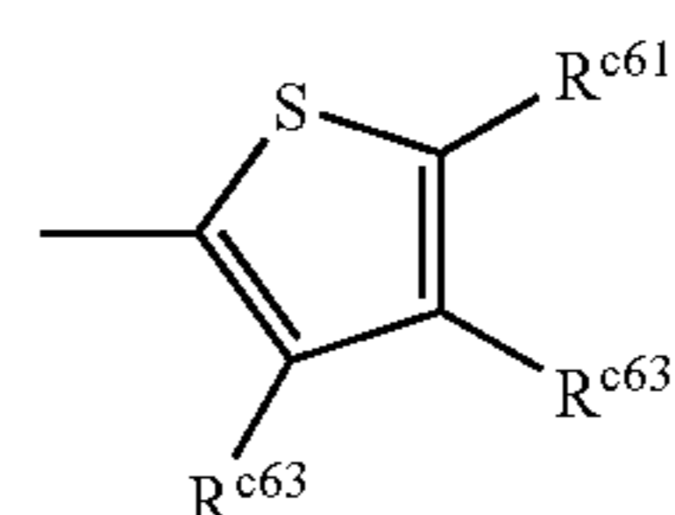
Structure 20c
