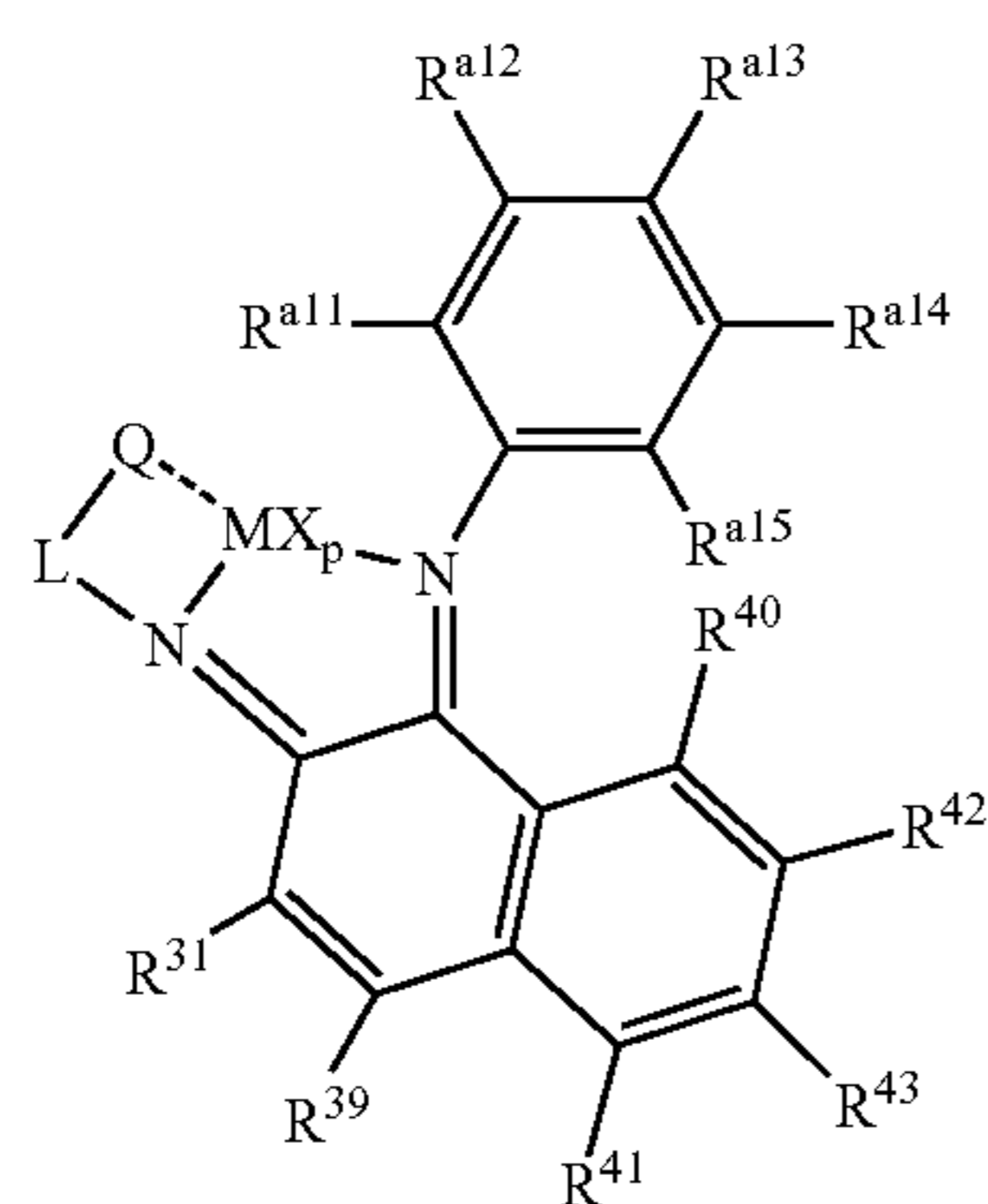
Structure 36e
