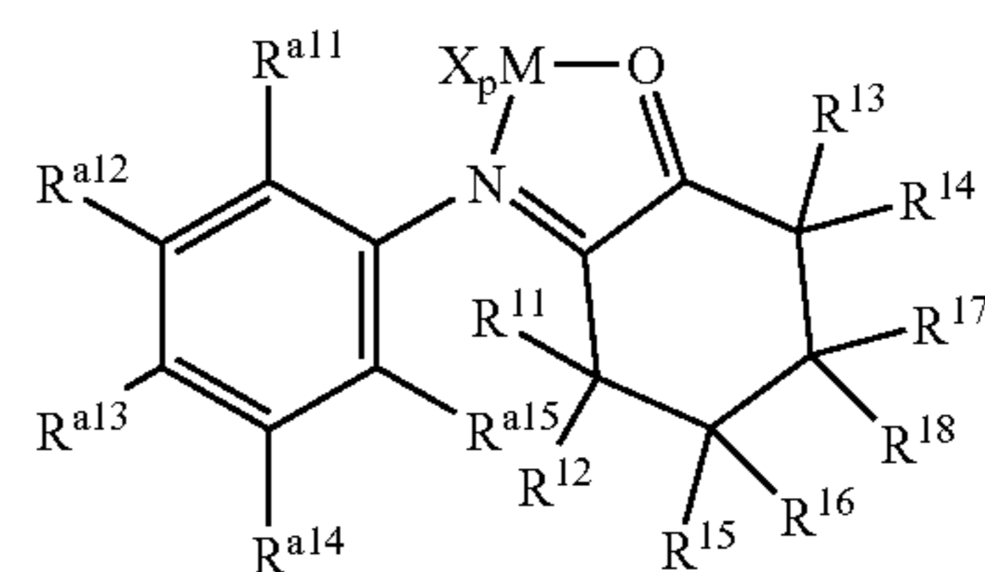
Structure 31d
