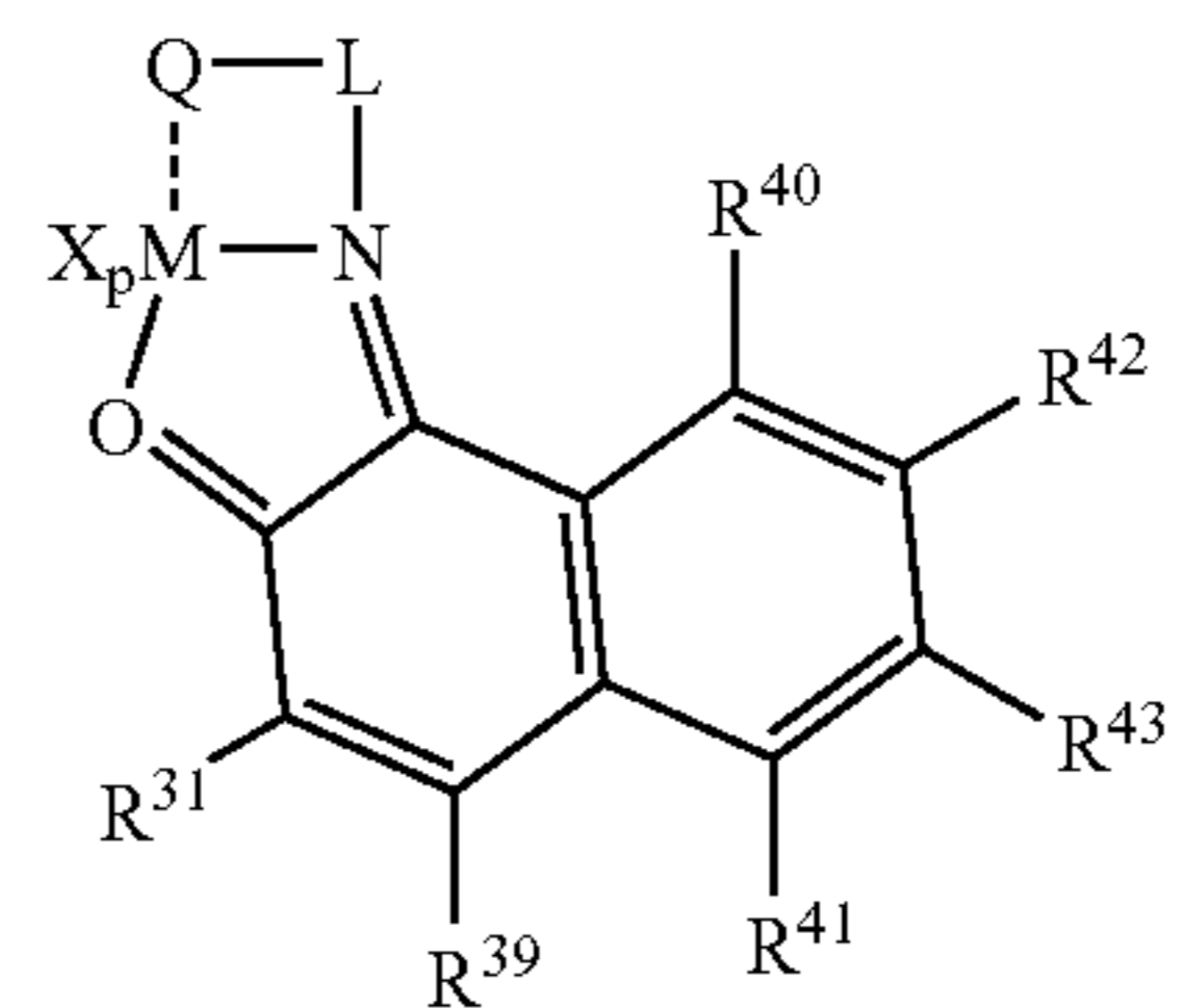
Structure 22d
