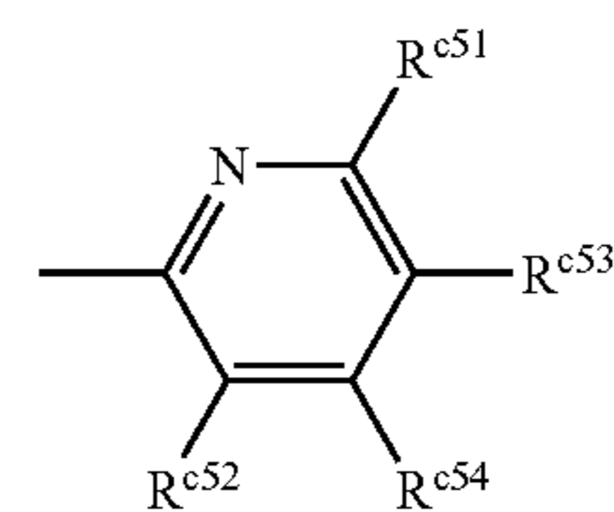
Structure 18c
