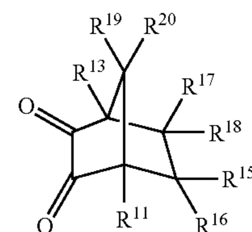
Structure 6
