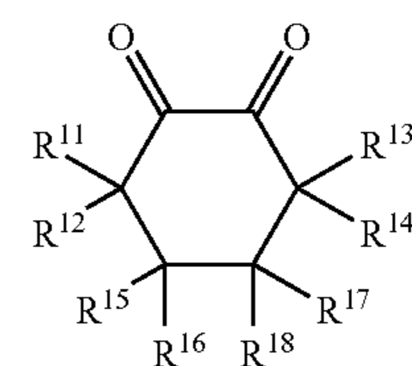
Structure 5
