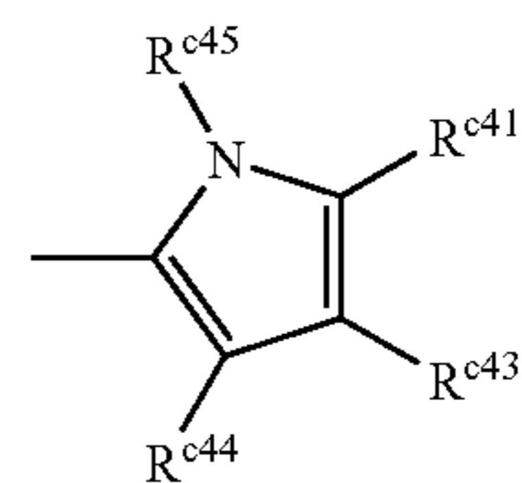
Structure 17c
