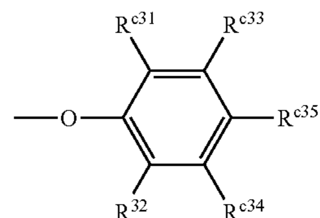
Structure 14c
