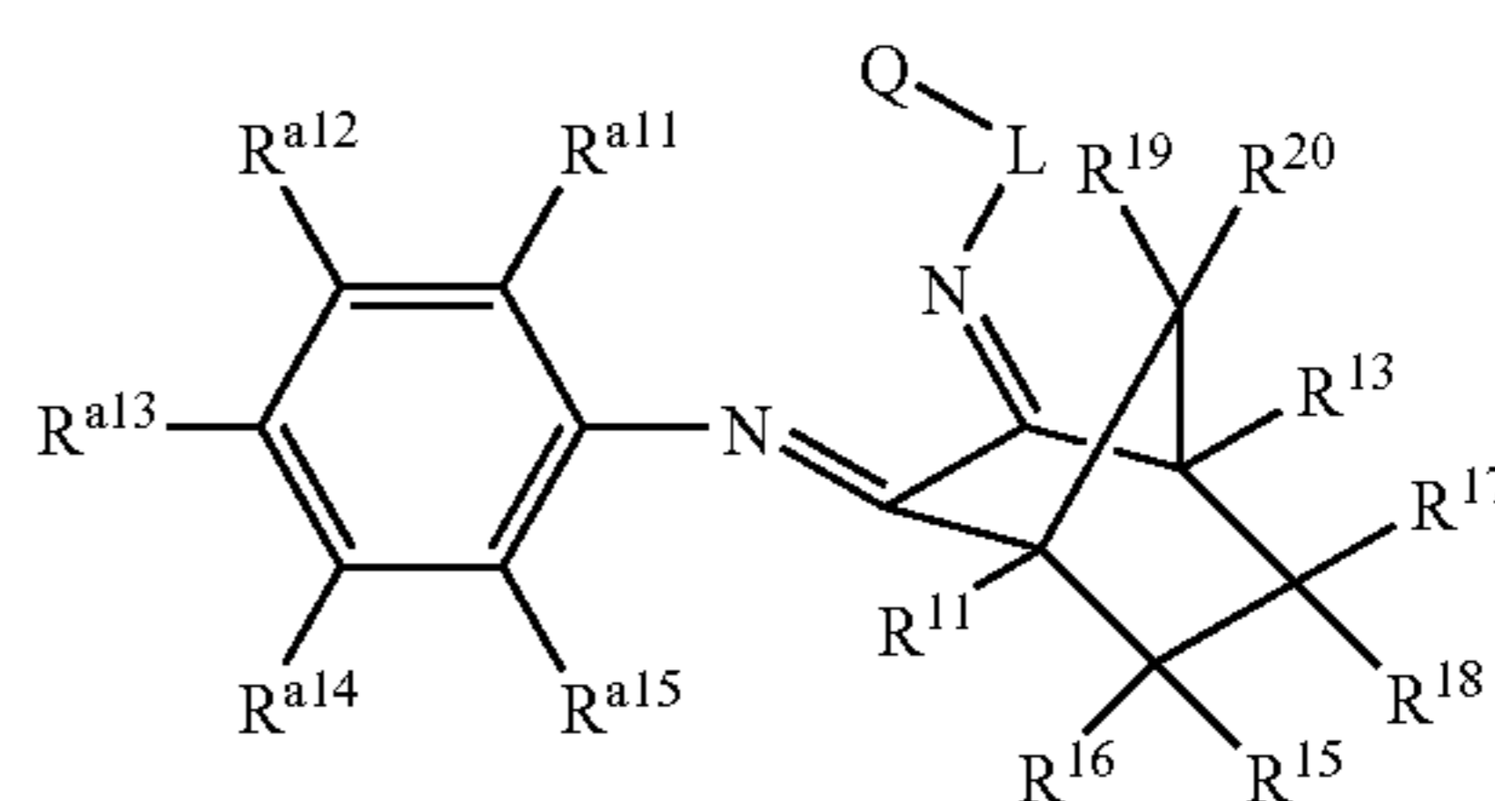
Structure 32f
