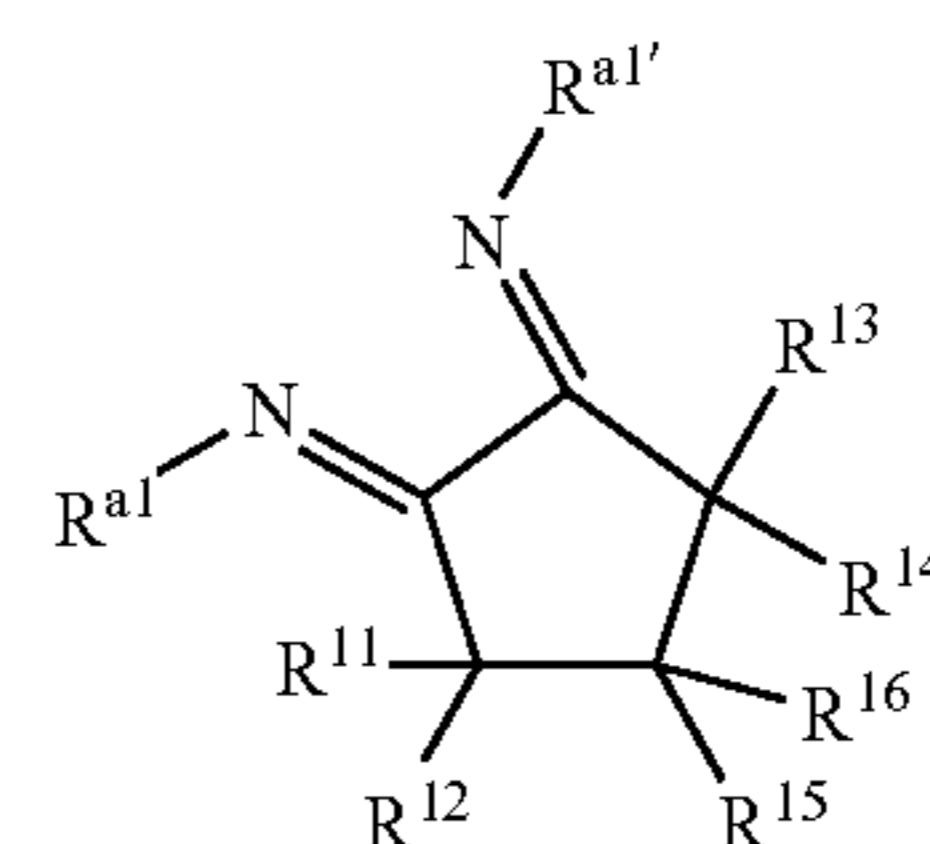
Structure 4f
