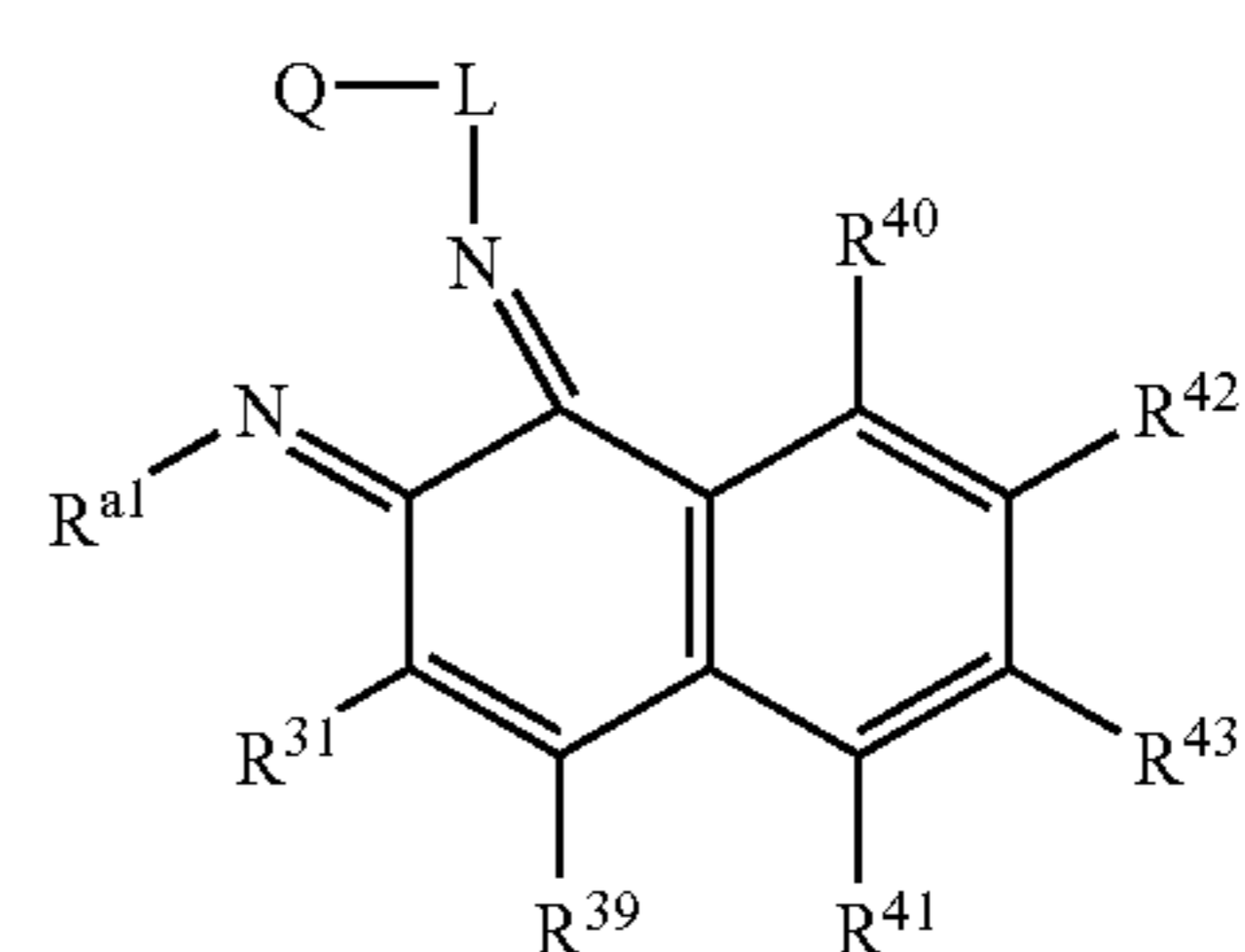
Structure 22f
