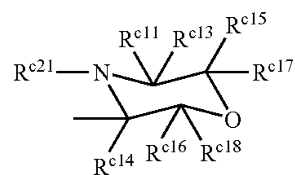
Structure 10c
