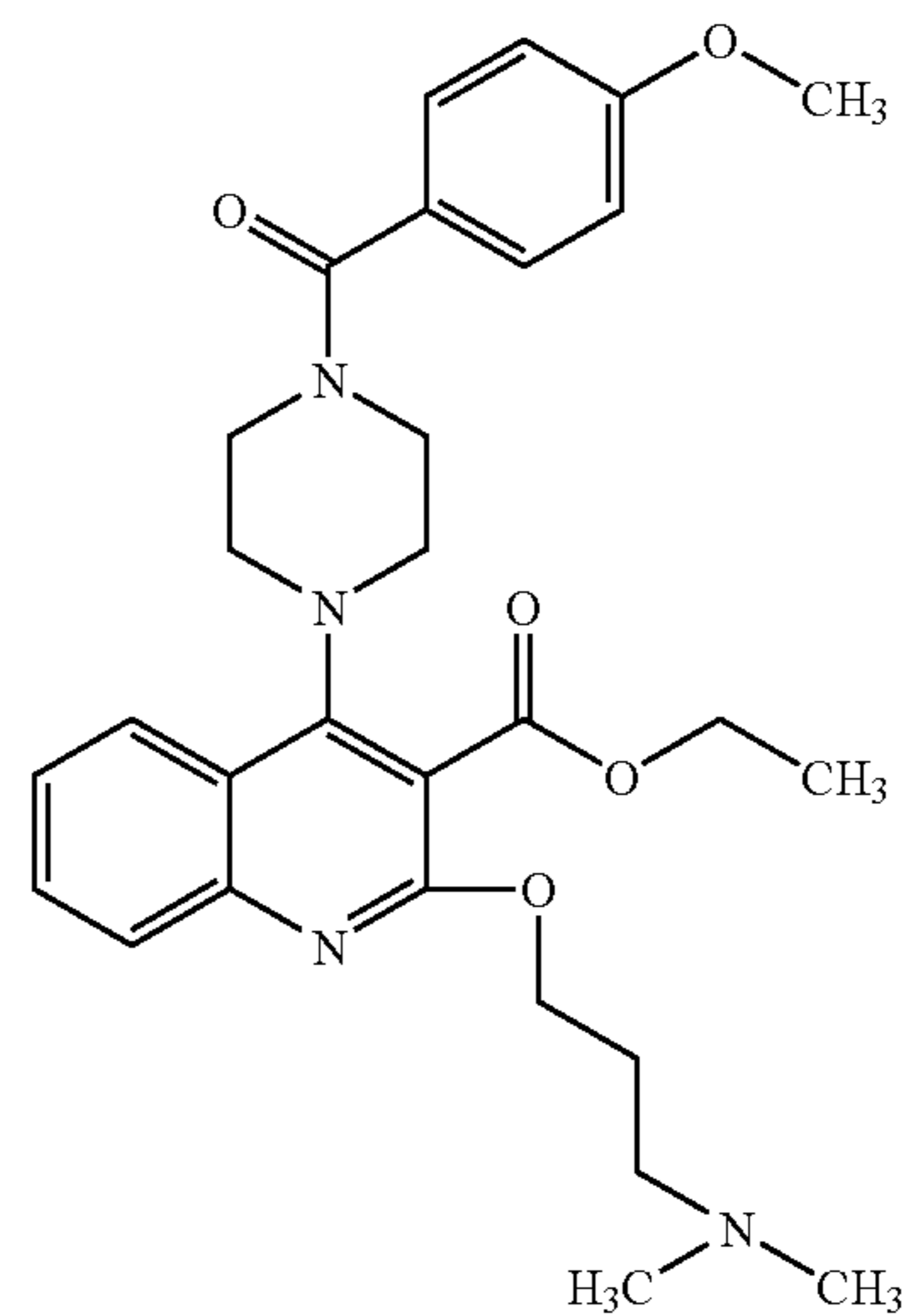
Compound 329
