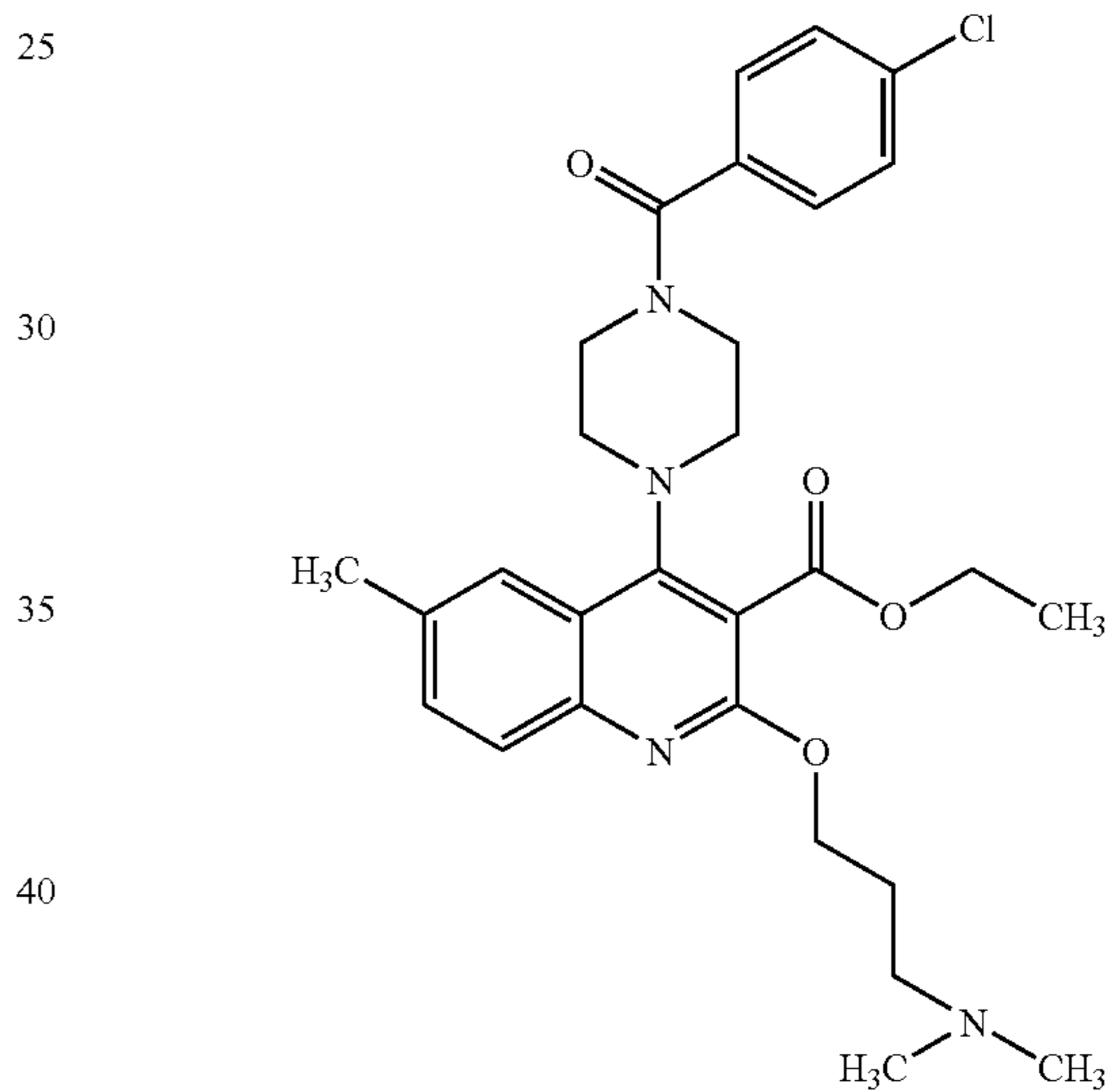
Compound 335
