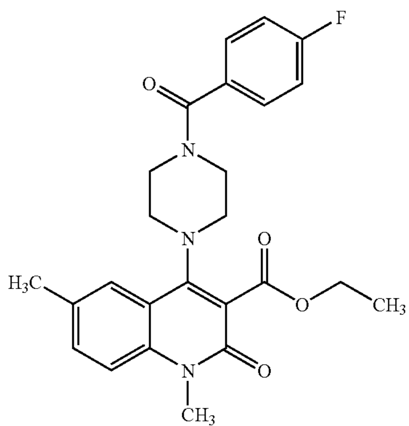
Compound 44
