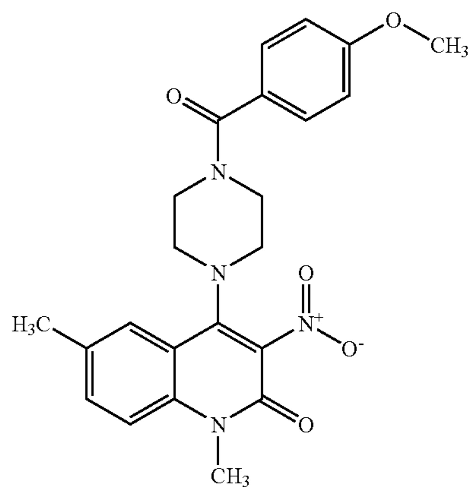
Compound 193
