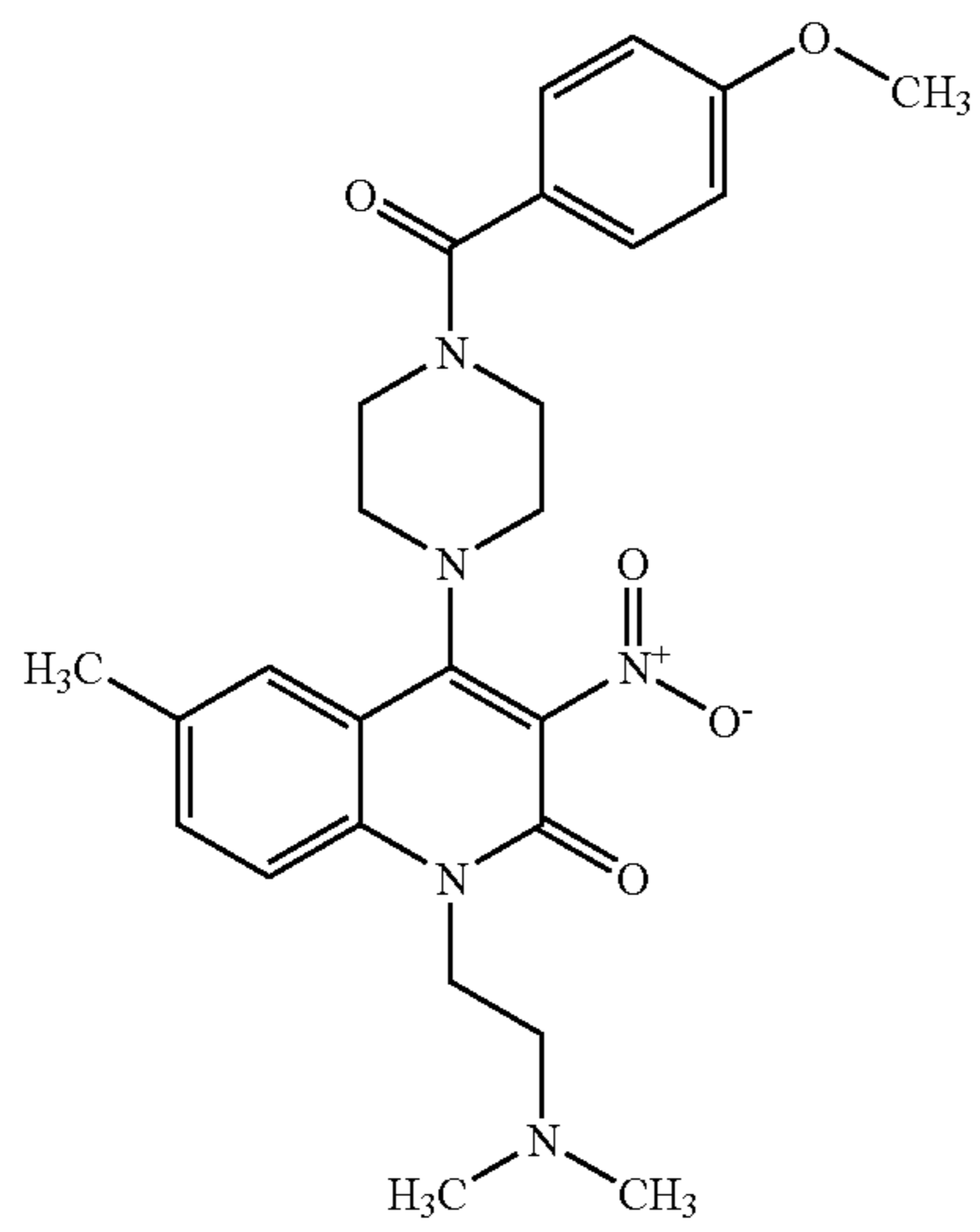
Compound 196
