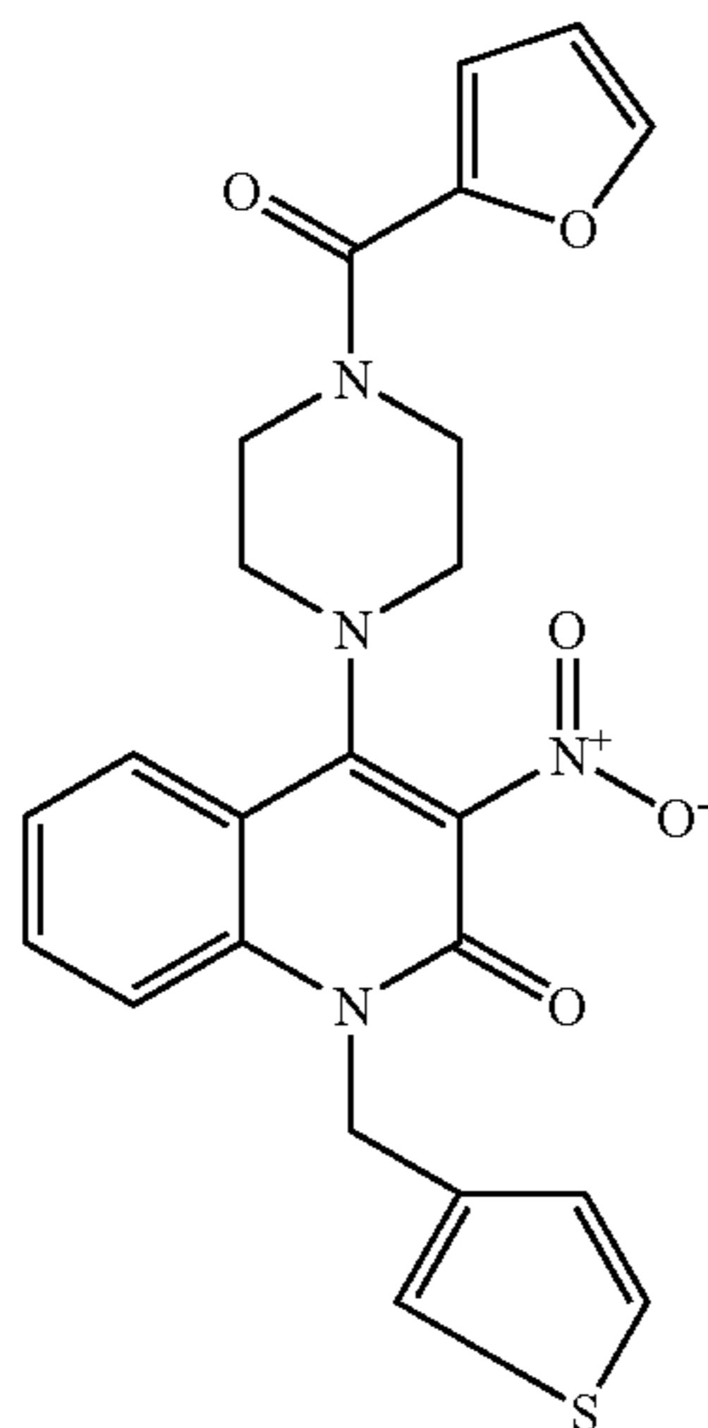
Compound 226
