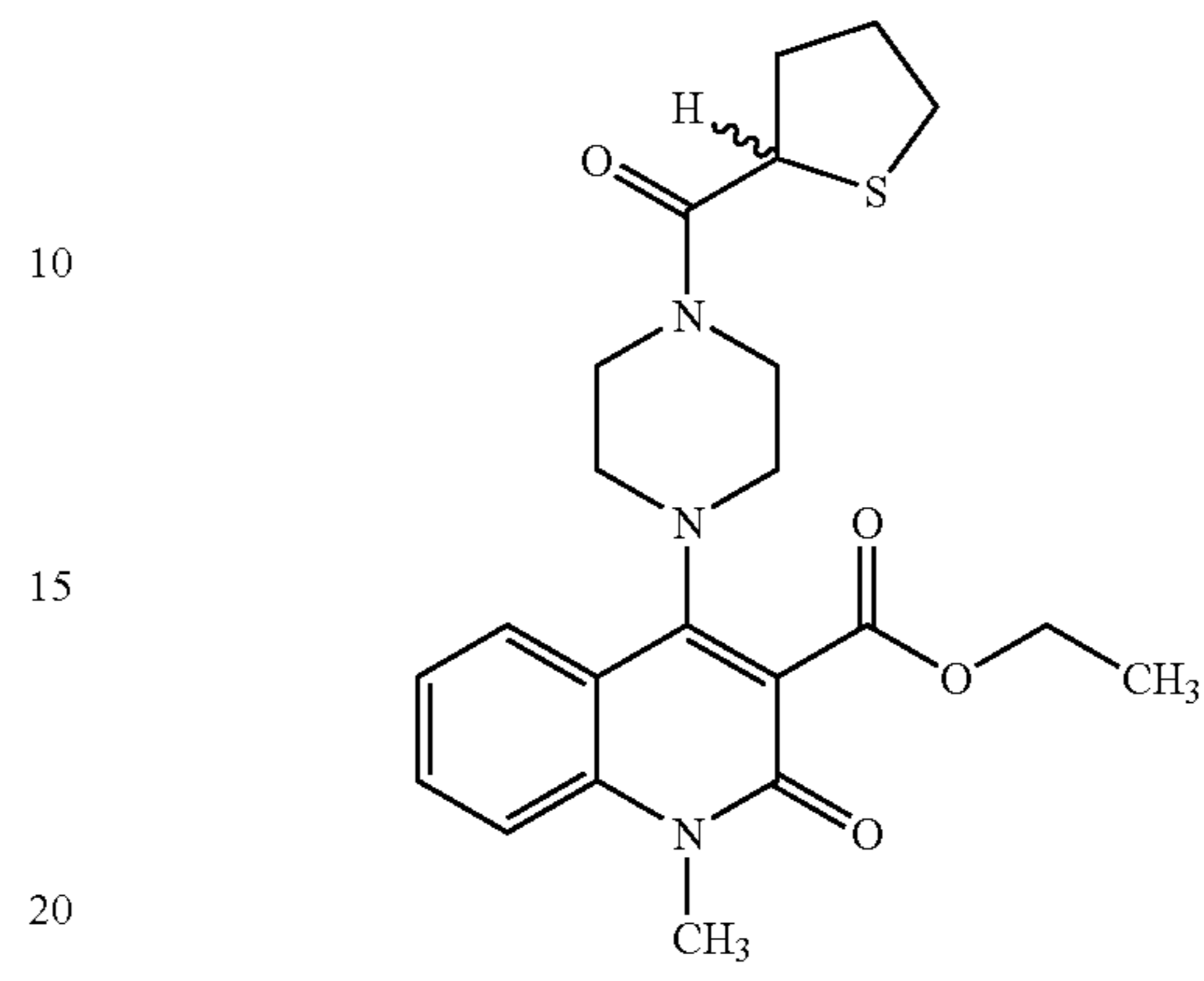
Compound 223
