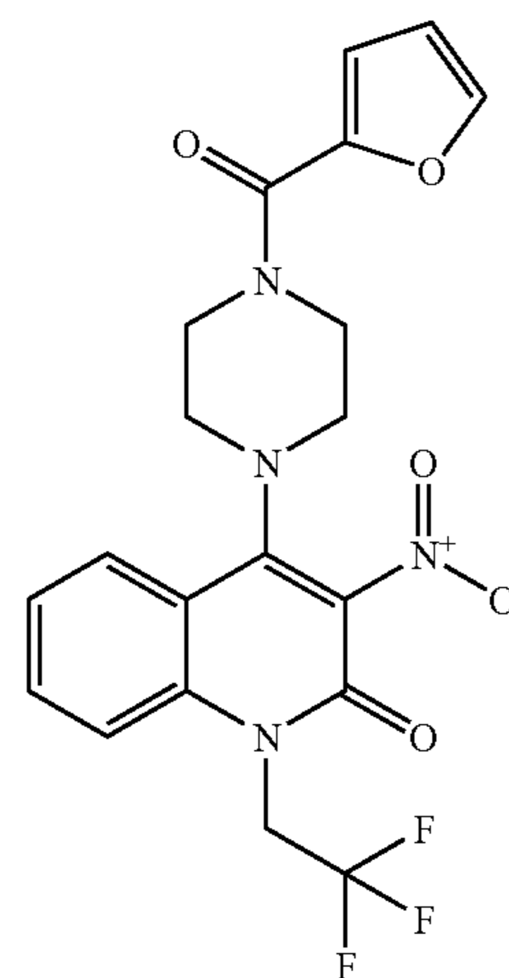
Compound 253
