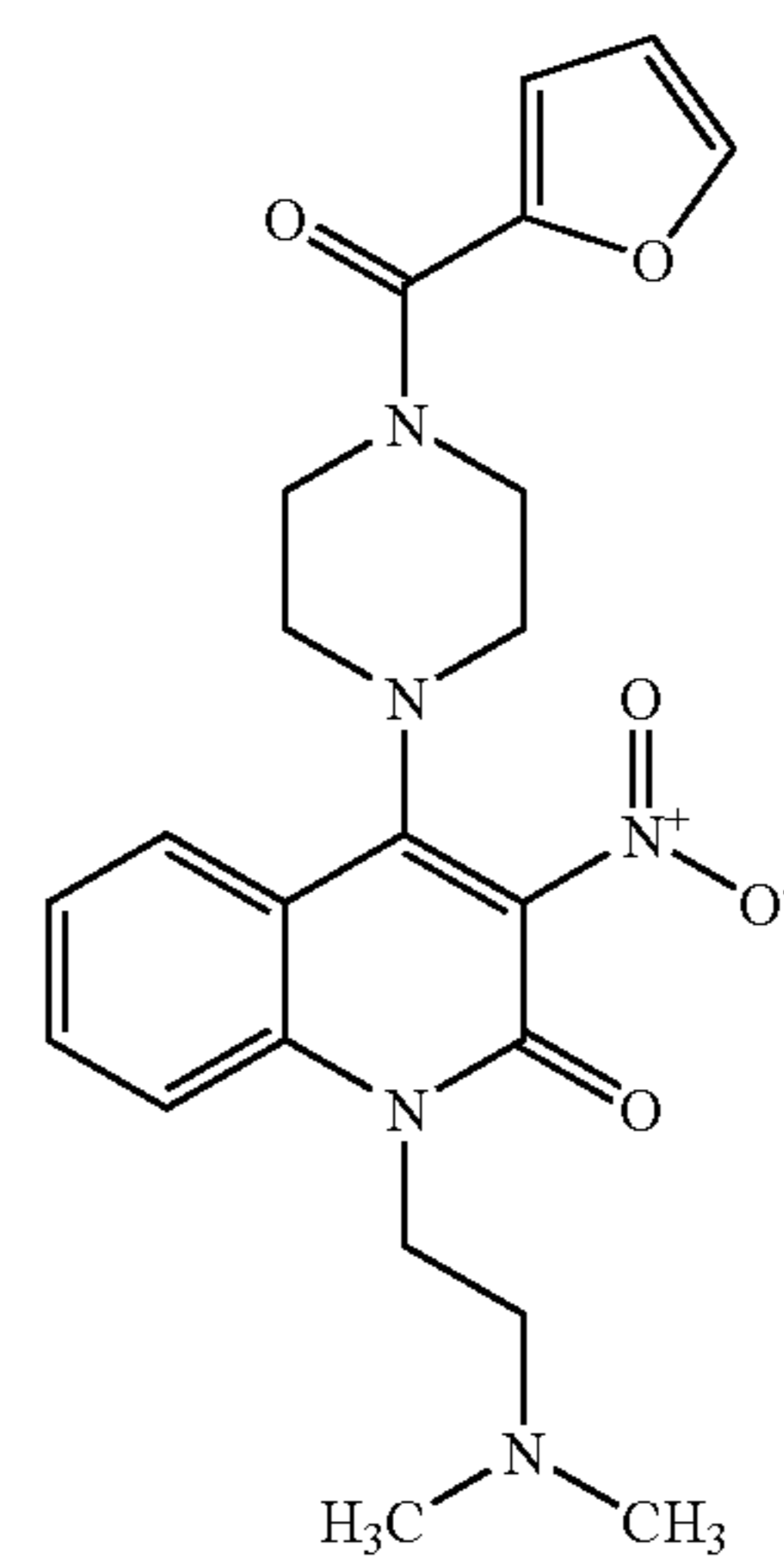
Compound 169
