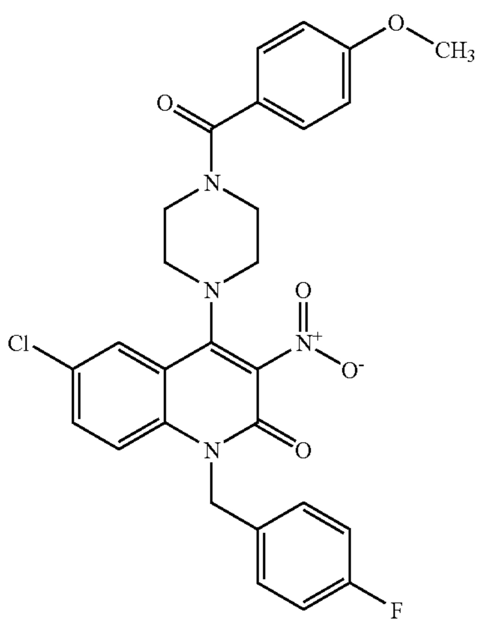
Compound 148
