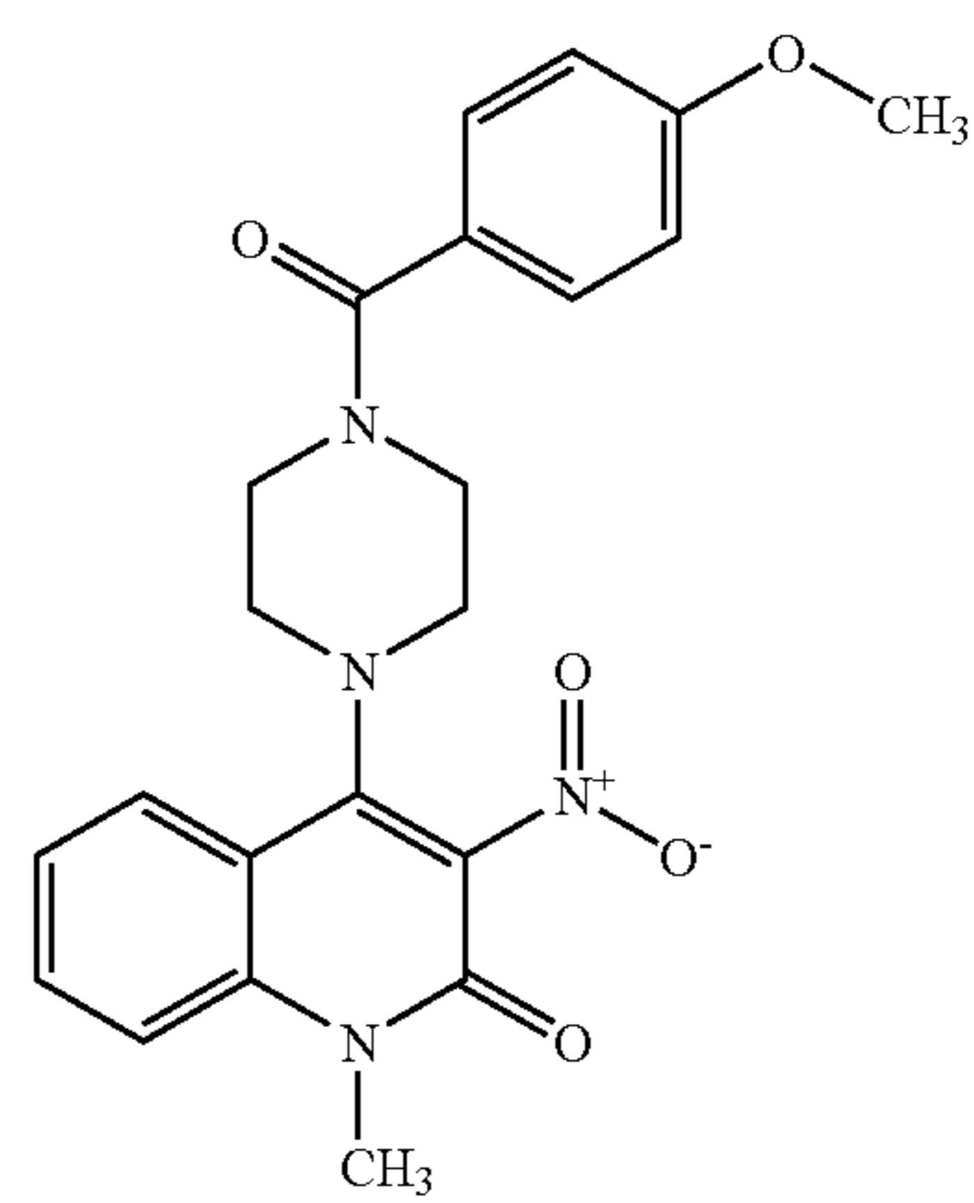
Compound 115
