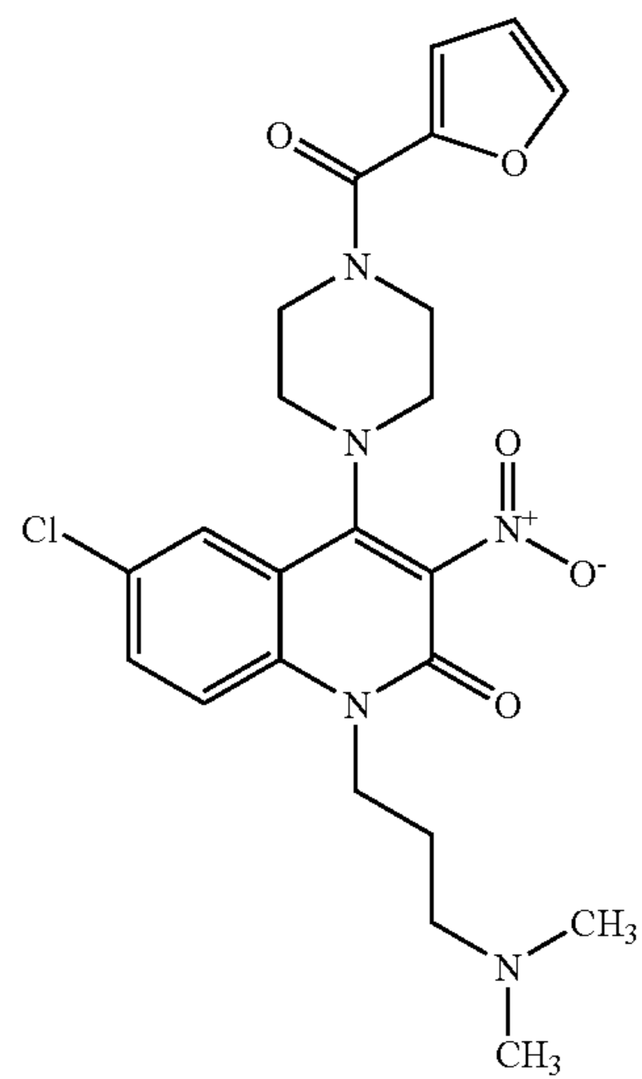
Compound 199
