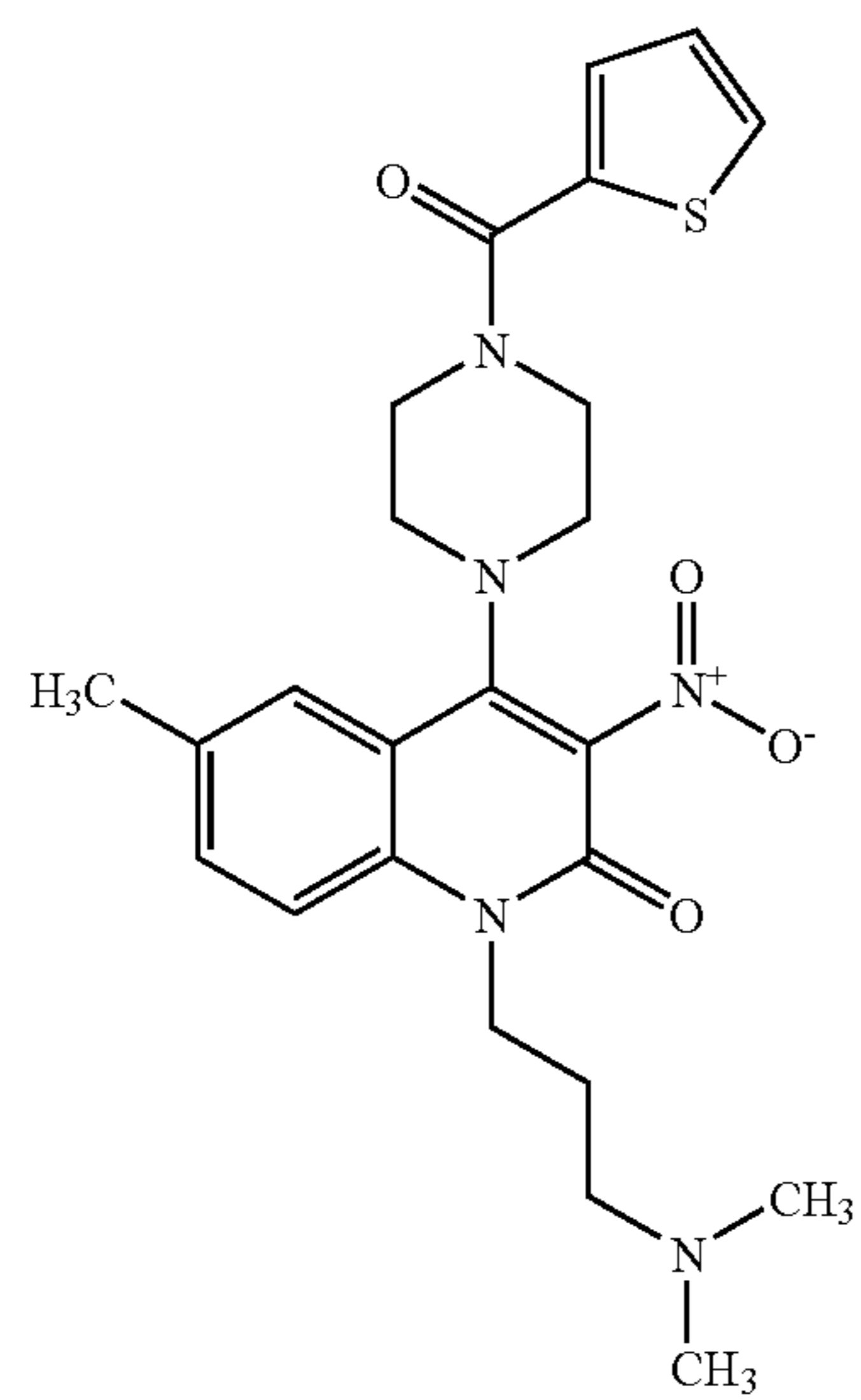
Compound 178
