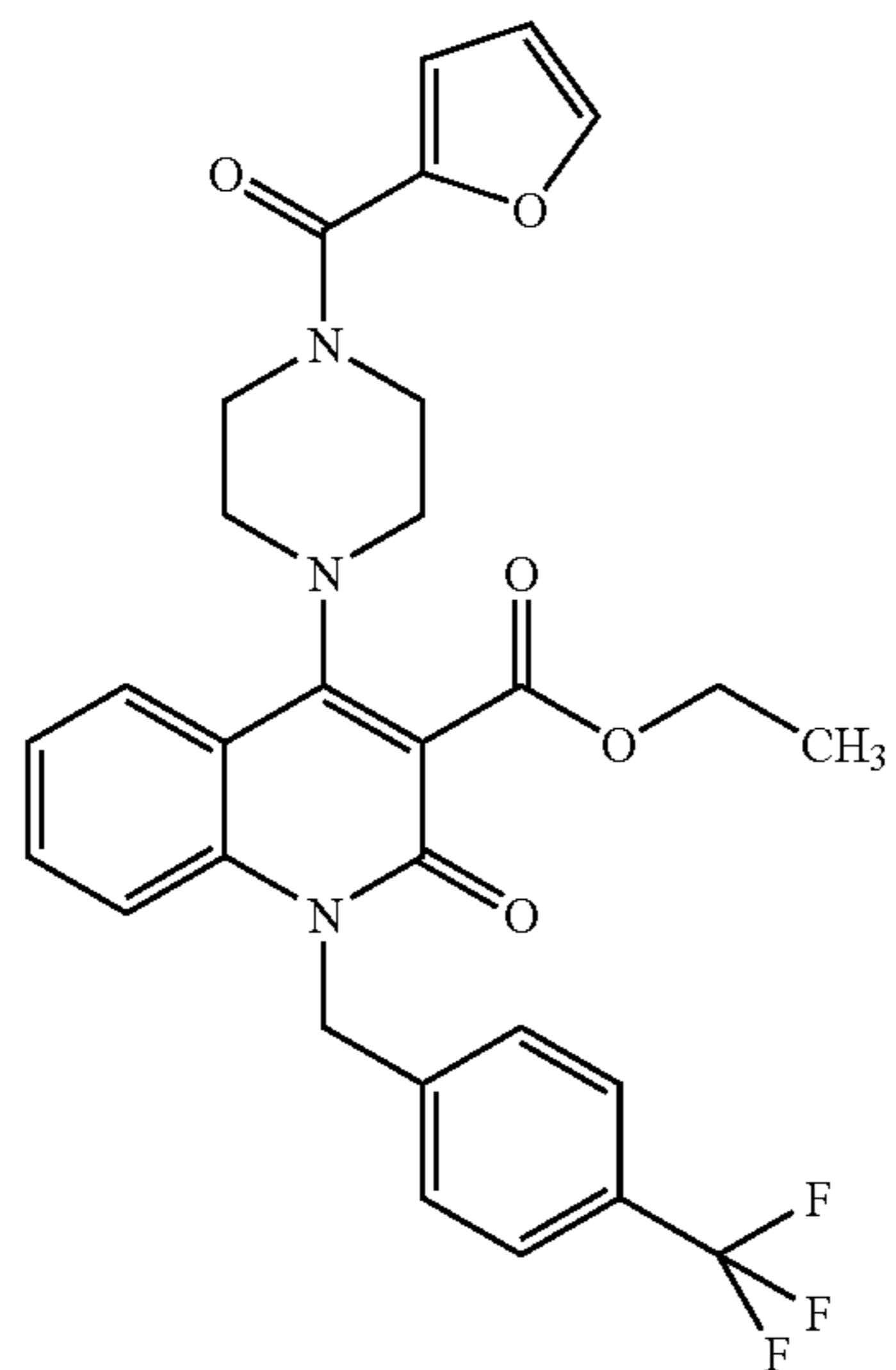
Compound 292
