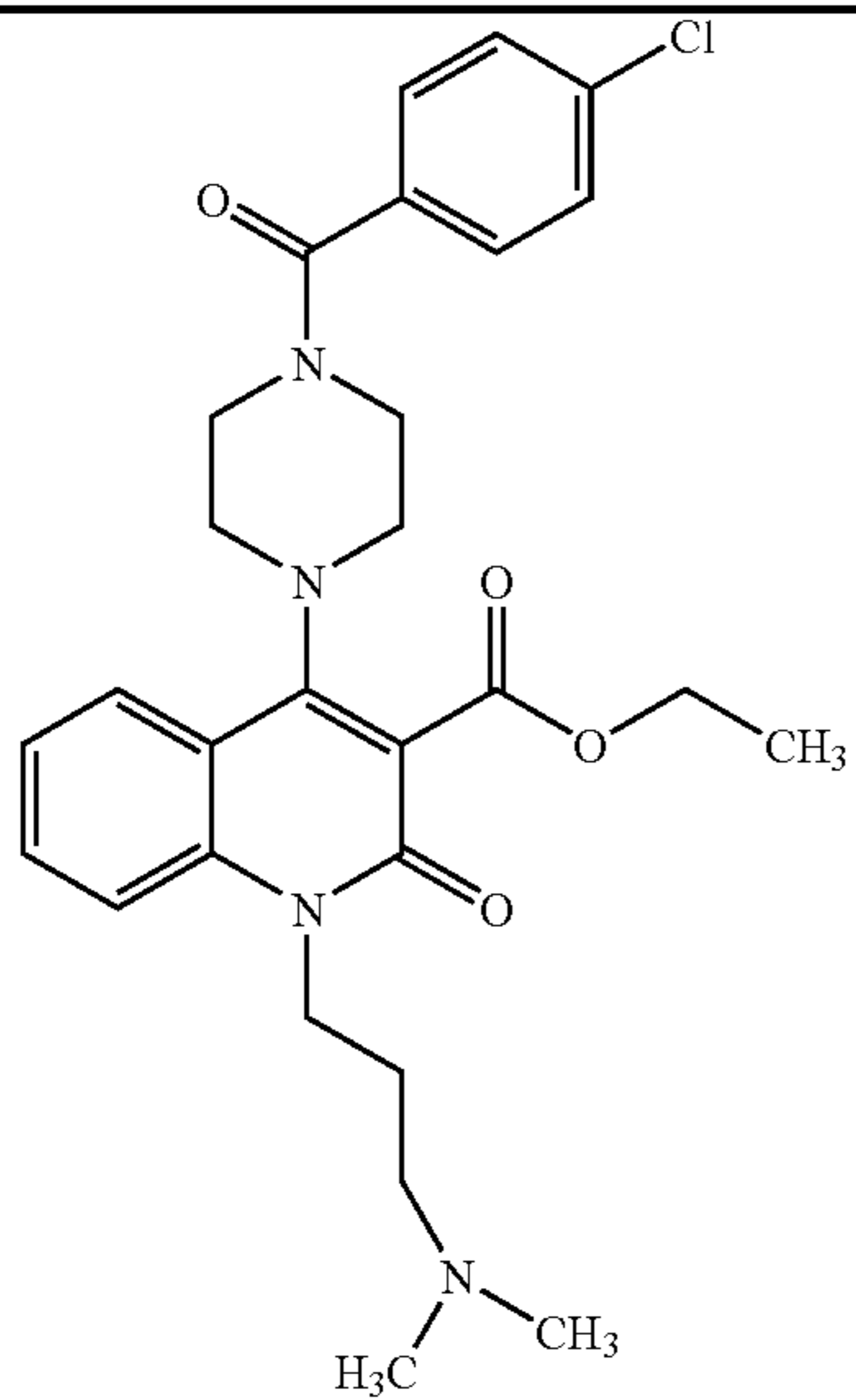
Compound 88
