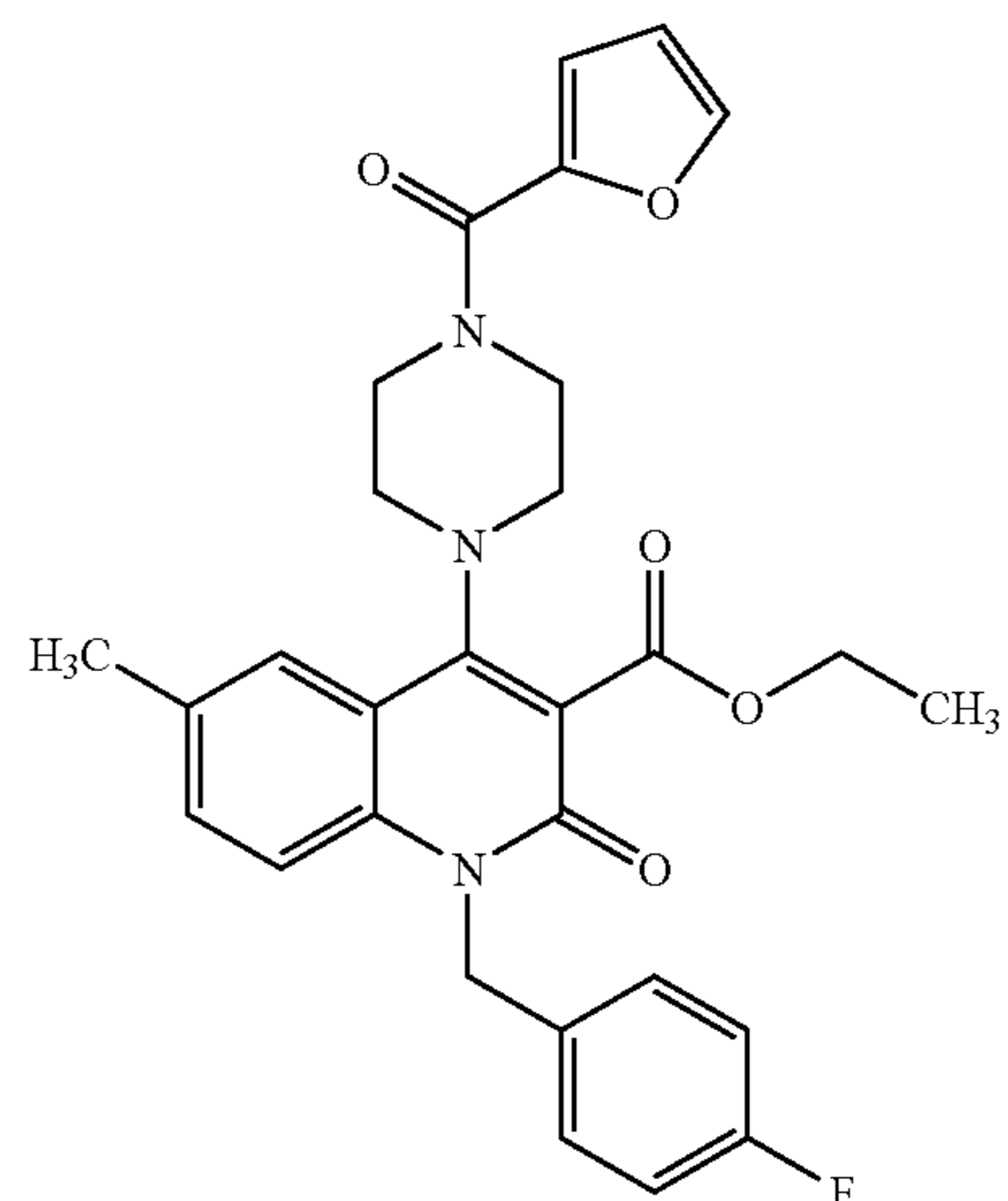
Compound 49
