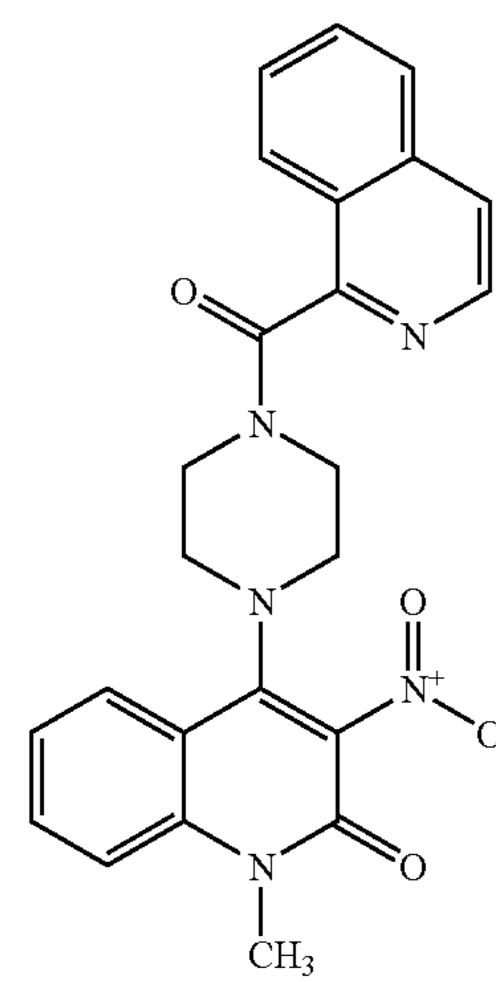
Compound 285
