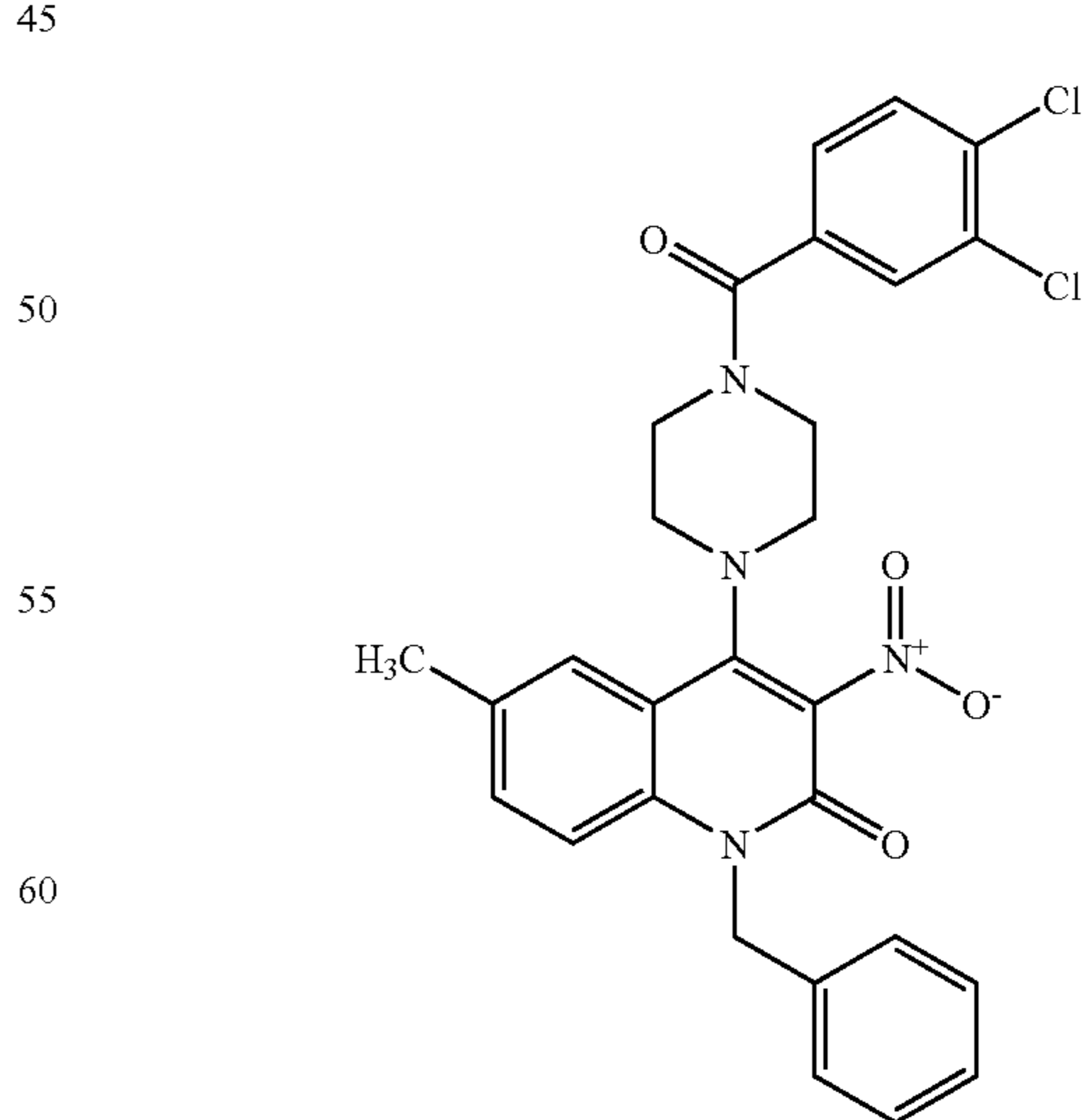
Compound 189
