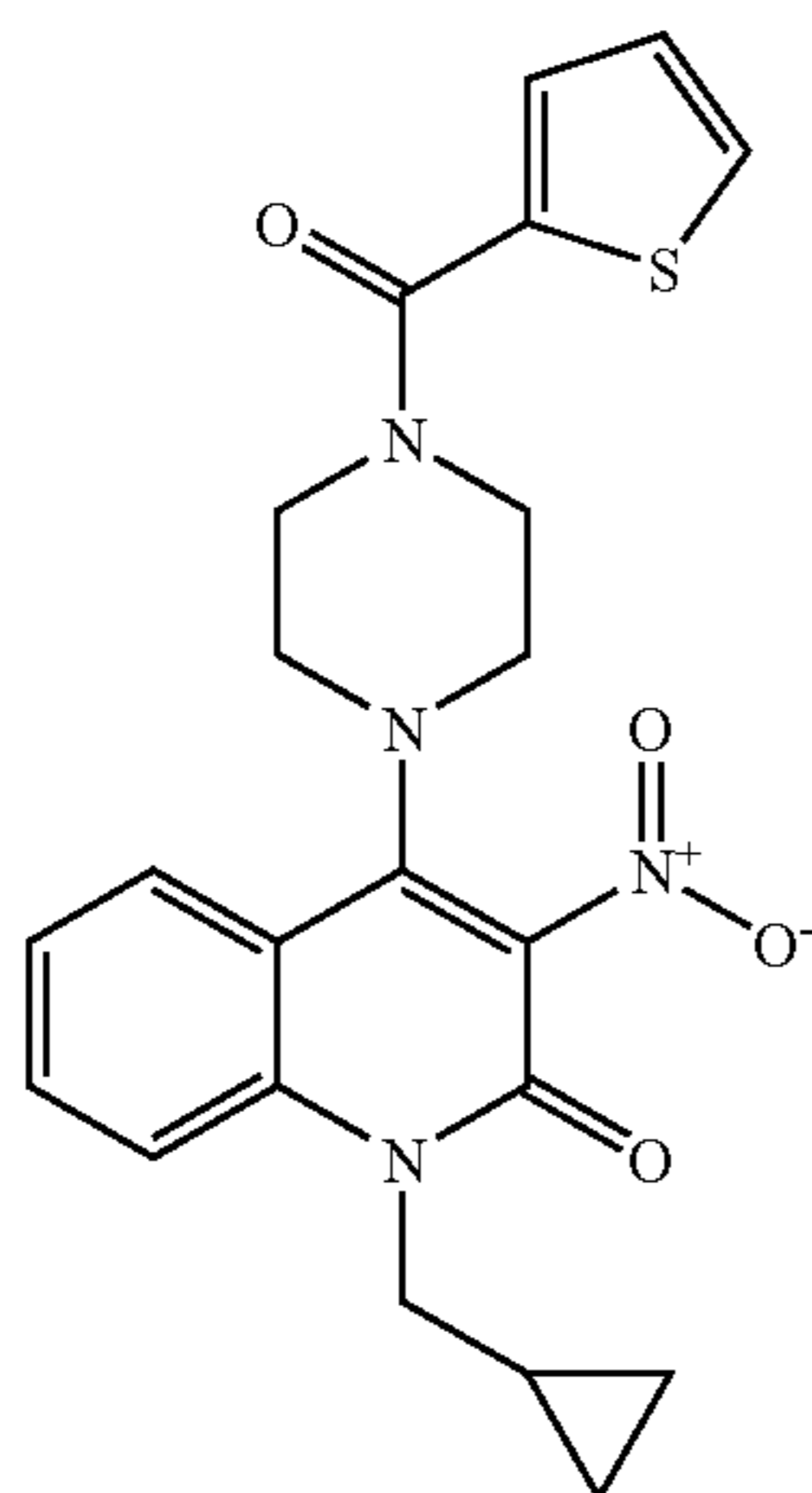
Compound 276
