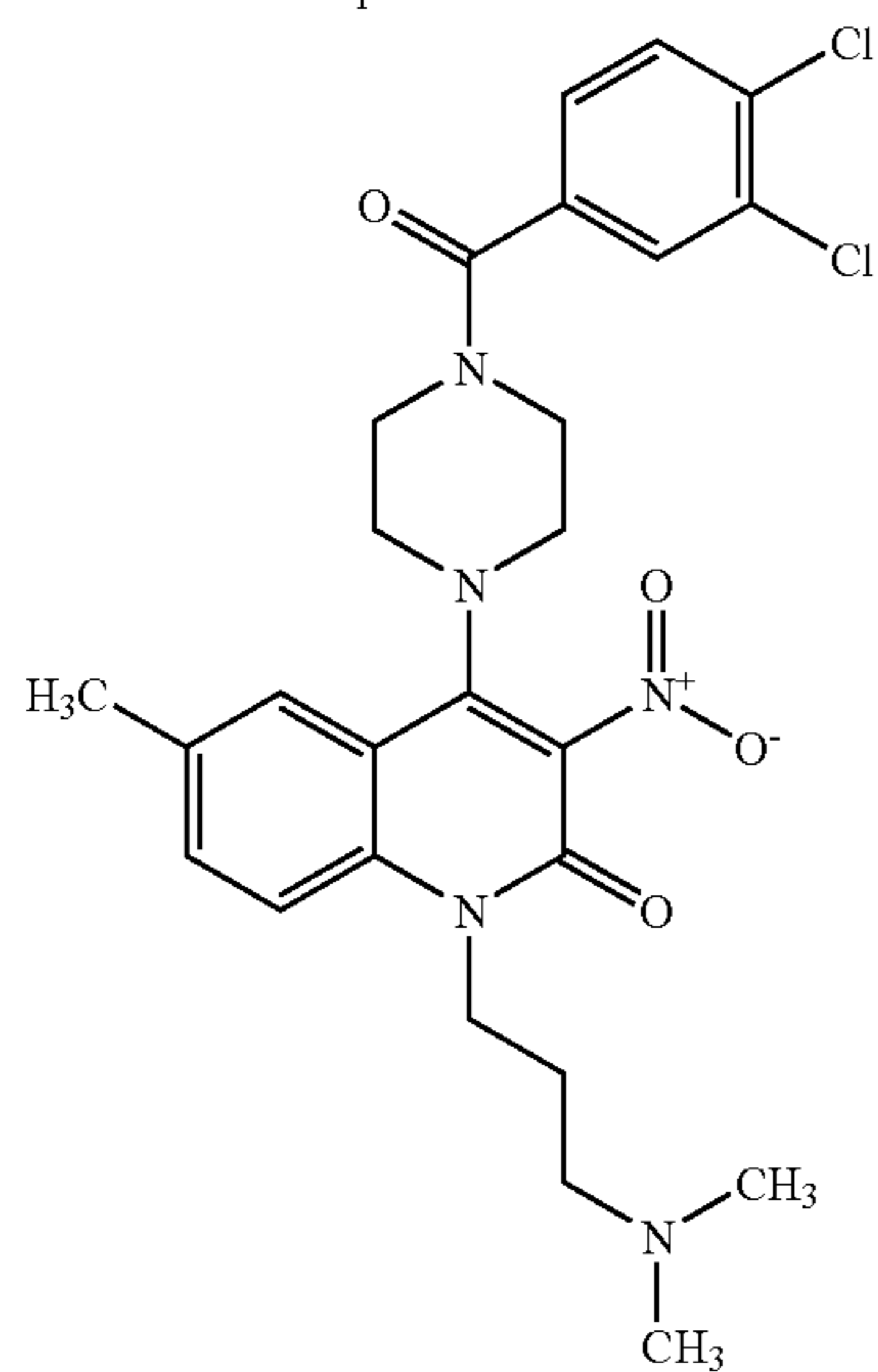
Compound 192
