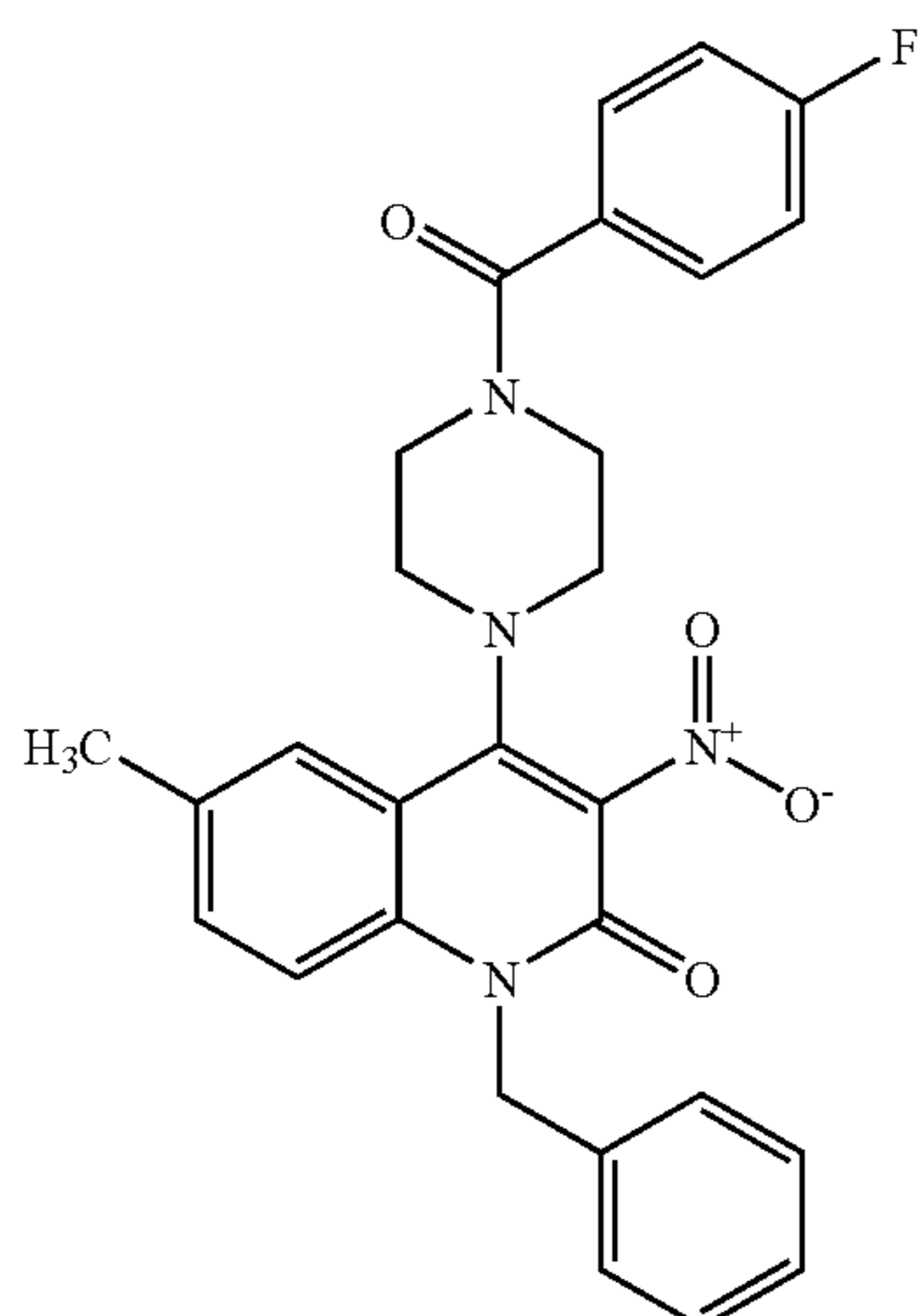
Compound 180
