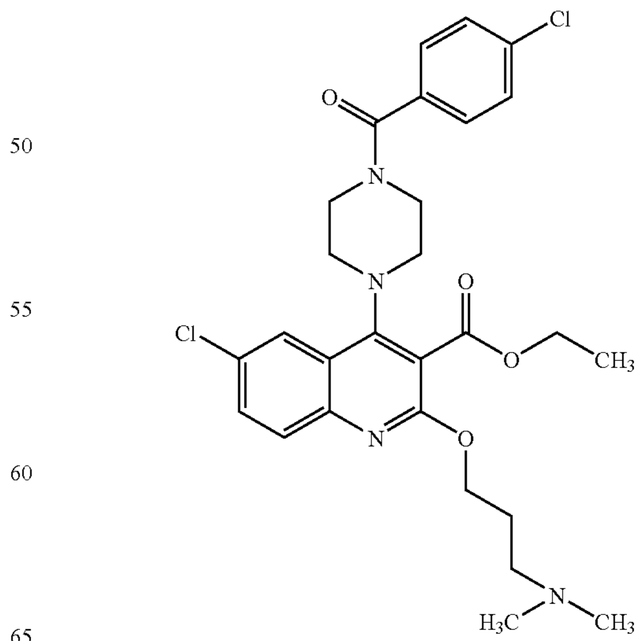
Compound 336
