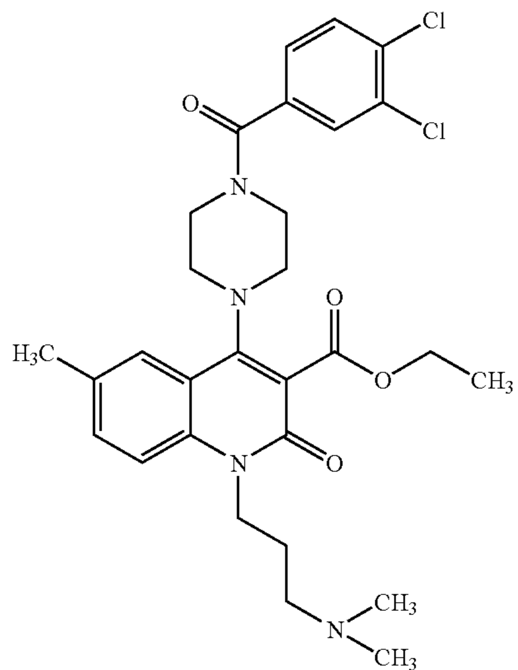
Compound 154
