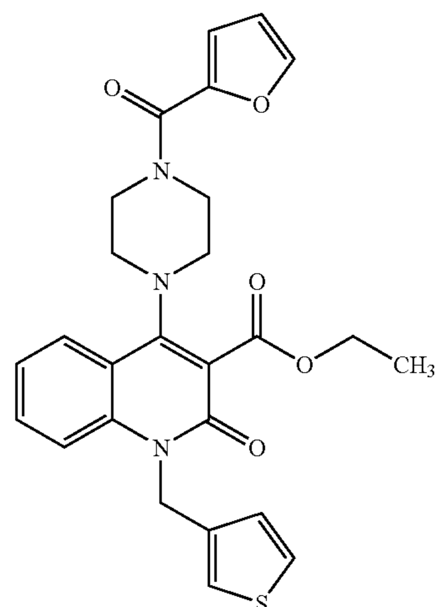
Compound 291
