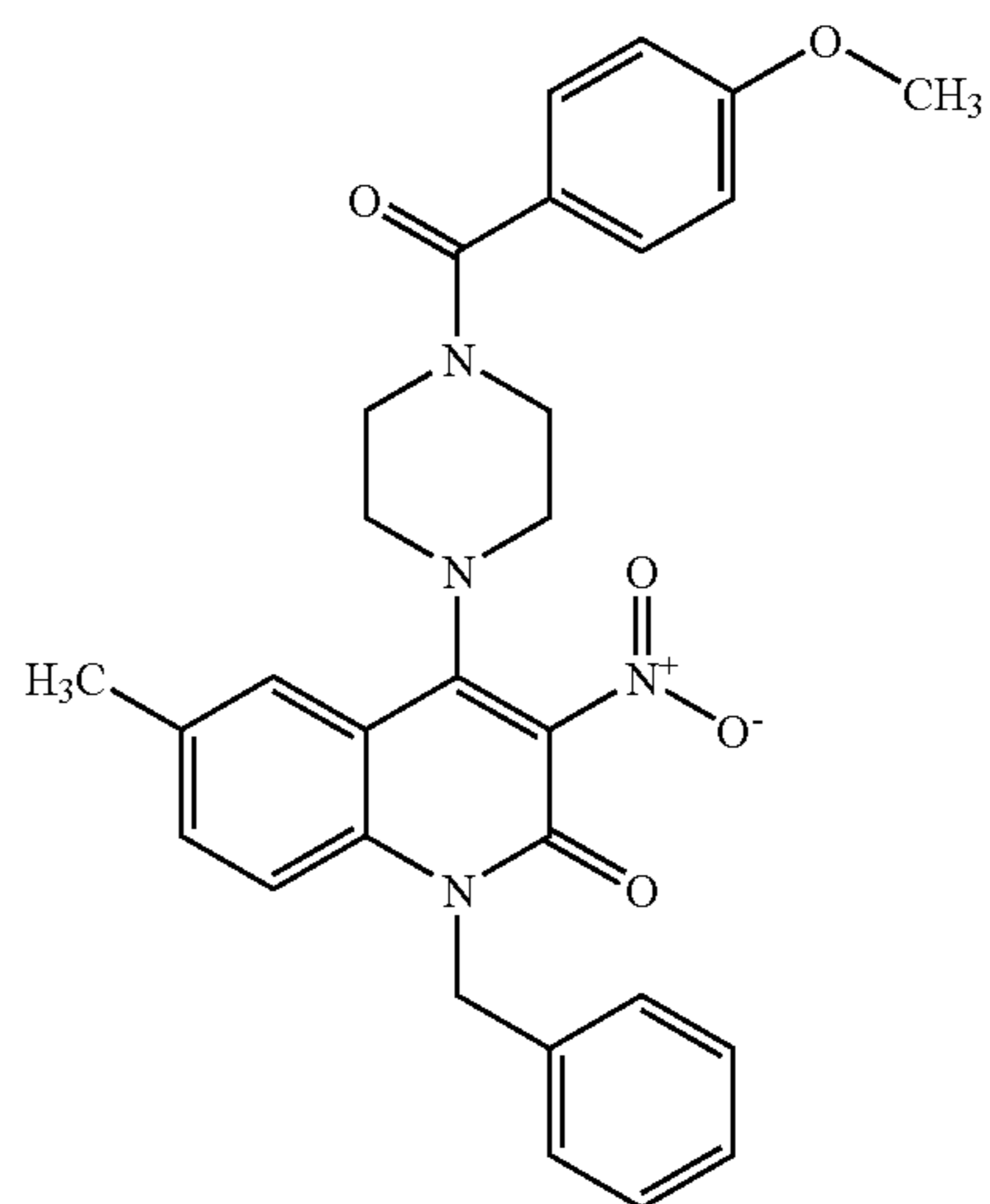
Compound 194
