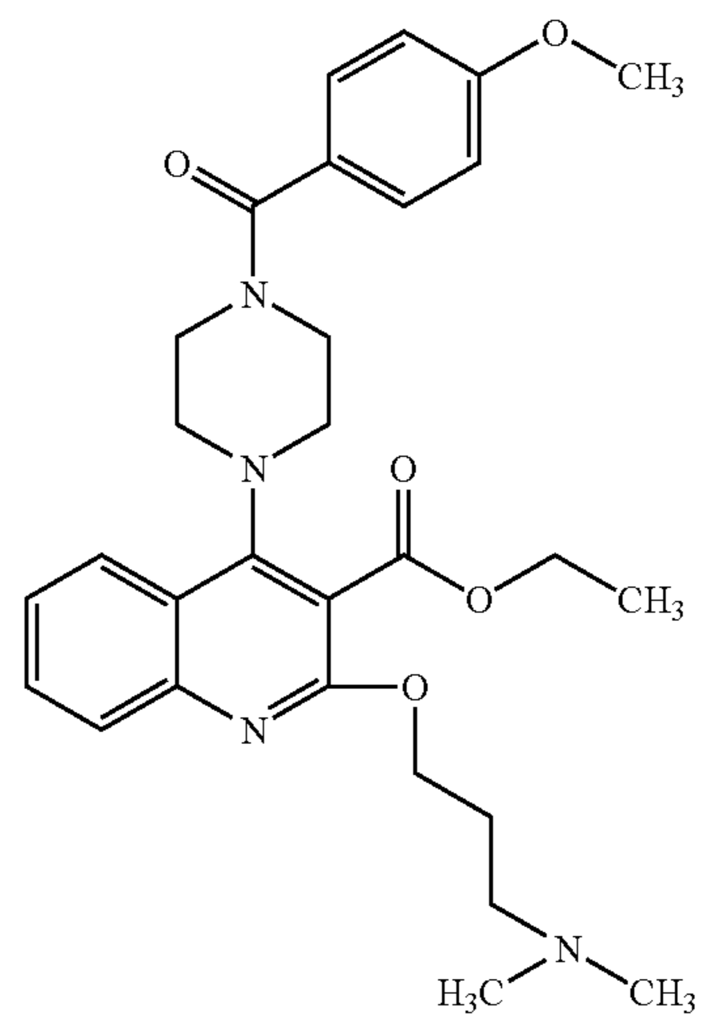
Compound 329
