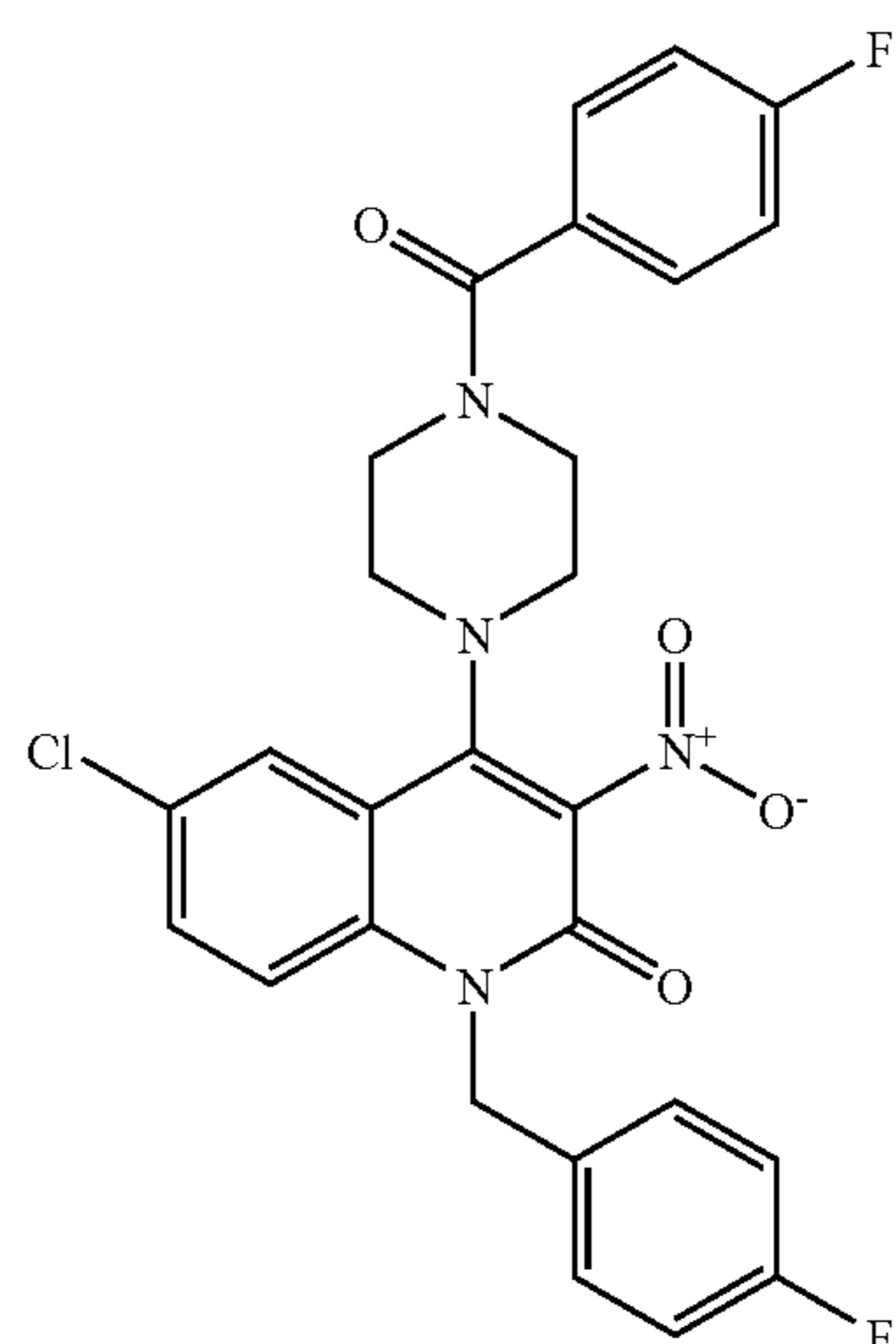
Compound 144
