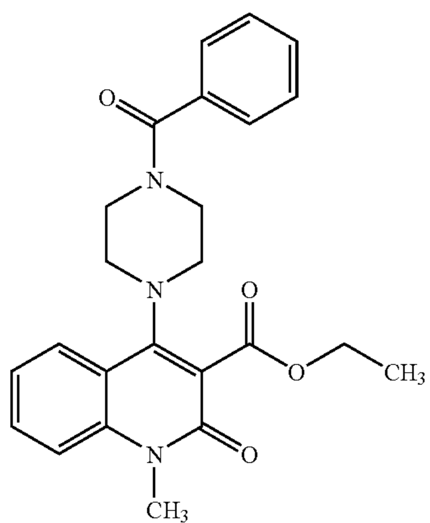
Compound 12
