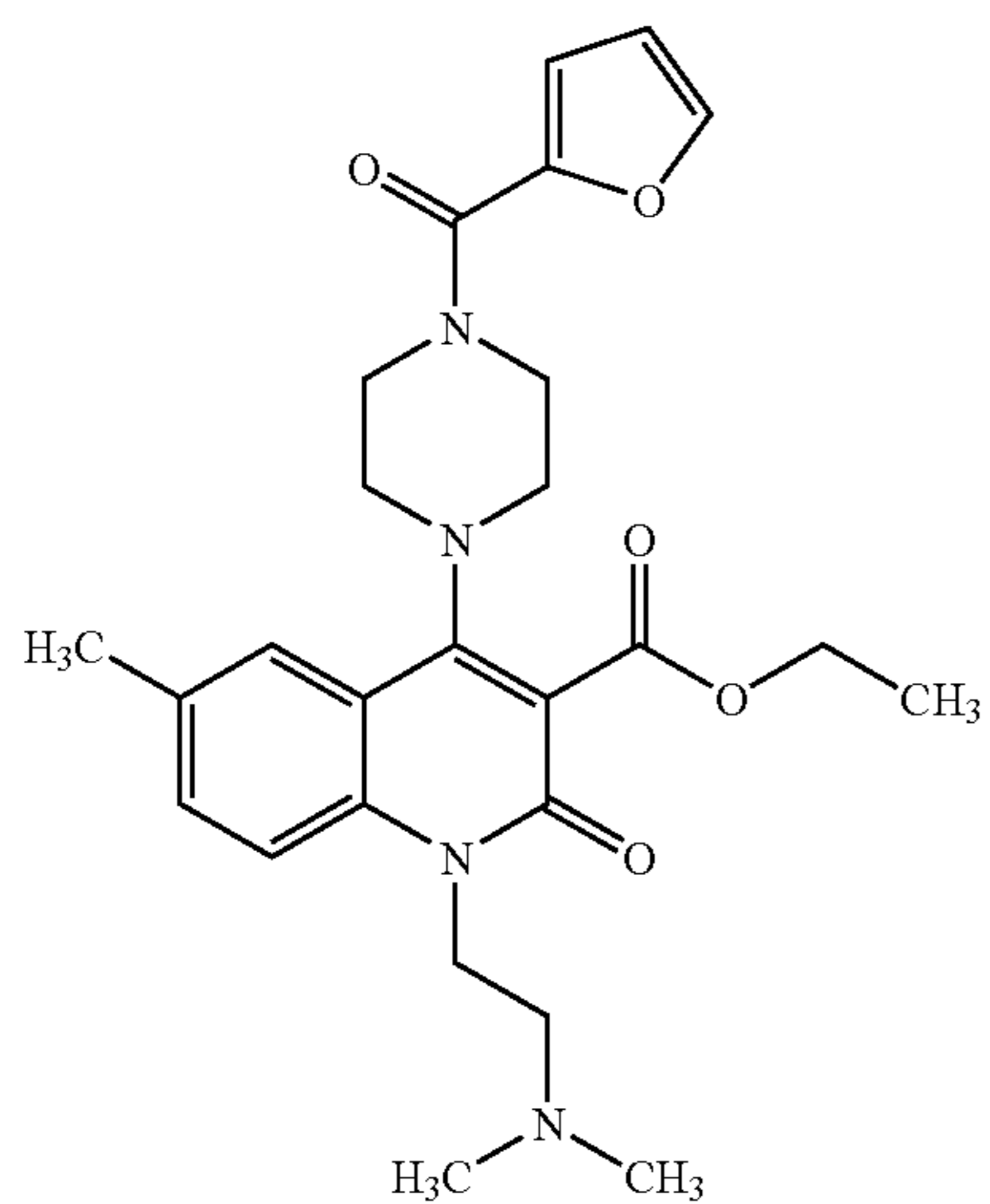
Compound 65
