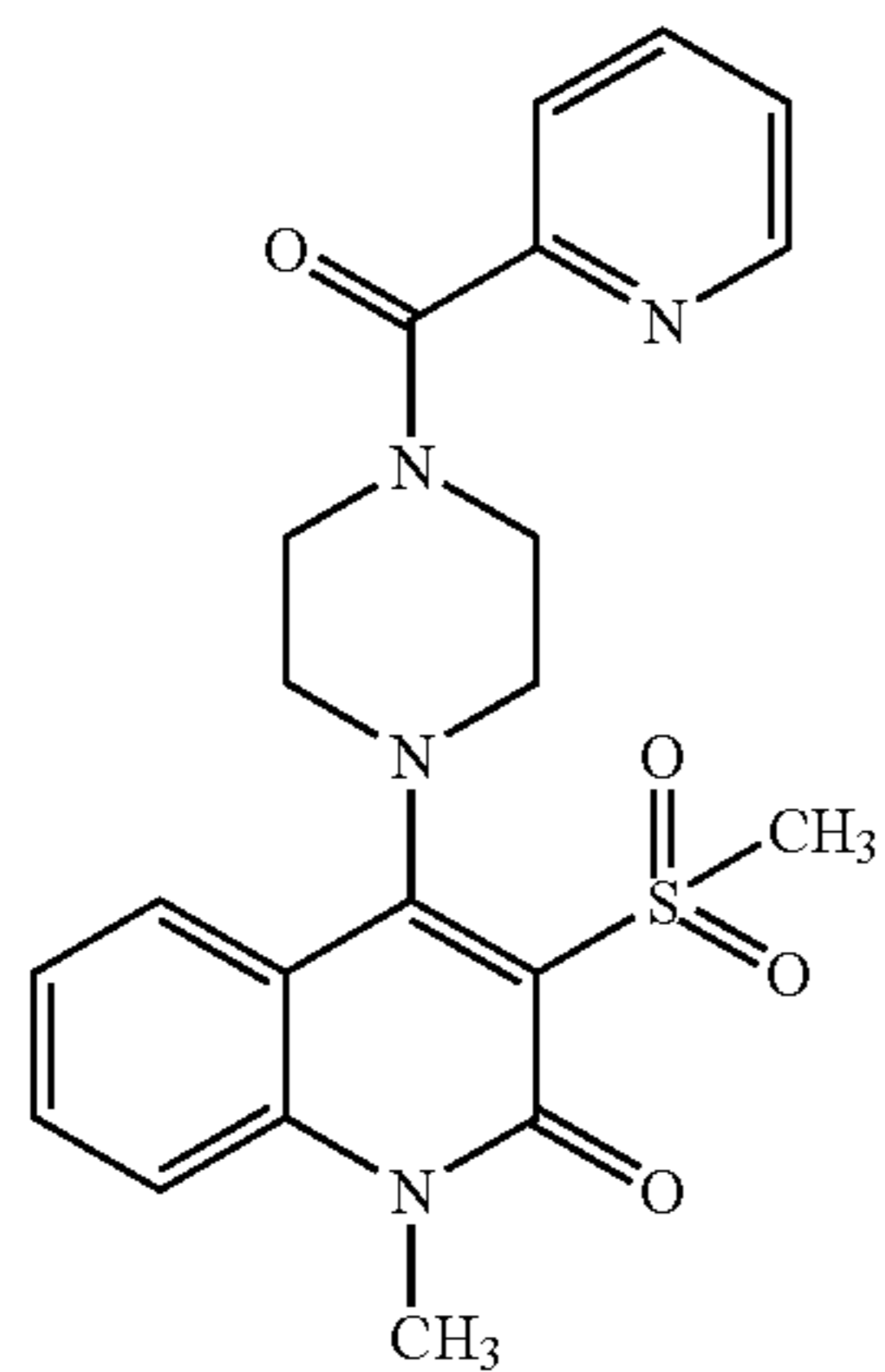
Compound 102
