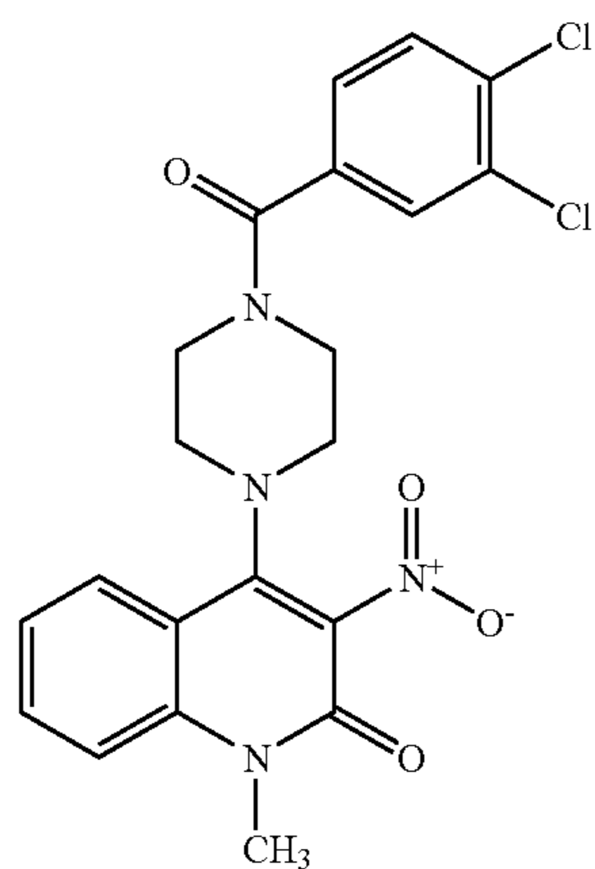
Compound 120
