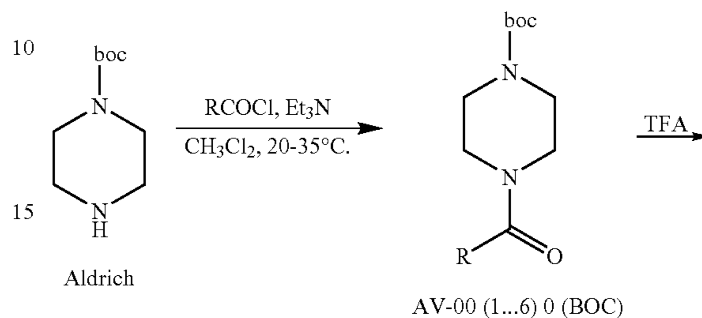
Reaction Scheme 23
