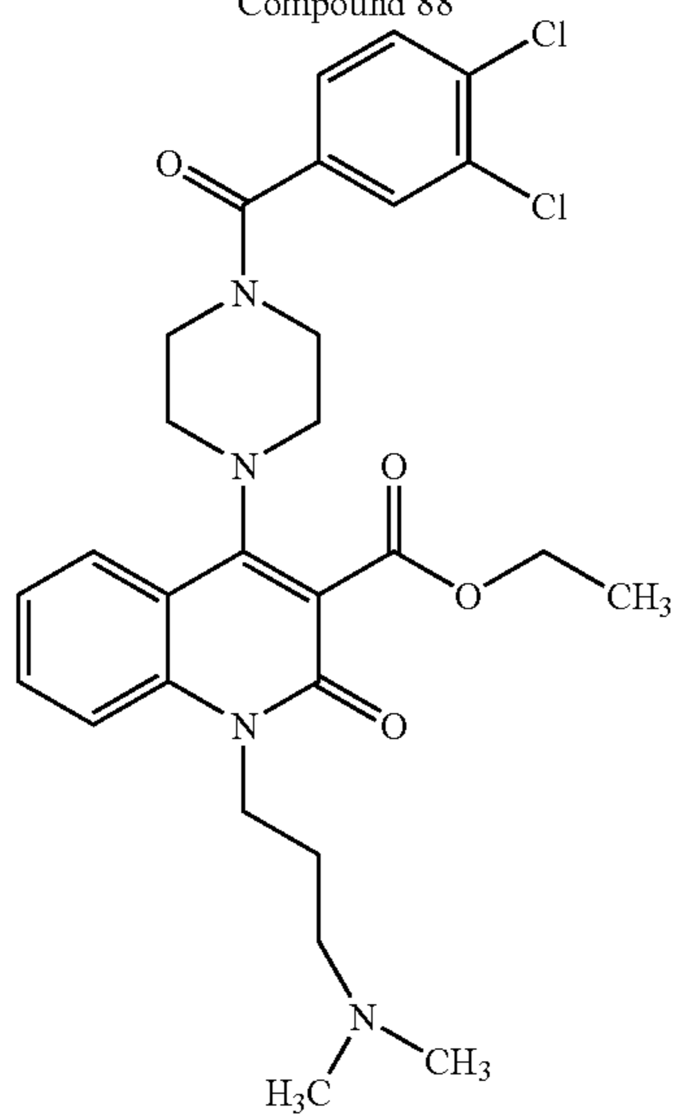
Compound 89
