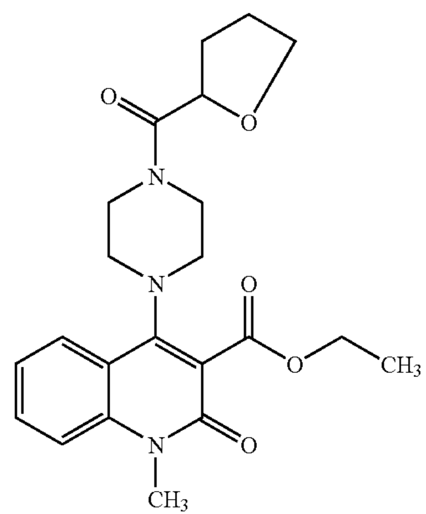
Compound 290
