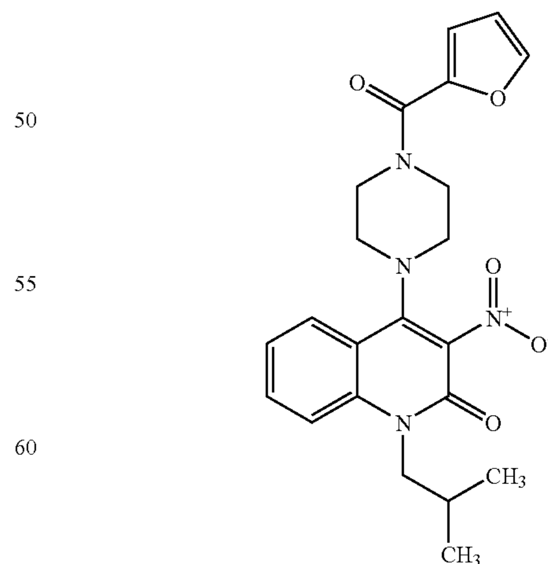
Compound 225
