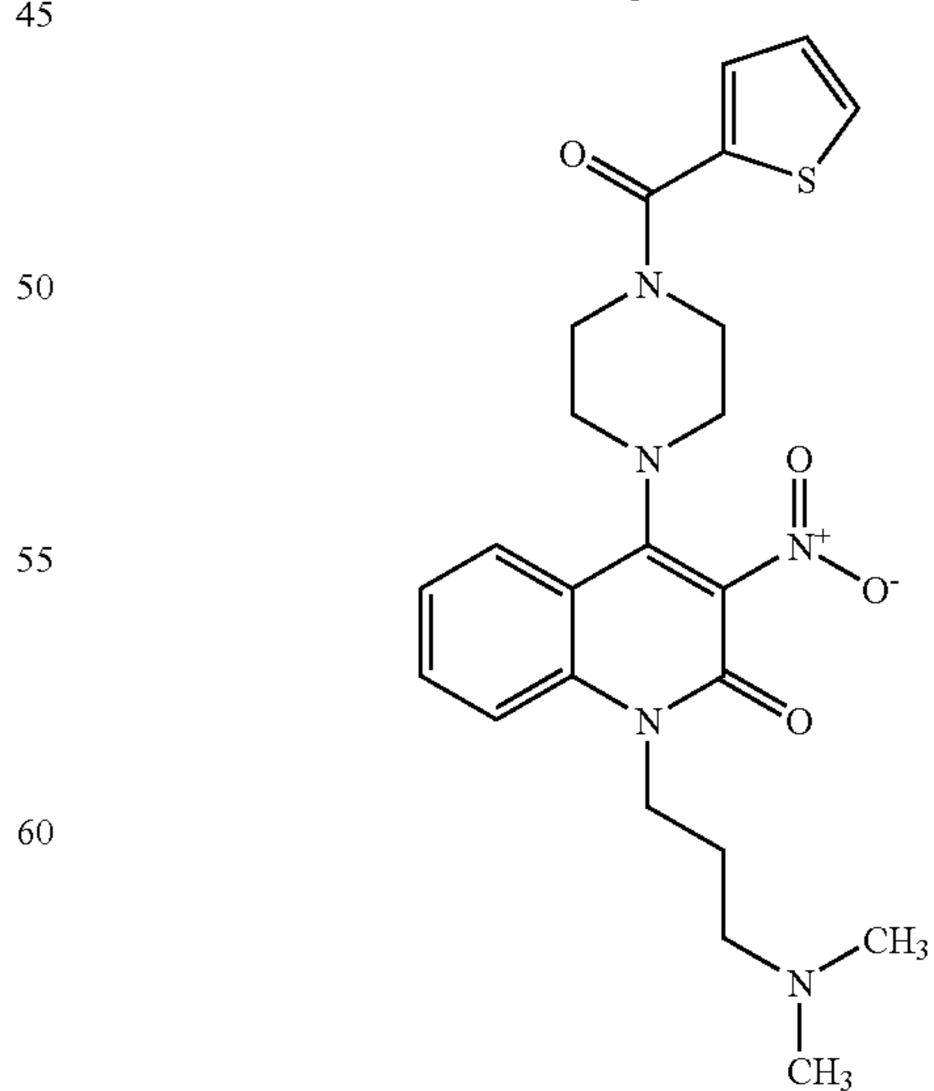
Compound 159
