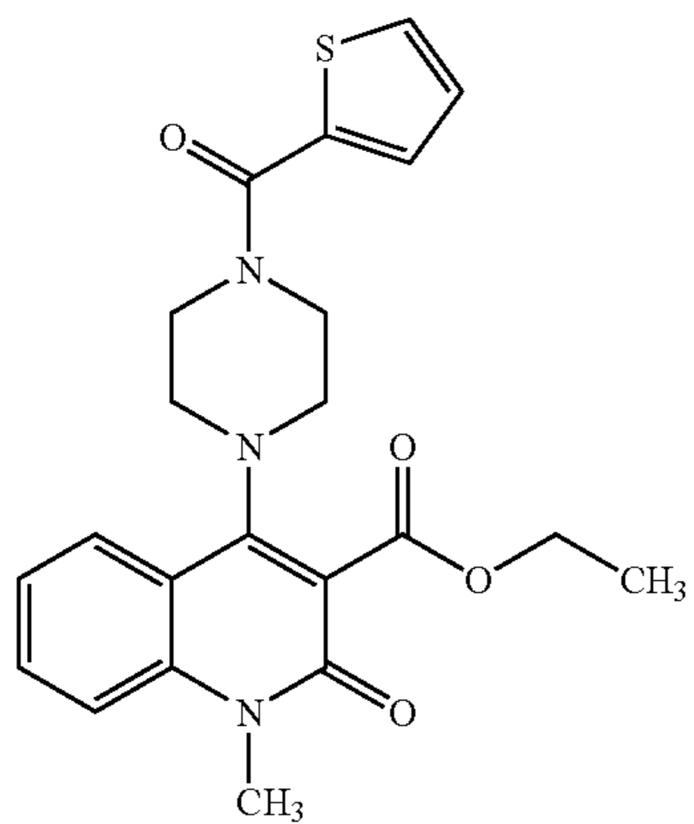
Compound 11
