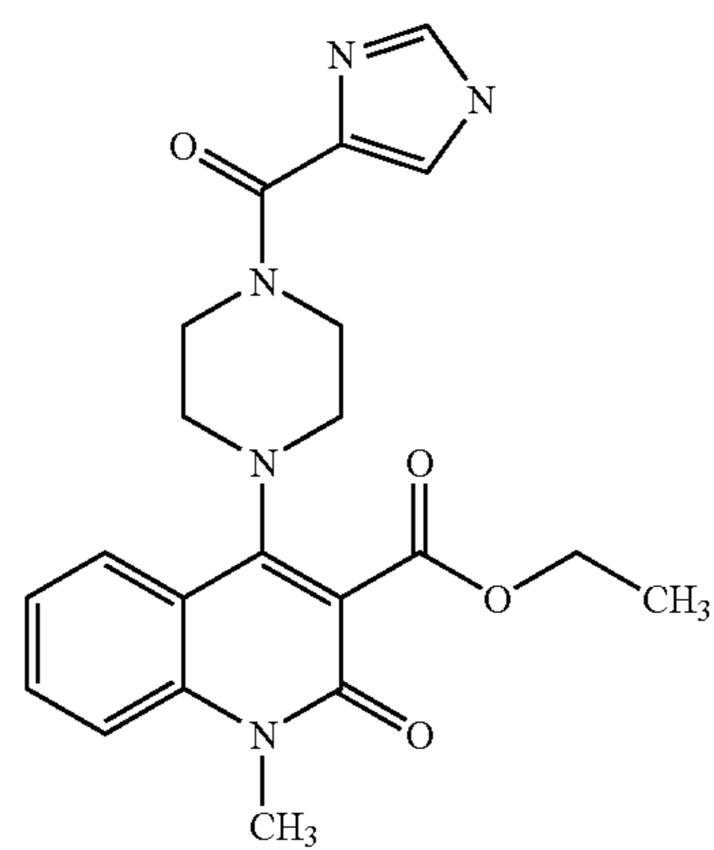
Compound 267
