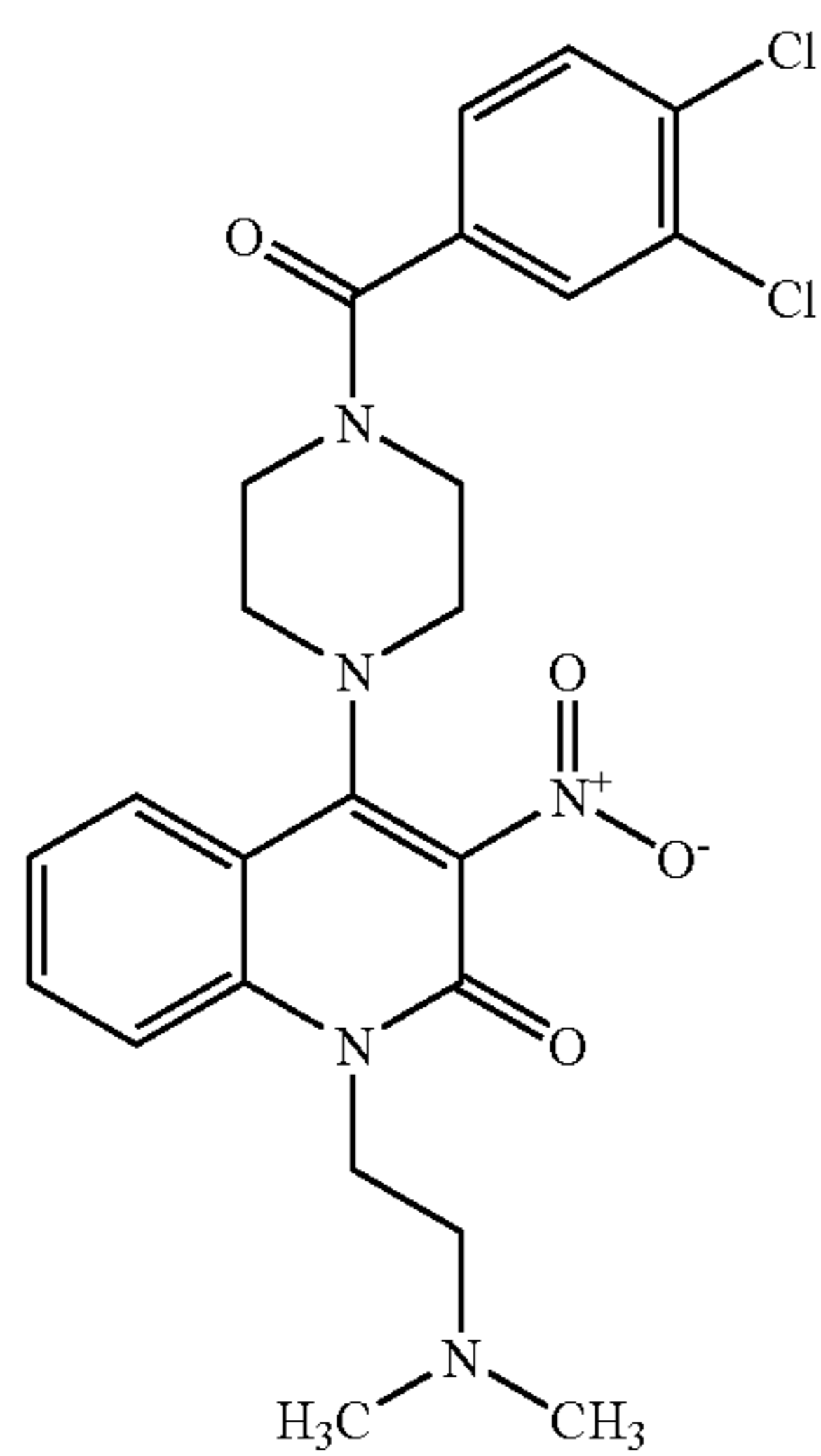
Compound 172
