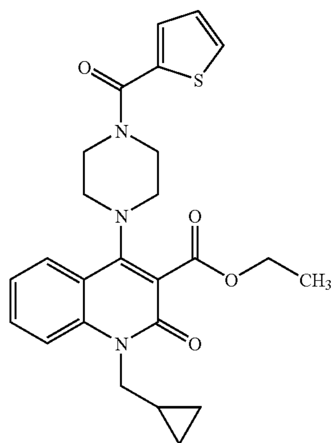
Compound 298
