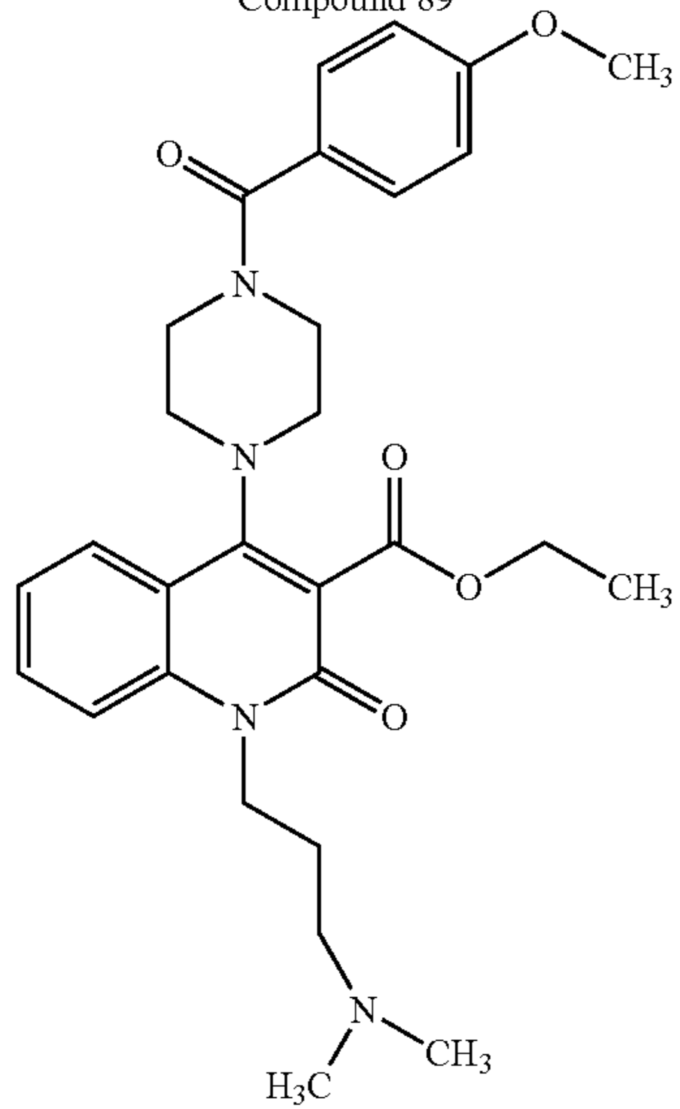
Compound 90
