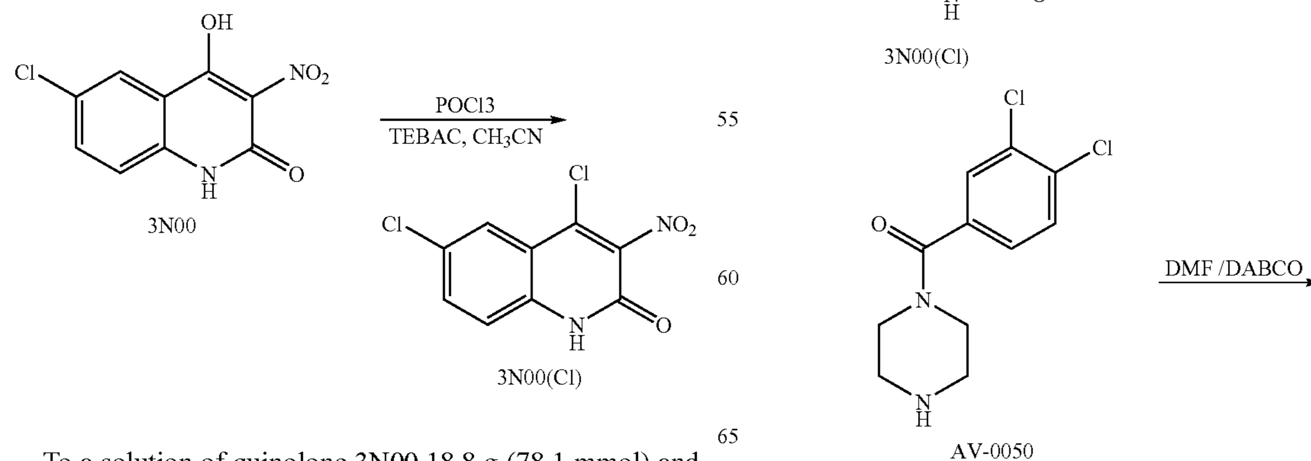
Reaction Scheme 27
