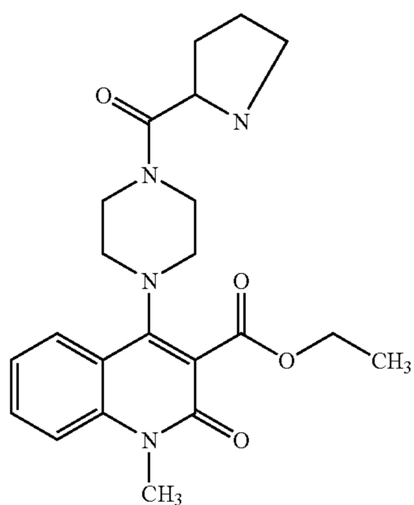
Compound 288
