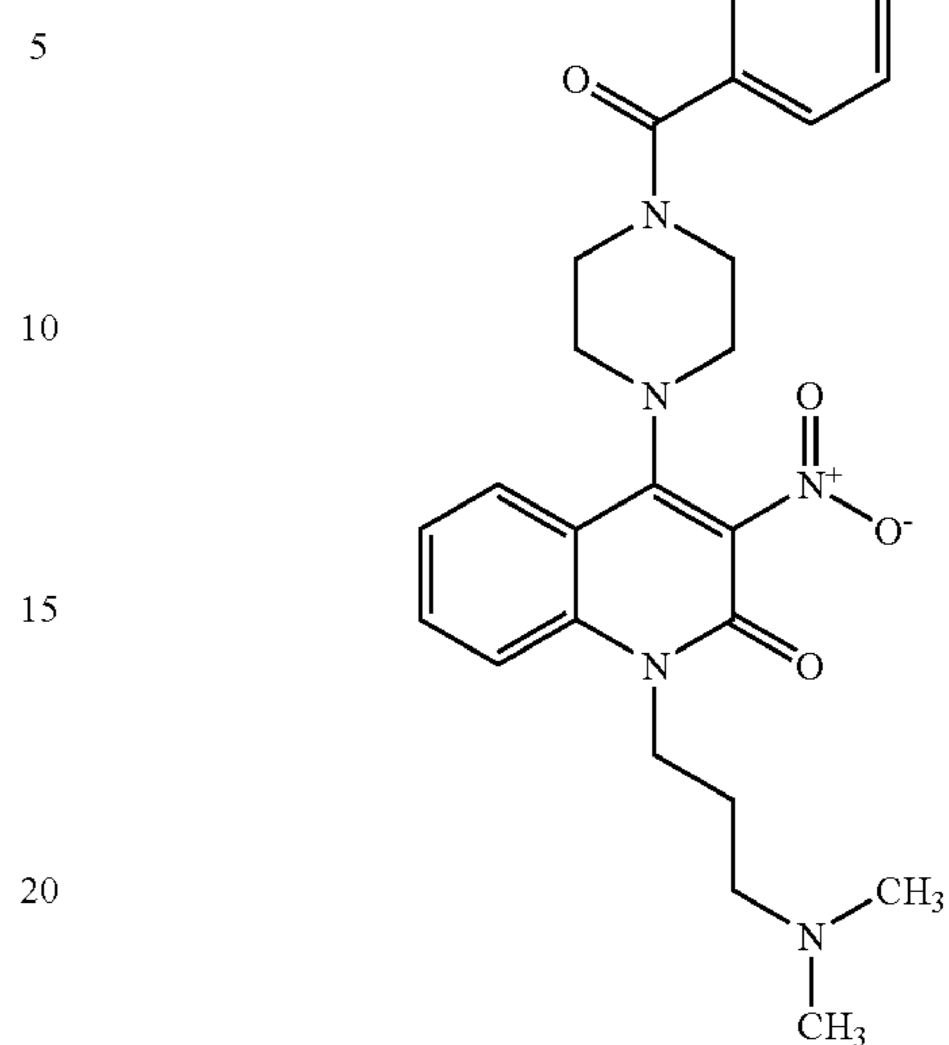
Compound 139
