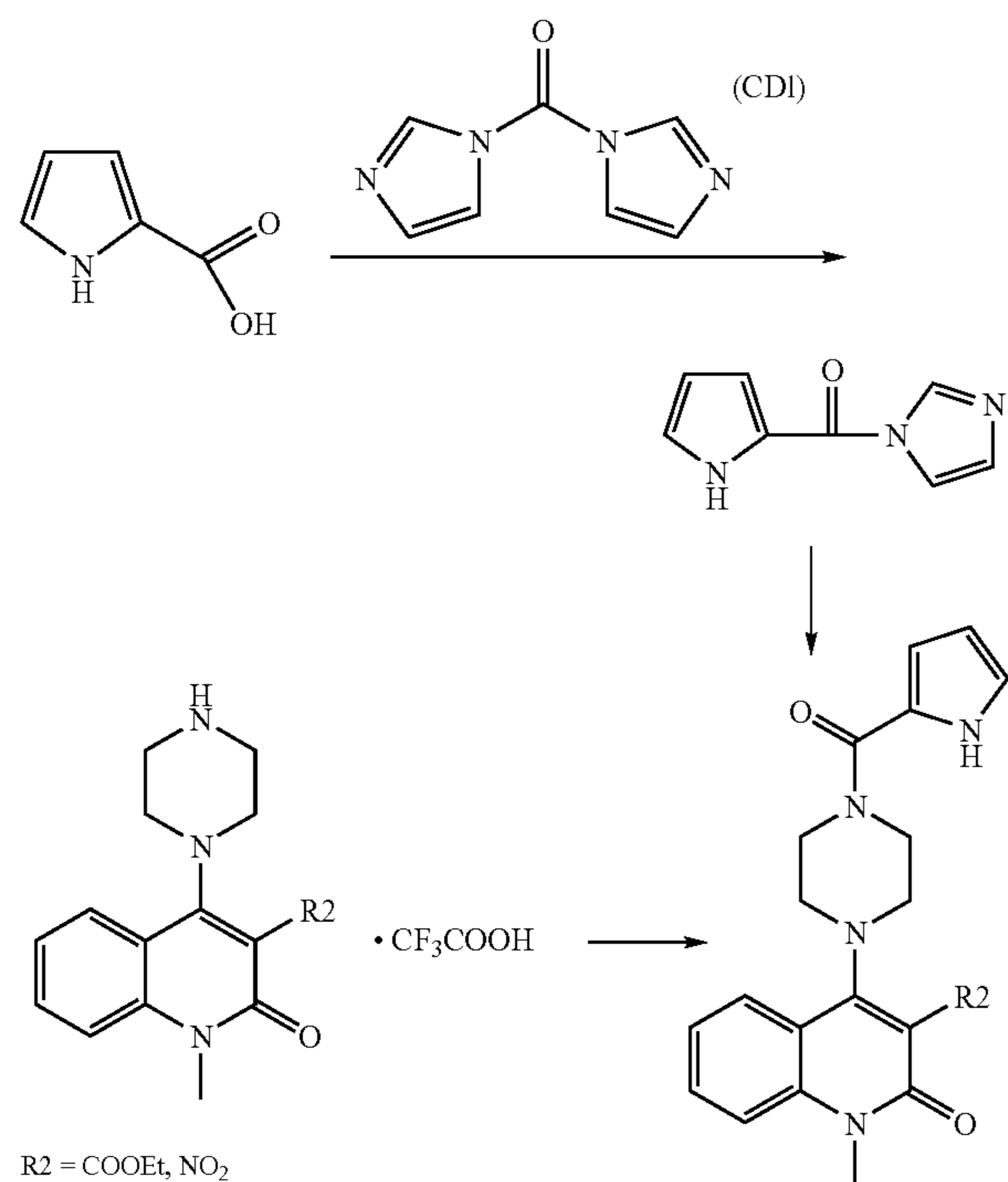
Reaction Scheme 17
