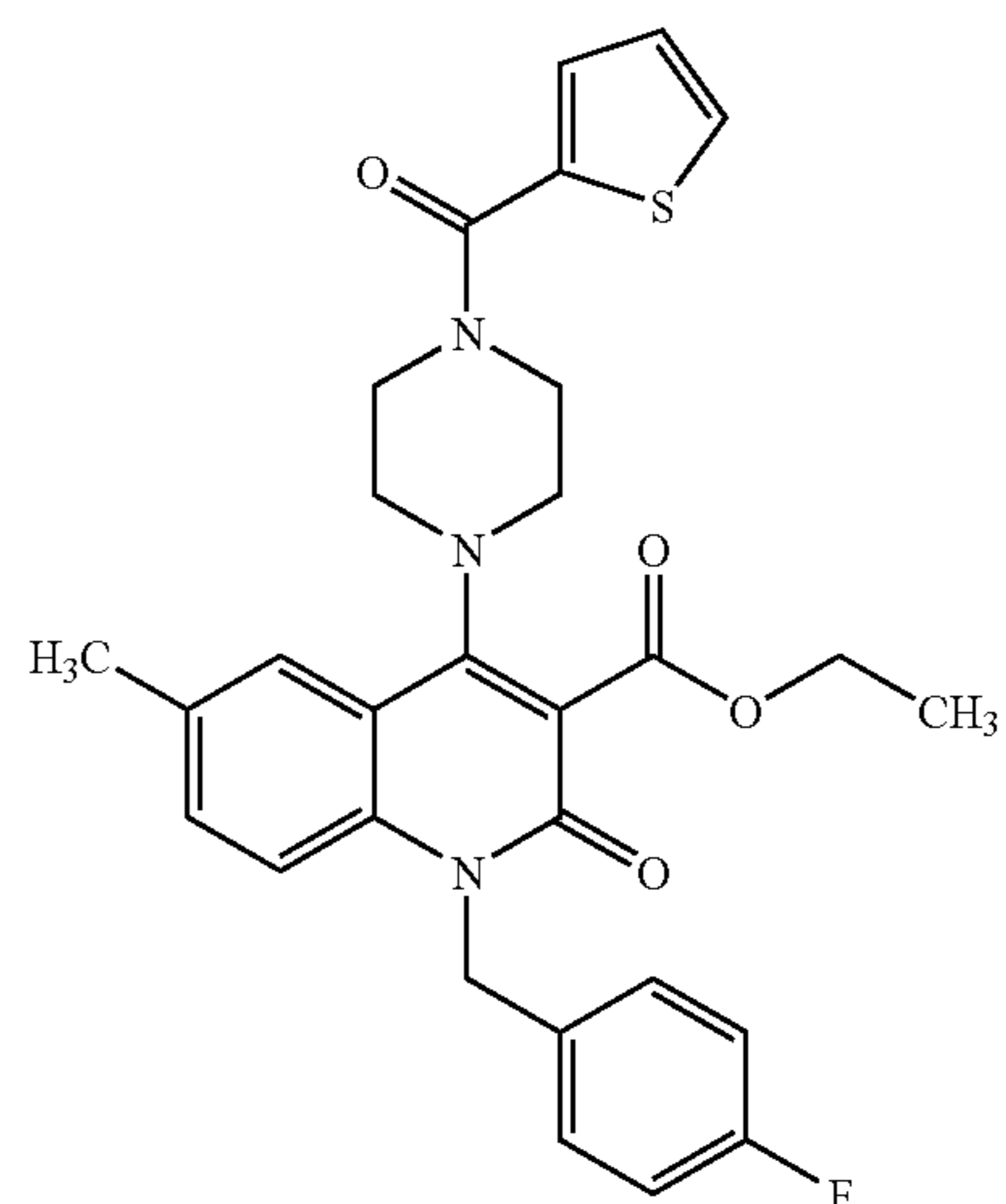
Compound 51
