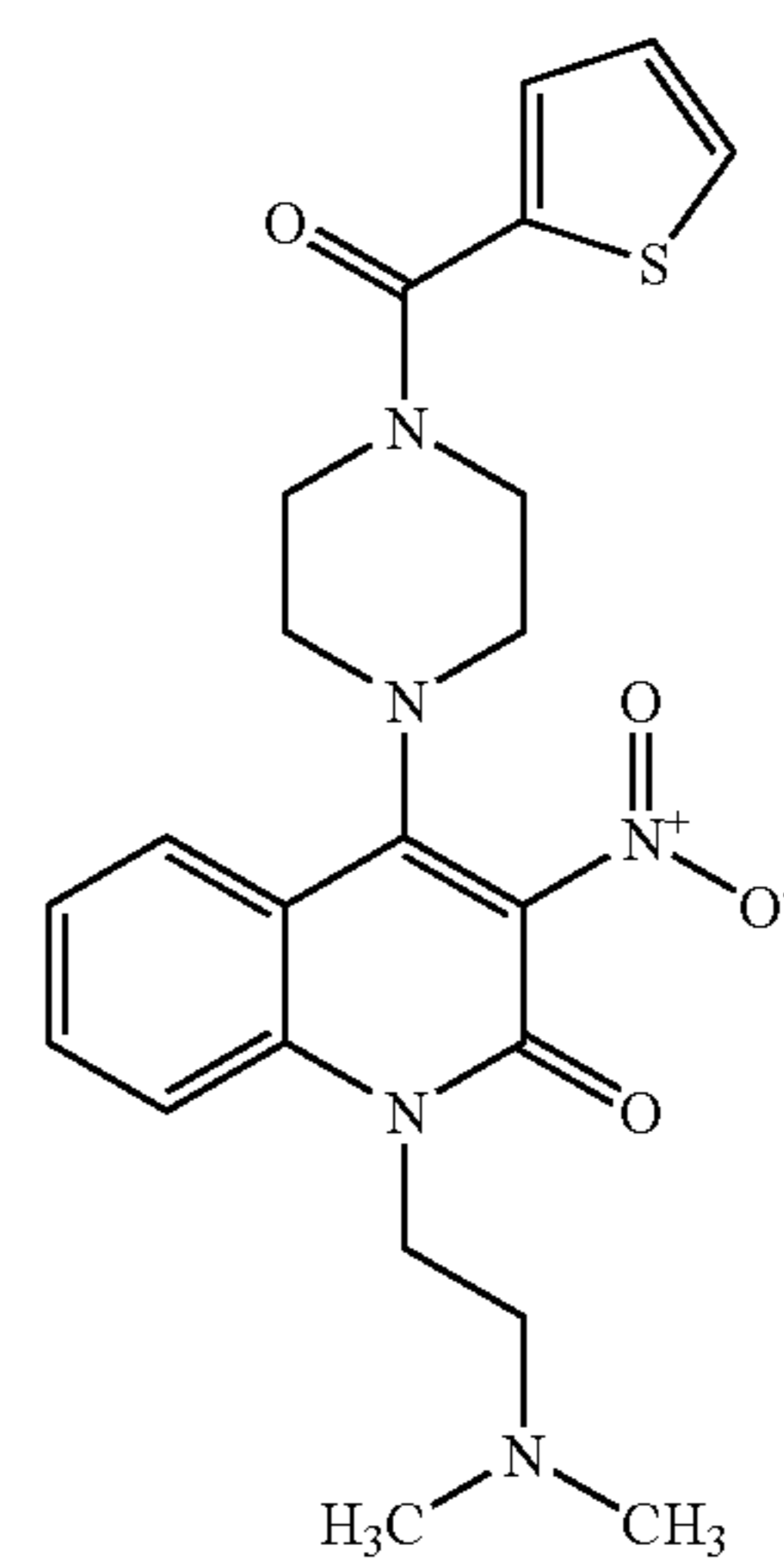
Compound 170
