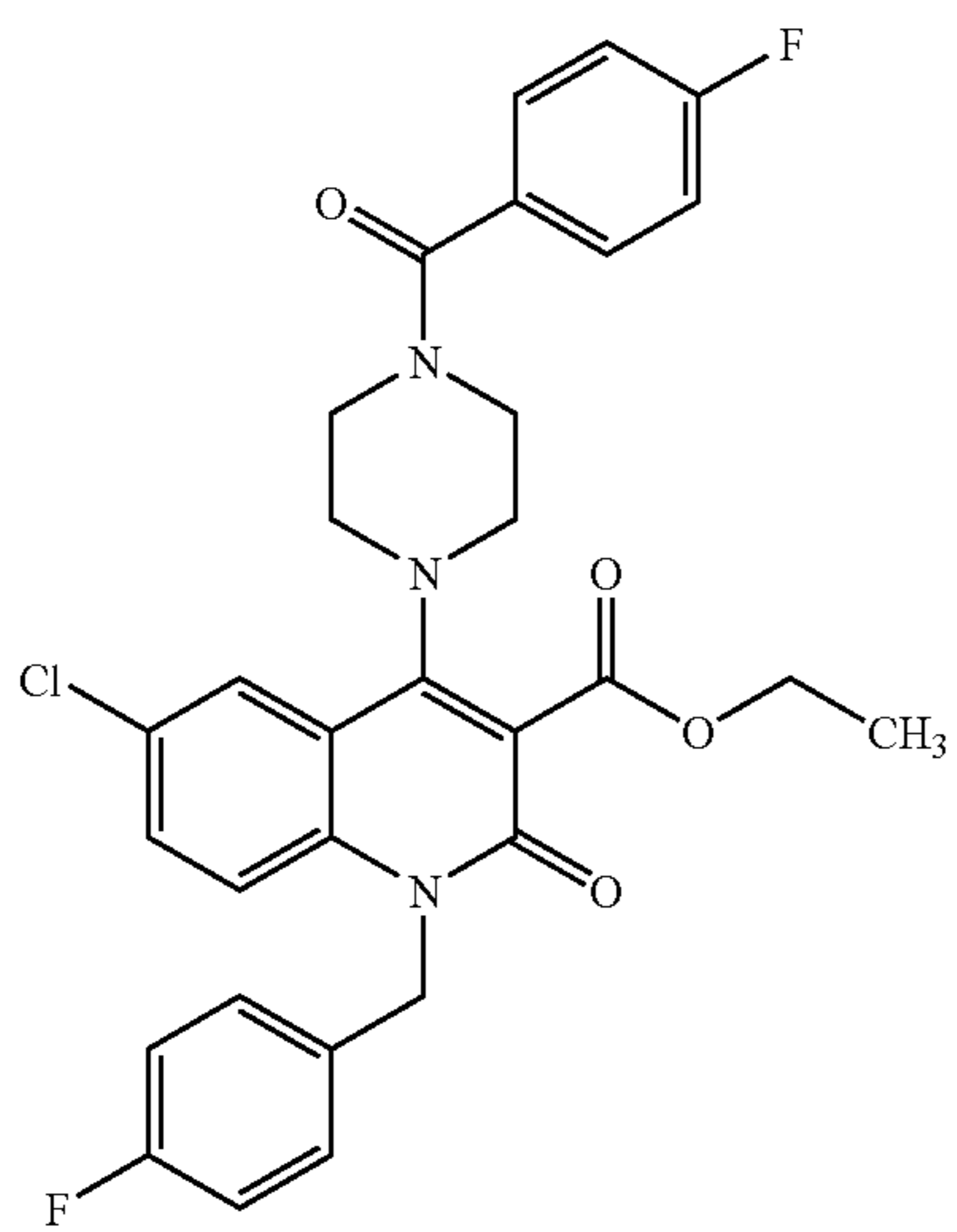
Compound 41
