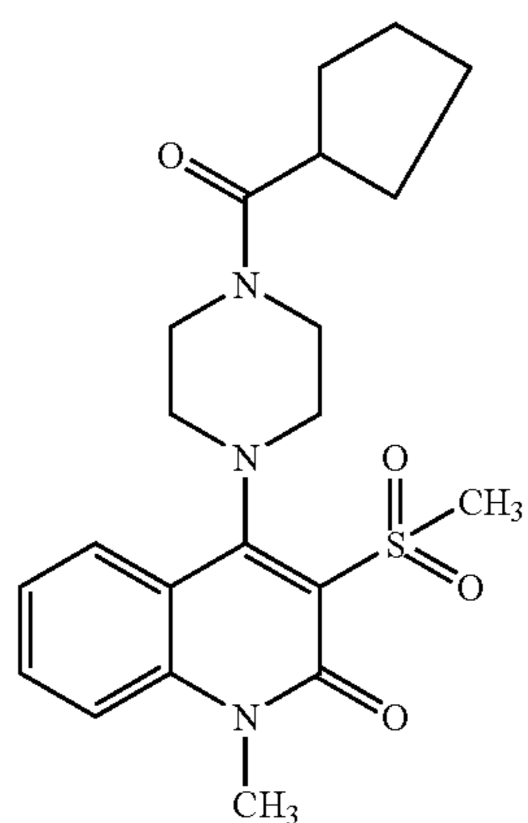
Compound 101
