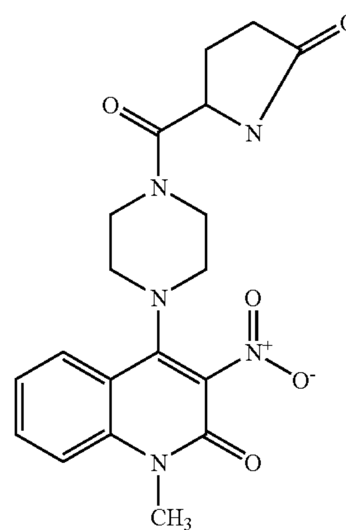
Compound 303
