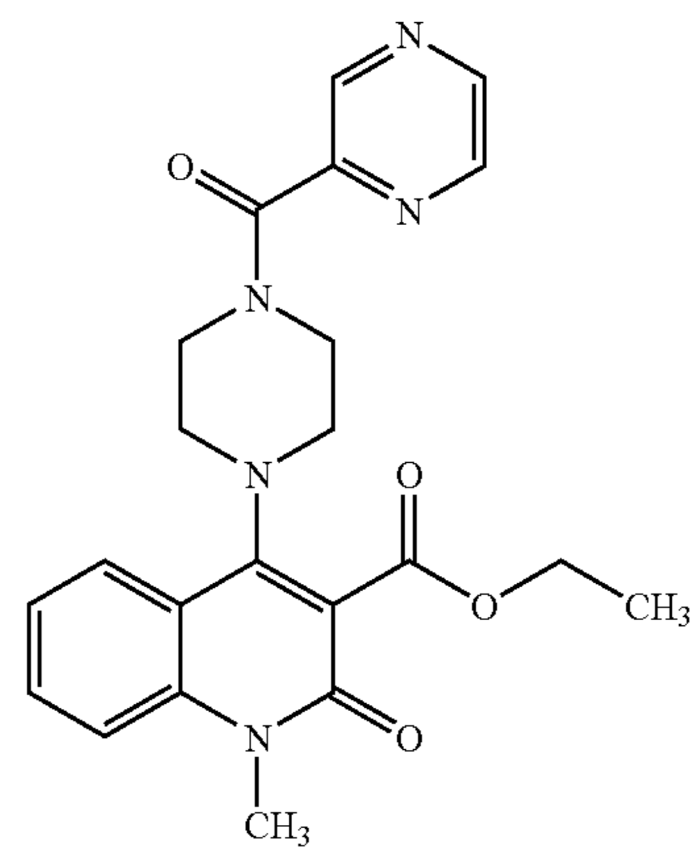
Compound 301
