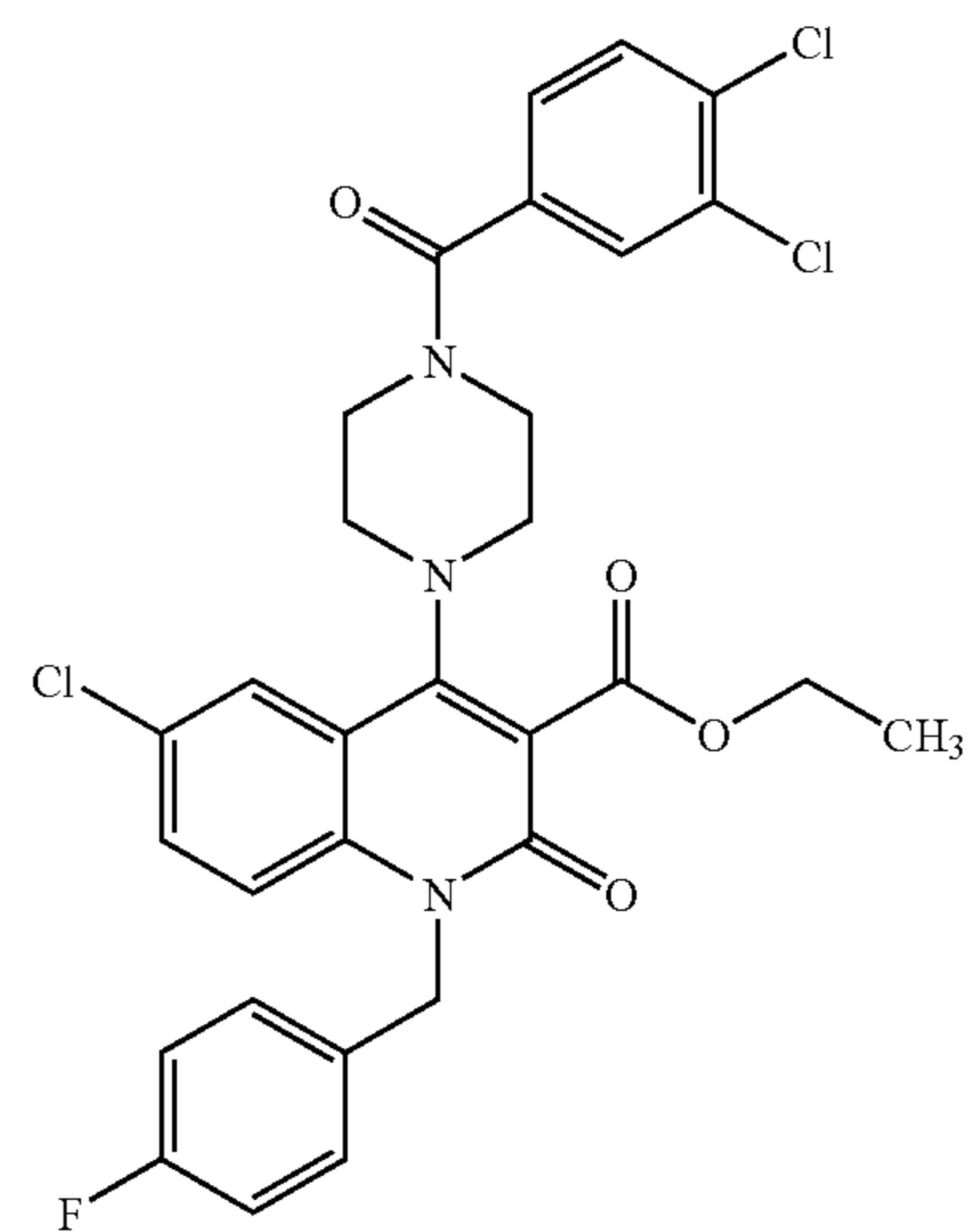
Compound 43
