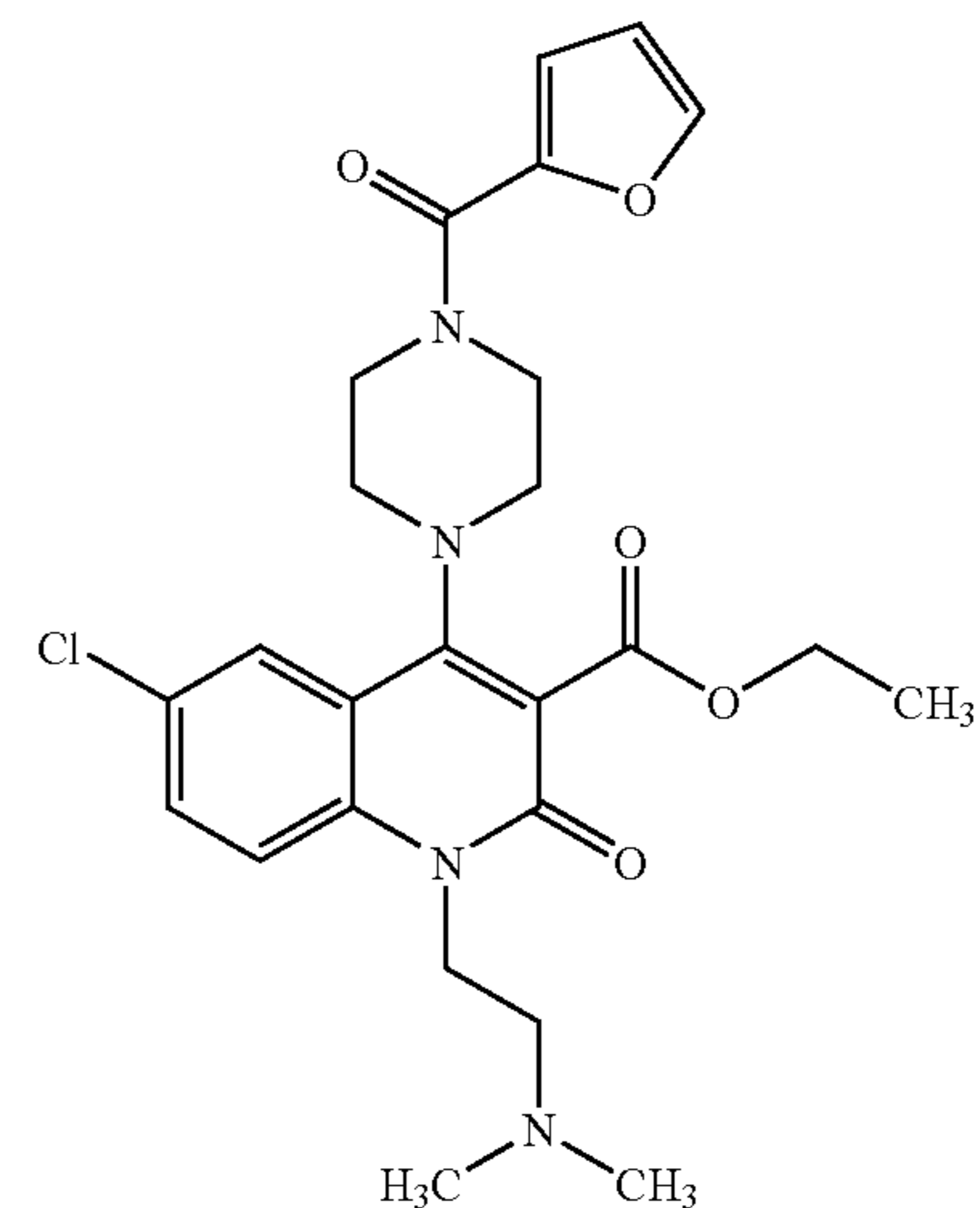
Compound 111
