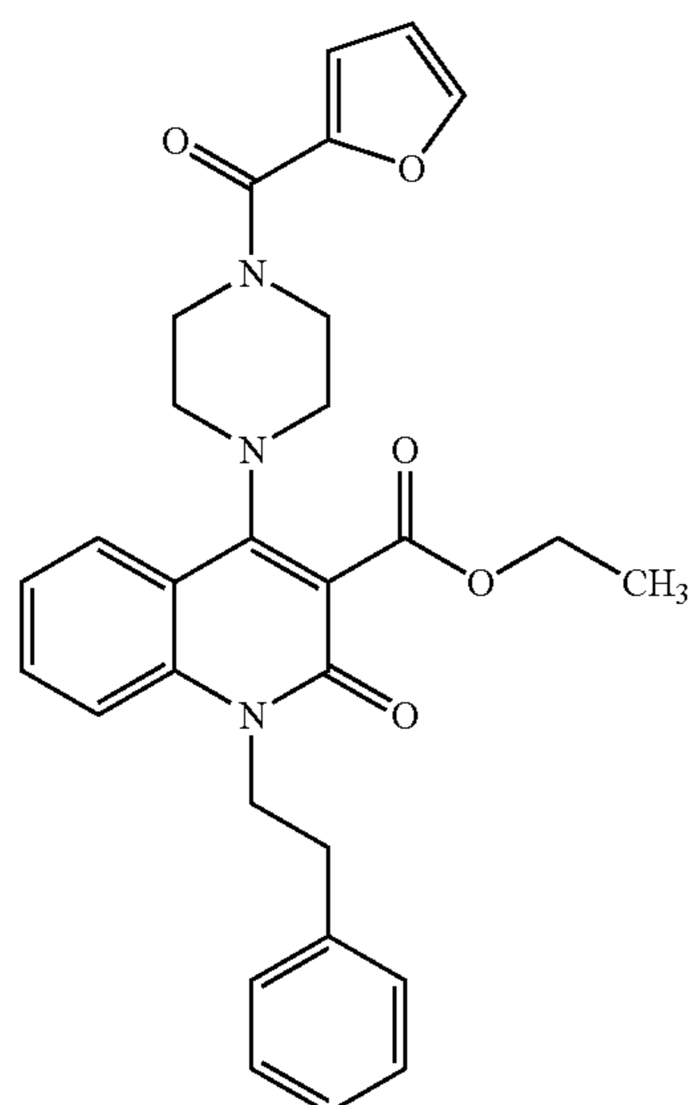
Compound 294
