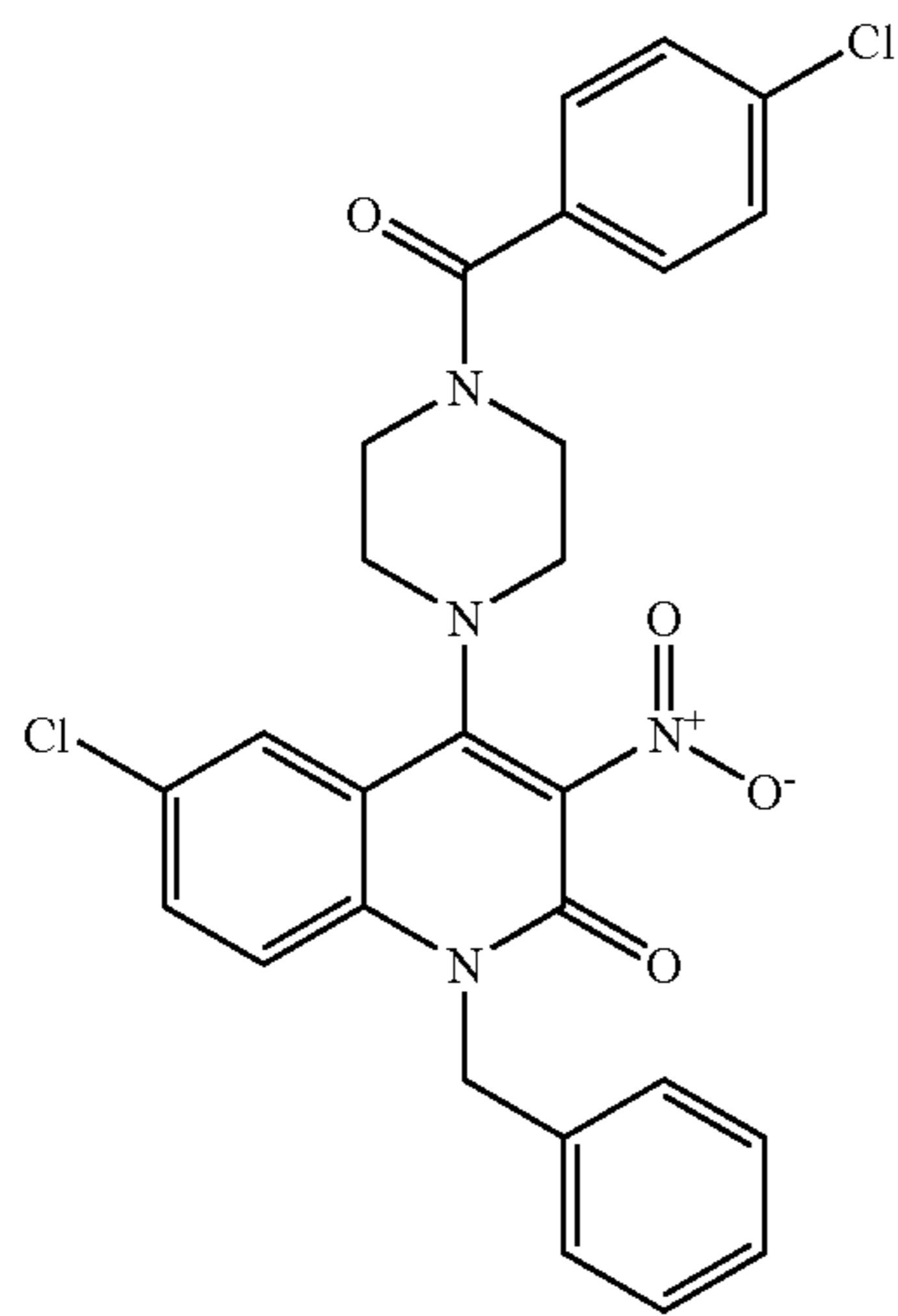
Compound 166
