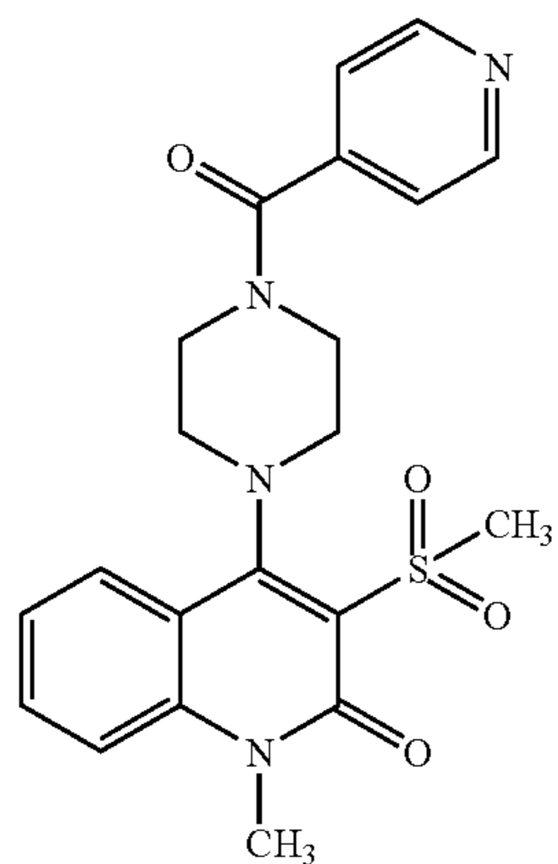
Compound 100
