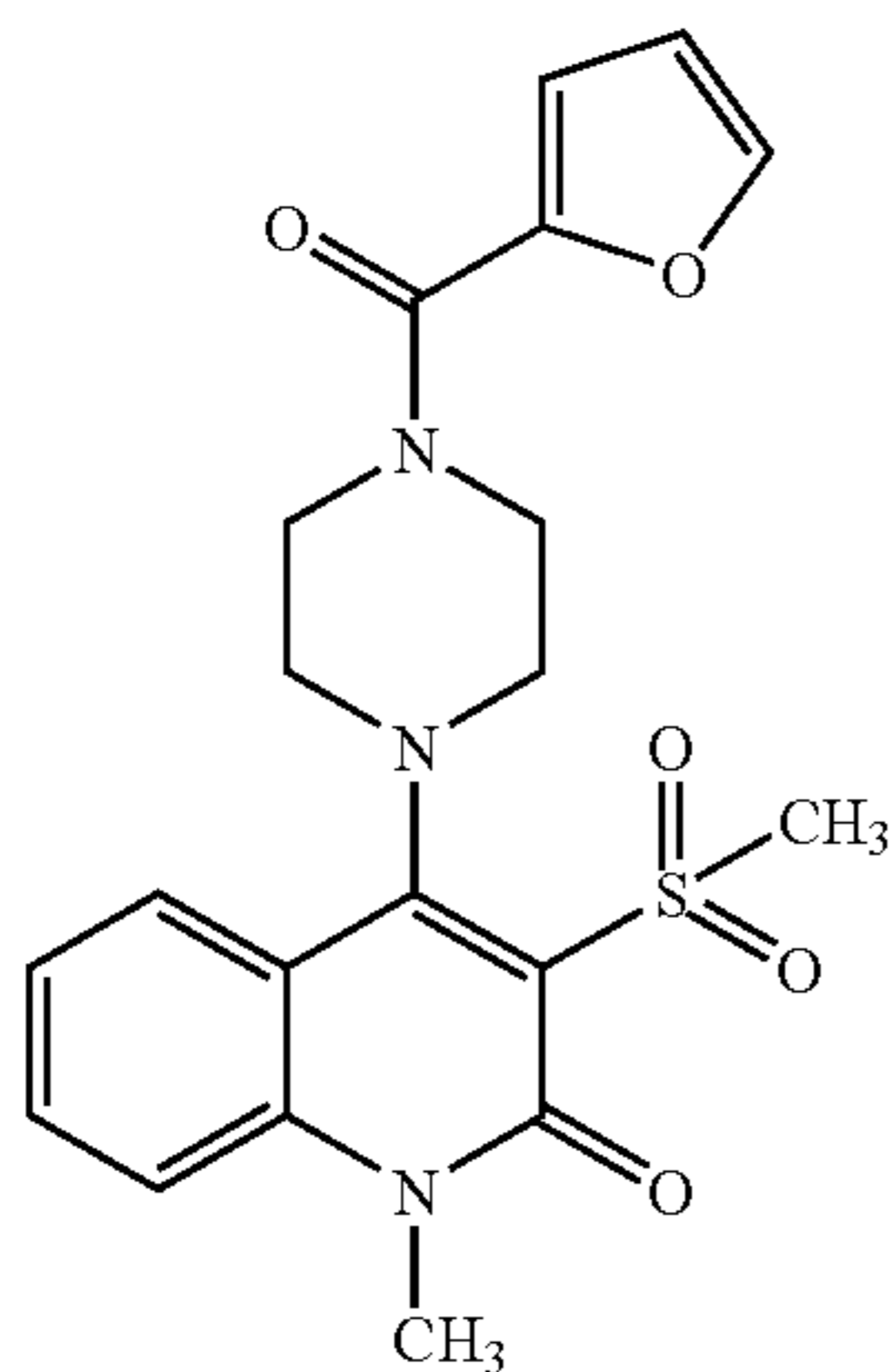
Compound 78
