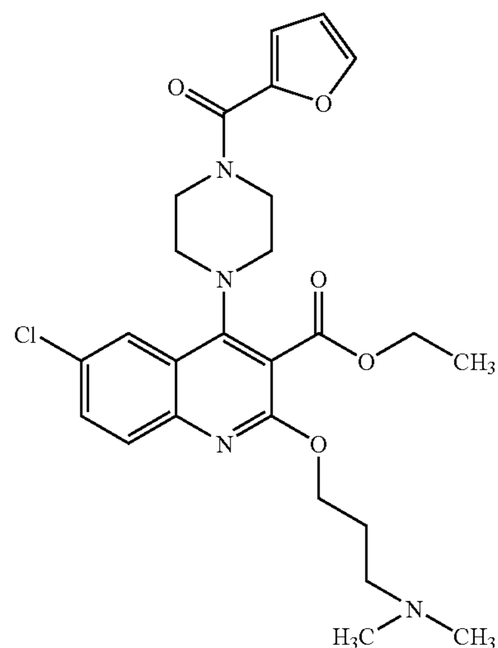
Compound 330
