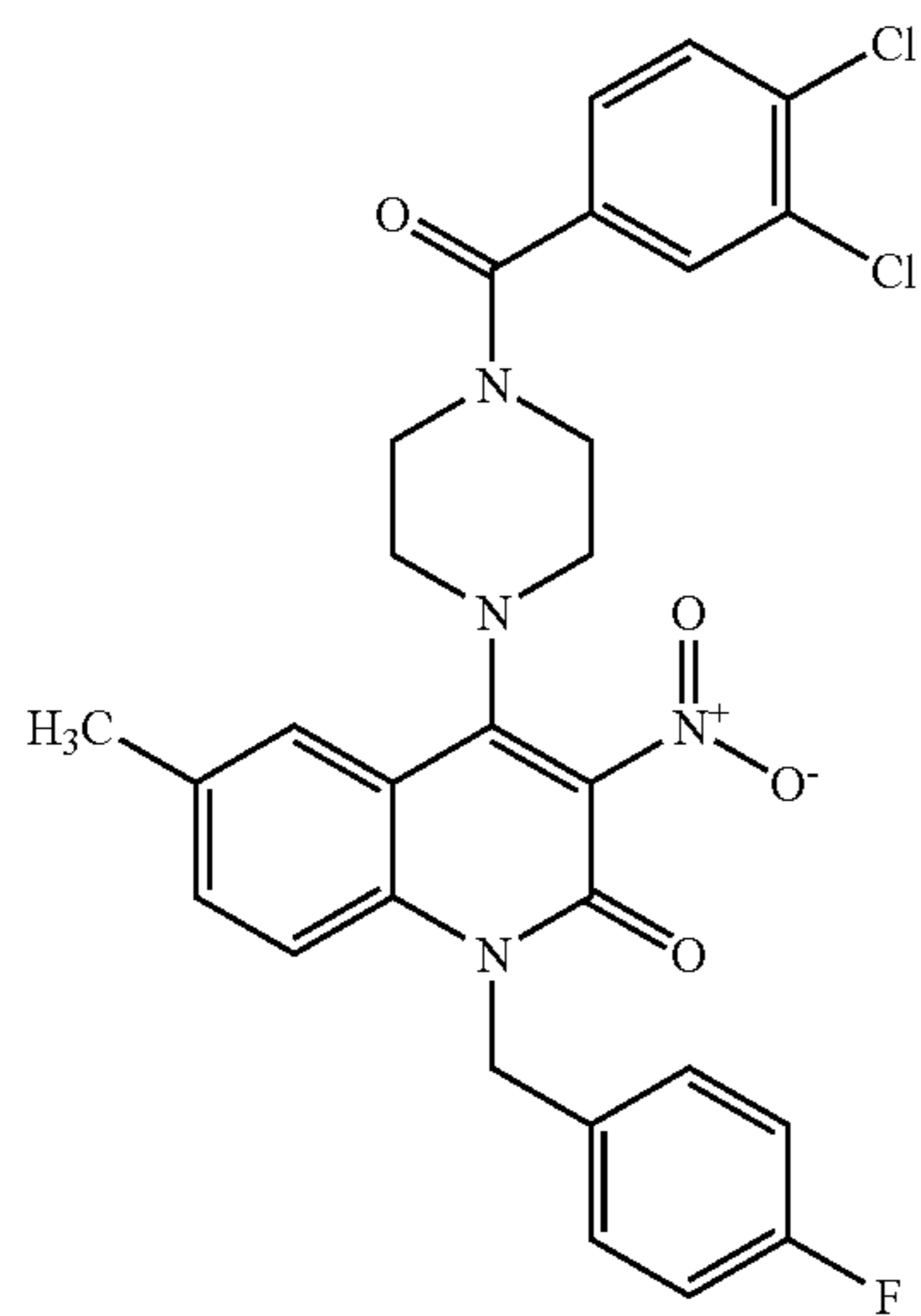
Compound 190
