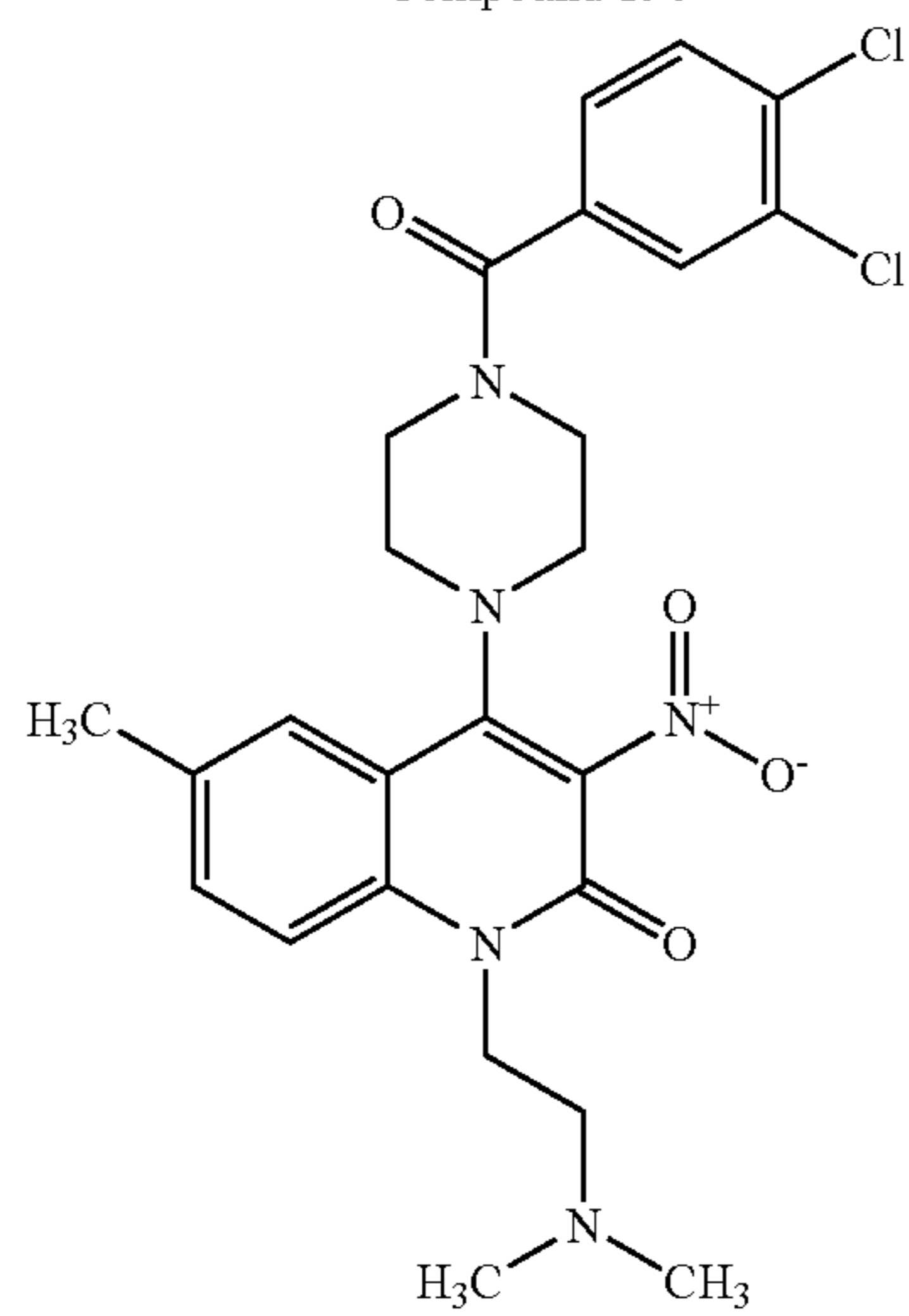
Compound 191
