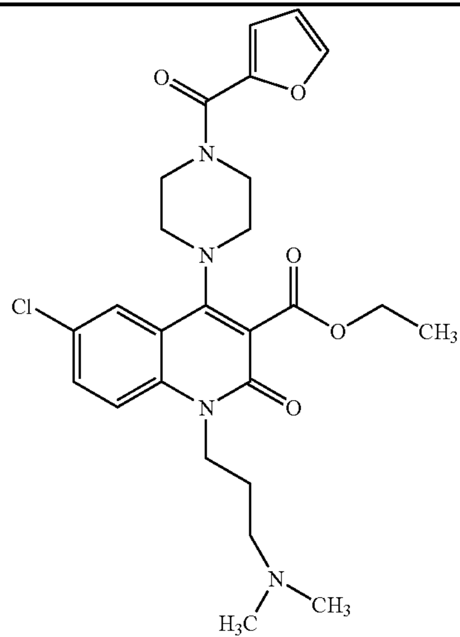
Compound 91
