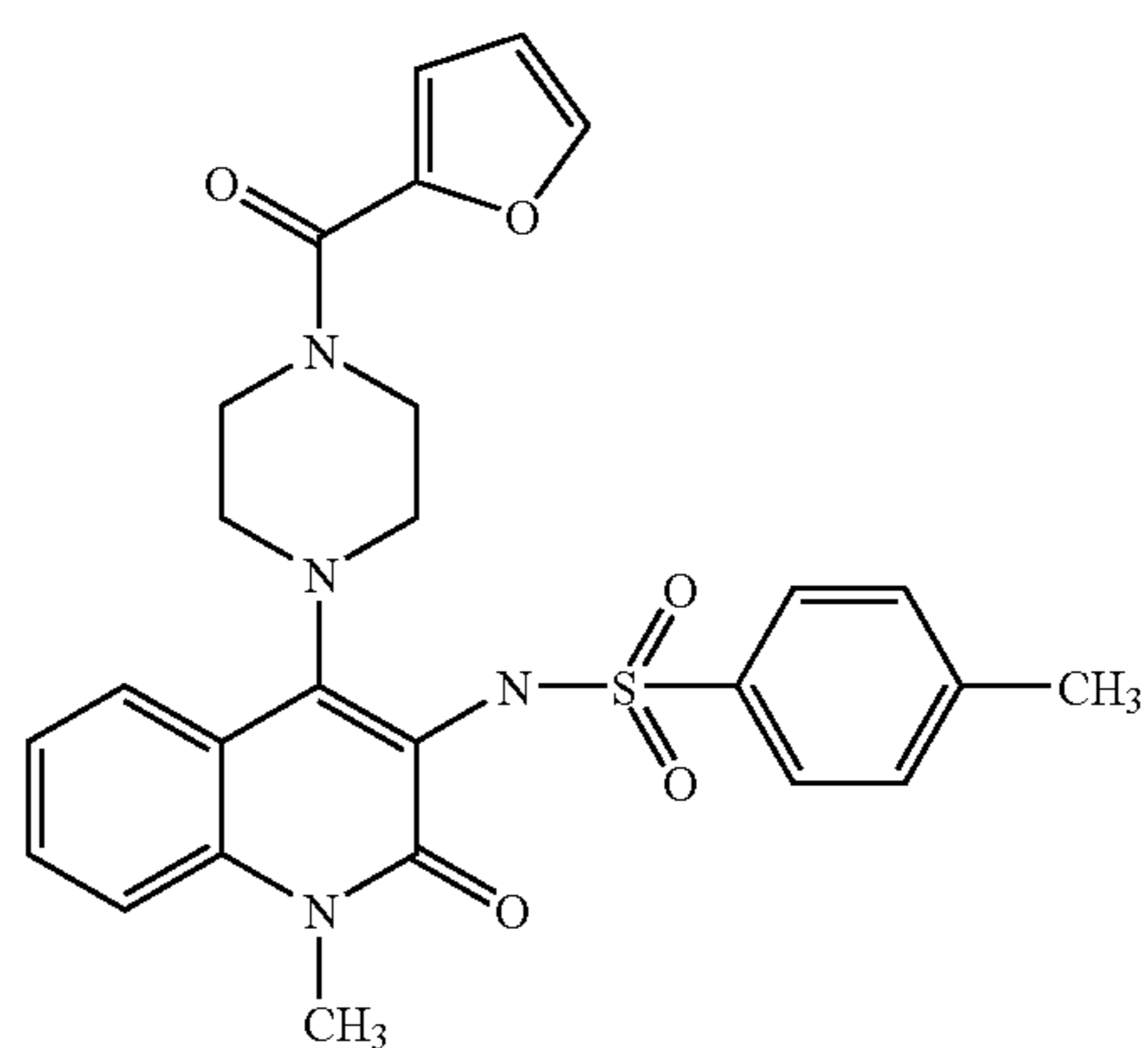
Compound 80
