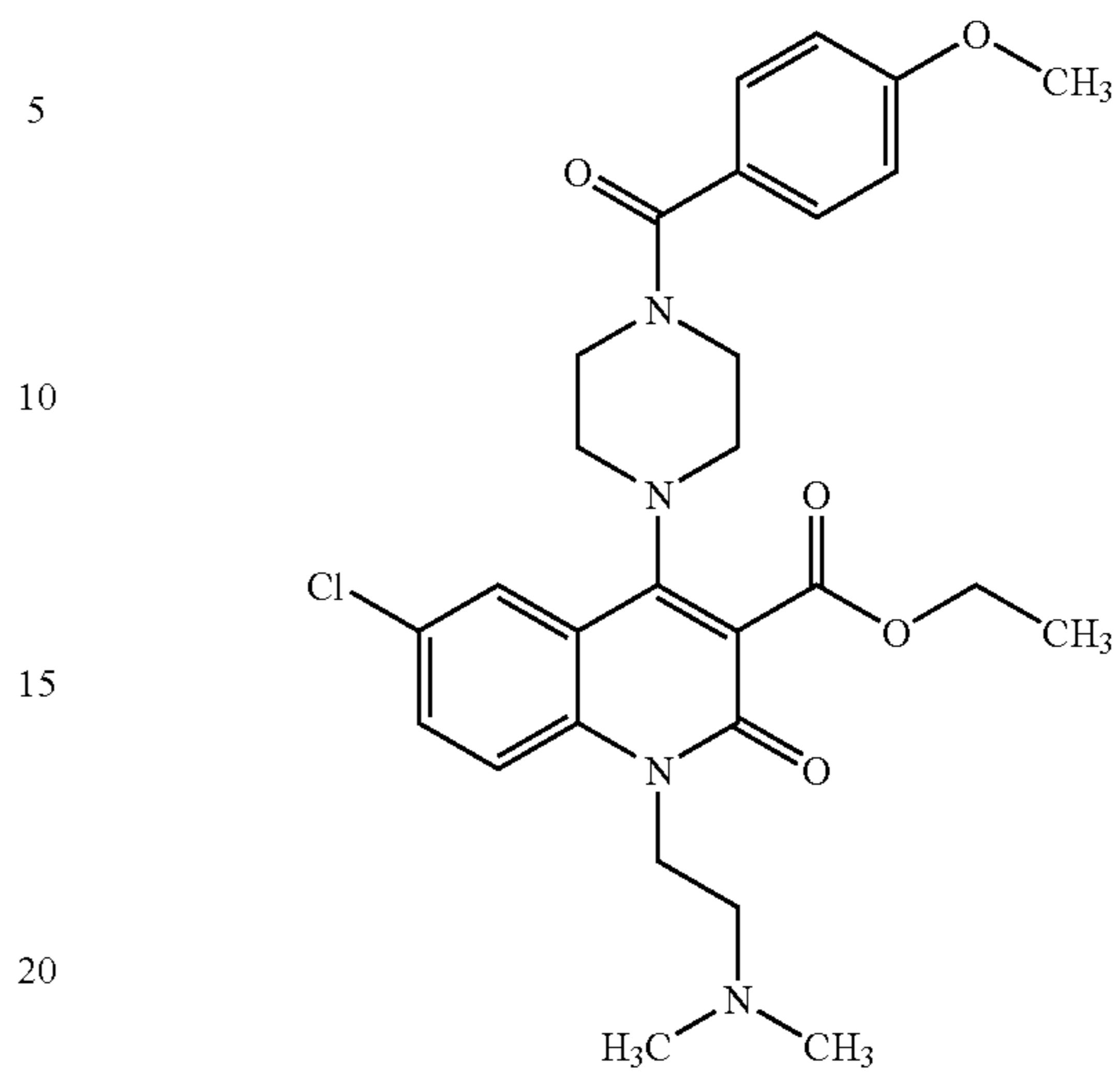
Compound 157
