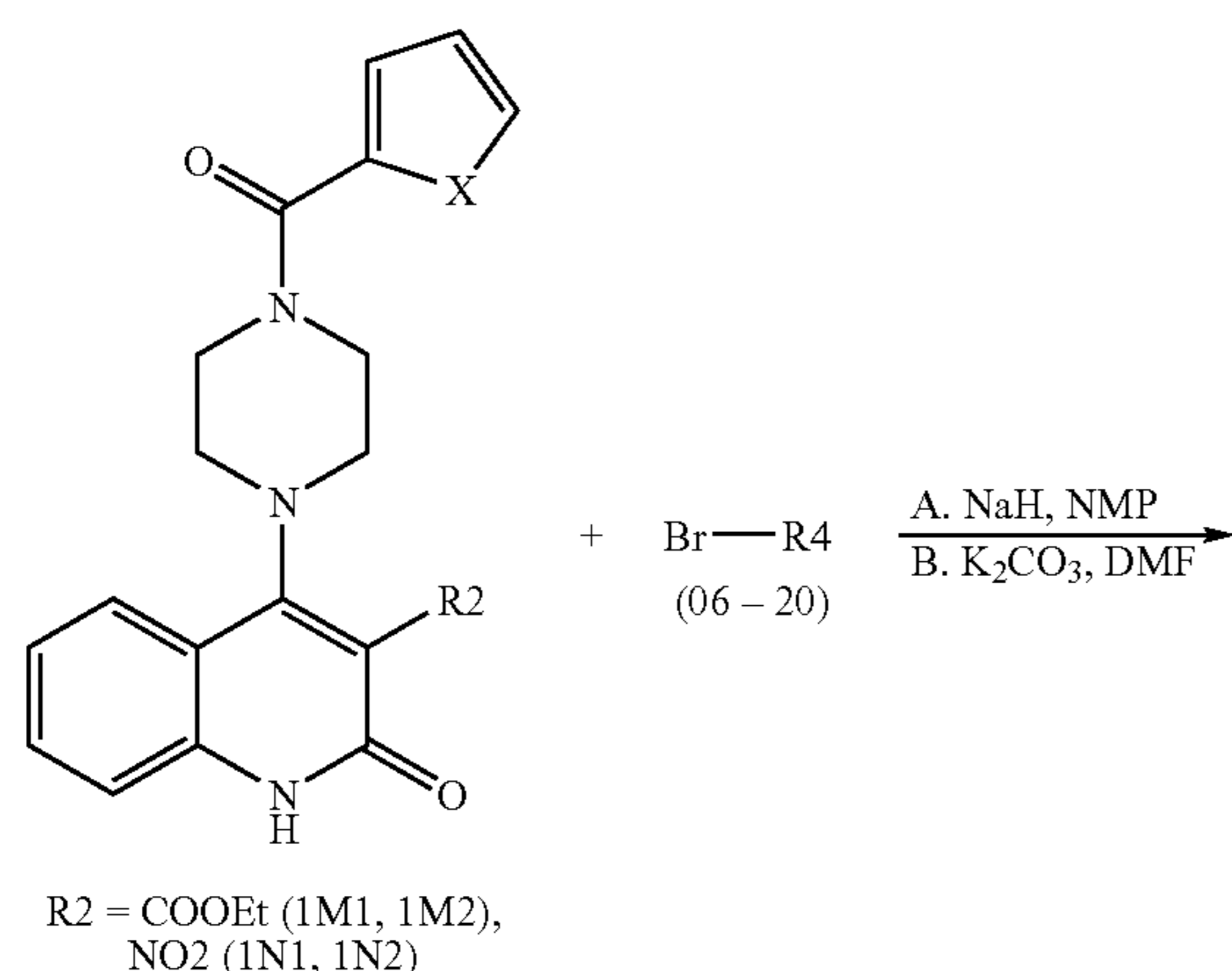
Reaction Scheme 13
