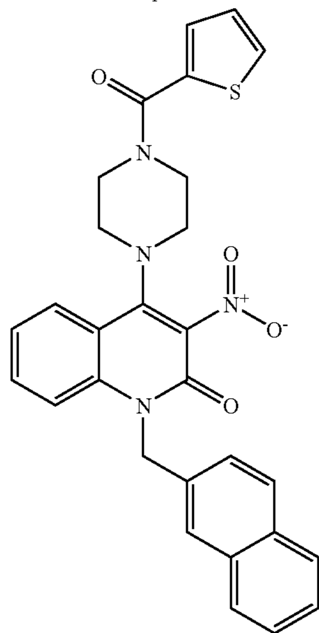
Compound 282
