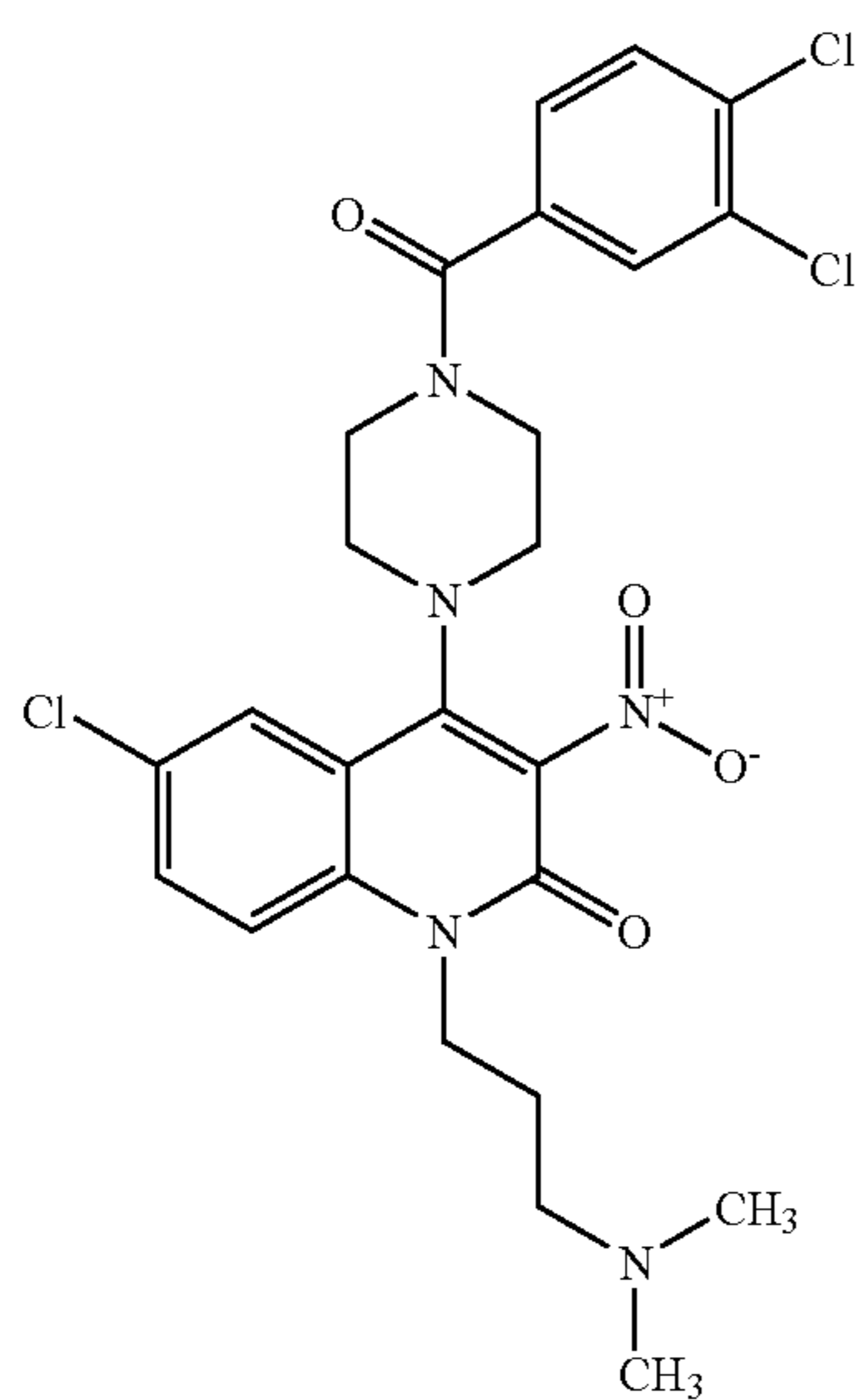
Compound 210
