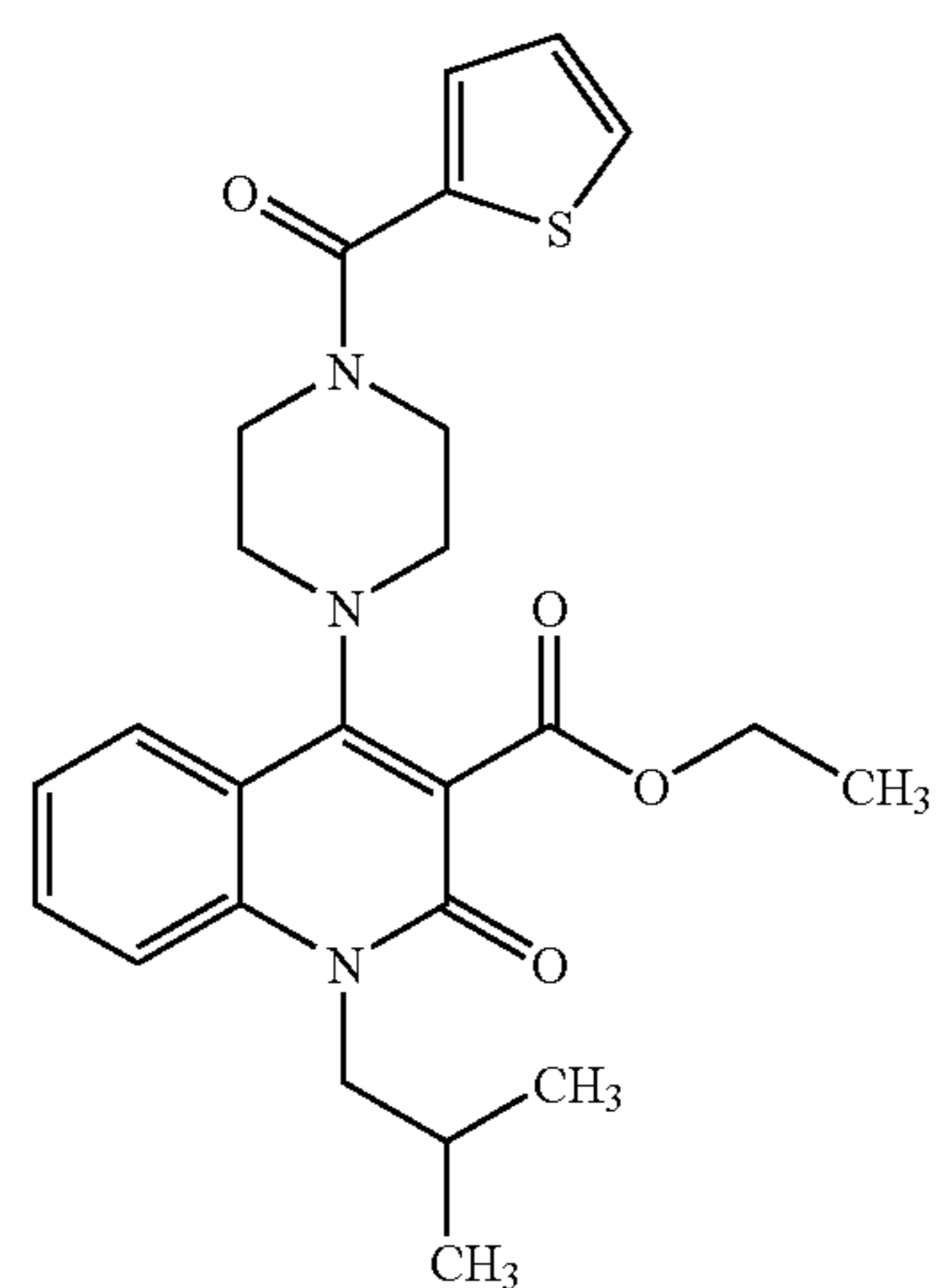
Compound 297
