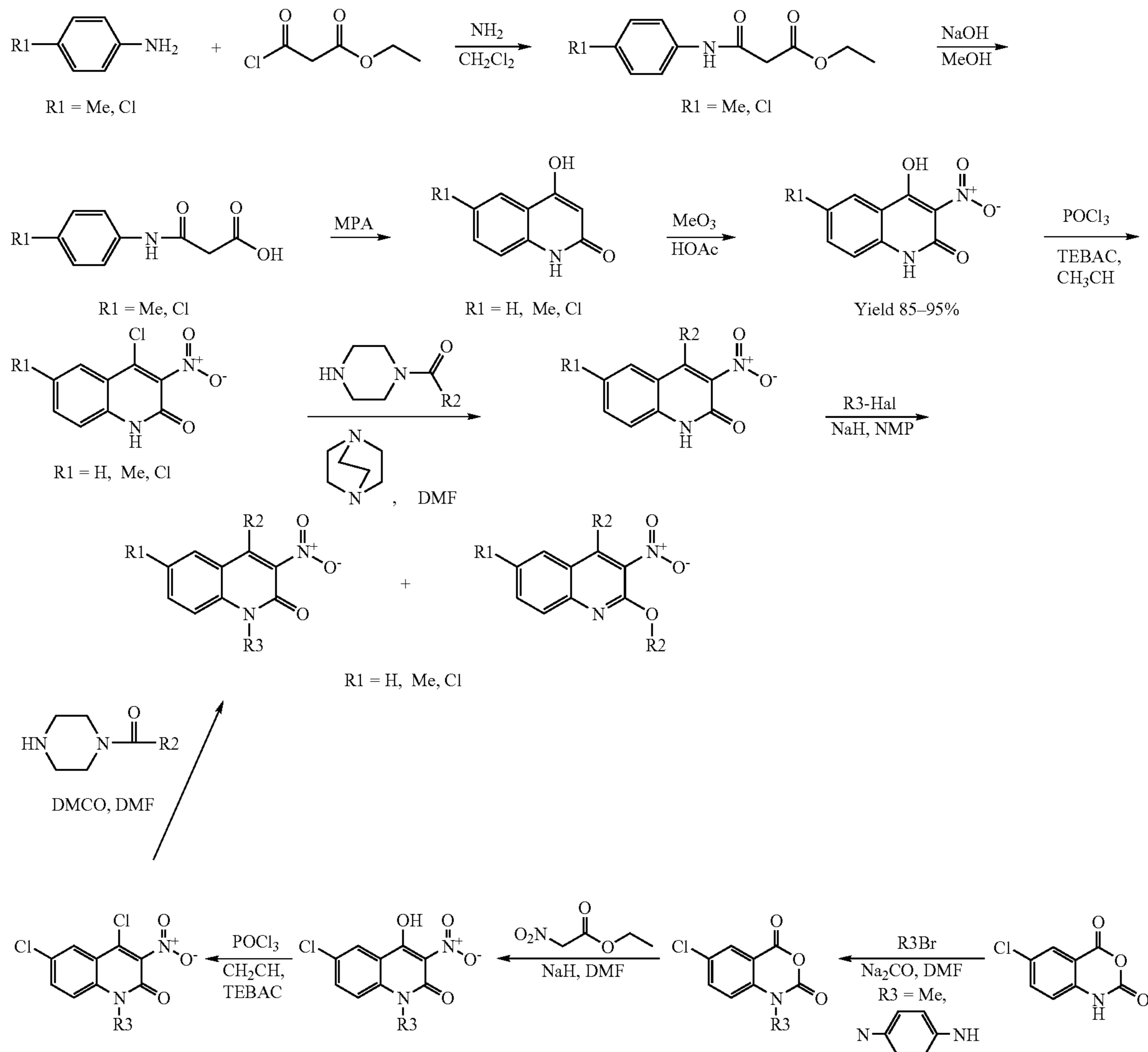
Reaction Scheme 22
