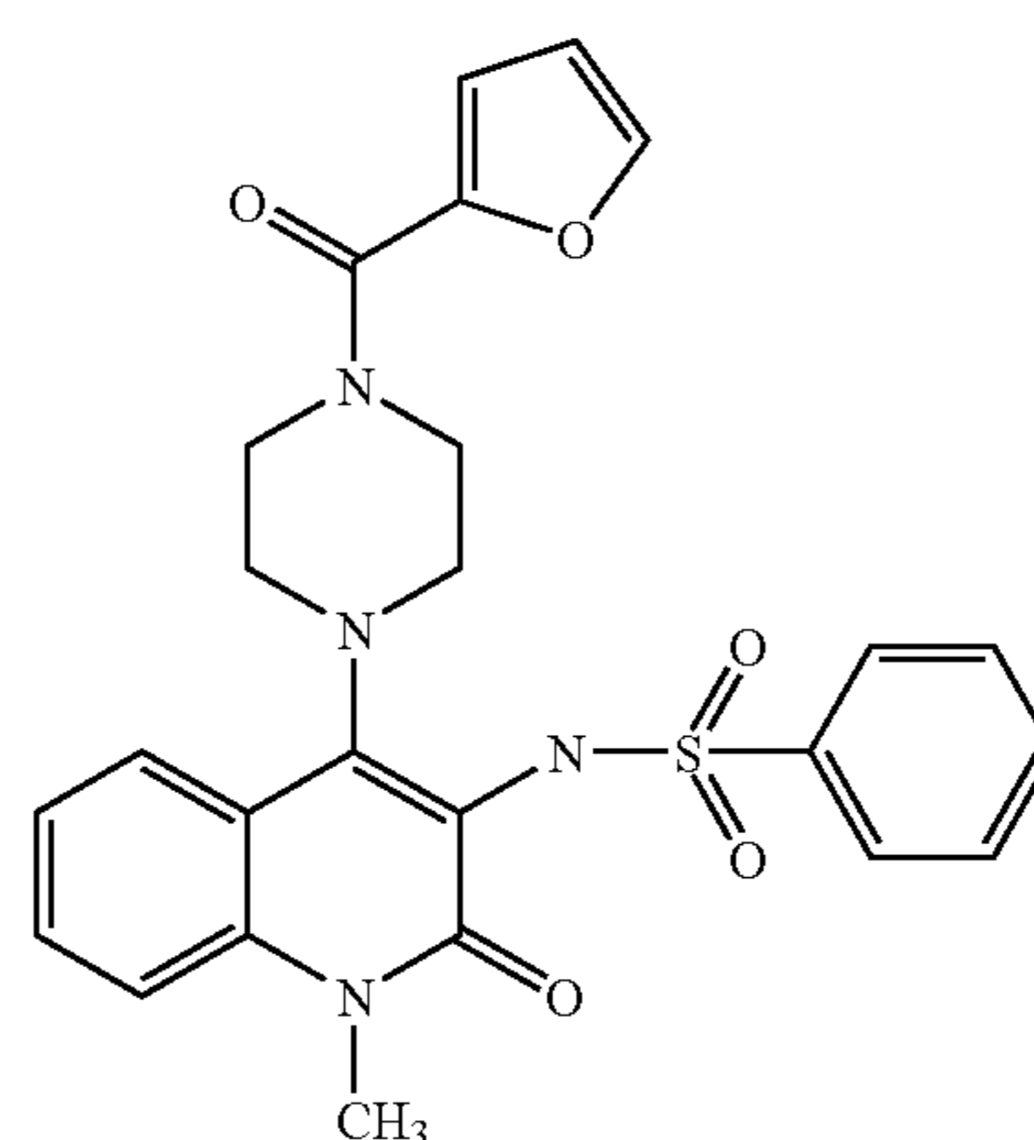
Compound 81
