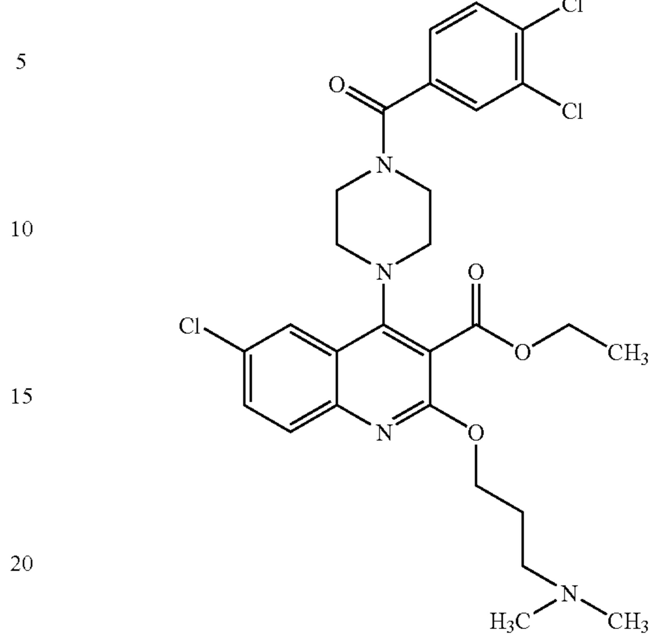
Compound 334
