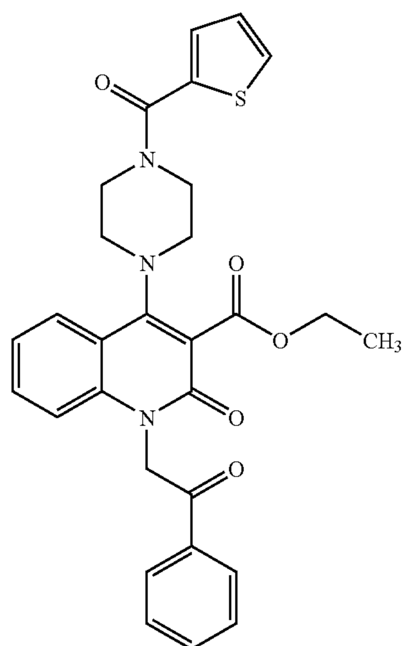
Compound 299
