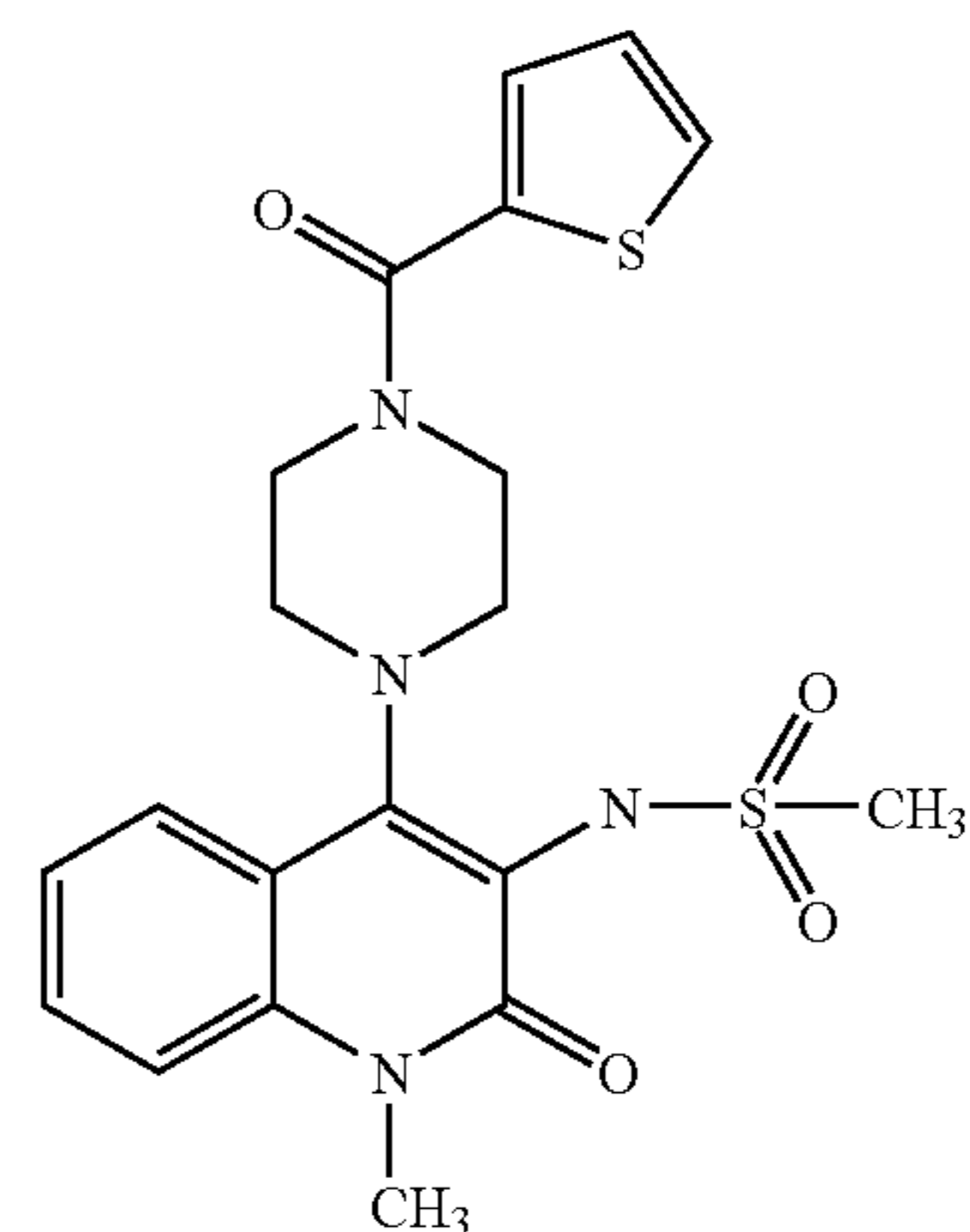
Compound 45
