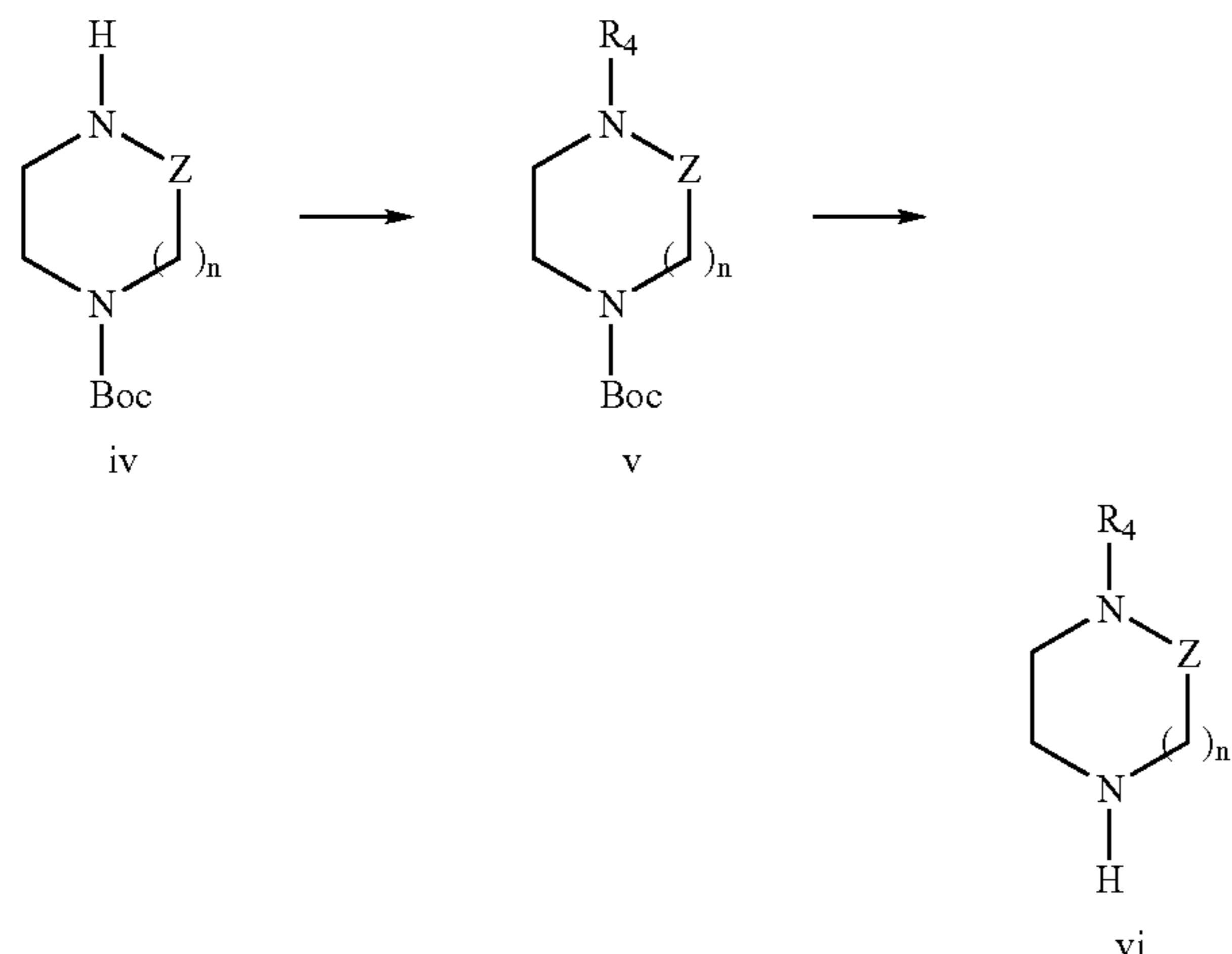
Reaction Scheme 2
