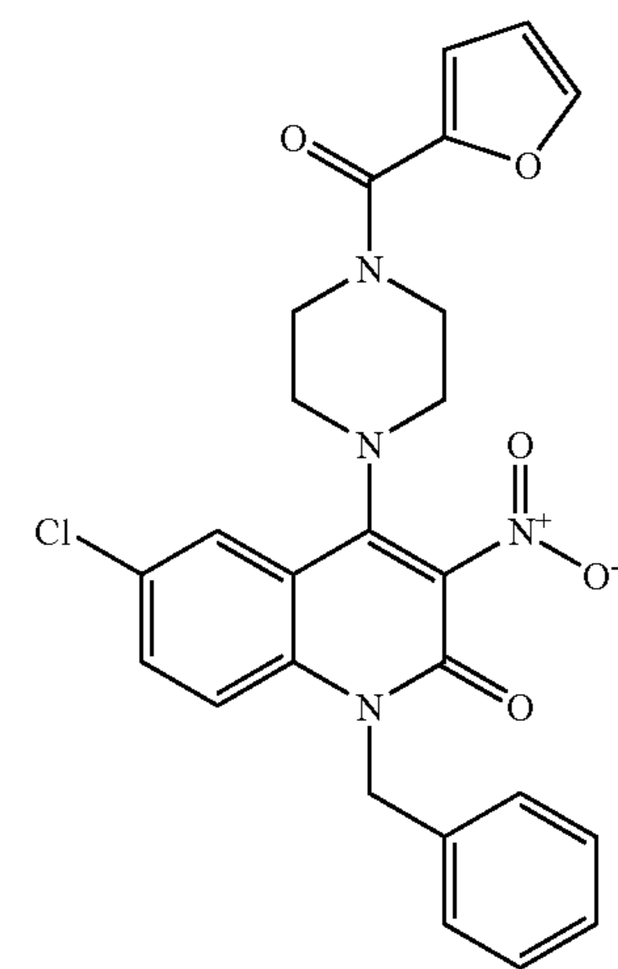
Compound 165
