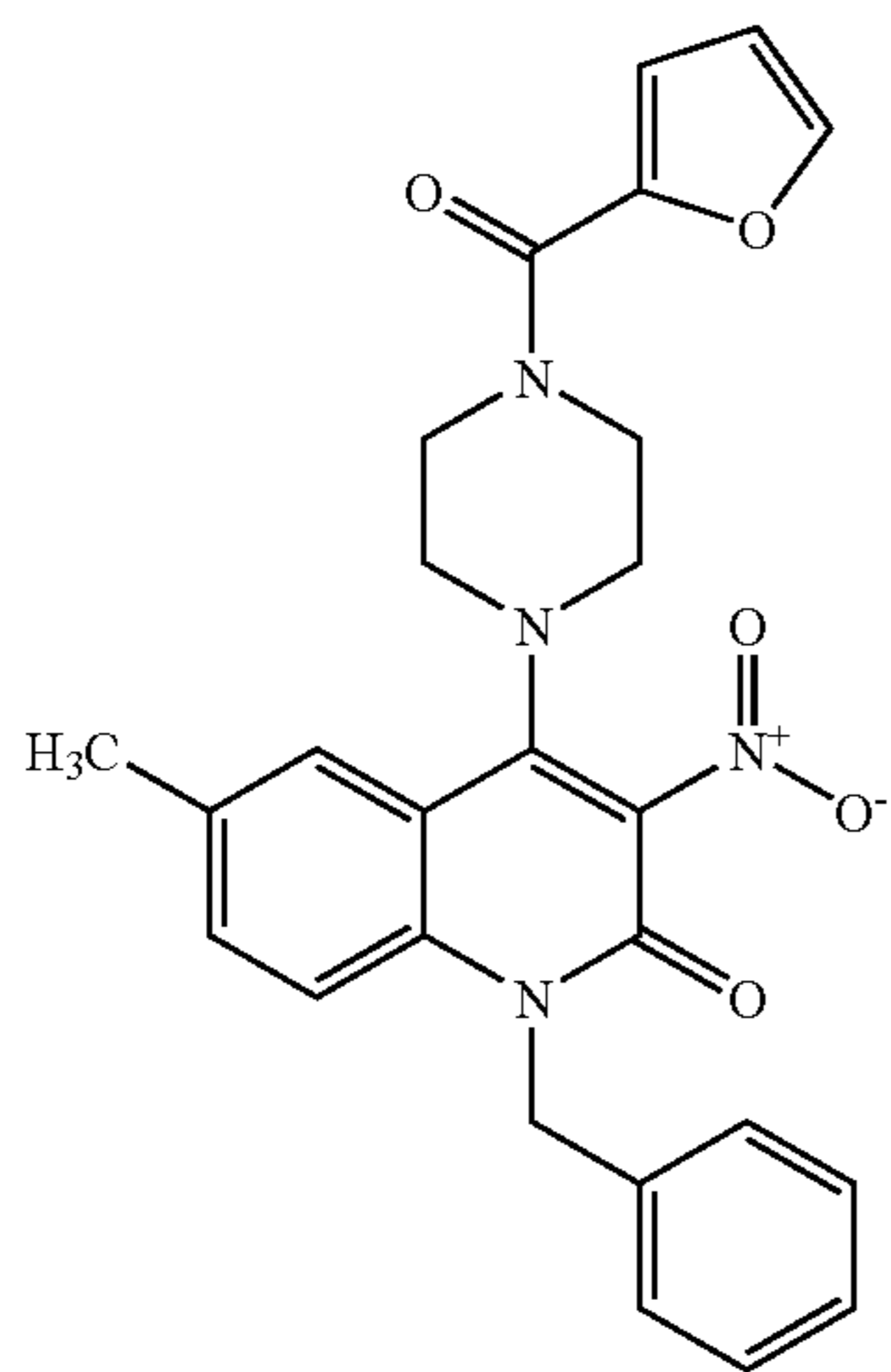
Compound 161
