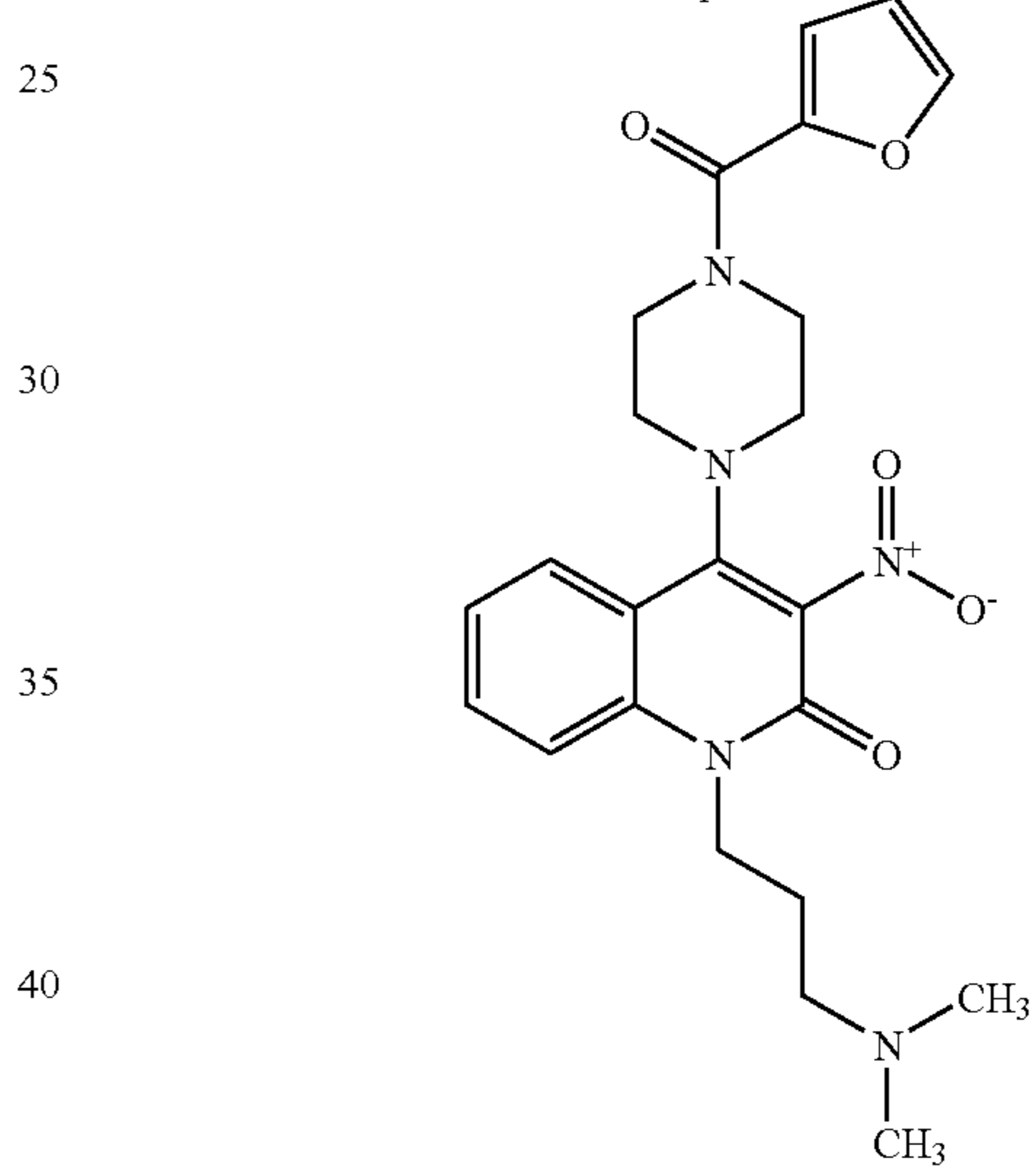
Compound 158
