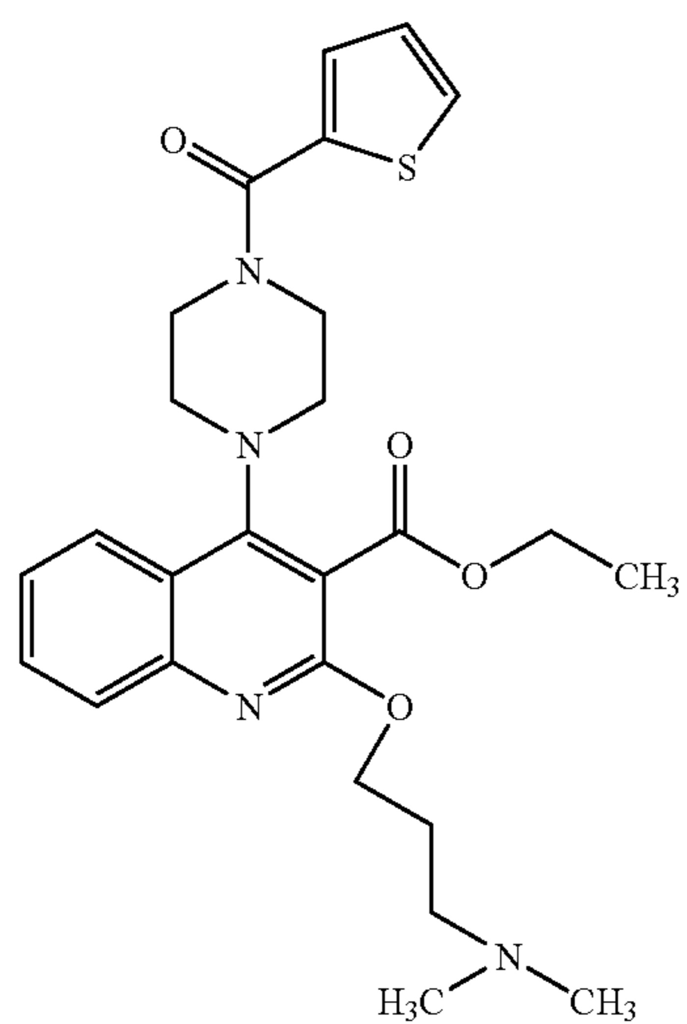
Compound 333
