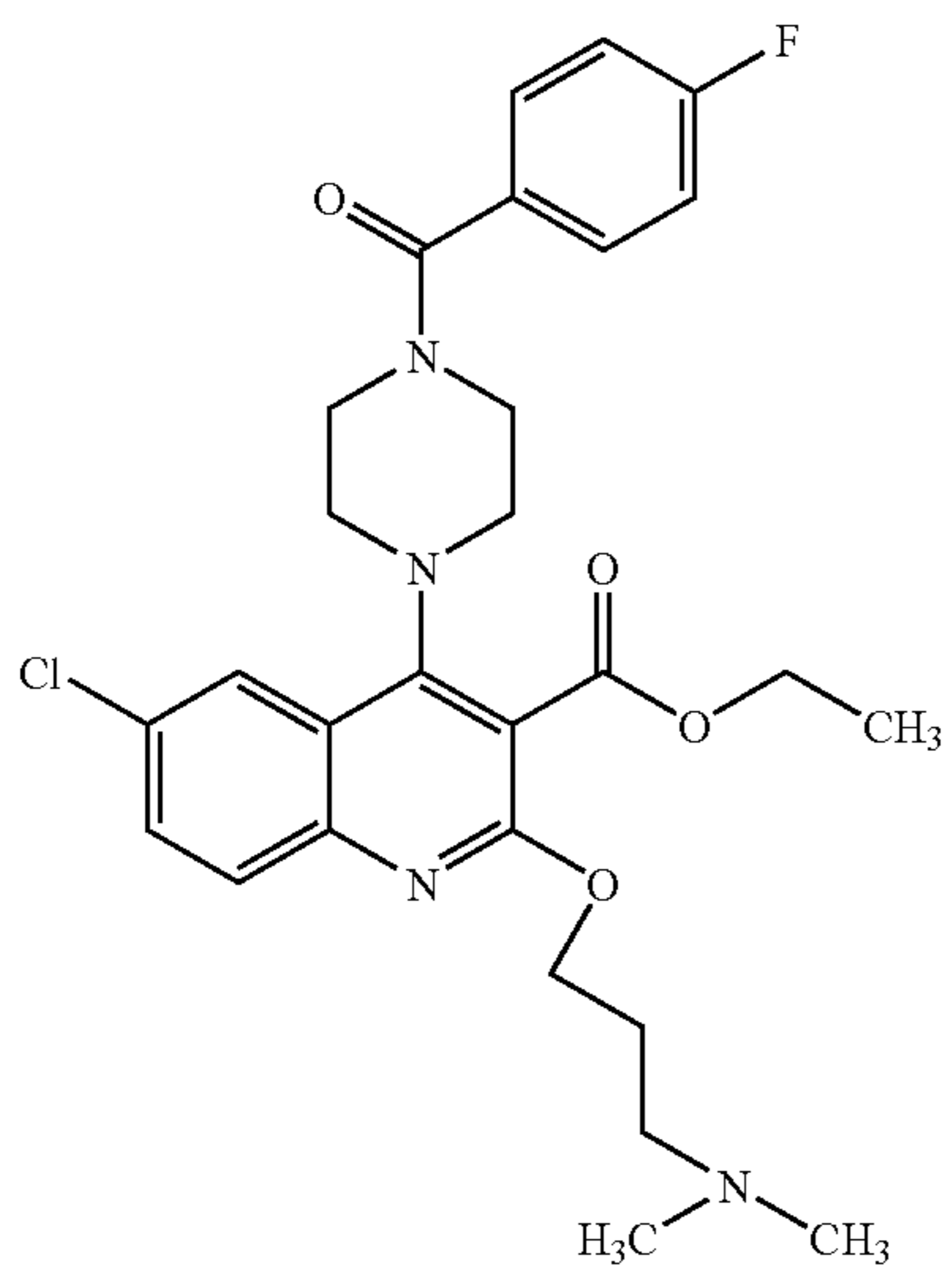
Compound 331
