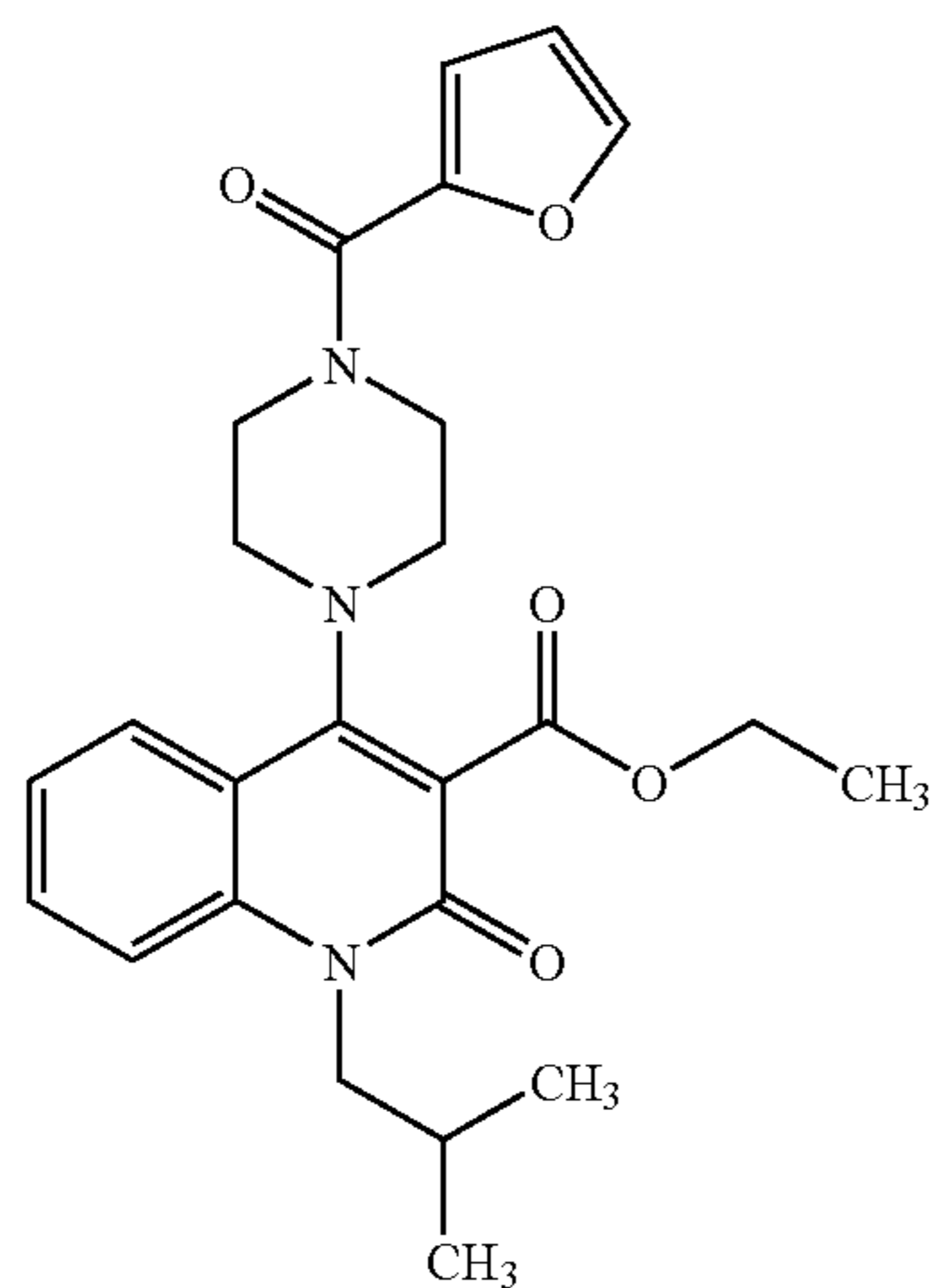
Compound 232
