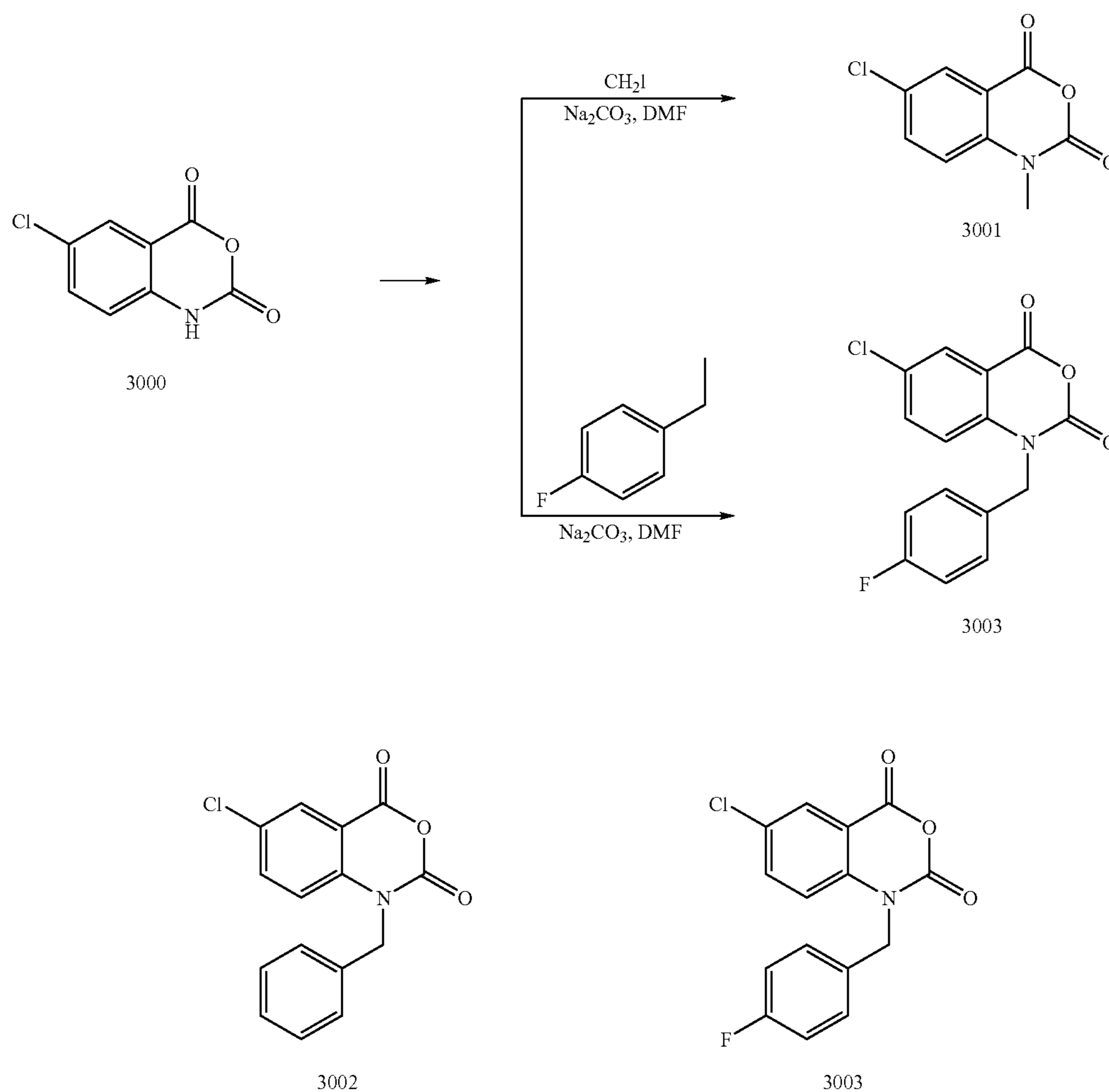
Reaction Scheme 26
