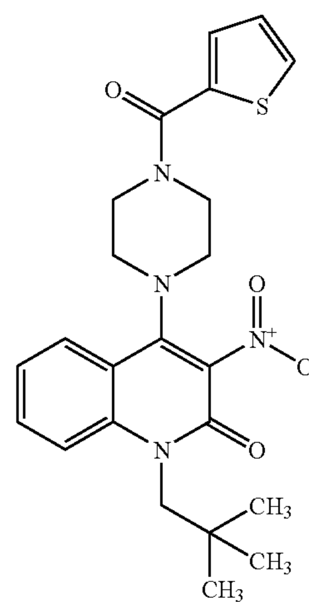
Compound 254
