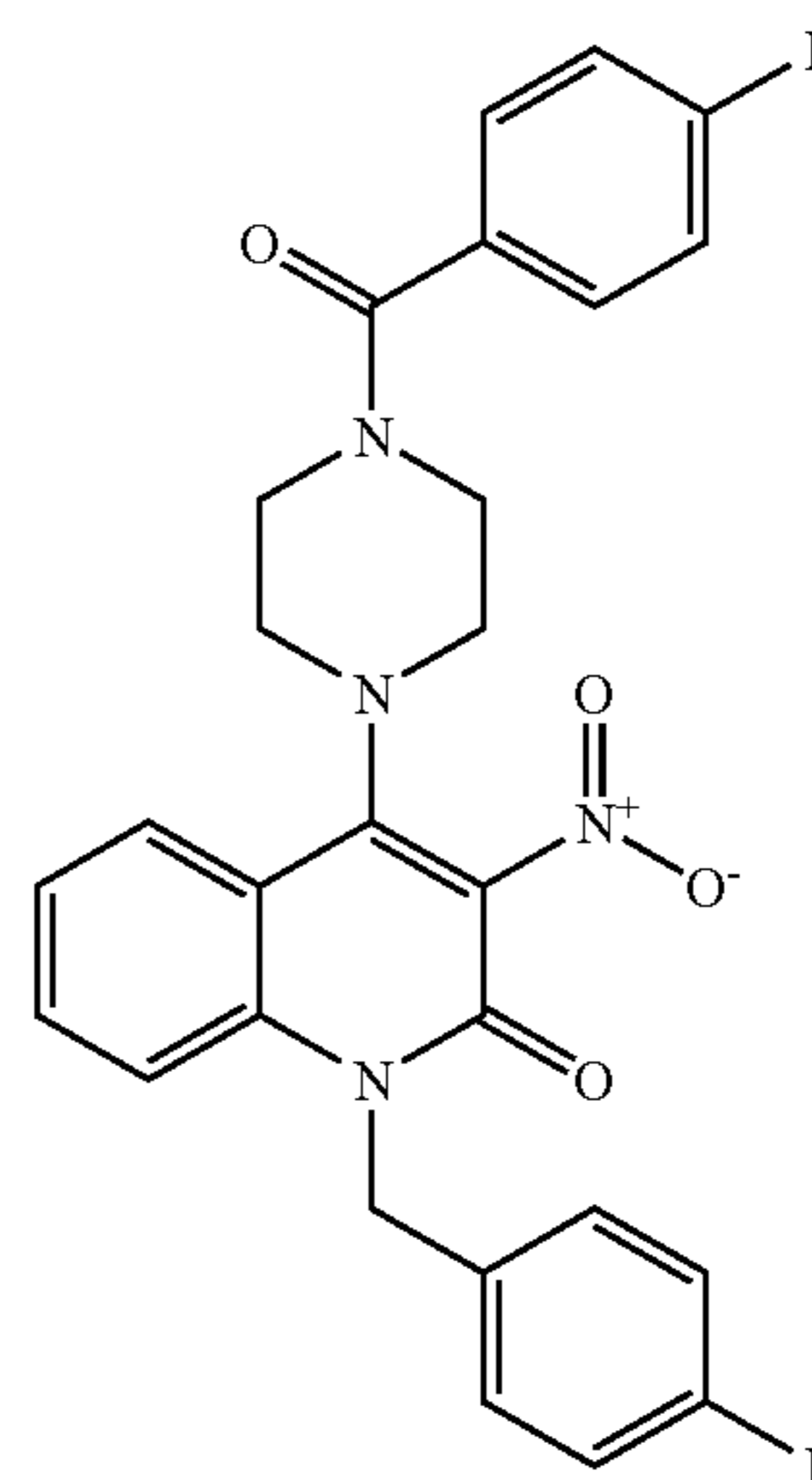
Compound 133
