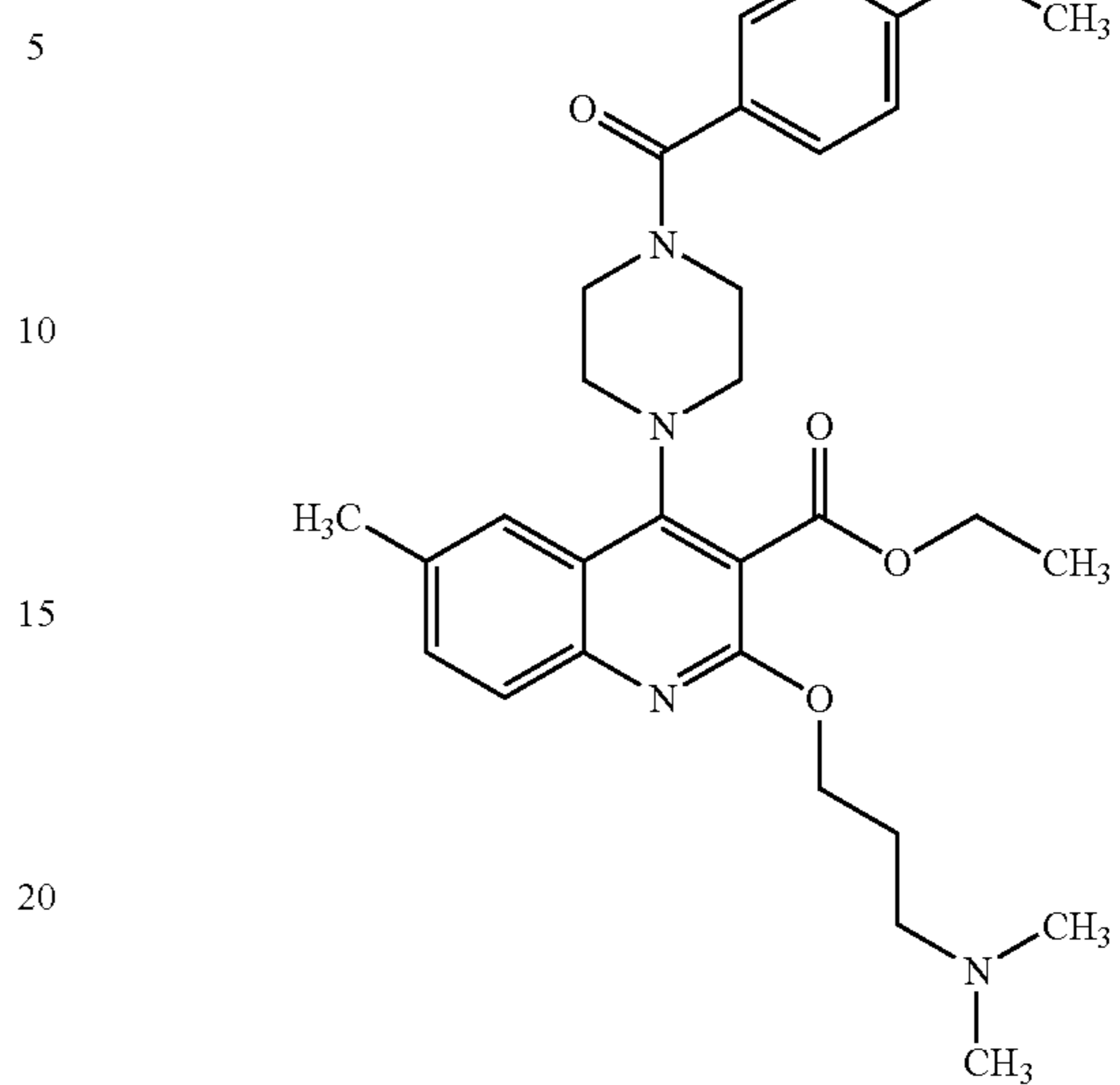
Compound 340
