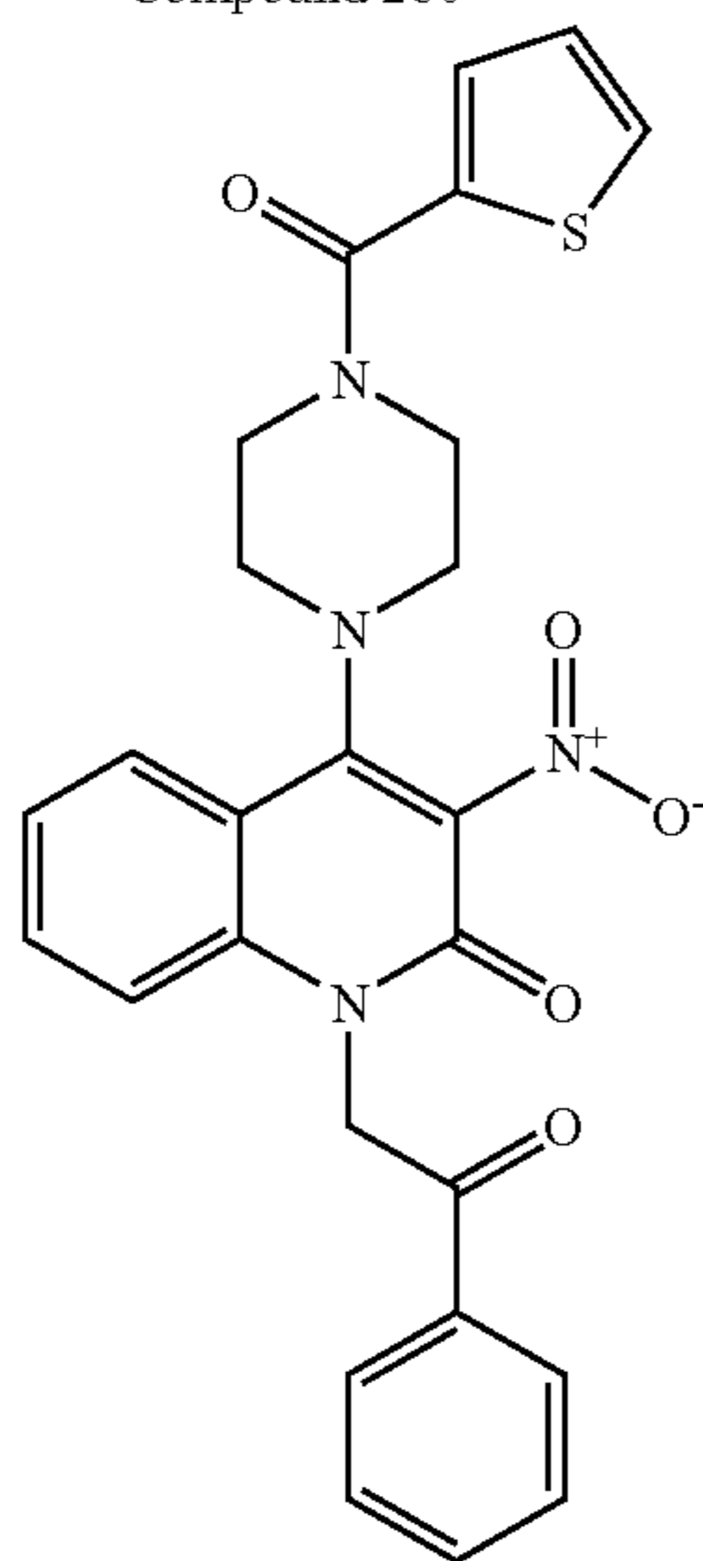
Compound 281
