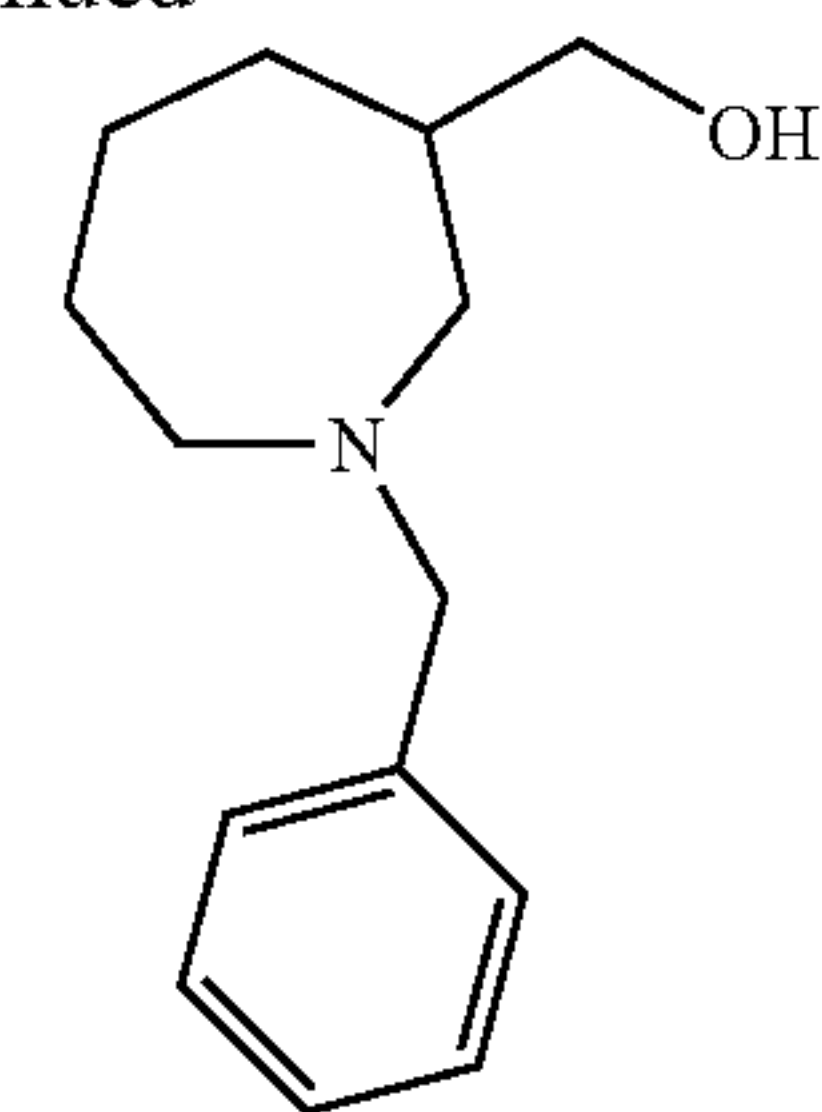
(1-Benzyl-azepan-3-yl)-methanol
