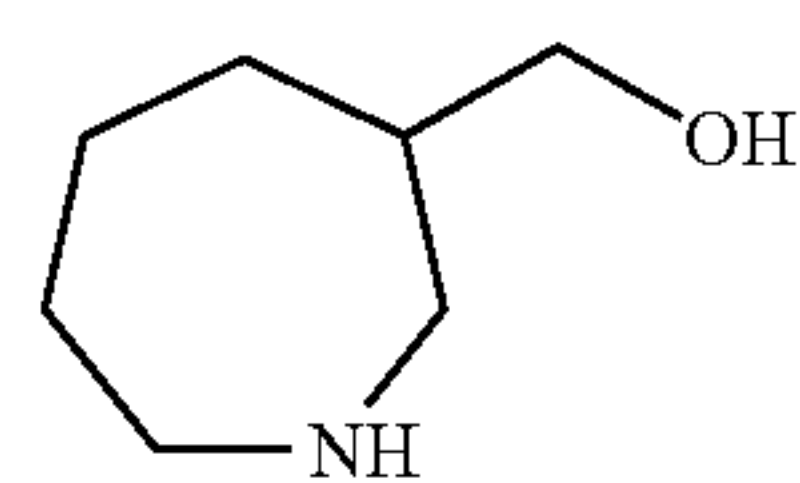
Azepan-3-yl-methanol 145
