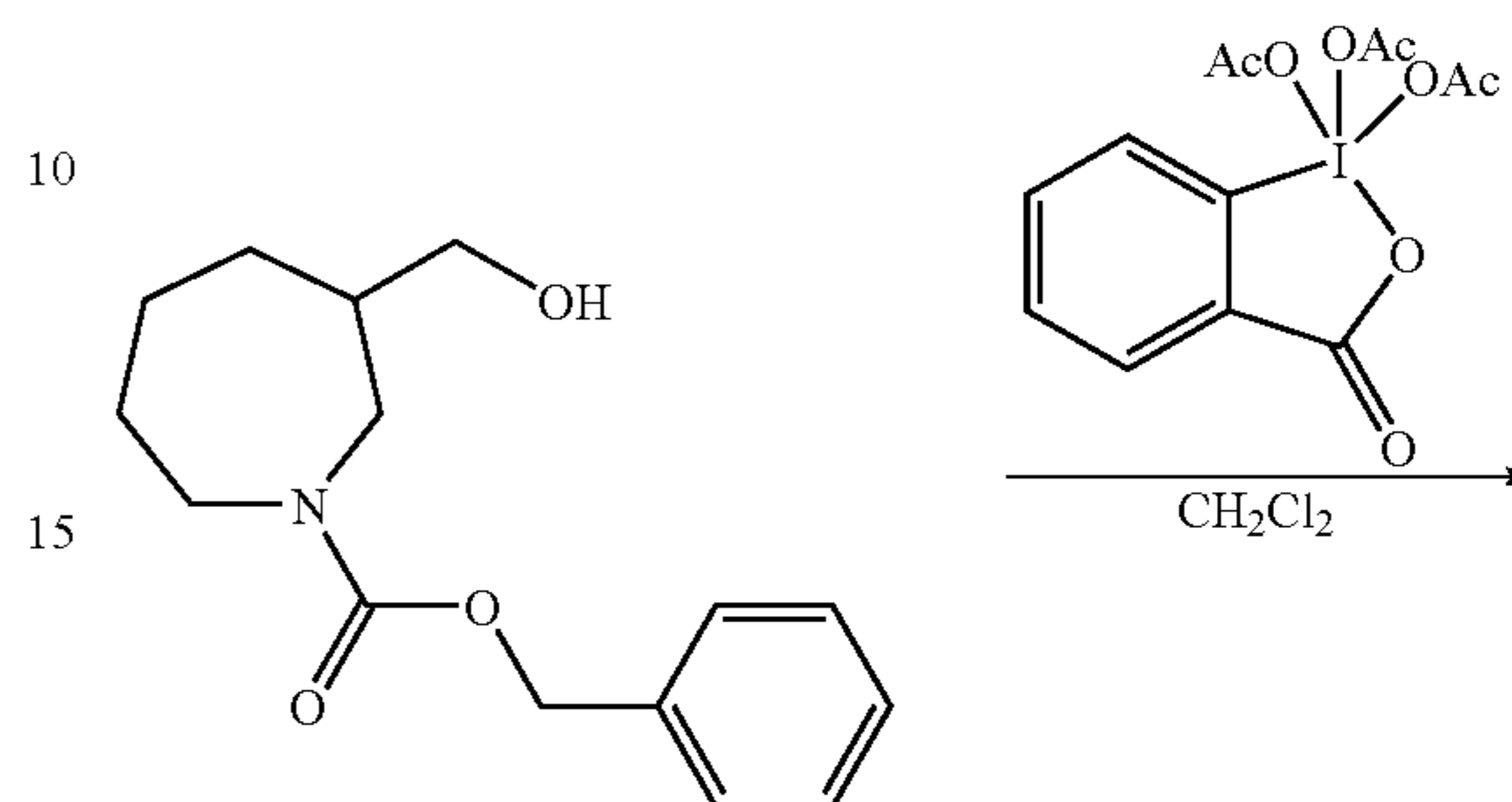
3-Hydroxymethyl-azepane-1-carboxylic acid benzyl ester 146
