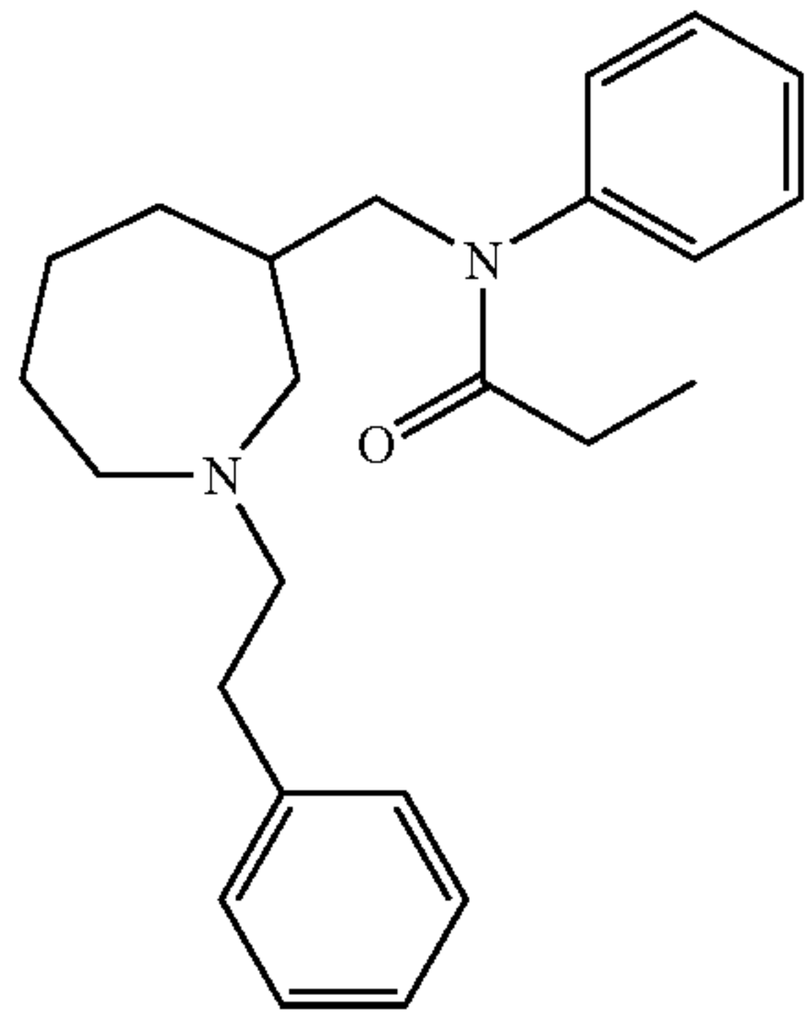
N-(1-Phenethyl-azepan-3-ylmethyl)- N-phenyl-propionamide 150
