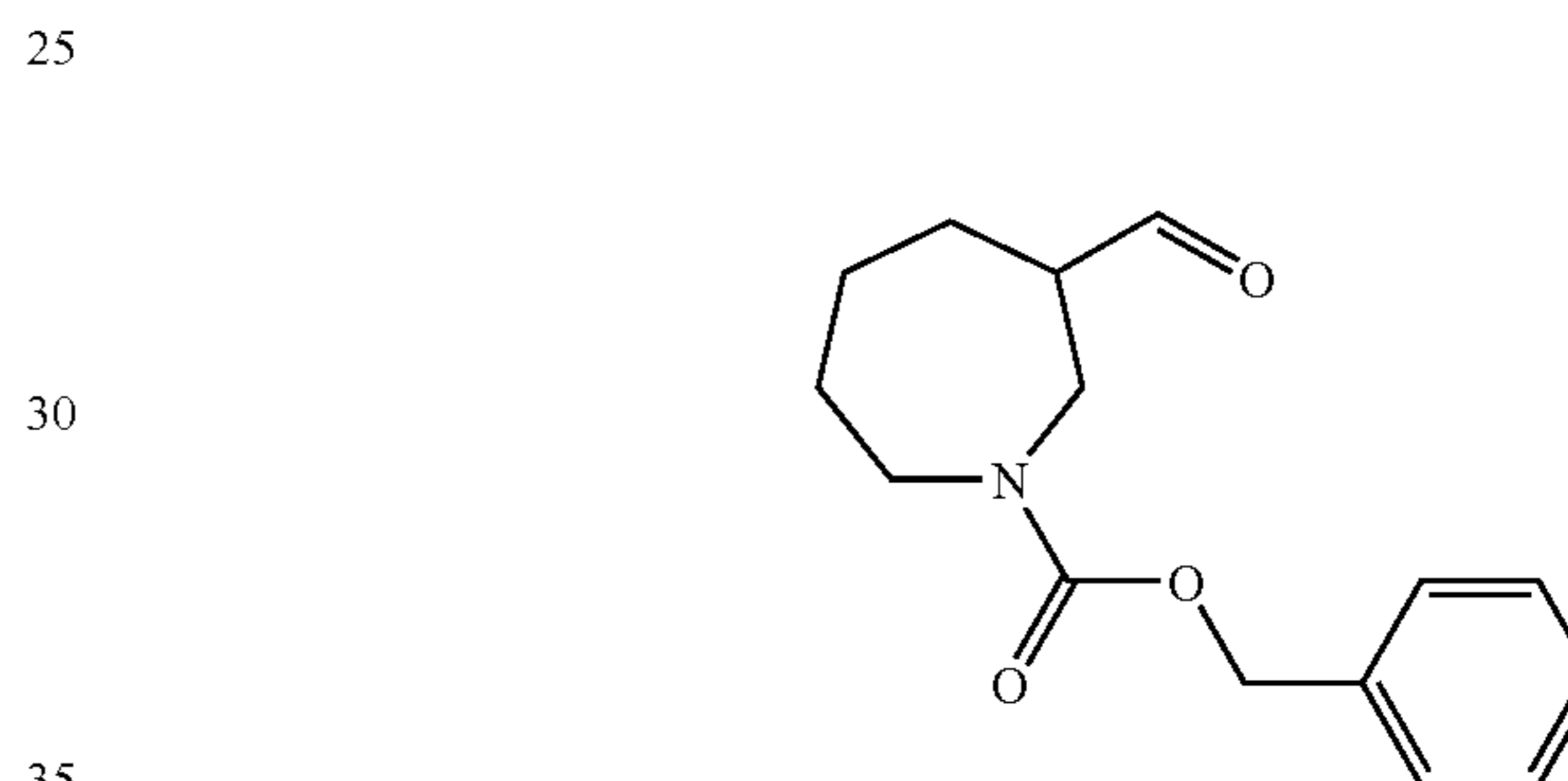
3-Formyl-azepane-1-carboxylic acid benzyl ester 147
