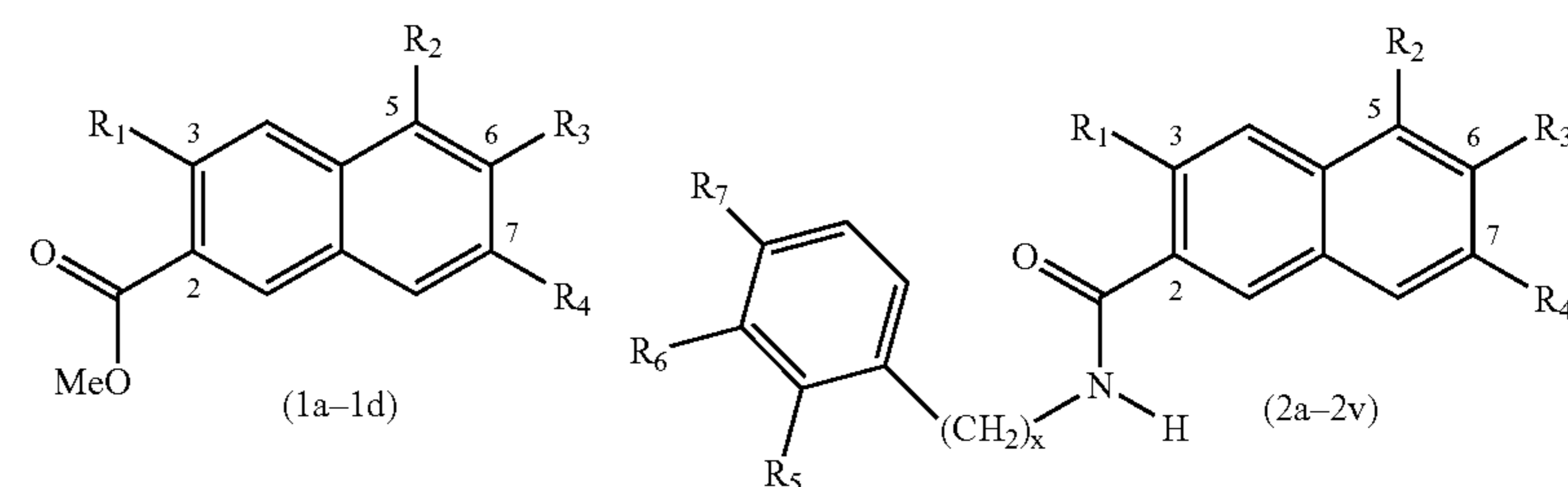
pp60 c-src INHIBITORY ACTIVITY OF HYDROXYNAPHTHALENE DERIVATIVES AND SELECT PUBLISHED INHIBITORS. a,b,c
