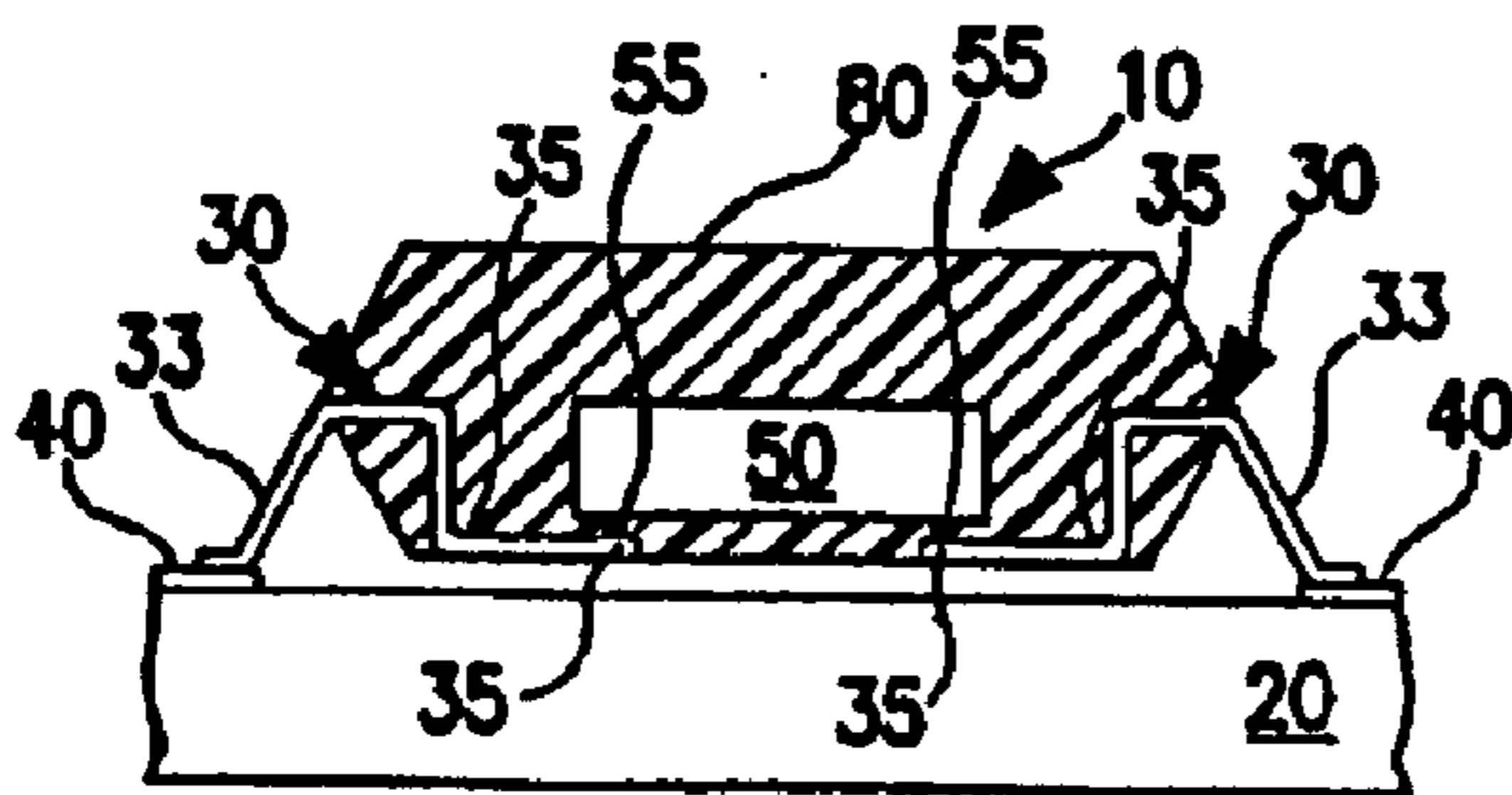
FIG. 2c PRIOR ART
