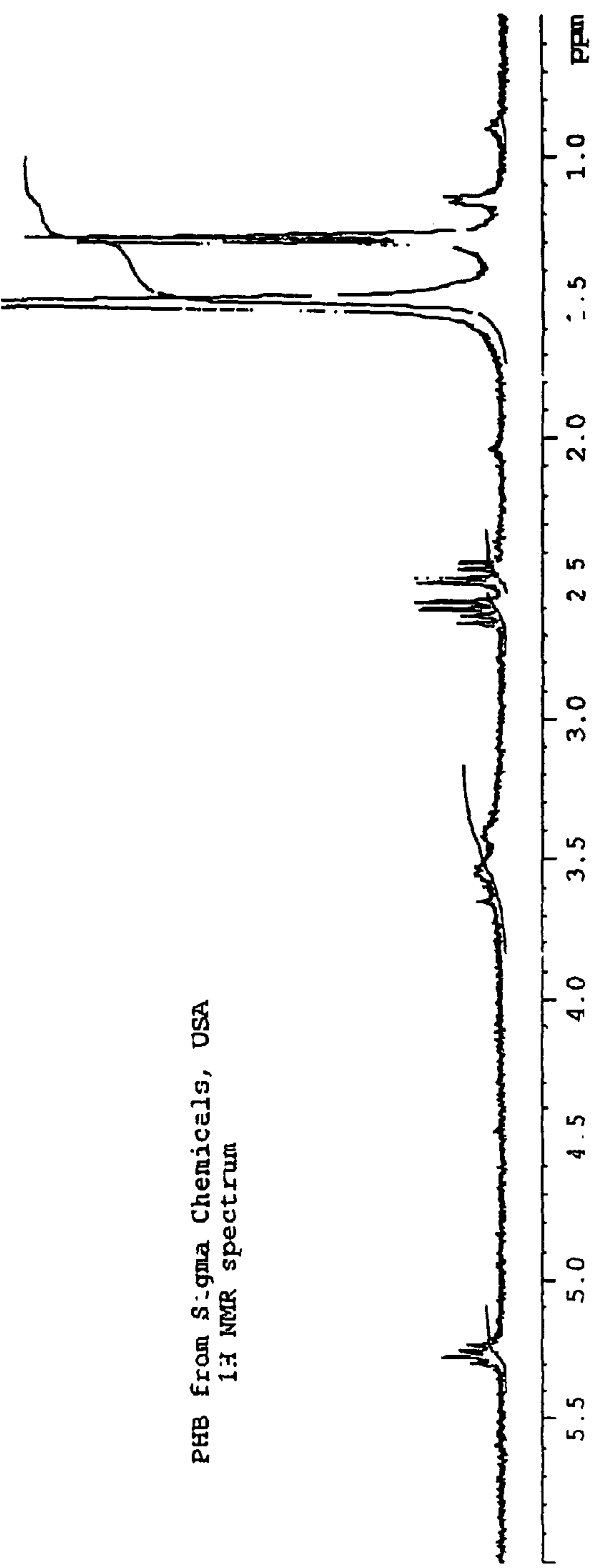
Figure 2 : Comparison of the 1H NMR spectra of PHE produced by Bacillus mycooides RLJ B-017 with sucrose/molasses as carbon source with that of M/3 Sigma Chemicals, USA
