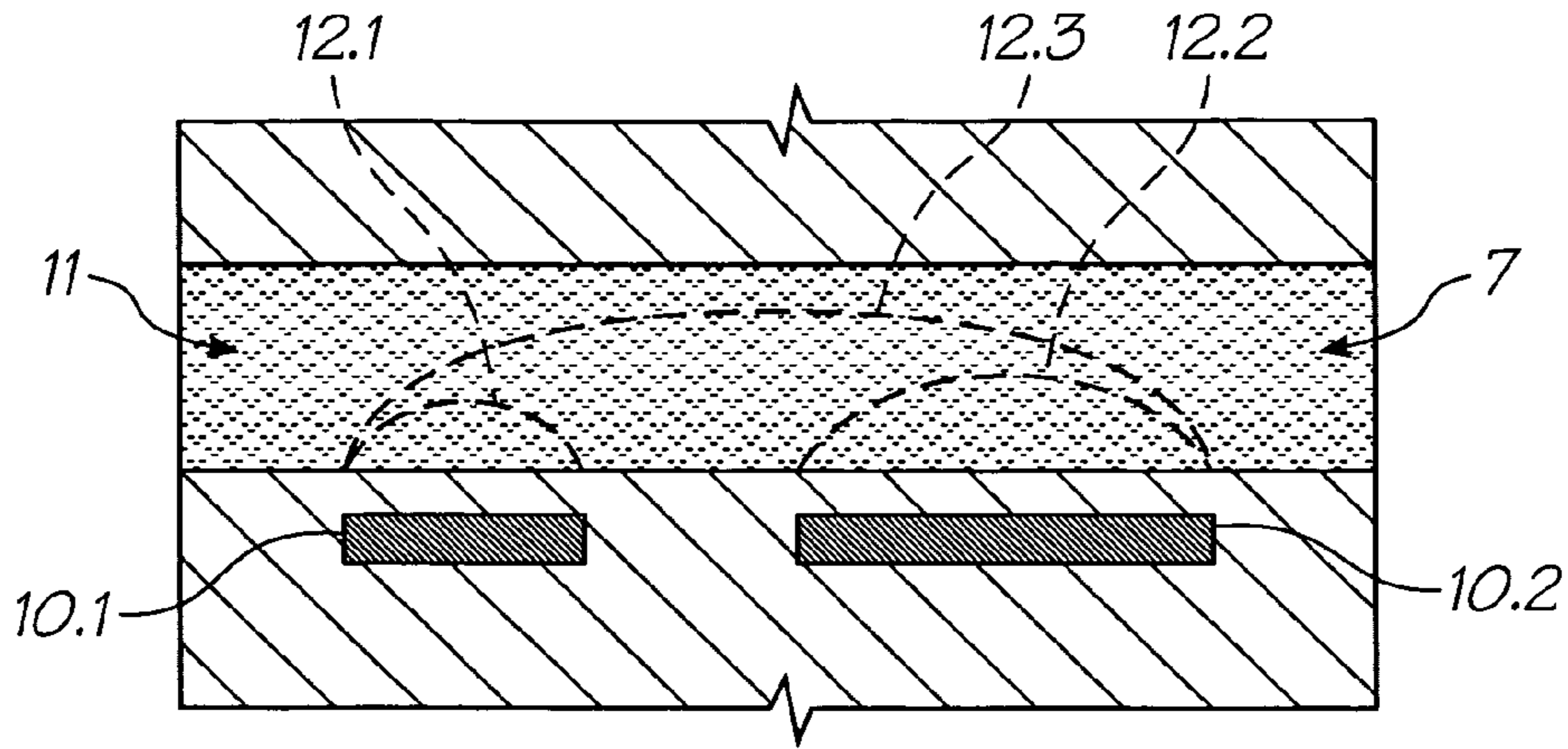
FIG. 52 (PRIOR ART)
