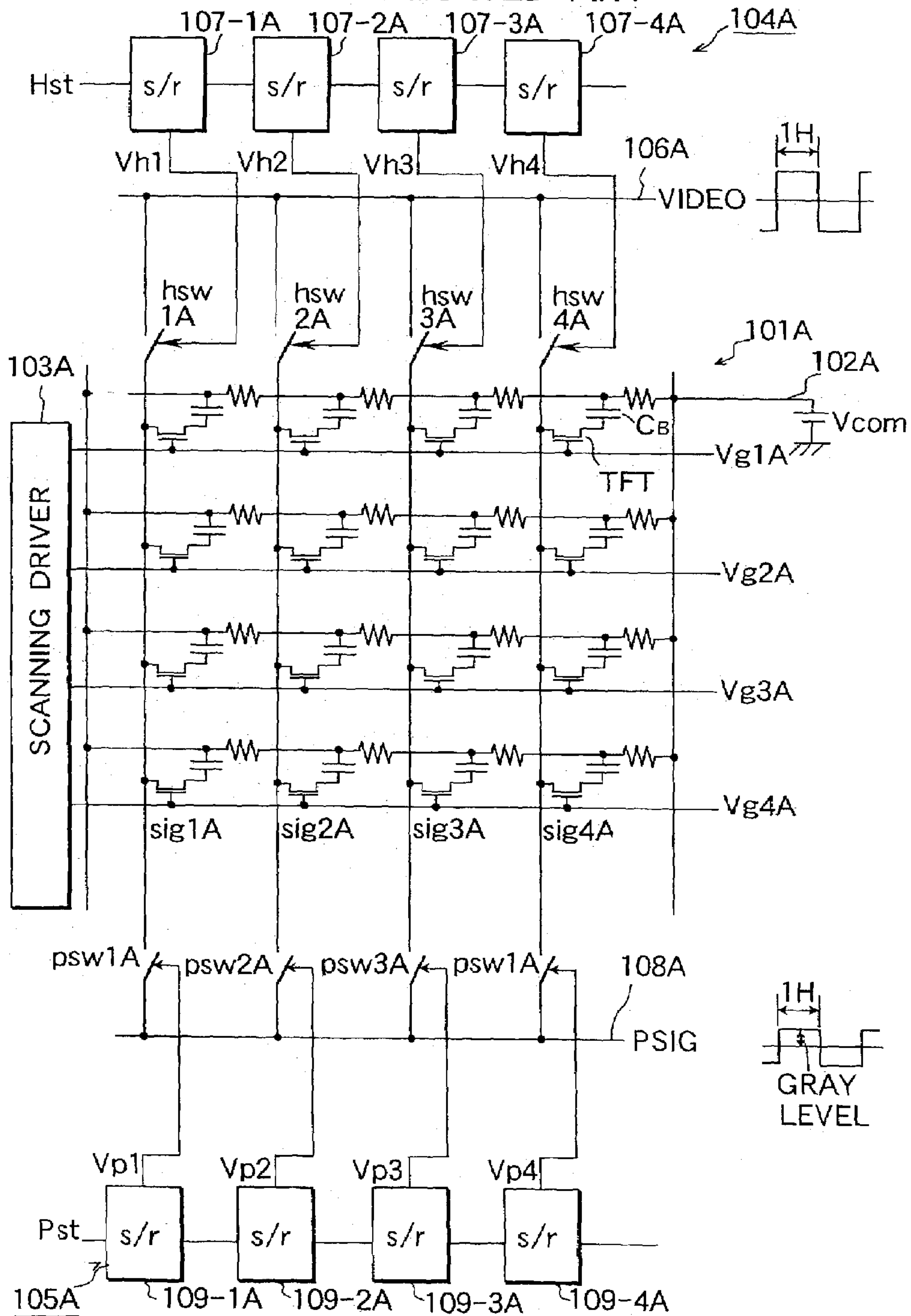
FIG.18 RELATED ART
