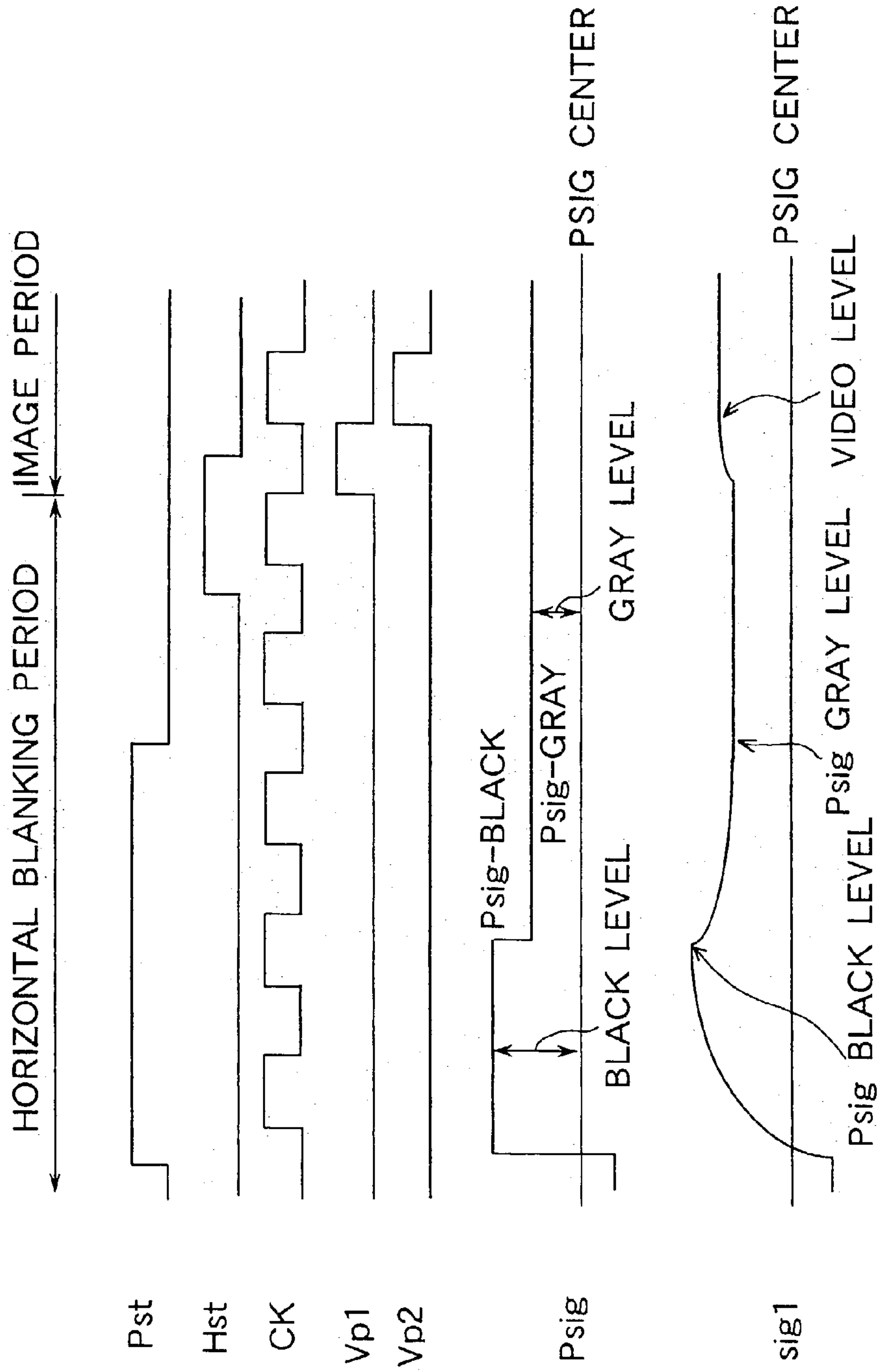
FIG. 21 RELATED ART
