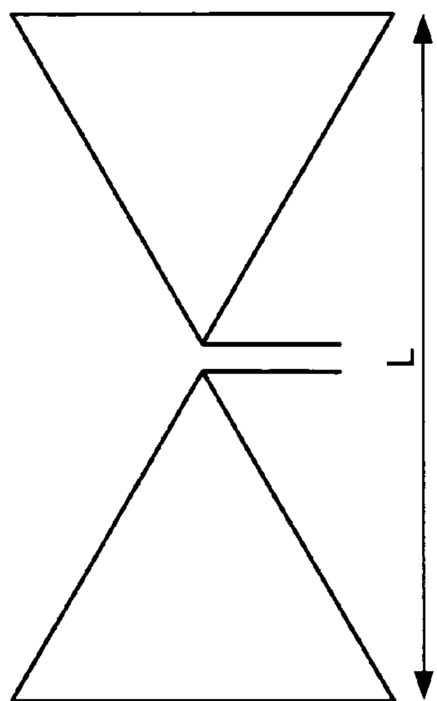
Fig. 1C (Prior Art)
