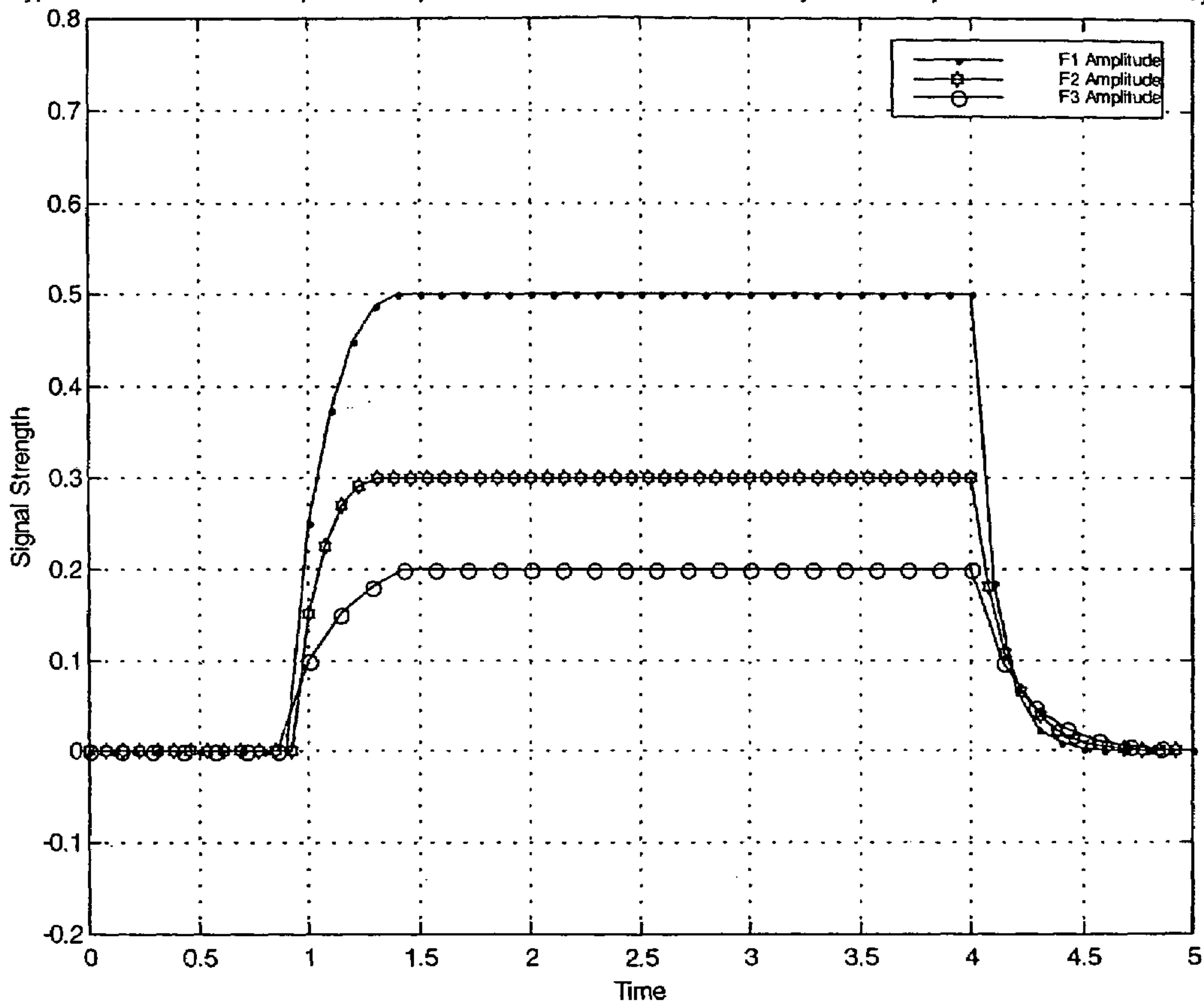
Typical Full Pulse Return Spectral Amplitudes for F1, F2, and F3 for the Synchronously Demodulated Pulsed System
