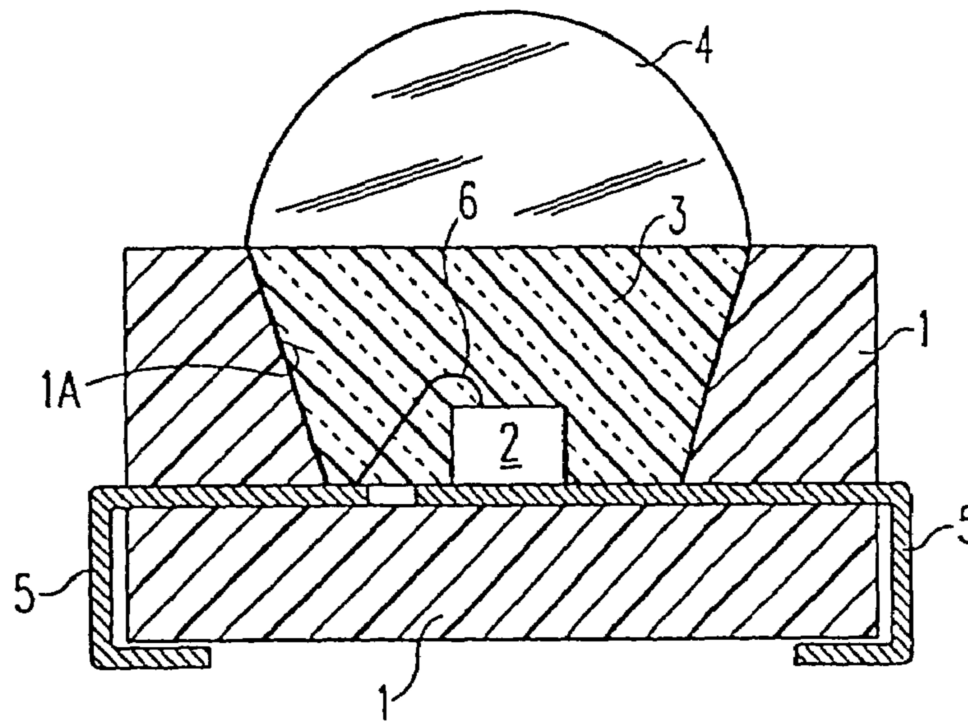
Fig. 1 PRIOR ART
