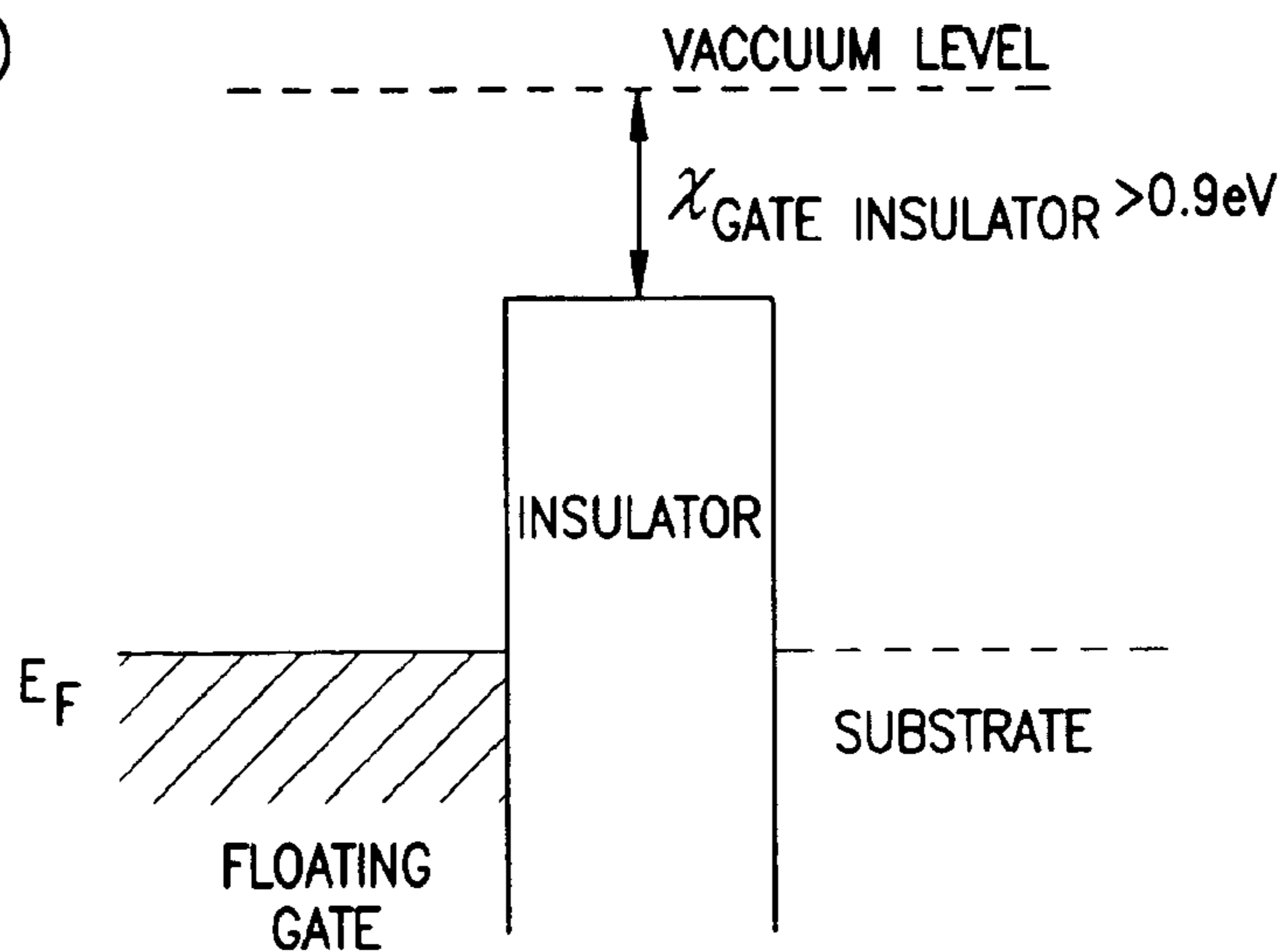
FIG. 1C (PRIOR ART)
