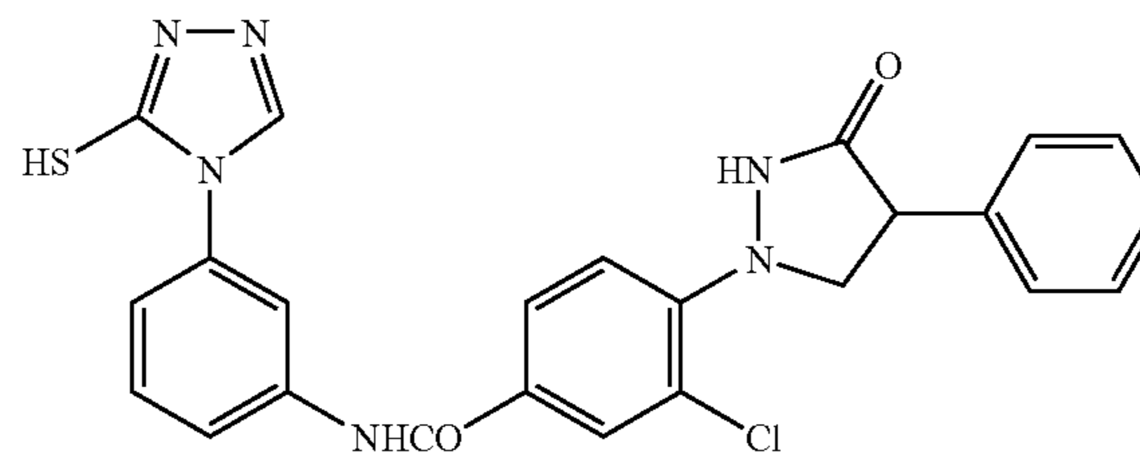
Comparative Compound-2
