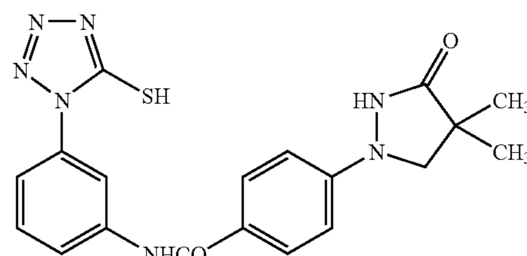
Comparative Compound-2
