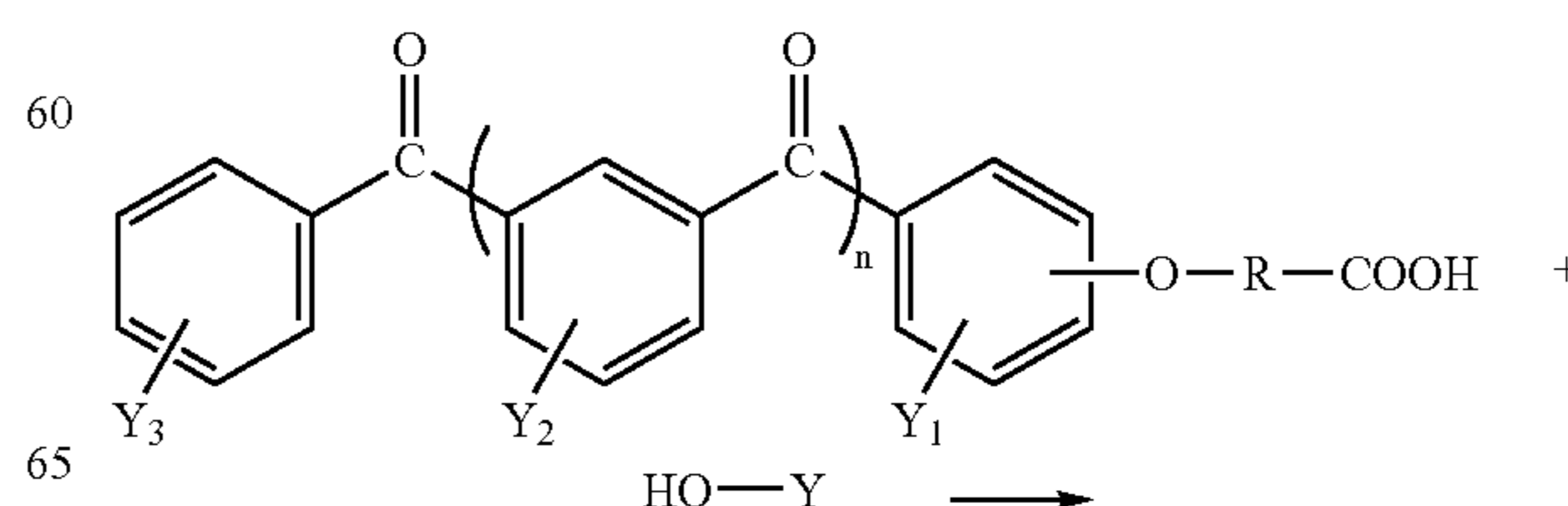
Reaction scheme (1)
