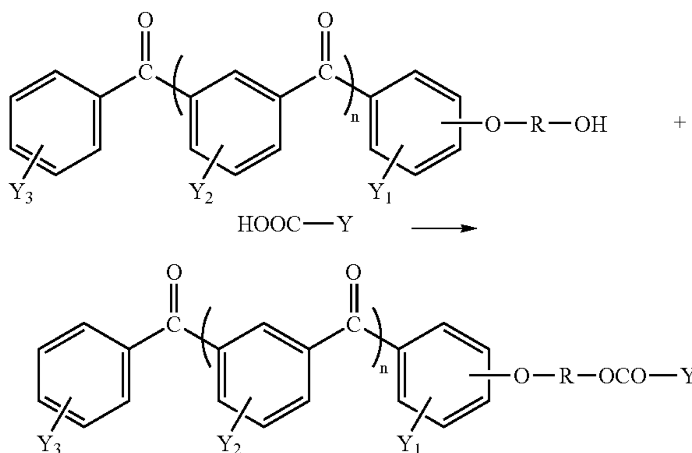
Reaction scheme (4)
