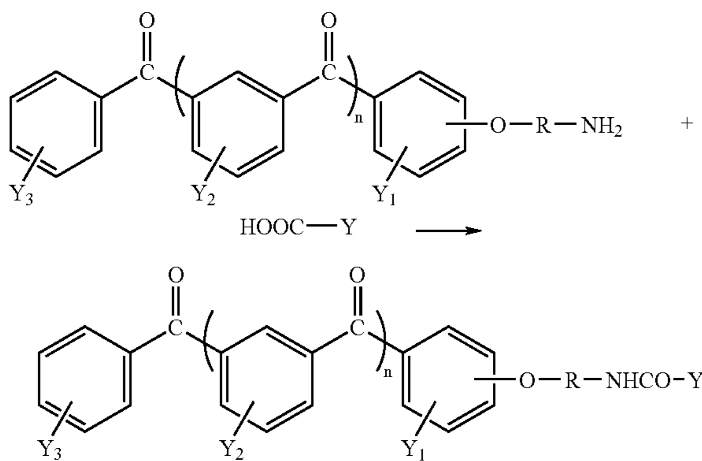
Reaction scheme (3)
