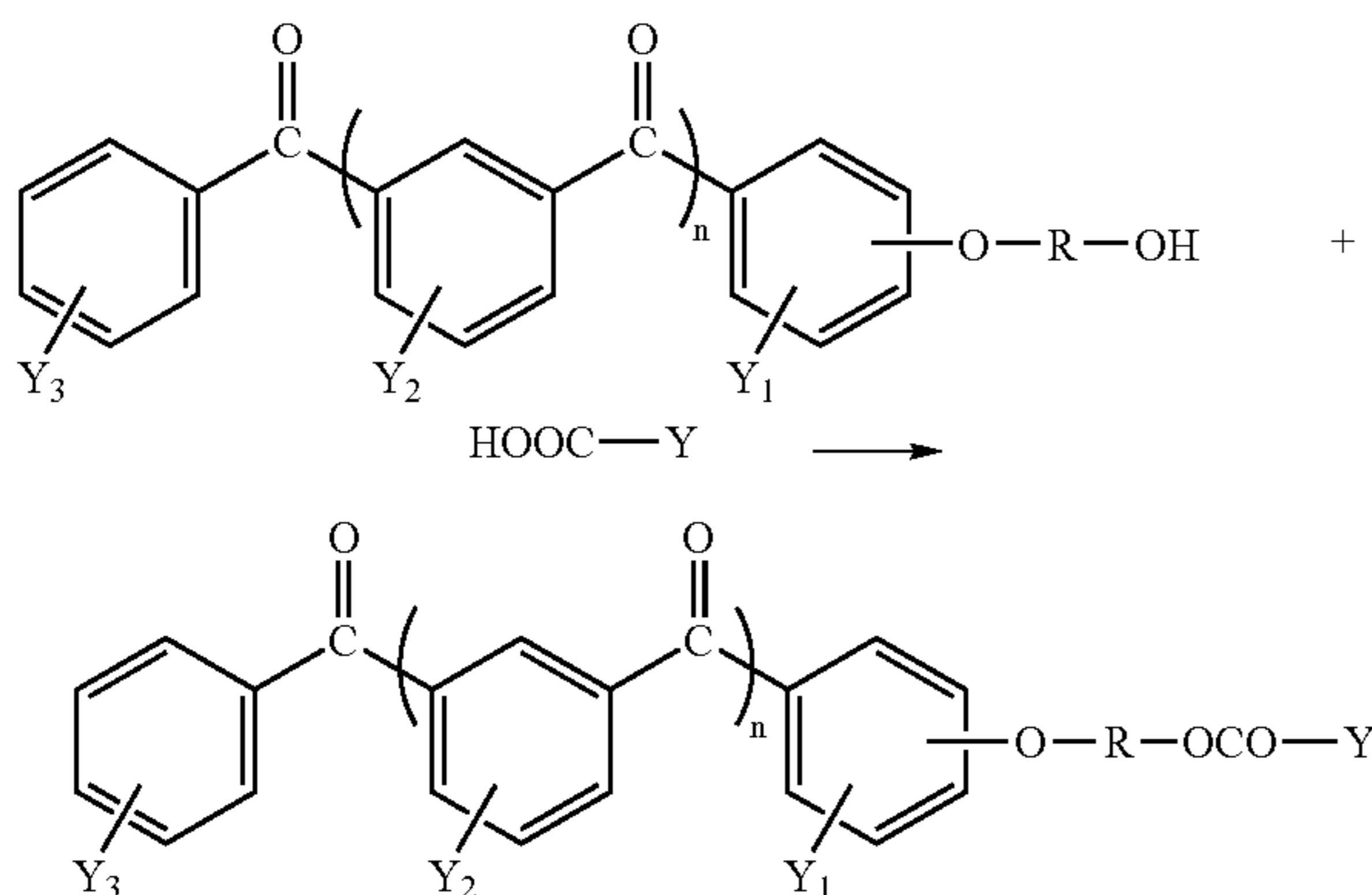
Reaction scheme (4)
