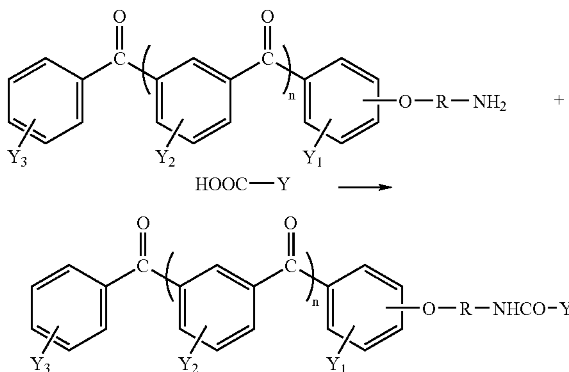
Reaction scheme (3)
