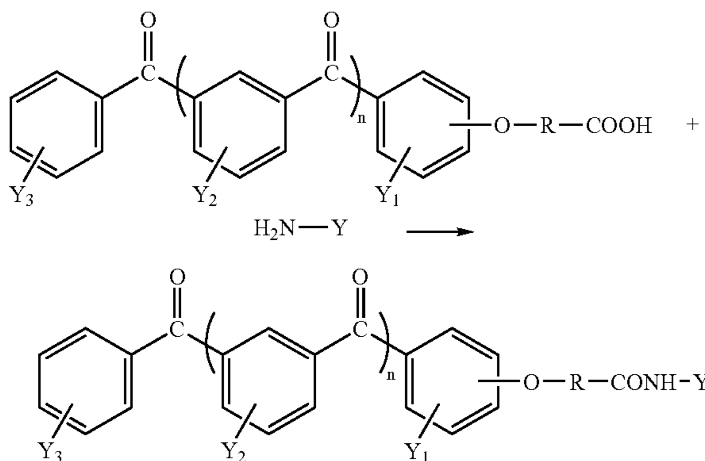
Reaction scheme (2)
