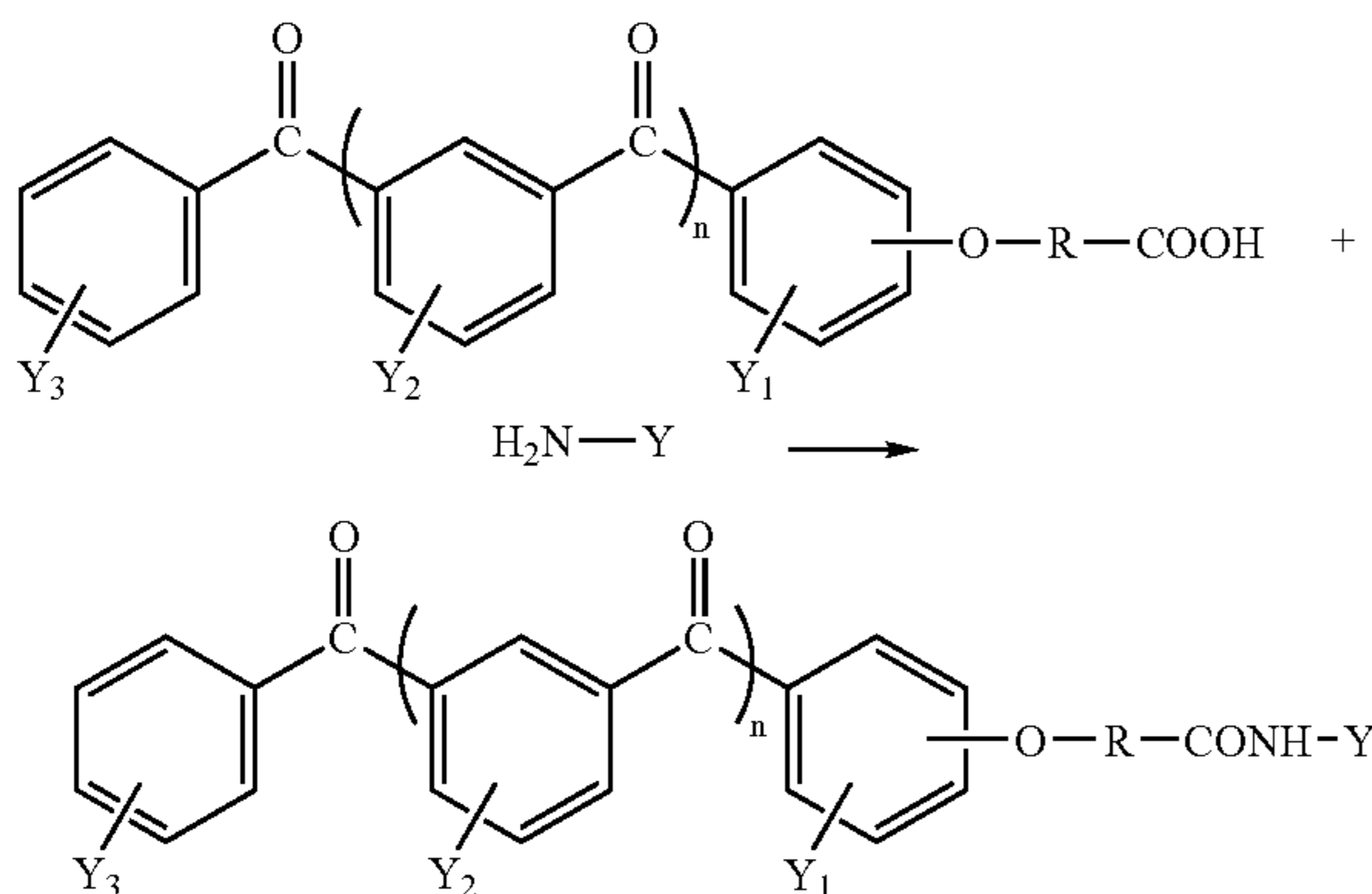
Reaction scheme (2)
