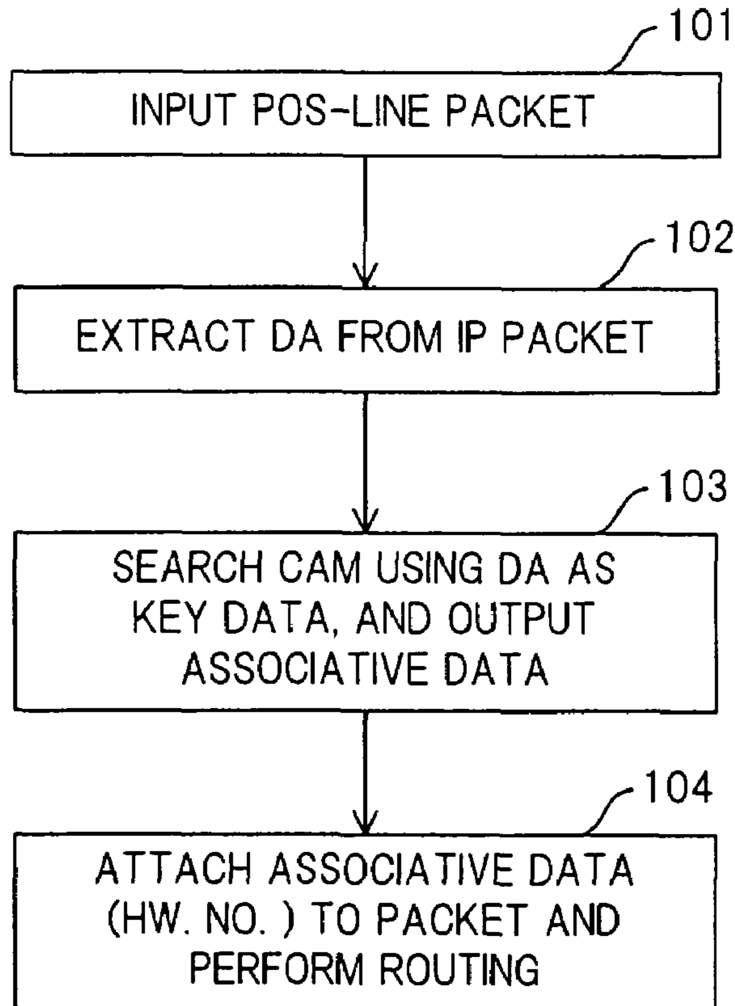
FIG. 17 PRIOR ART
