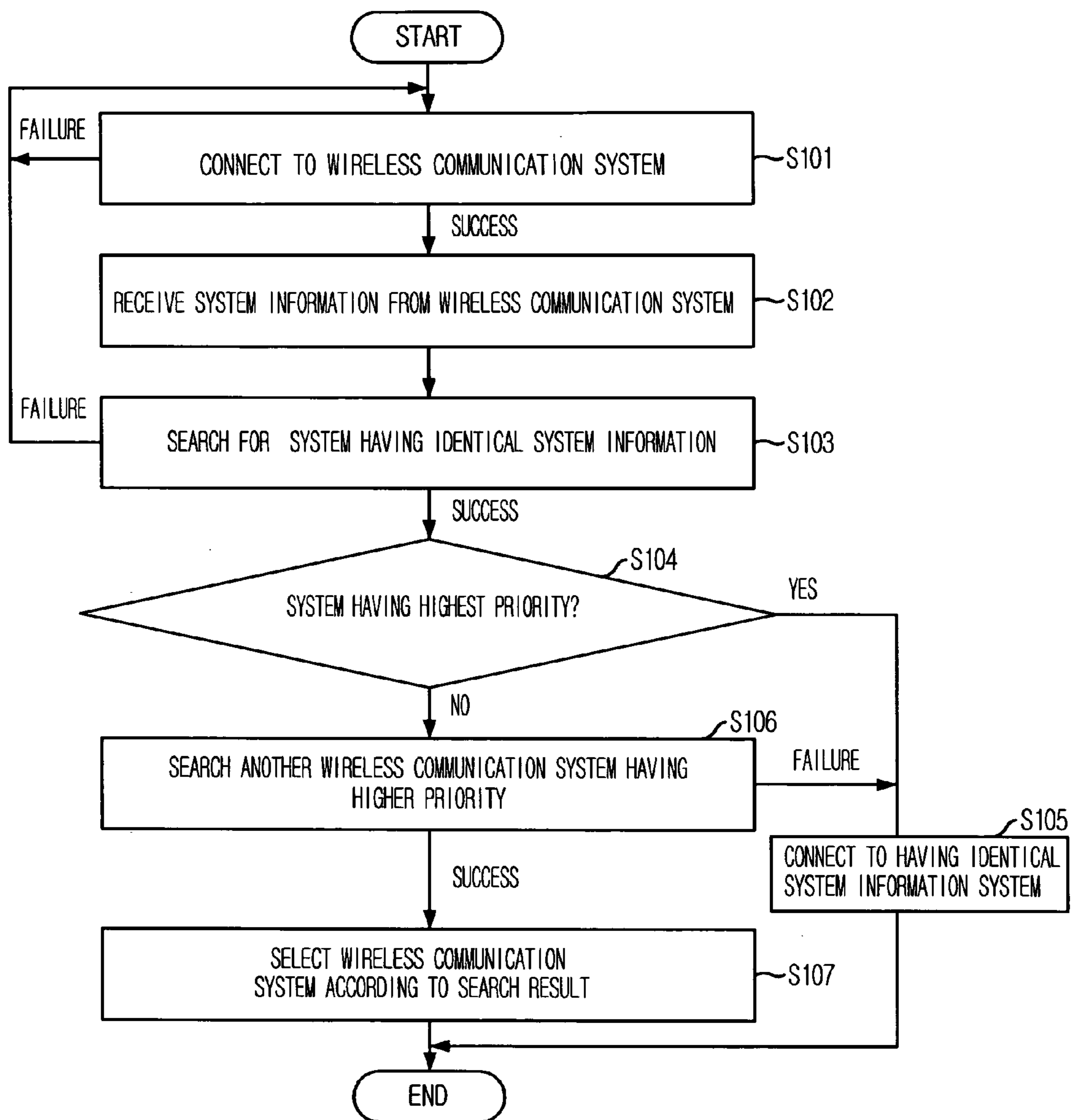
FIG. 1 (PRIOR ART)
