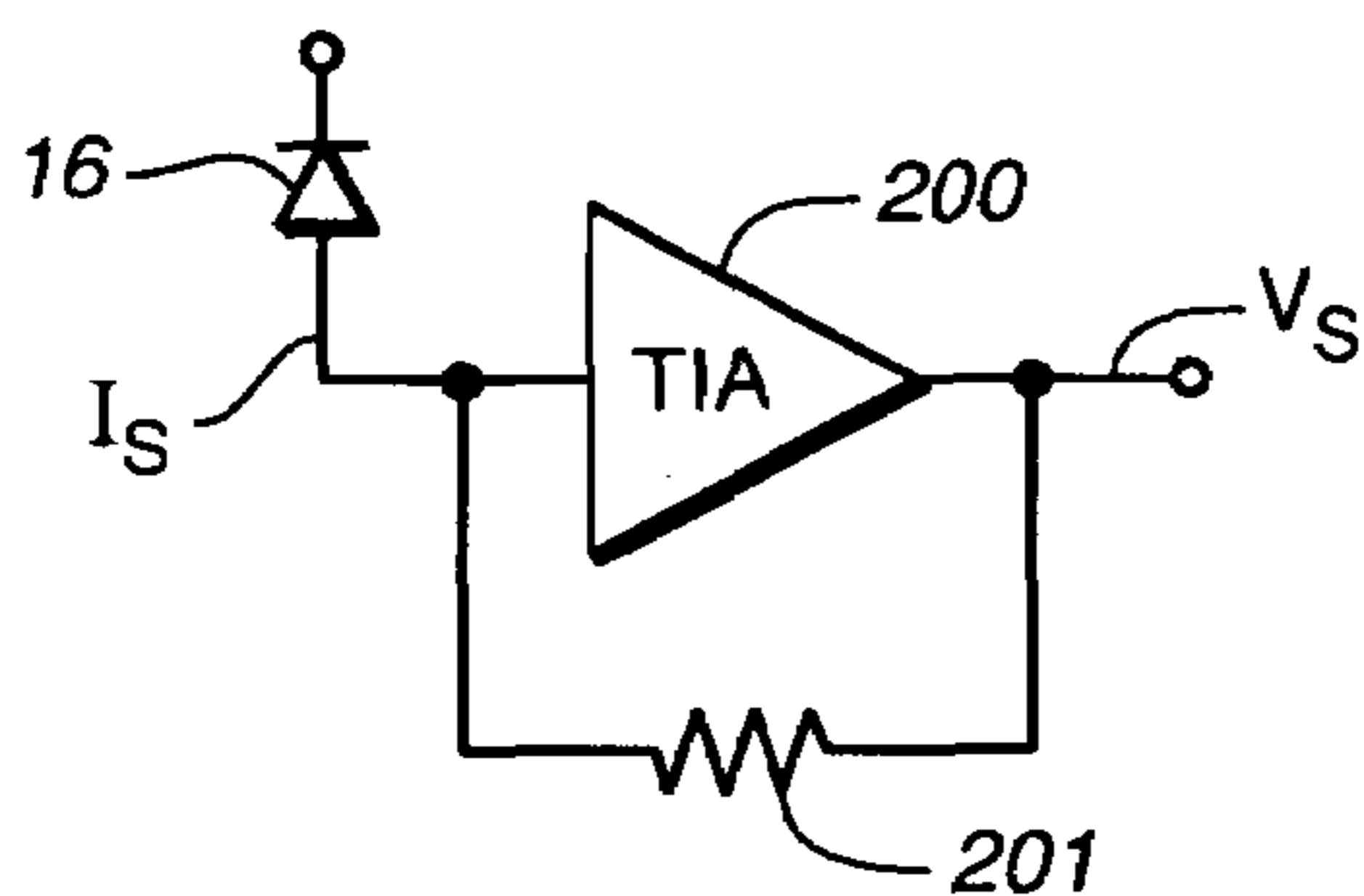
FIG. 48 (PRIOR ART)
