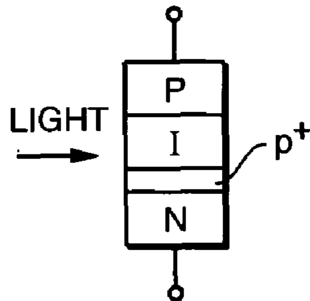
FIG. 26 (PRIOR ART)
