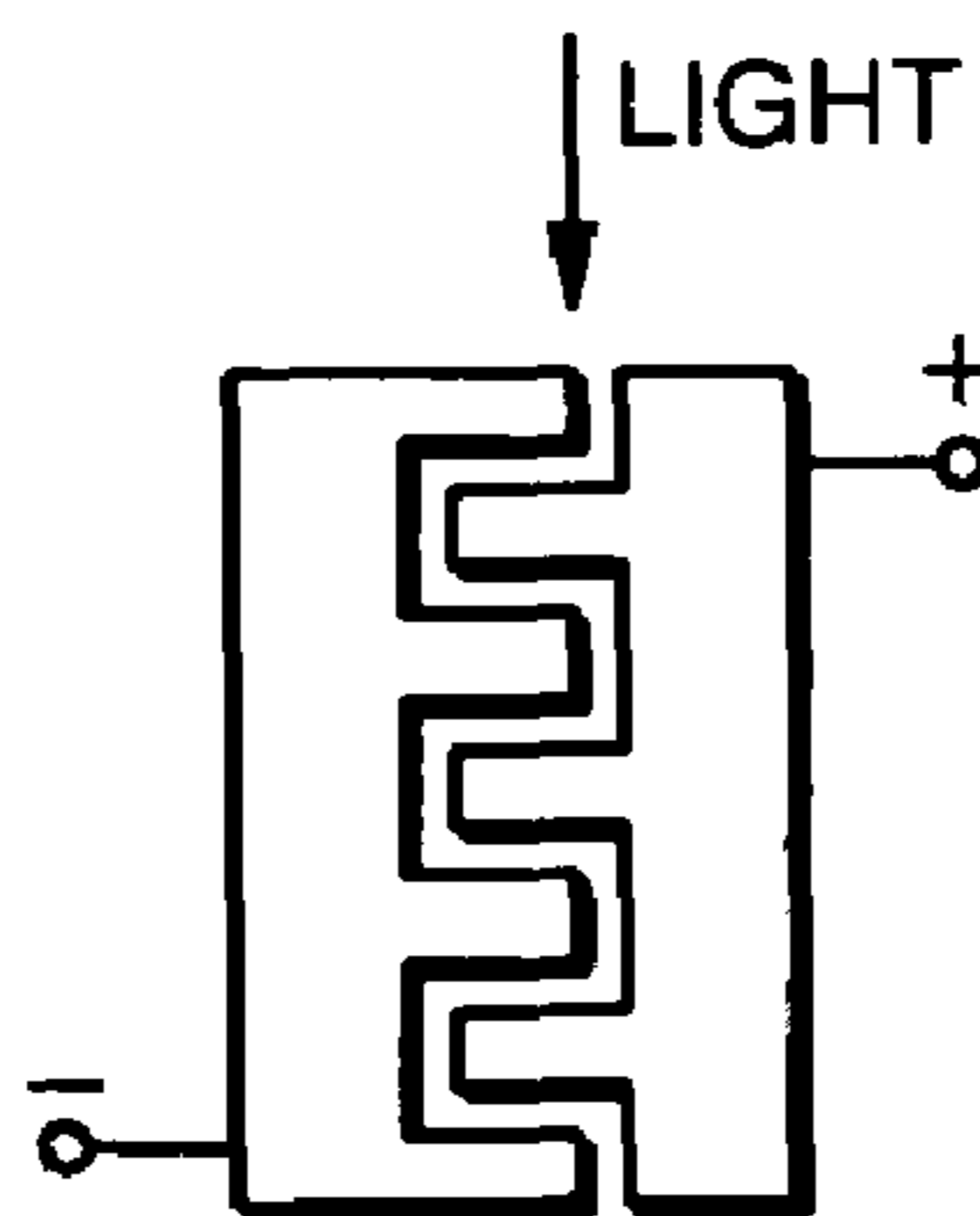
FIG. 27 (PRIOR ART)
