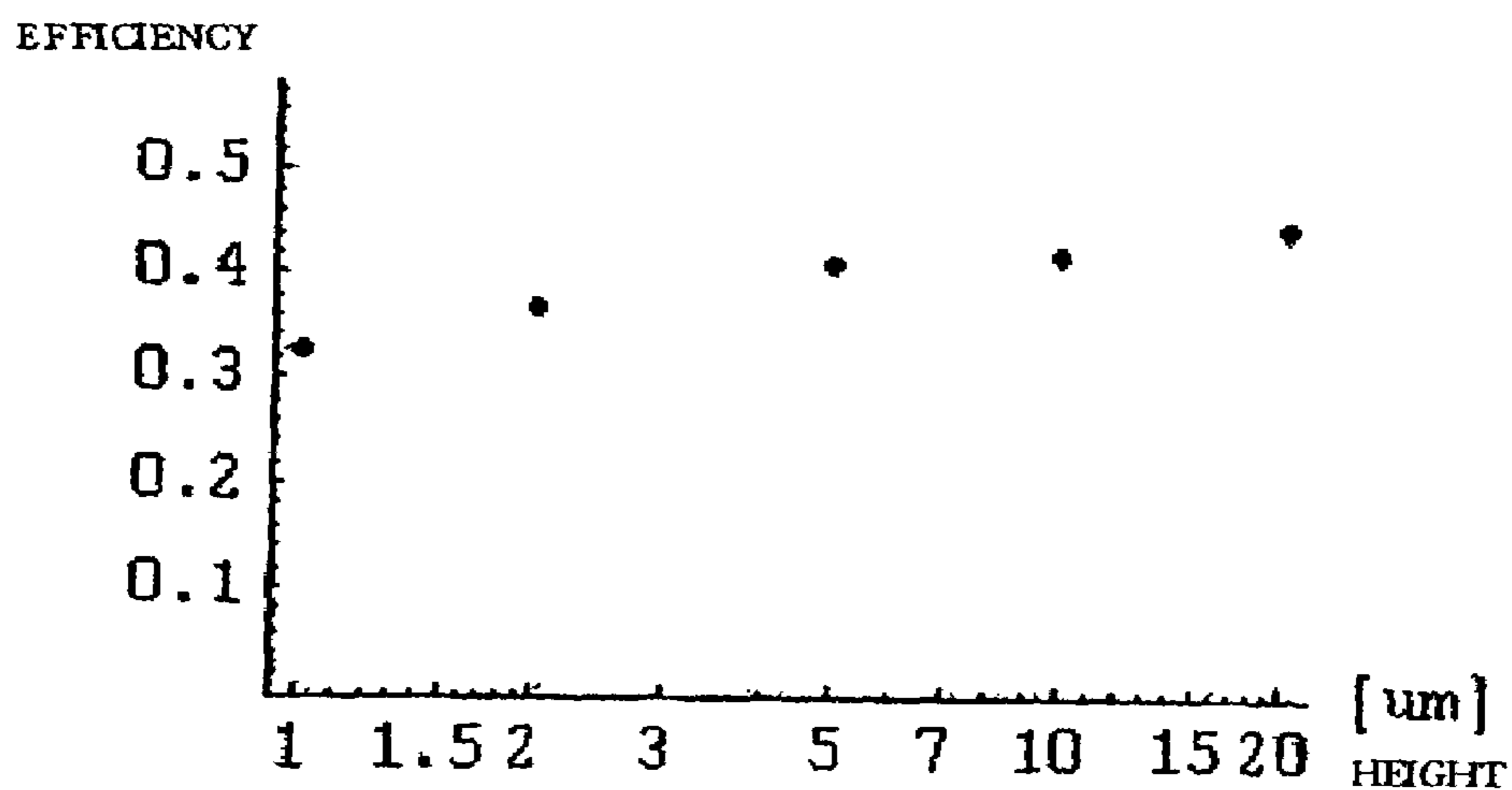
DEPENDENCE OF LIGHT EMERGENCE EFFICIENCY ON HEIGHT
