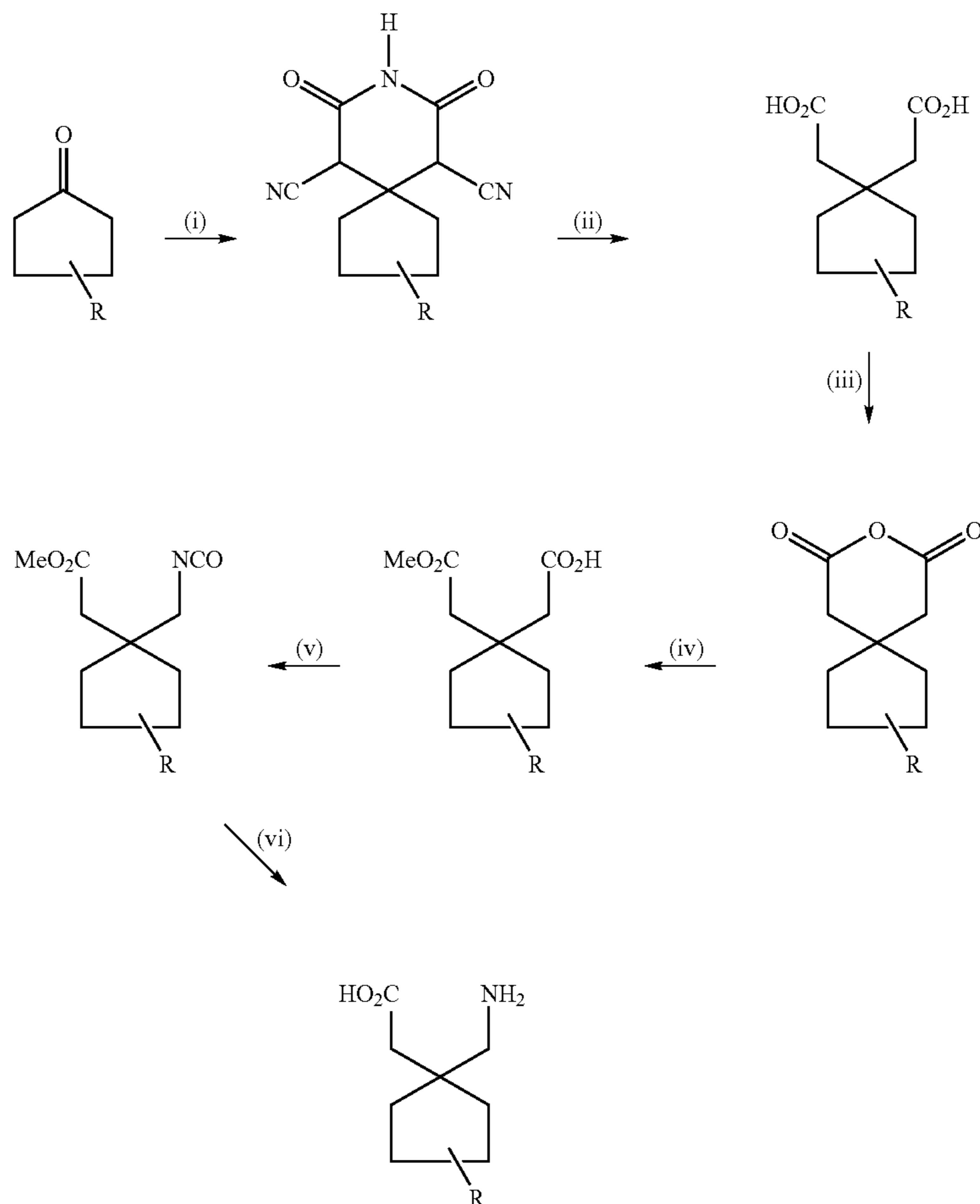
General Scheme 3
