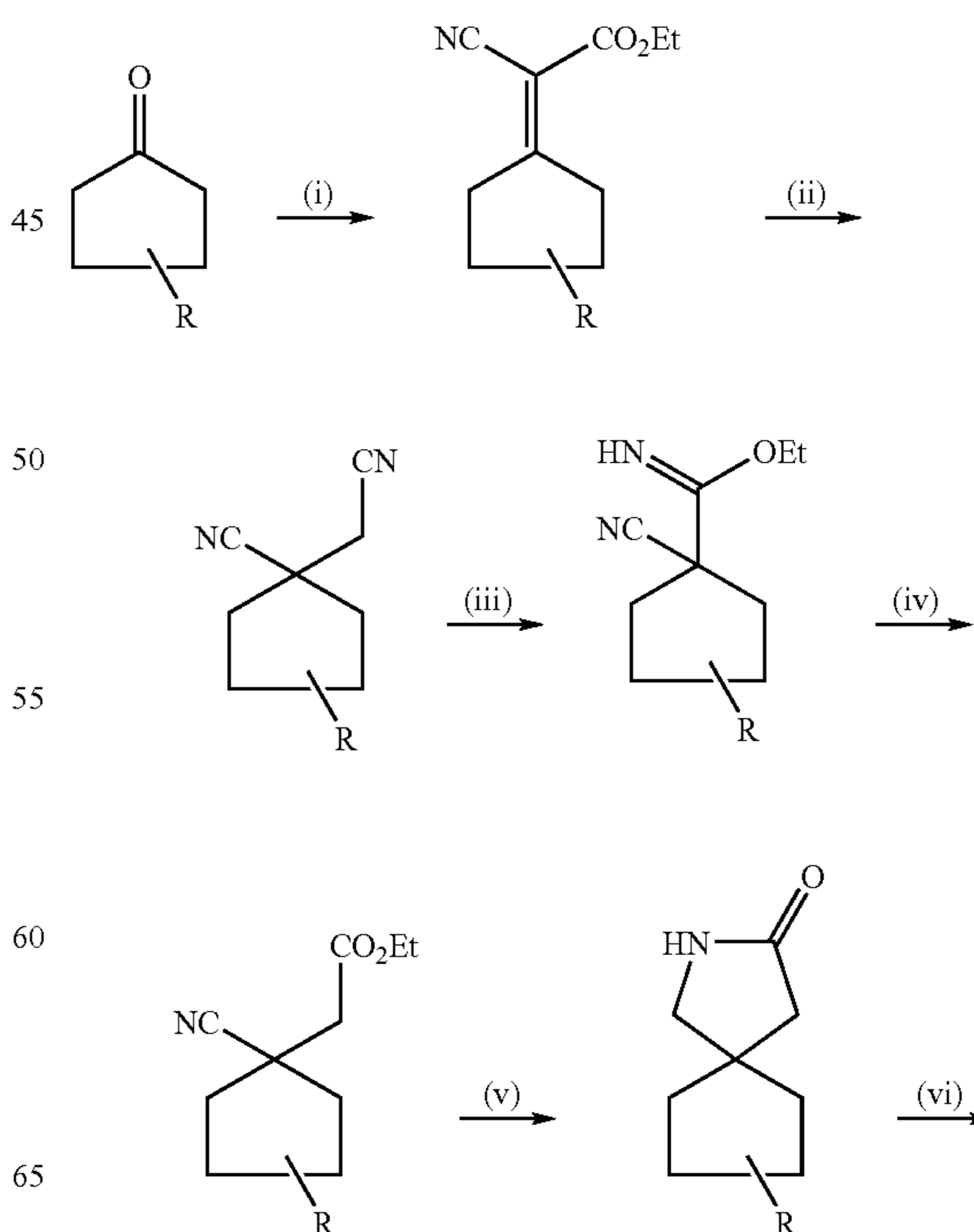
General Scheme 1
