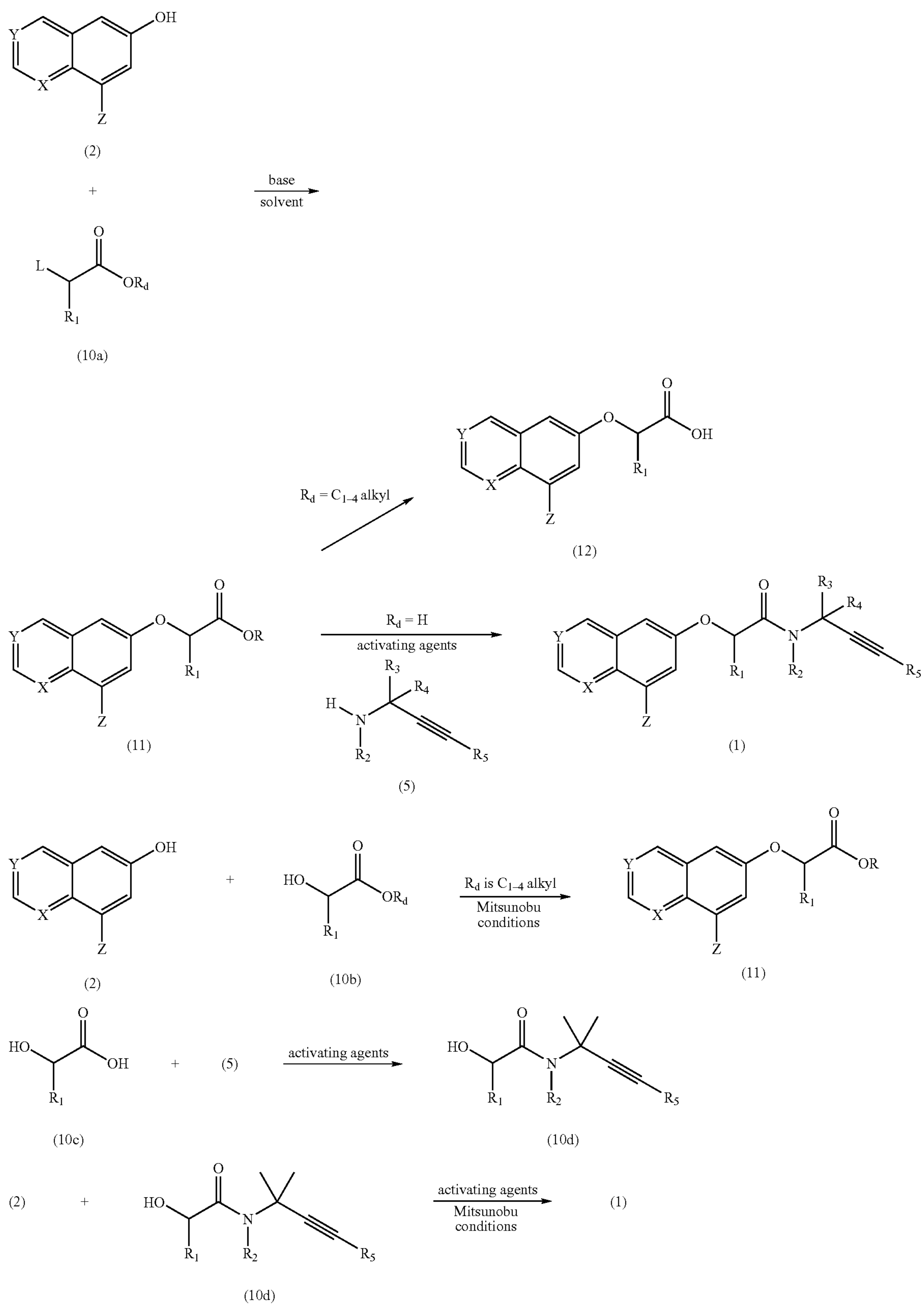
Scheme 4
