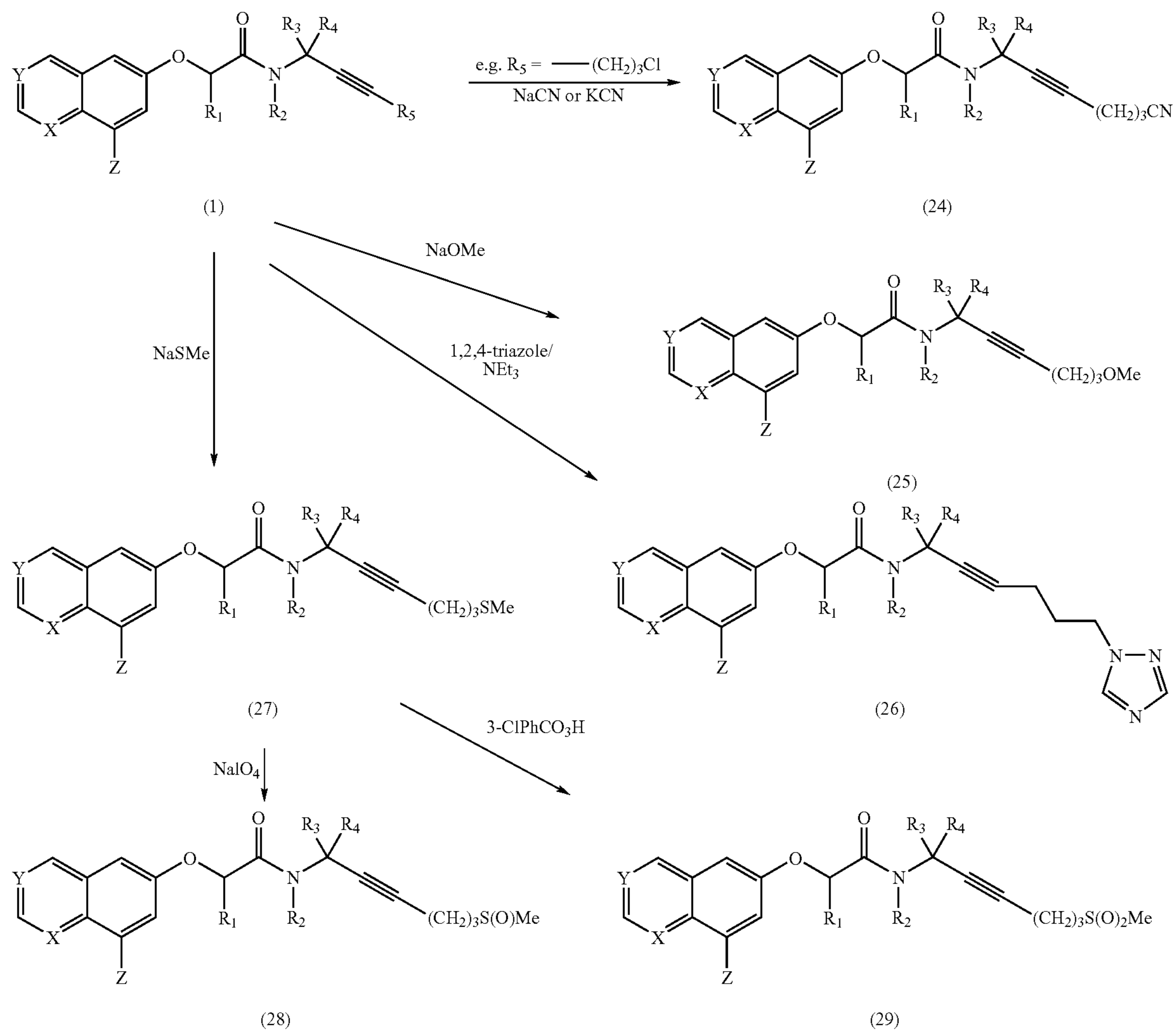
Scheme 10
