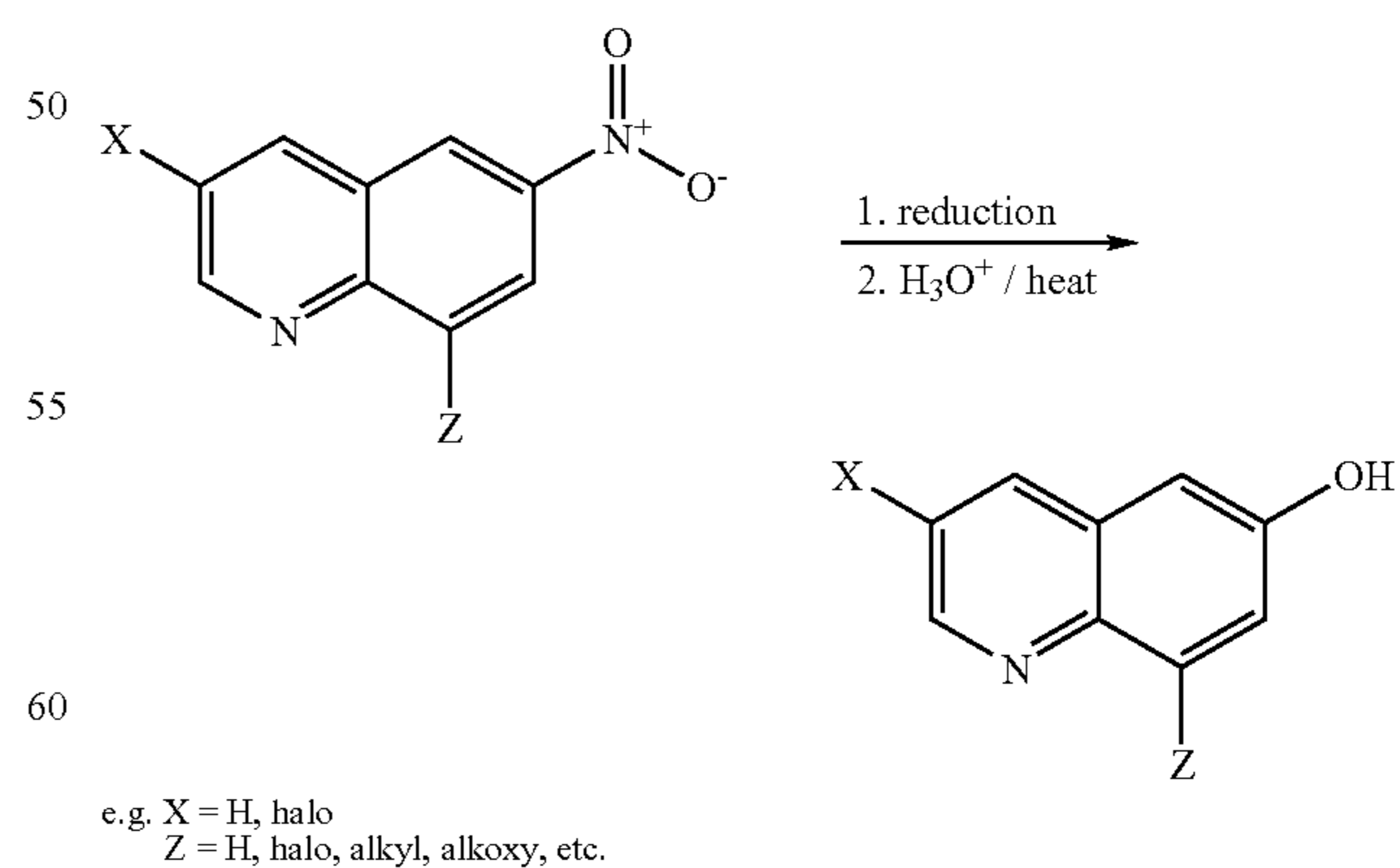
Scheme 11
