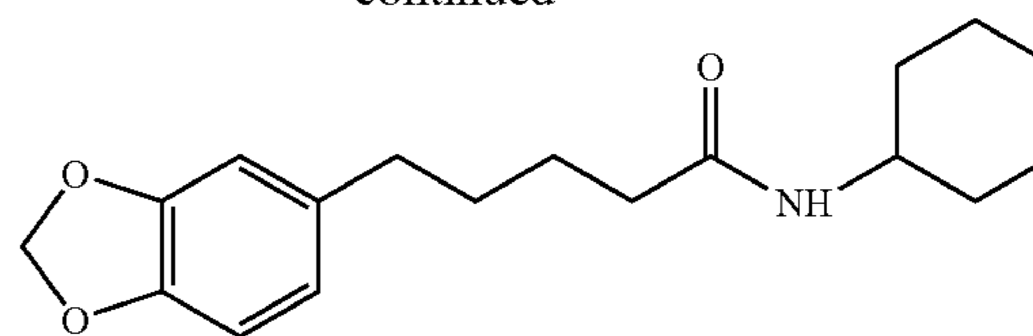
5-(3,4-methylenedioxy phenyl)2,4-pentanoic acid cyclohexyl amide
