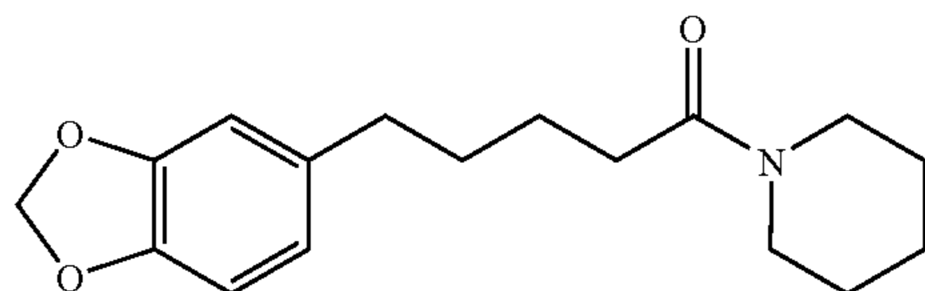
1-(5-benzo-1,3-dioxol-5-yl-pentanoyl)-piperidine
