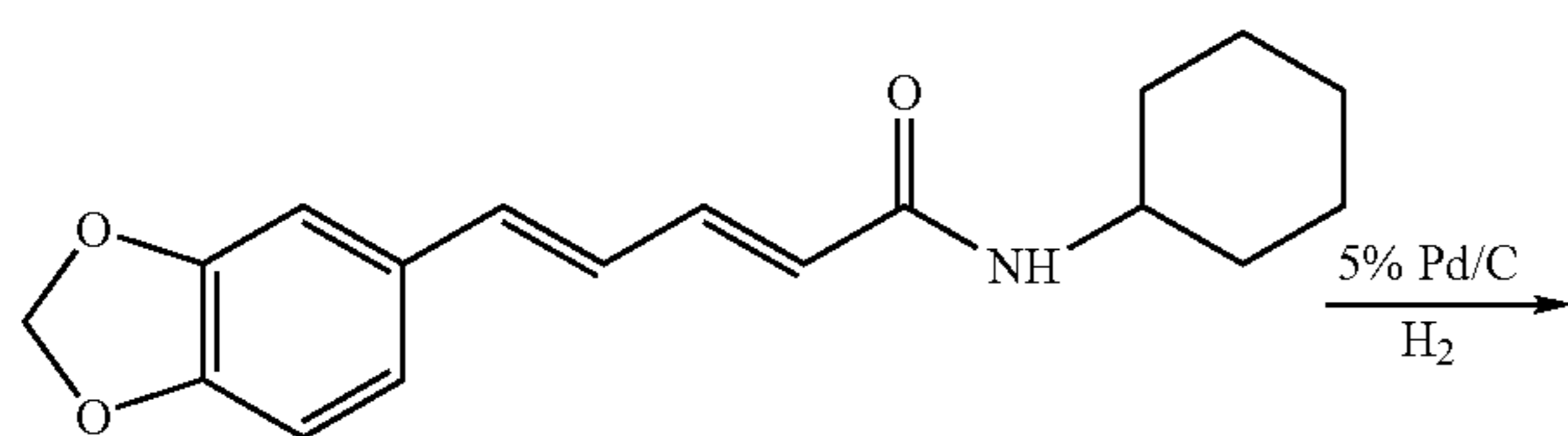
5-(3,4-methylenedioxy phenyl)2E,4E-pentadienoic acid cyclohexyl amide
