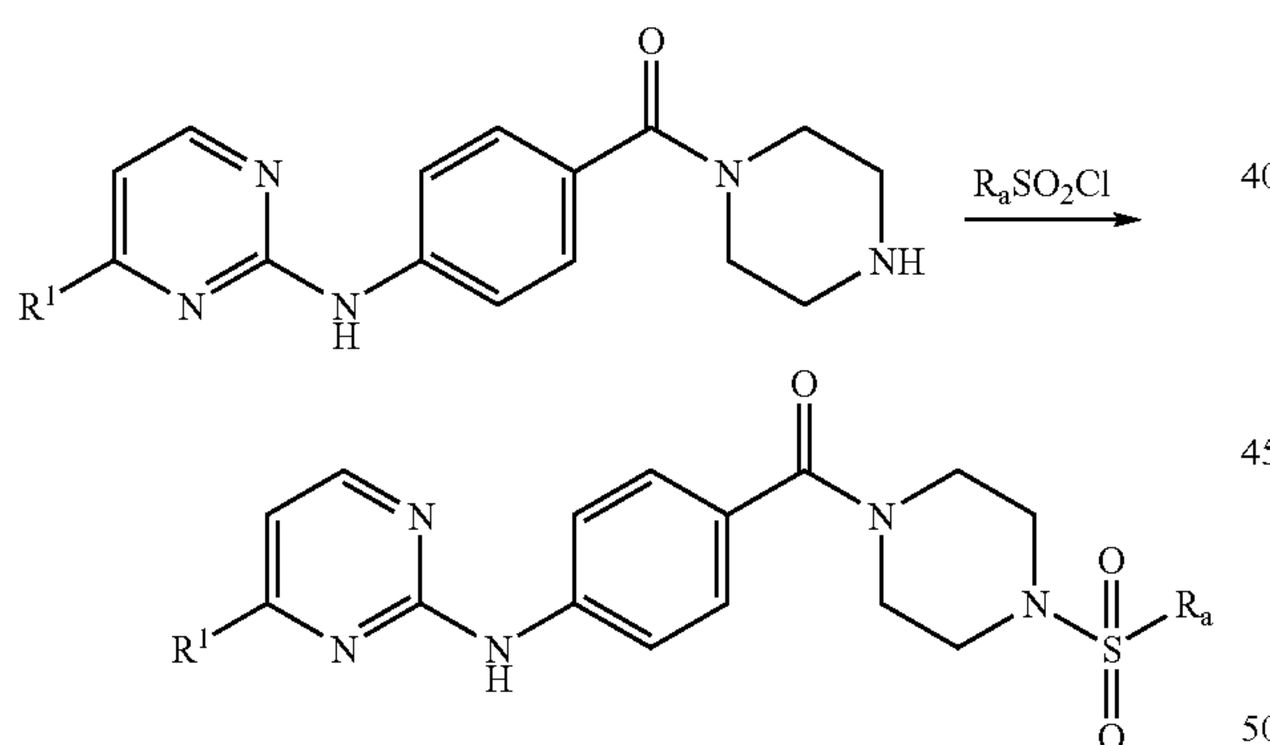
Reaction Scheme 6
