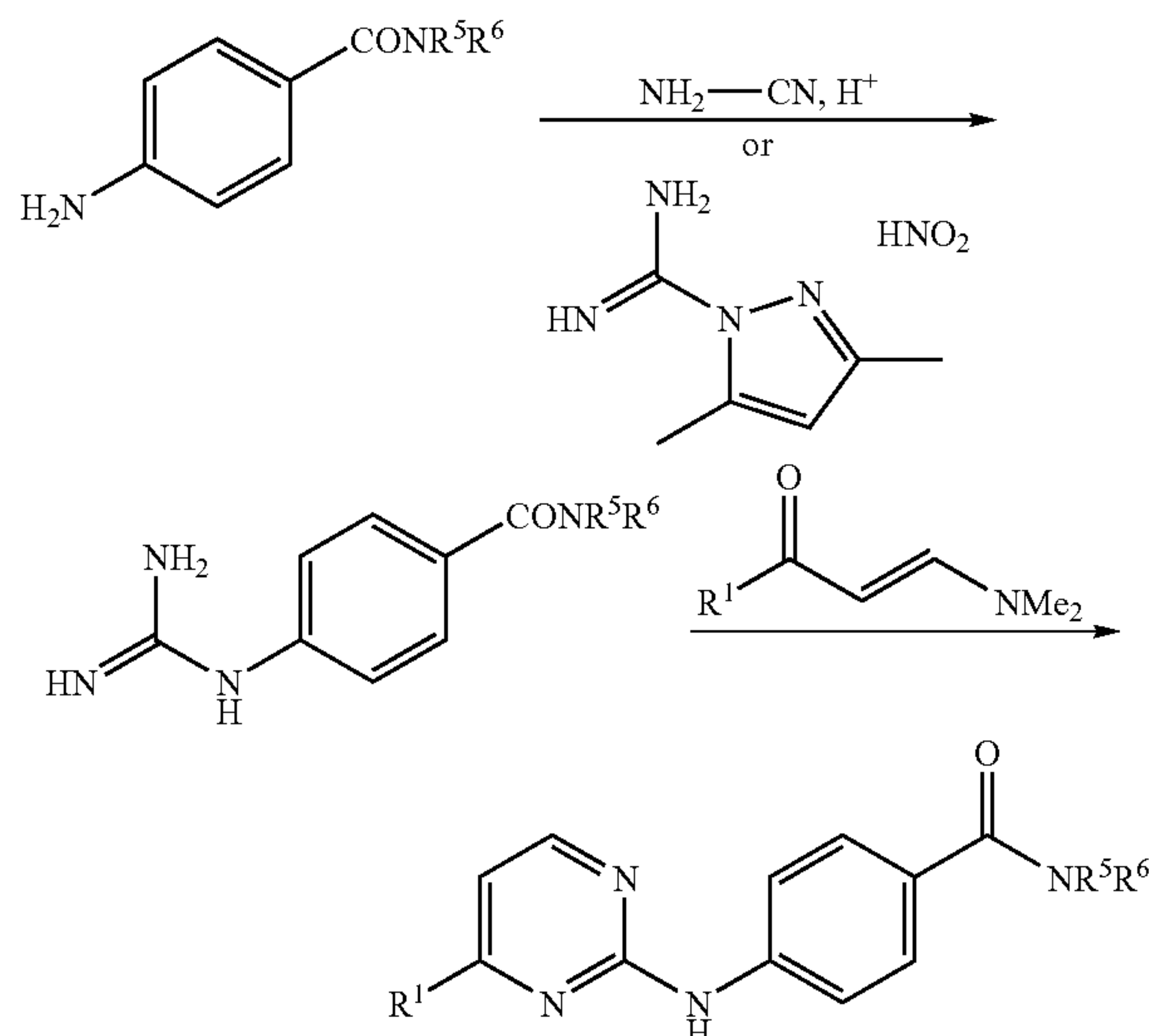
Reaction Scheme 3
