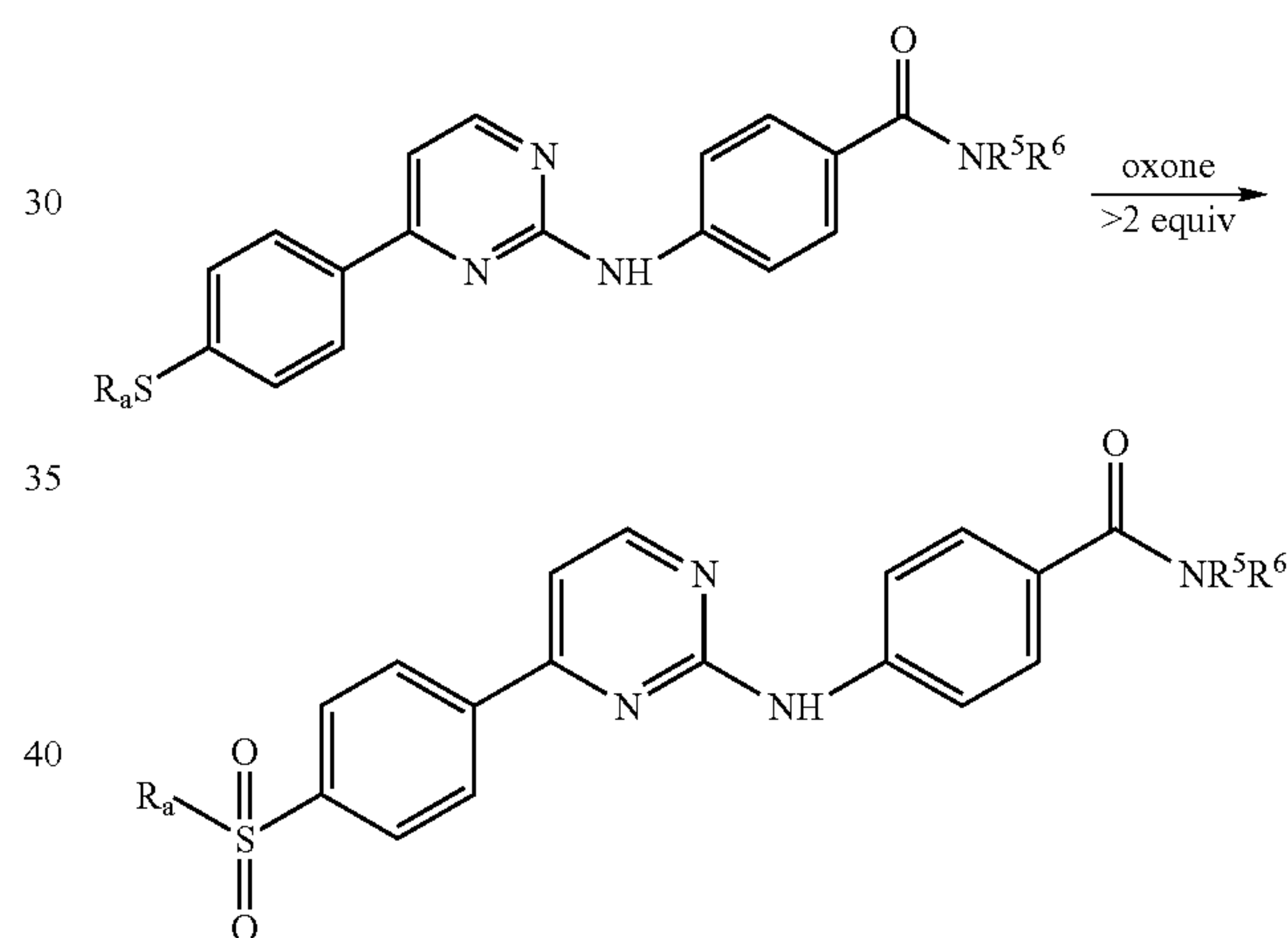
Reaction Scheme 9
