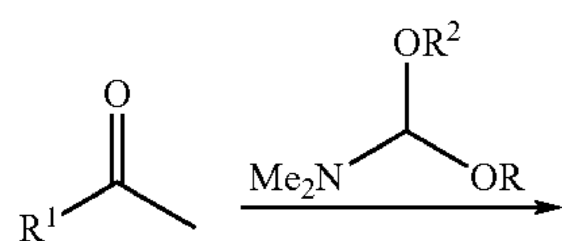
Reaction Scheme 2
