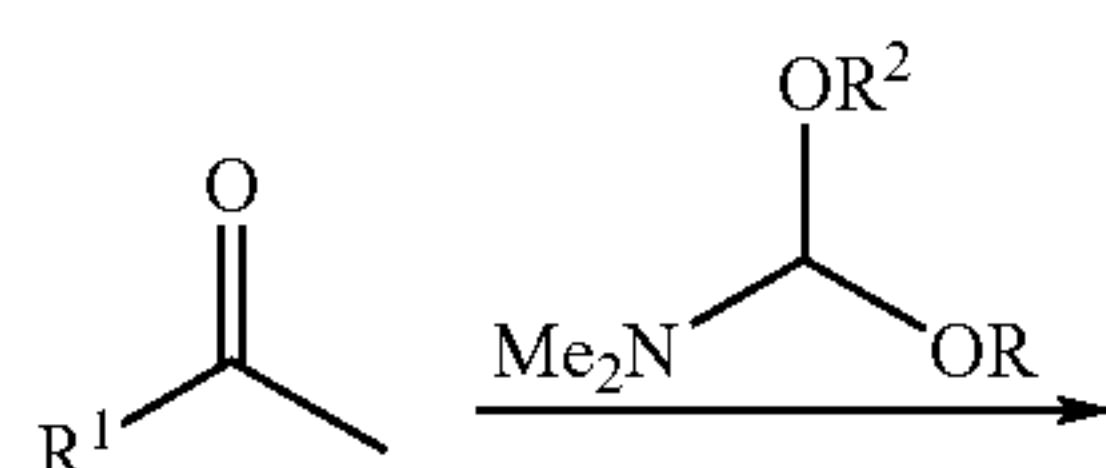
Reaction Scheme 2
