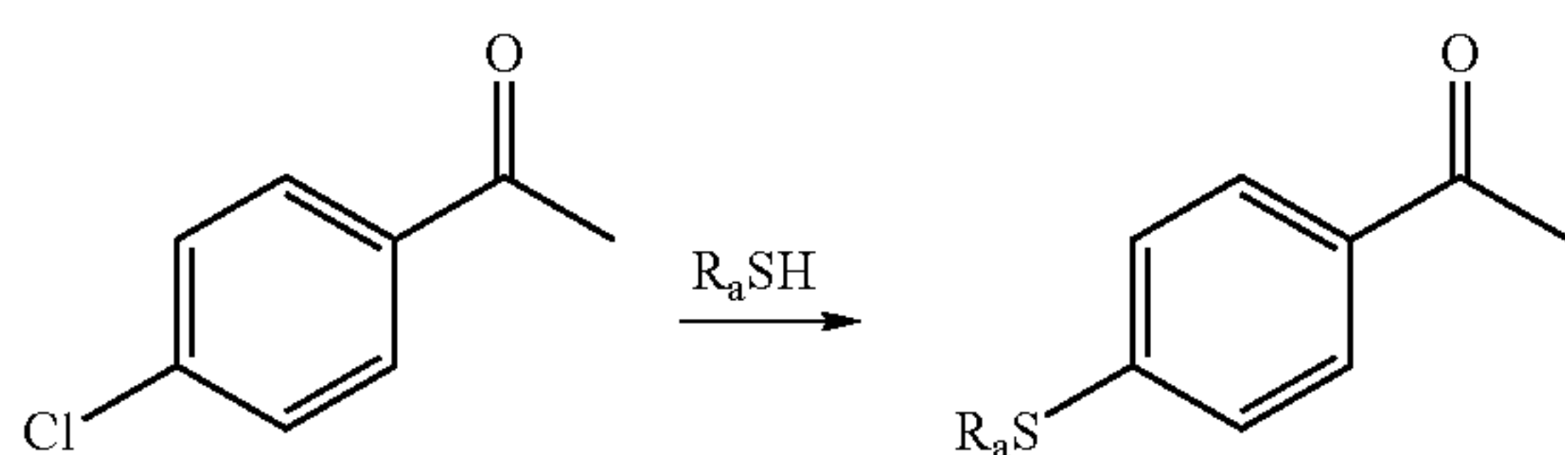
Reaction Scheme 7
