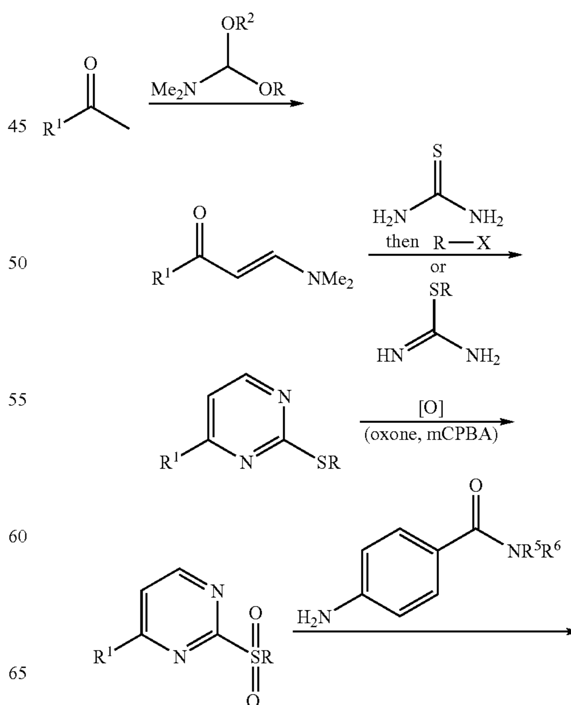
Reaction Scheme 1
