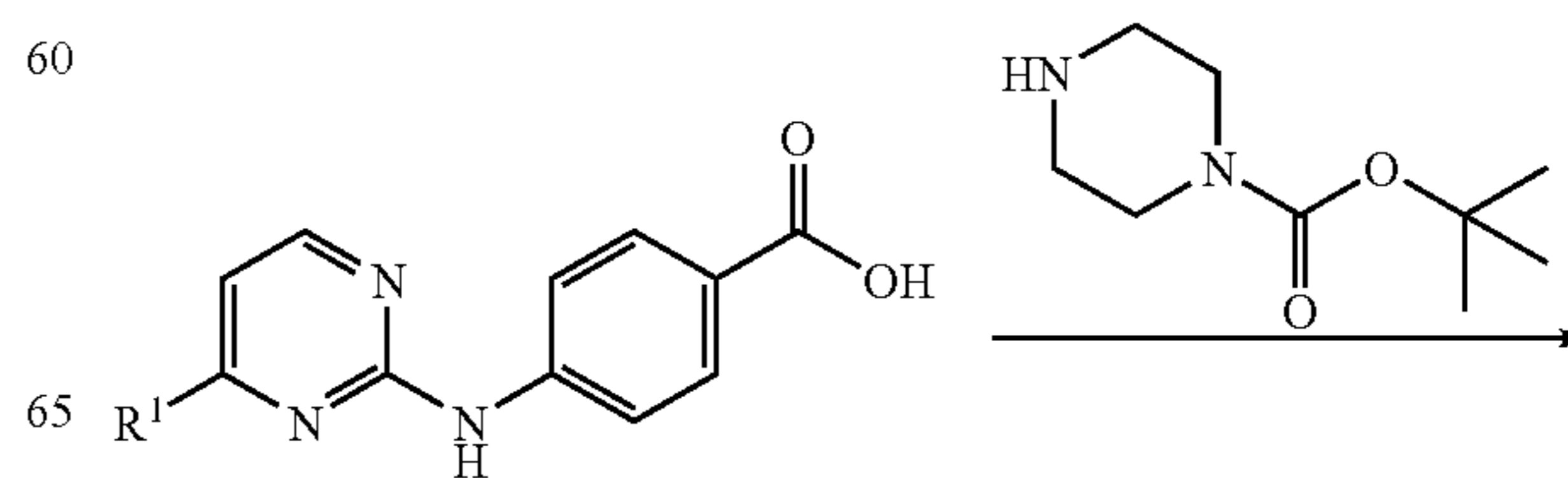
Reaction Scheme 5
