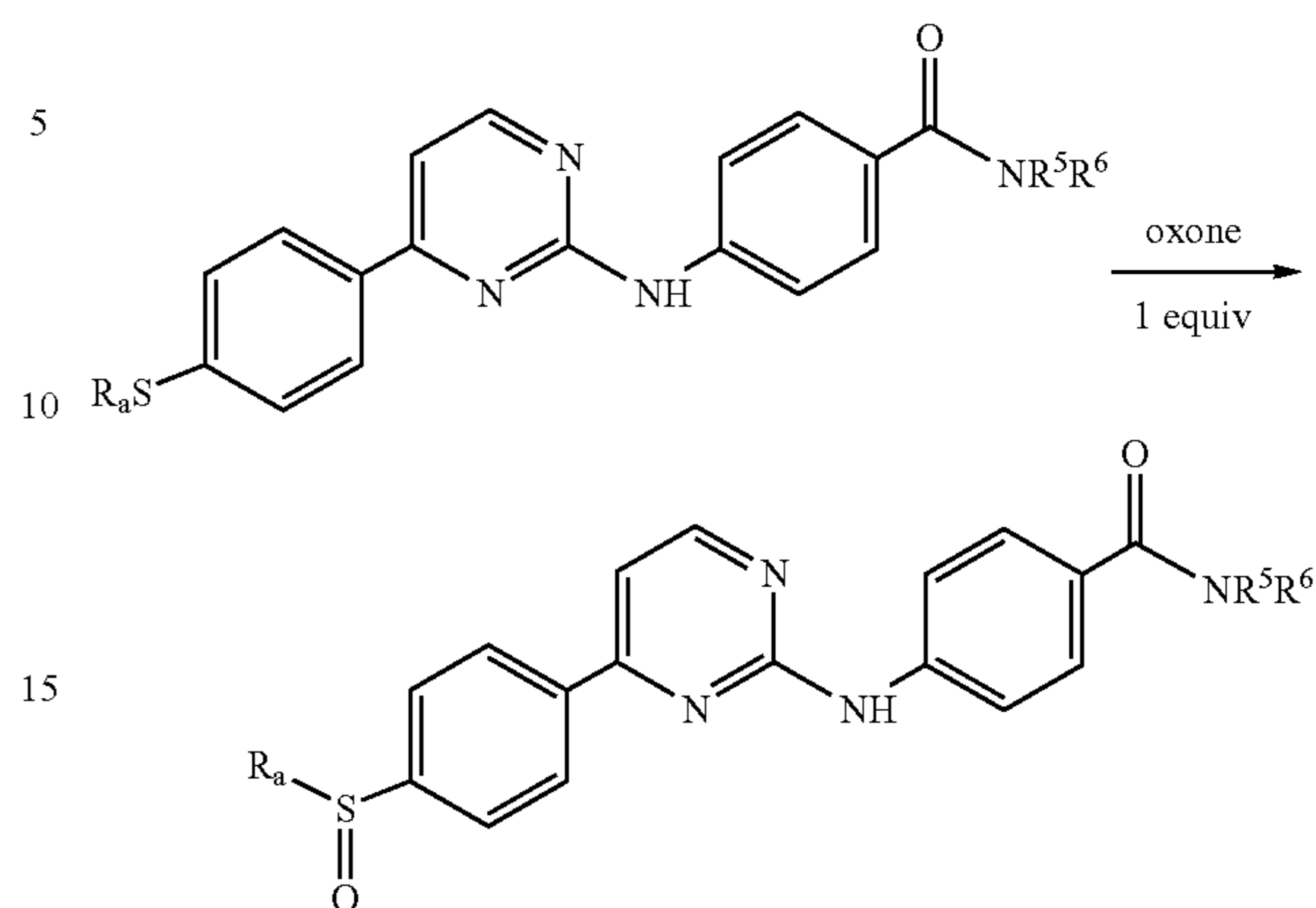
Reaction Scheme 8
