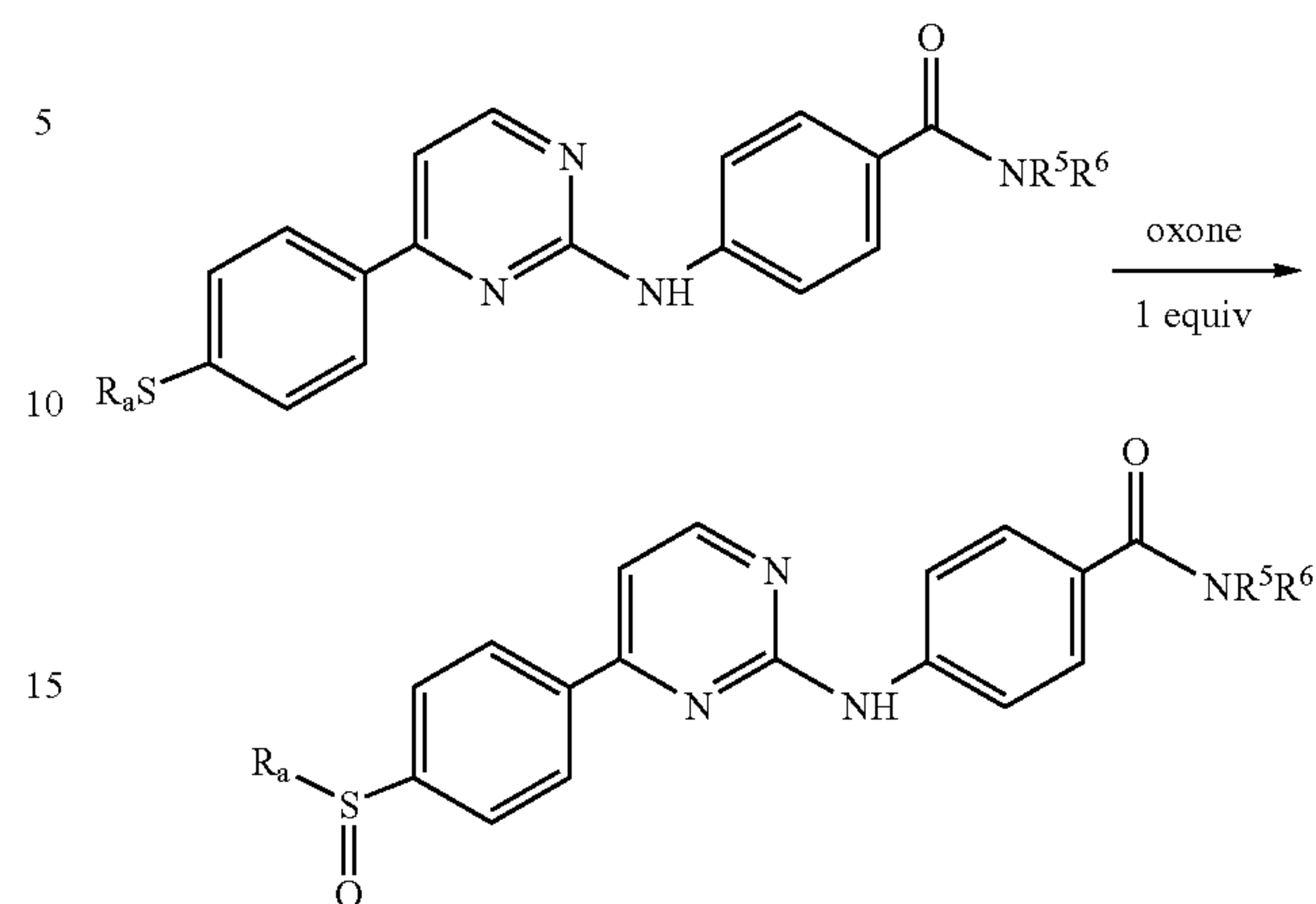
Reaction Scheme 8
