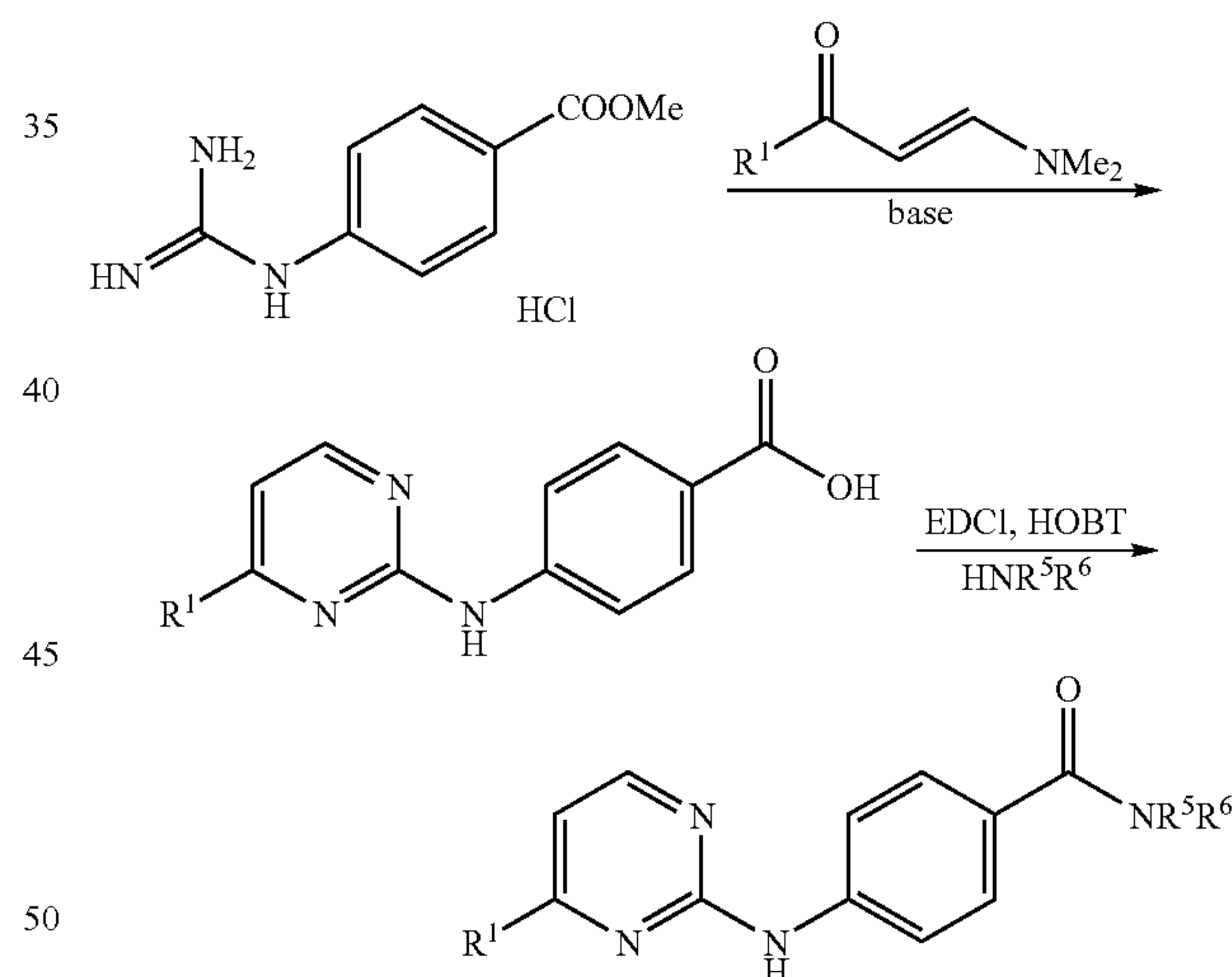
Reaction Scheme 4
