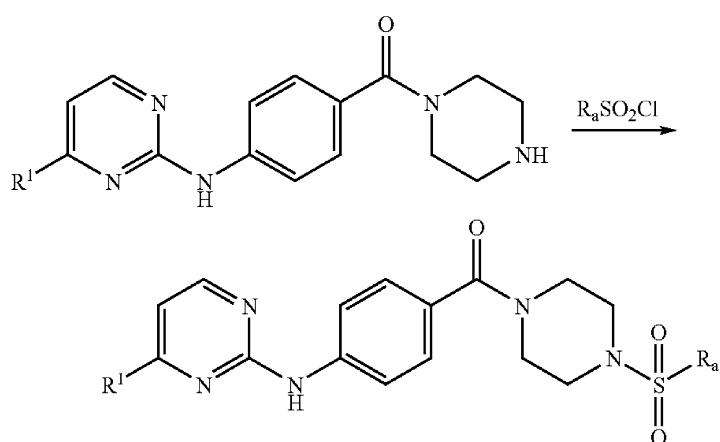
Reaction Scheme 6
