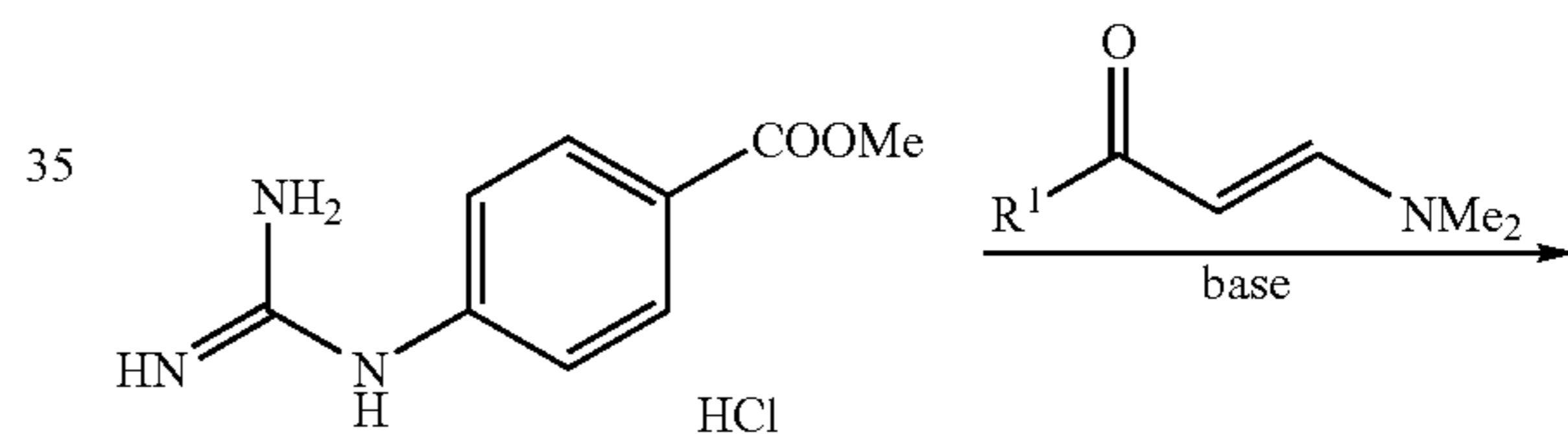
Reaction Scheme 4
