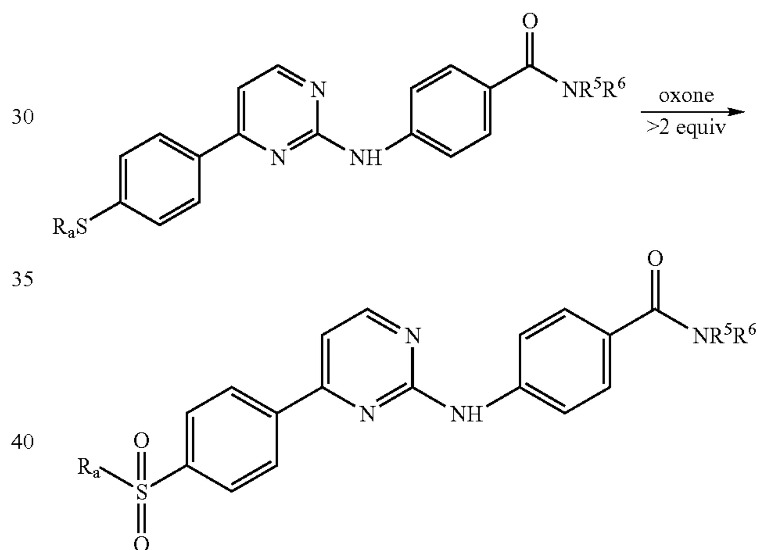
Reaction Scheme 9
