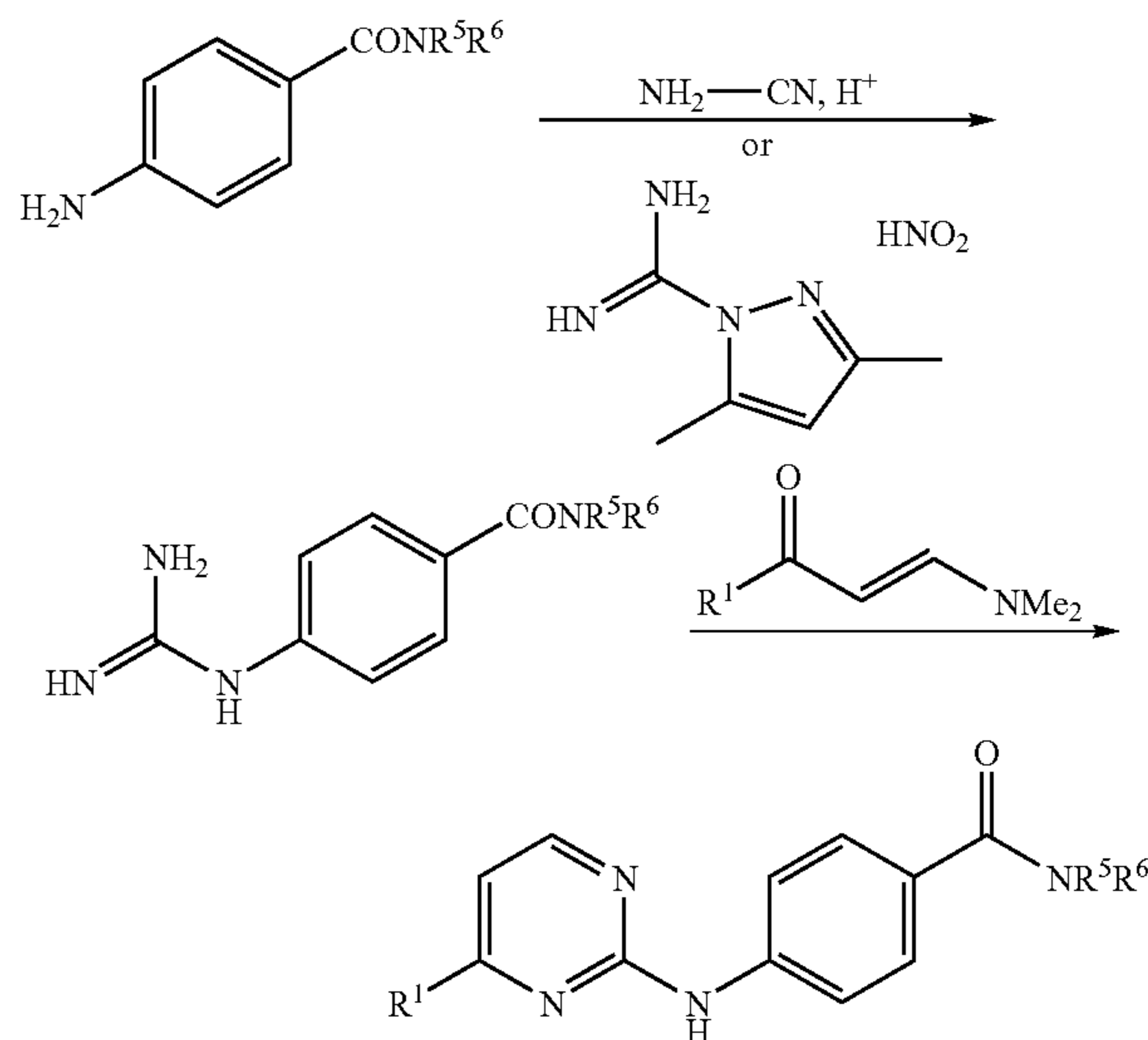
Reaction Scheme 3
