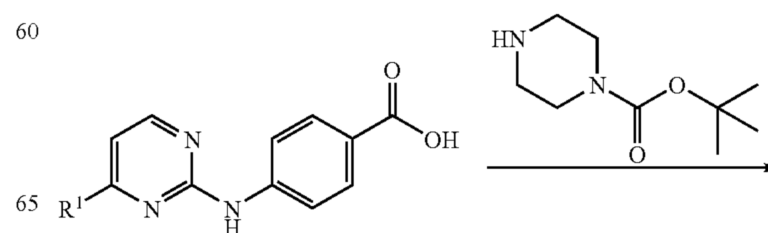
Reaction Scheme 5
