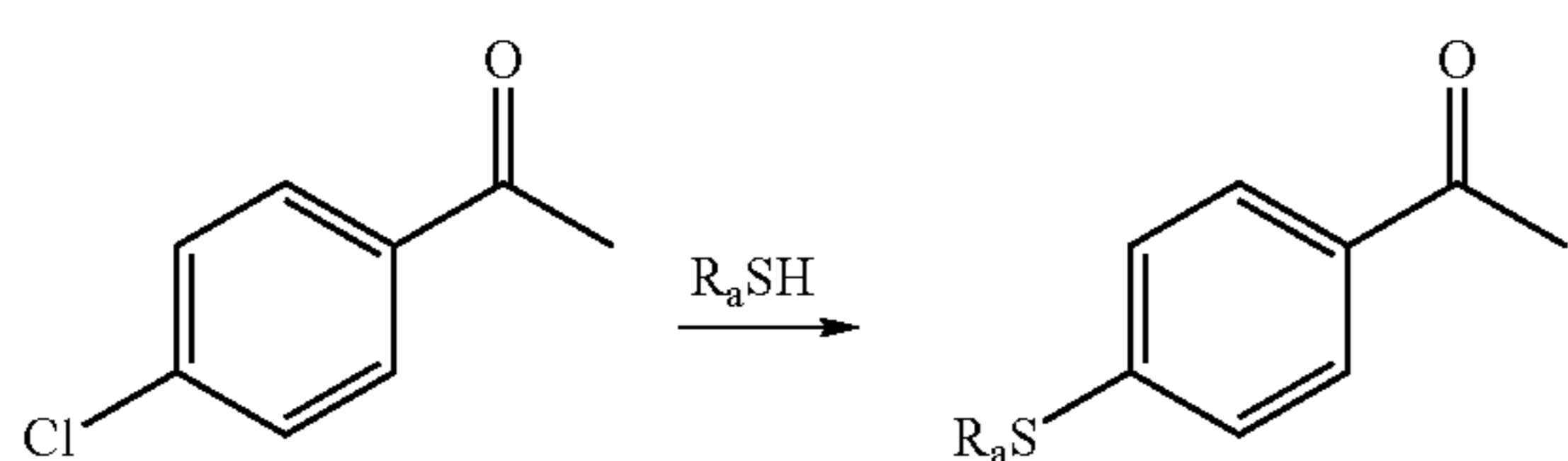
Reaction Scheme 7
