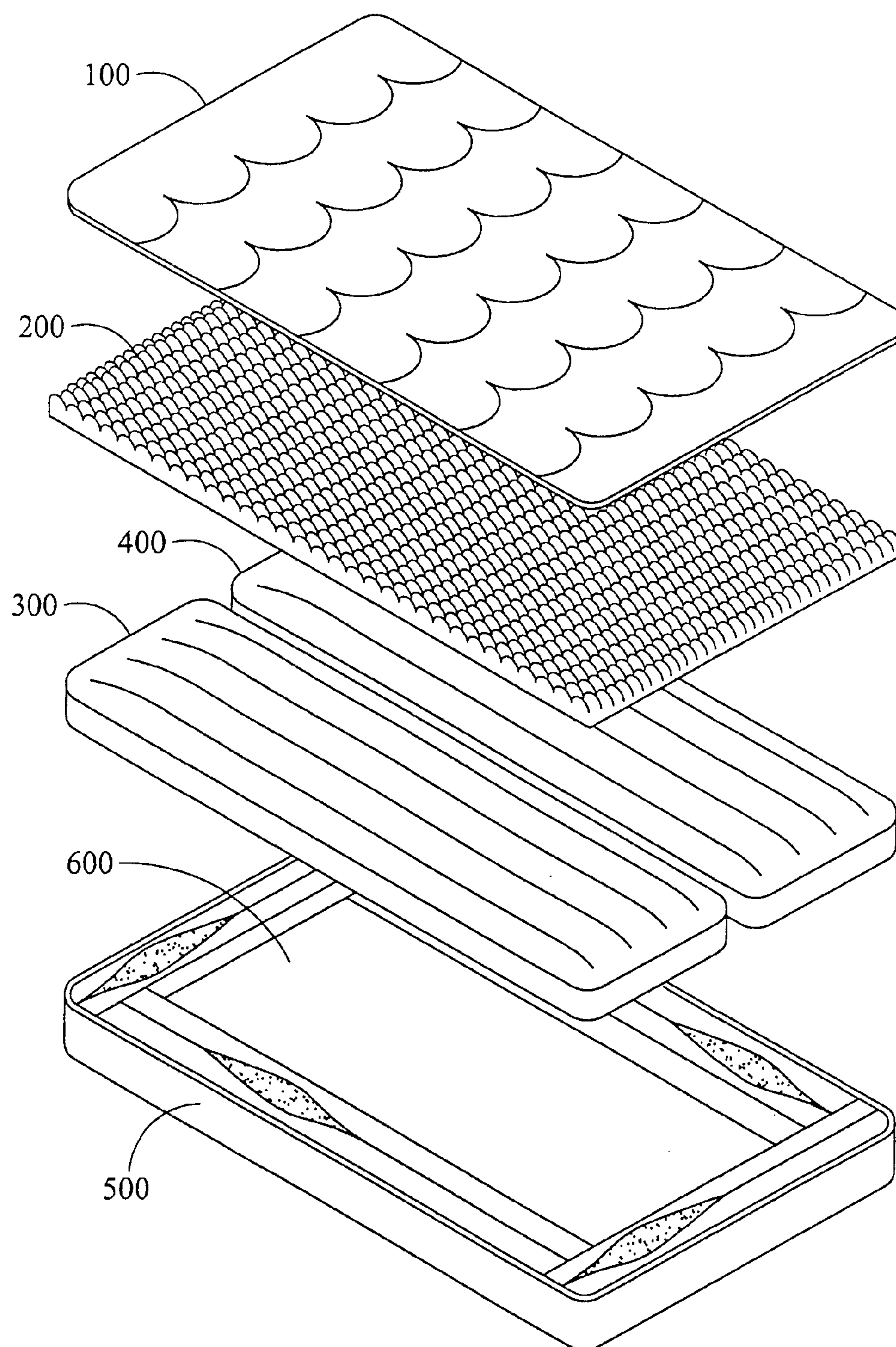
FIG. 11 ( PRIOR ART )
