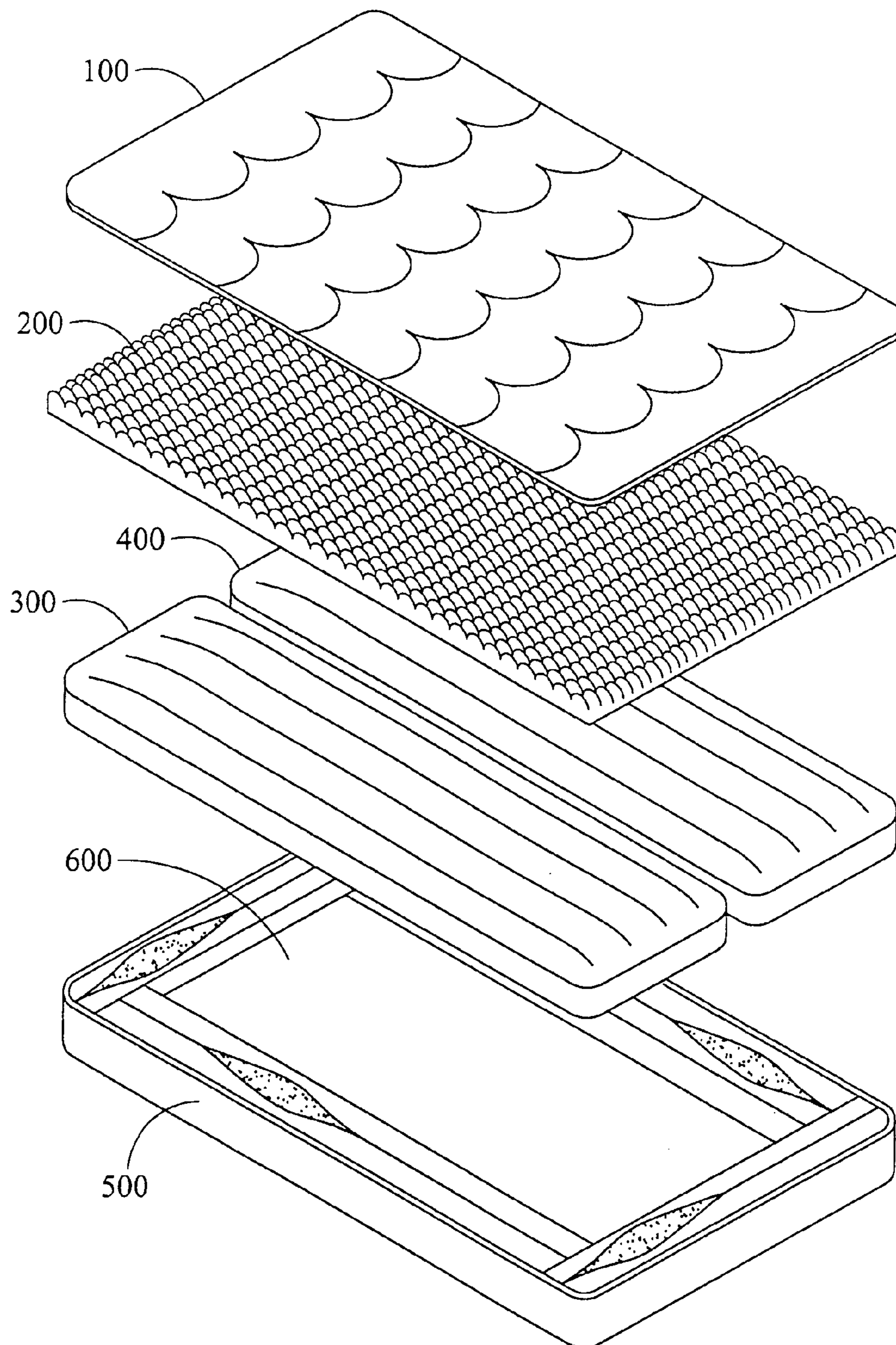
FIG. 11 ( PRIOR ART )
