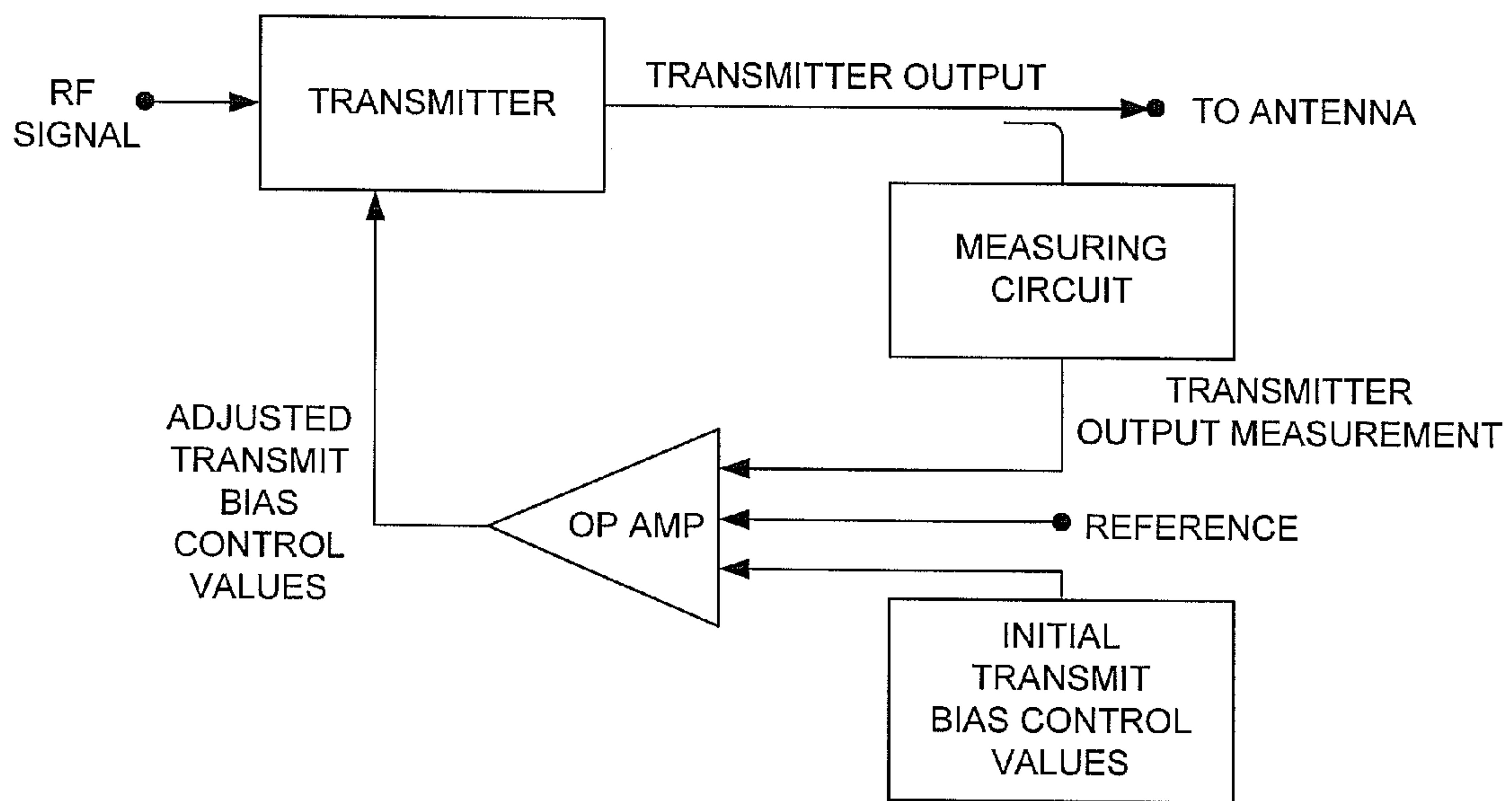
Fig. 1 (Prior Art)
