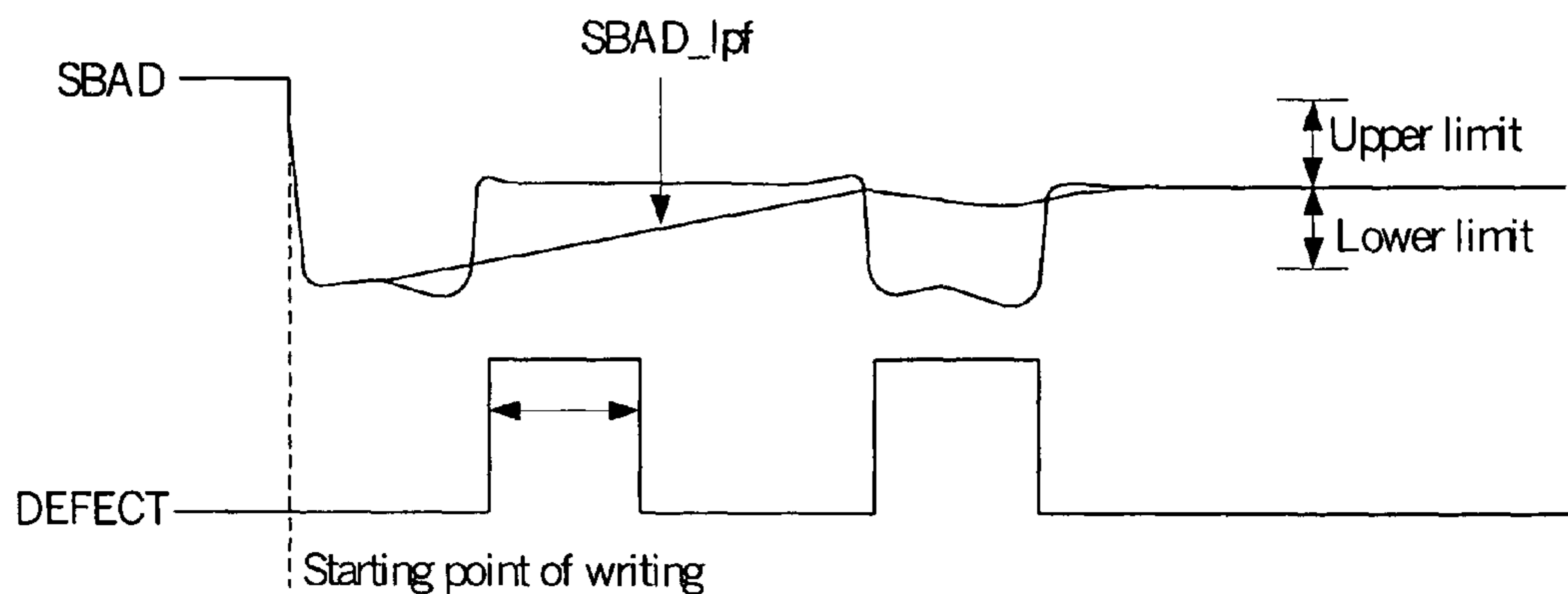
FIG. 5 (Prior Art)
