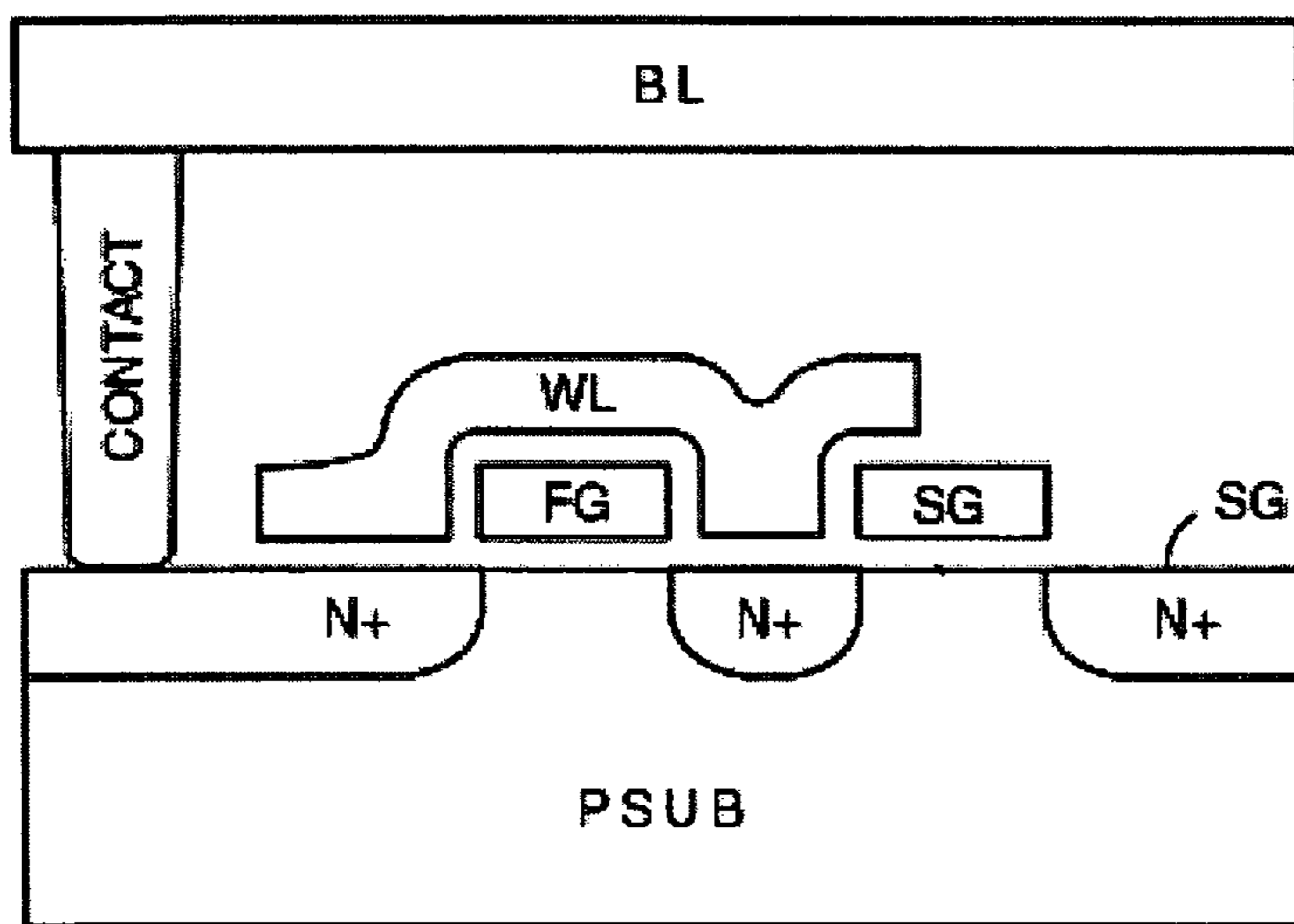
FIG. 5C (Prior Art)
