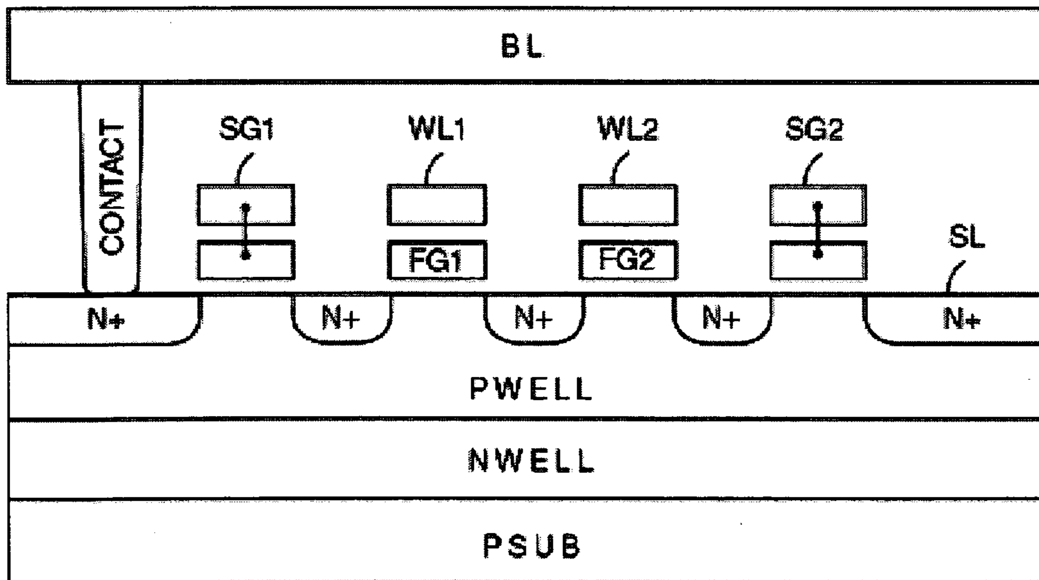
FIG. 3C (Prior Art)
