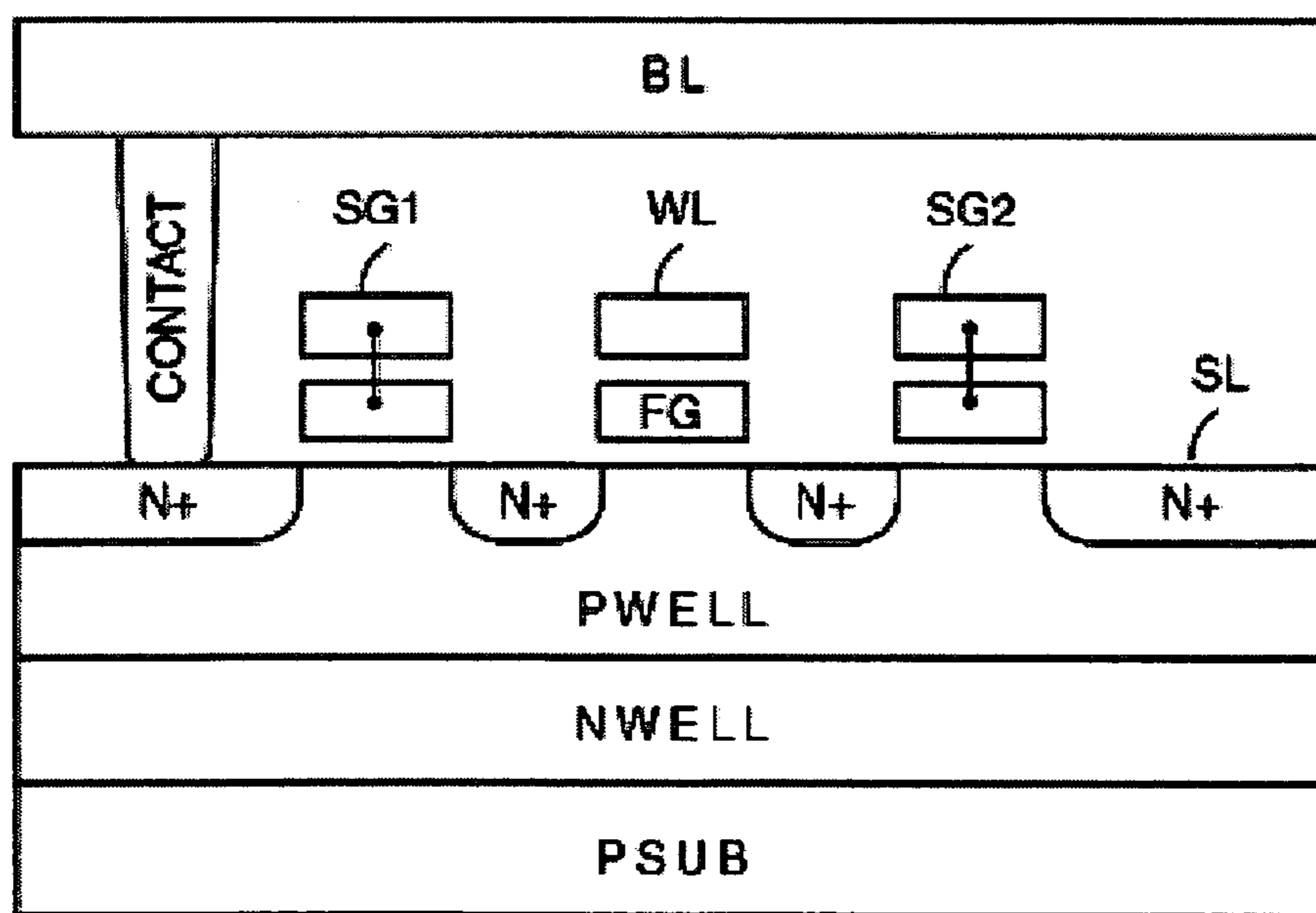
FIG. 2C (Prior Art)
