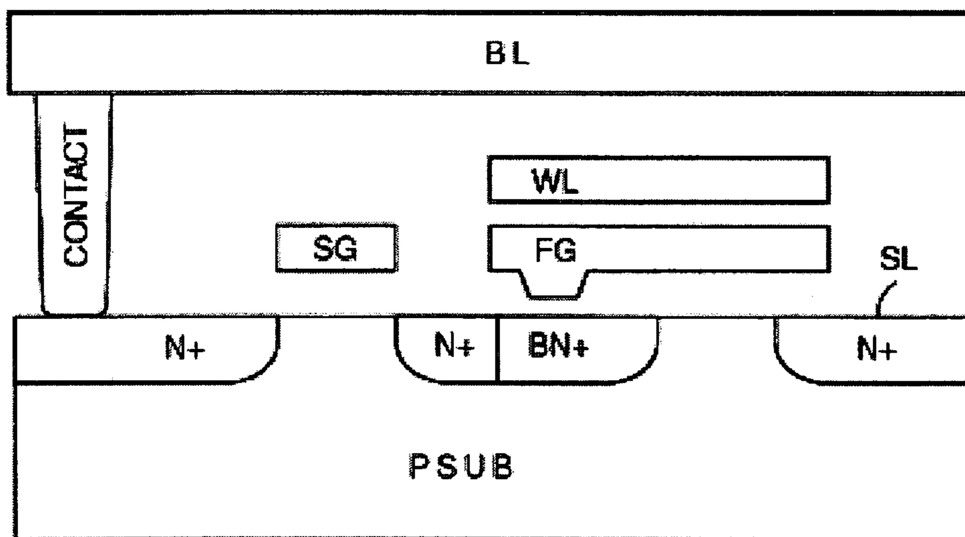
FIG. 1C (Prior Art)
