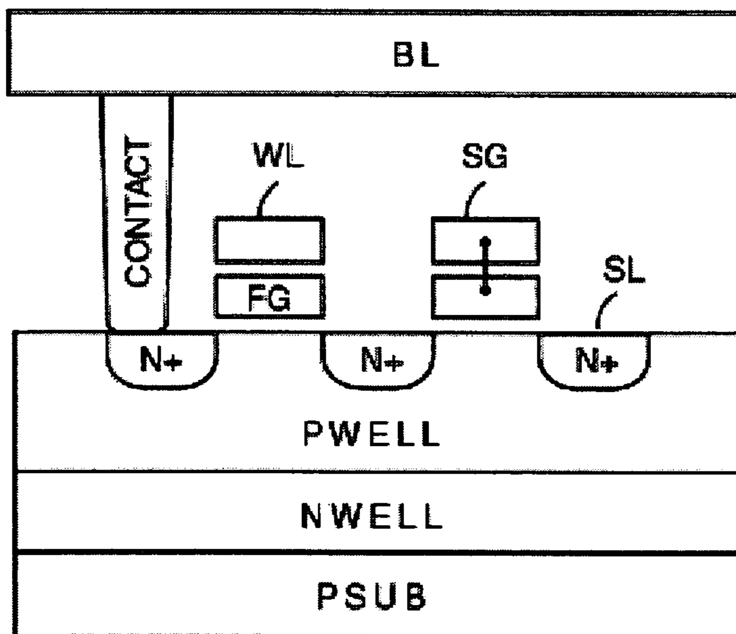
FIG. 4C (Prior Art)
