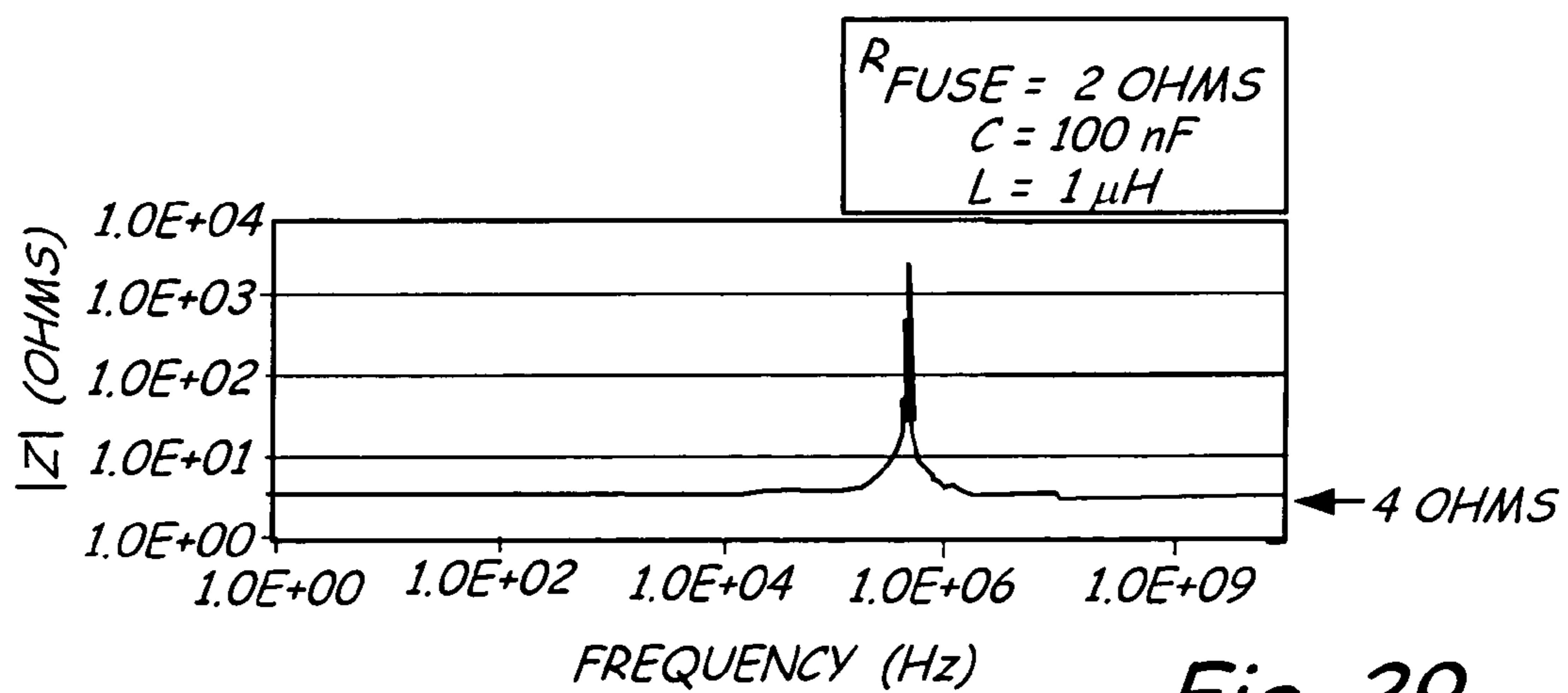
IMPEDANCE VS FREQUENCY FOR BAND EXCLUDE SHUNT
