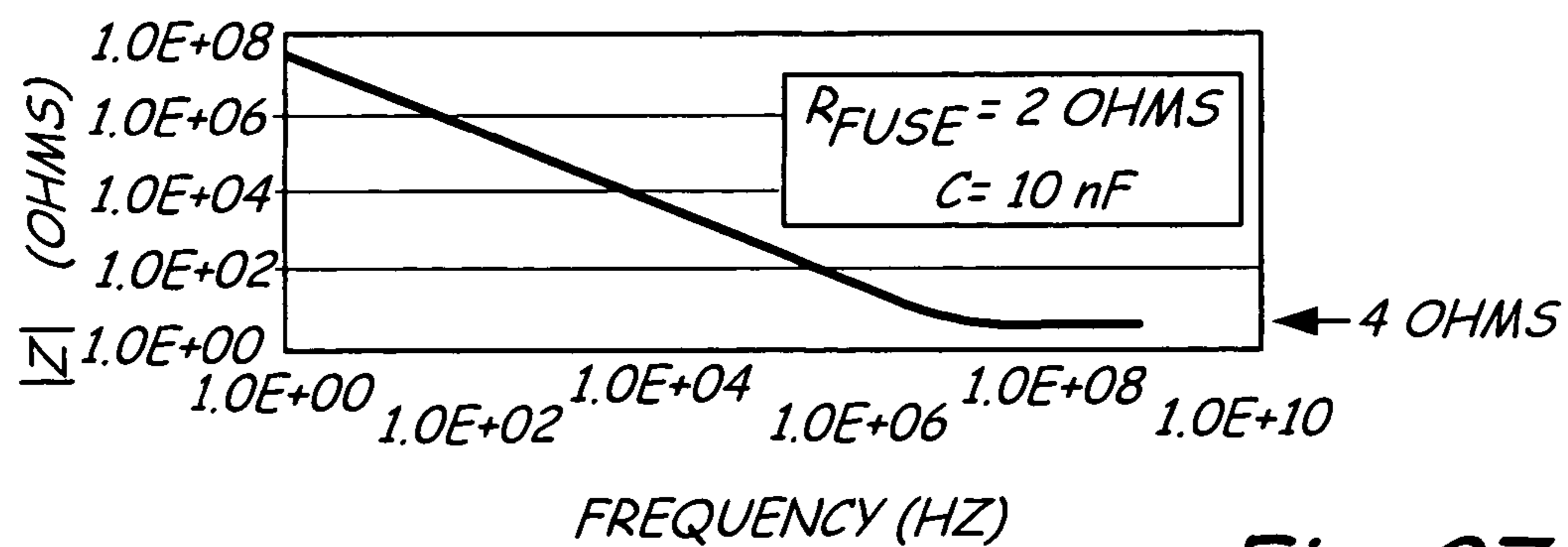
IMPEDANCE VS FREQUENCY FOR HIGH PASS SHUNT
