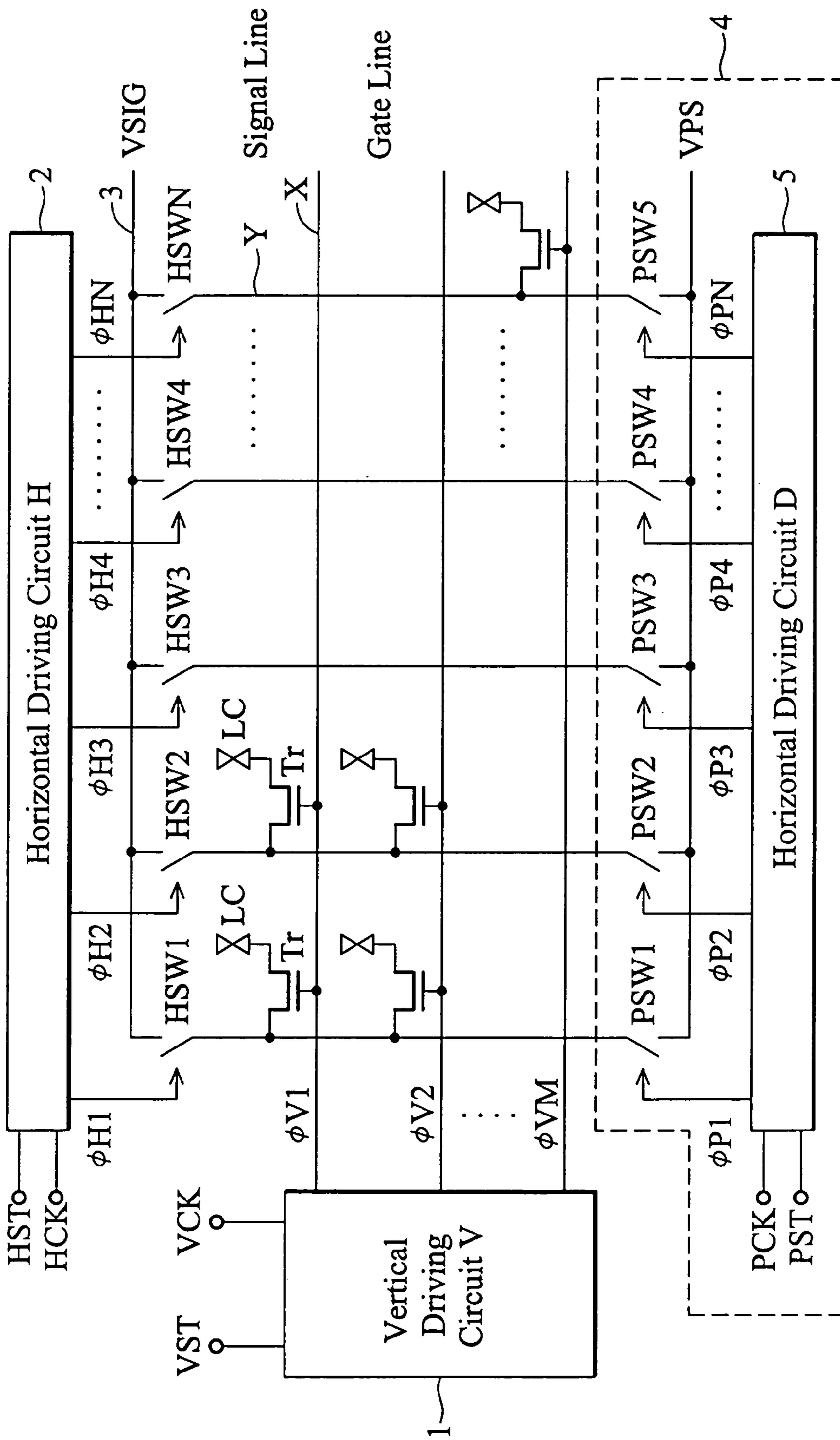
FIG. 1 (RELATED ART)
