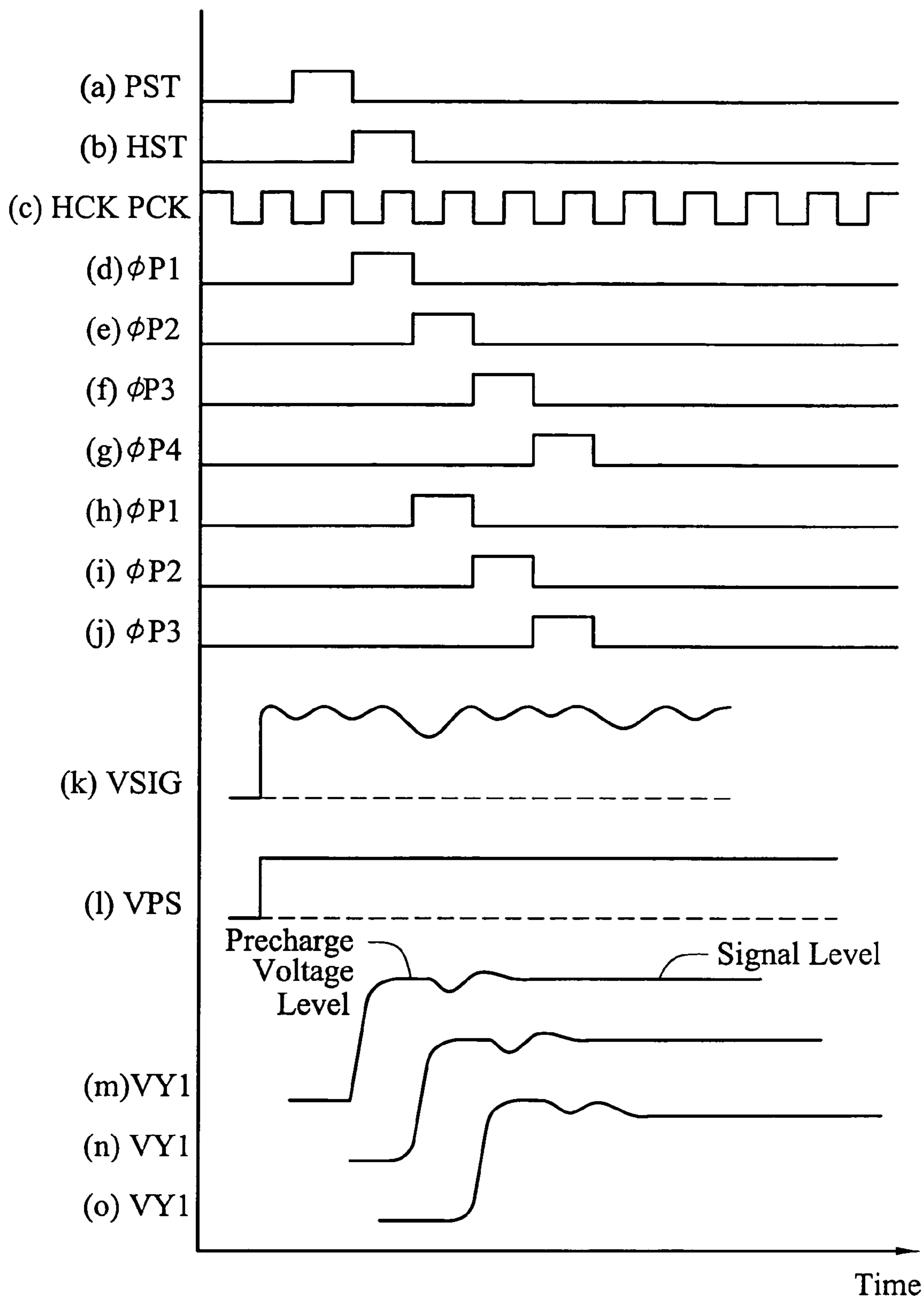
FIG. 2 (RELATED ART)
